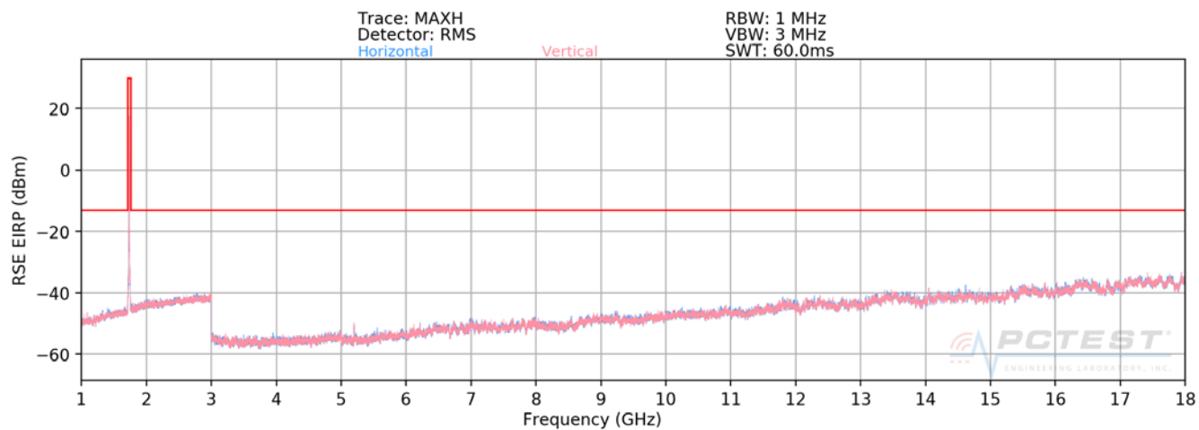
Plot 7-78. Radiated Spurious Plot above 1GHz (AWS WCDMA Mode) – CLOSED
