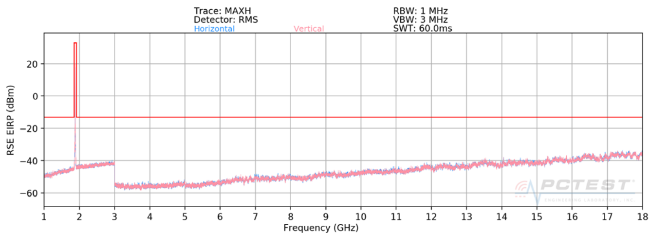
Plot 7-82. Radiated Spurious Plot above 1GHz (PCS WCDMA Mode) – CLOSED
