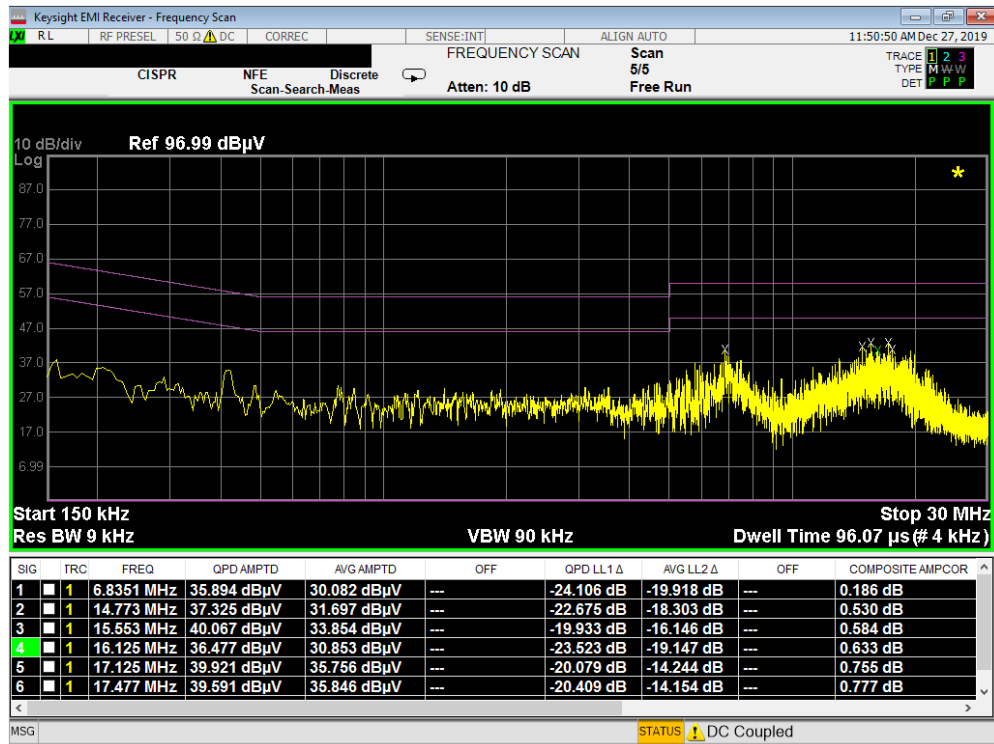
Plot 7-6. Line-Conducted Test Plot (L1) – OPEN
