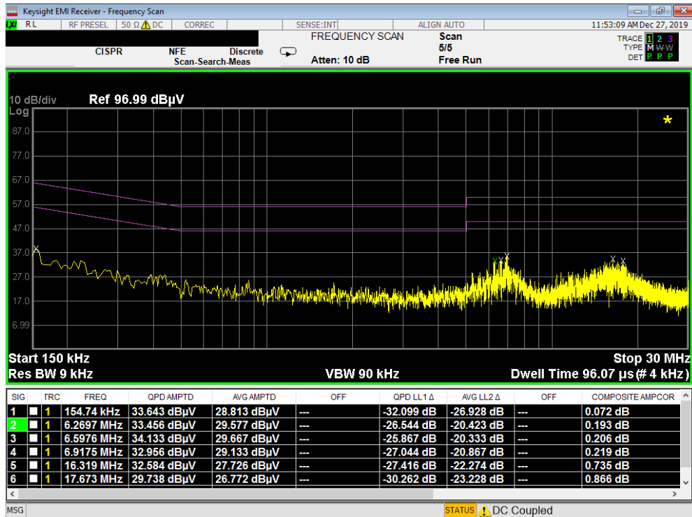
Plot 7-9. Line-Conducted Test Plot (N) – CLOSED
