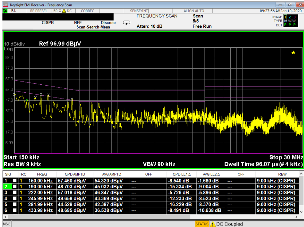
Plot 7-11. Line-Conducted Test Plot (N) – OPEN with WCP
