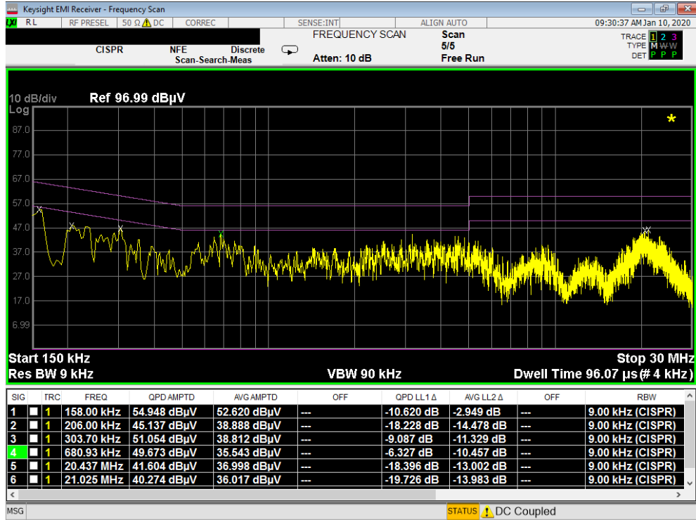
Plot 7-12. Line-Conducted Test Plot (L1) – CLOSED with WCP
