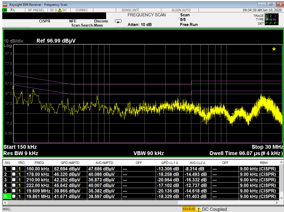
Plot 7-13. Line-Conducted Test Plot (N) – CLOSED with WCP
