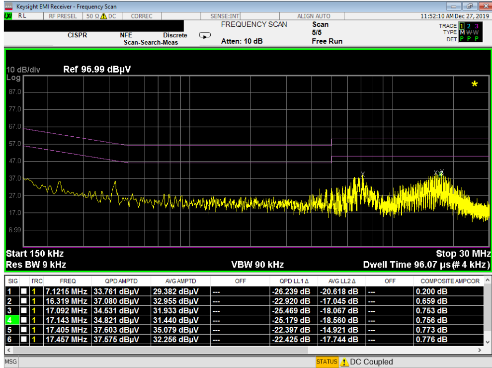
Plot 7-8. Line-Conducted Test Plot (L1) – CLOSED
