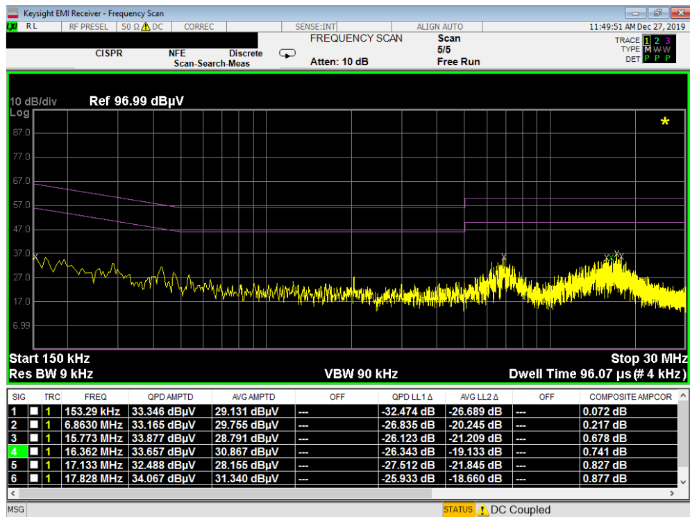
Plot 7-7. Line-Conducted Test Plot (N) – OPEN
