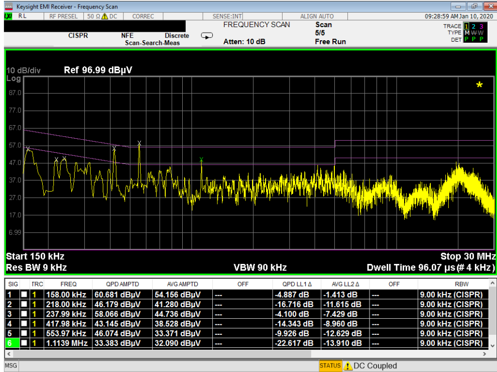
Plot 7-10. Line-Conducted Test Plot (L1) – OPEN with WCP
