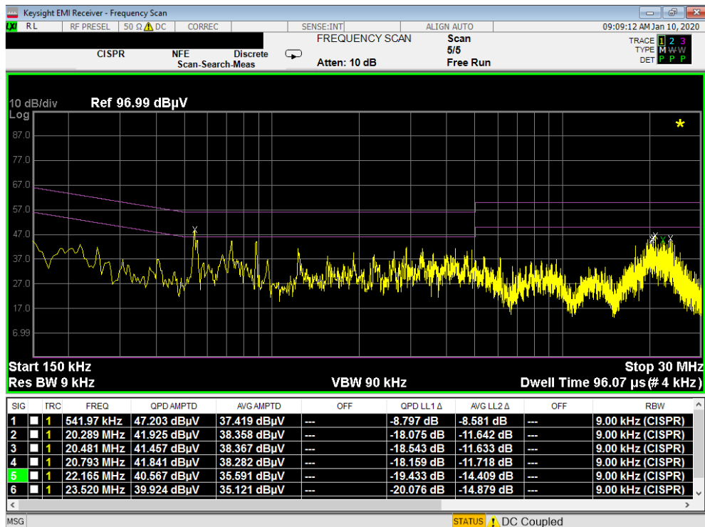
Plot 7-58. Line Conducted Plot with Bluetooth LE (N) – OPEN with WCP
