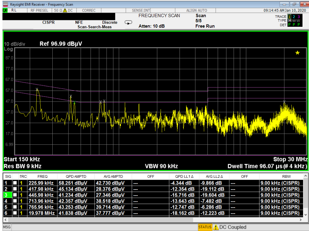
Plot 7-59. Line Conducted Plot with Bluetooth LE (L1) – CLOSED with WCP
