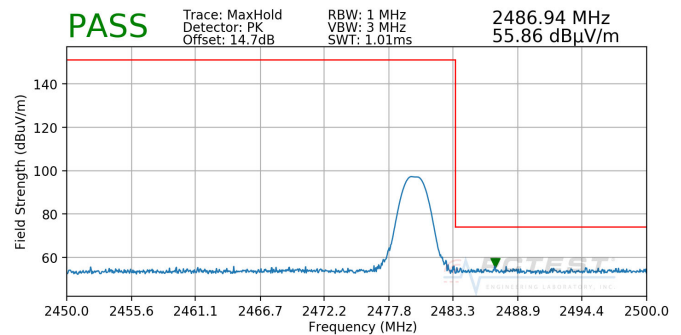
Plot 7-52. Radiated Restricted Upper Band Edge Measurement (Peak)
