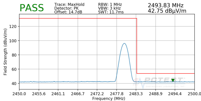
Plot 7-51. Radiated Restricted Upper Band Edge Measurement (Average)
