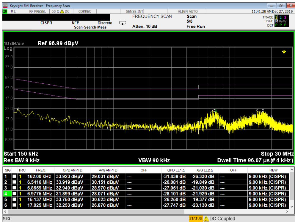
Plot 7-54. Line Conducted Plot with Bluetooth LE (N) – OPEN
