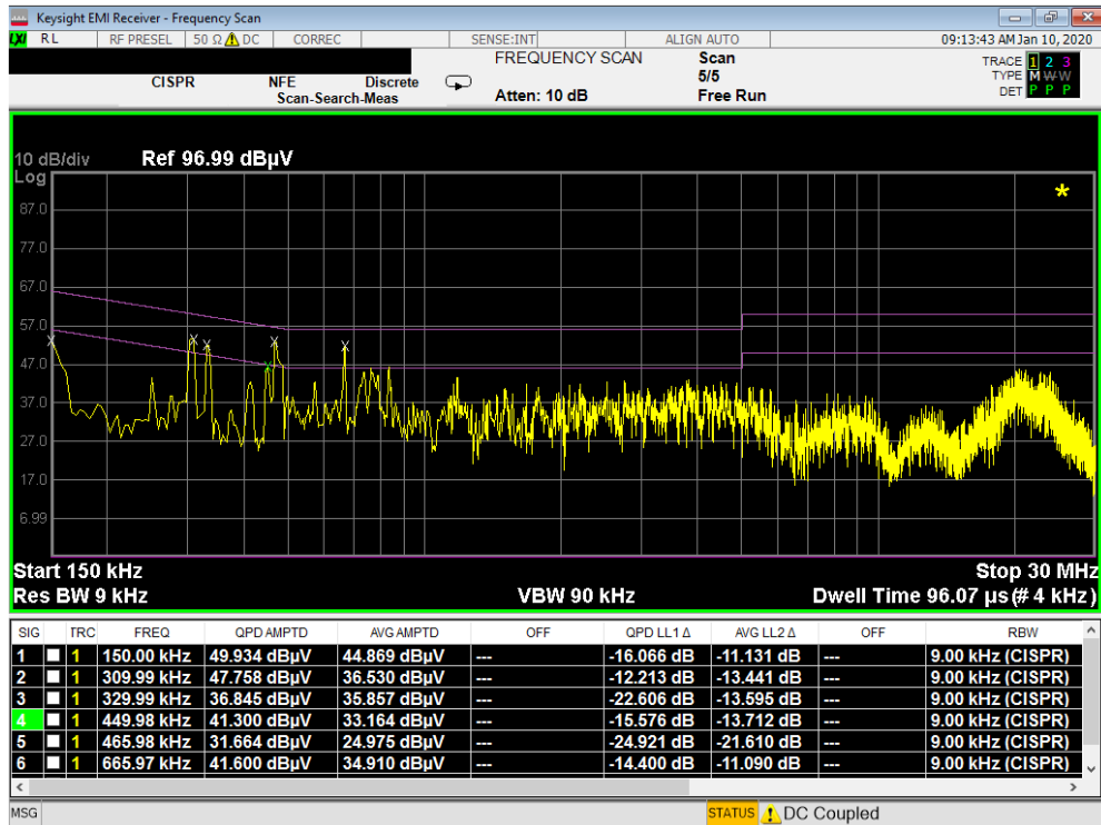
Plot 7-57. Line Conducted Plot with Bluetooth LE (L1) – OPEN with WCP
