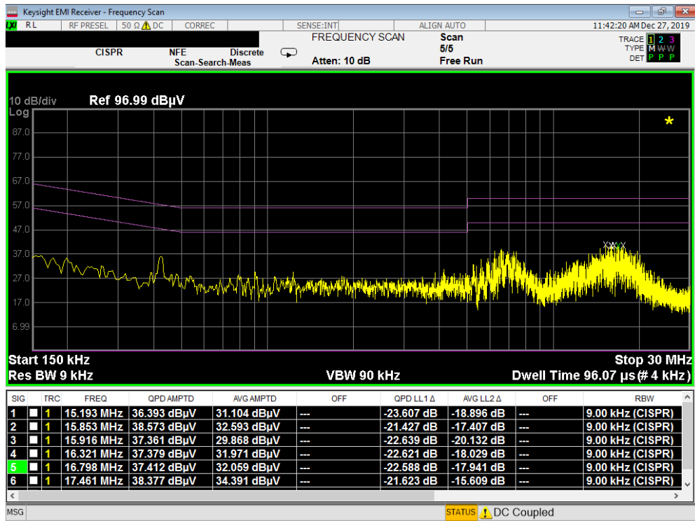
Plot 7-53. Line Conducted Plot with Bluetooth LE (L1) – OPEN
