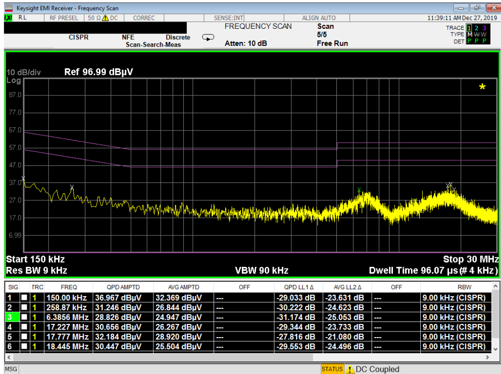
Plot 7-56. Line Conducted Plot with Bluetooth LE (N) – CLOSED
