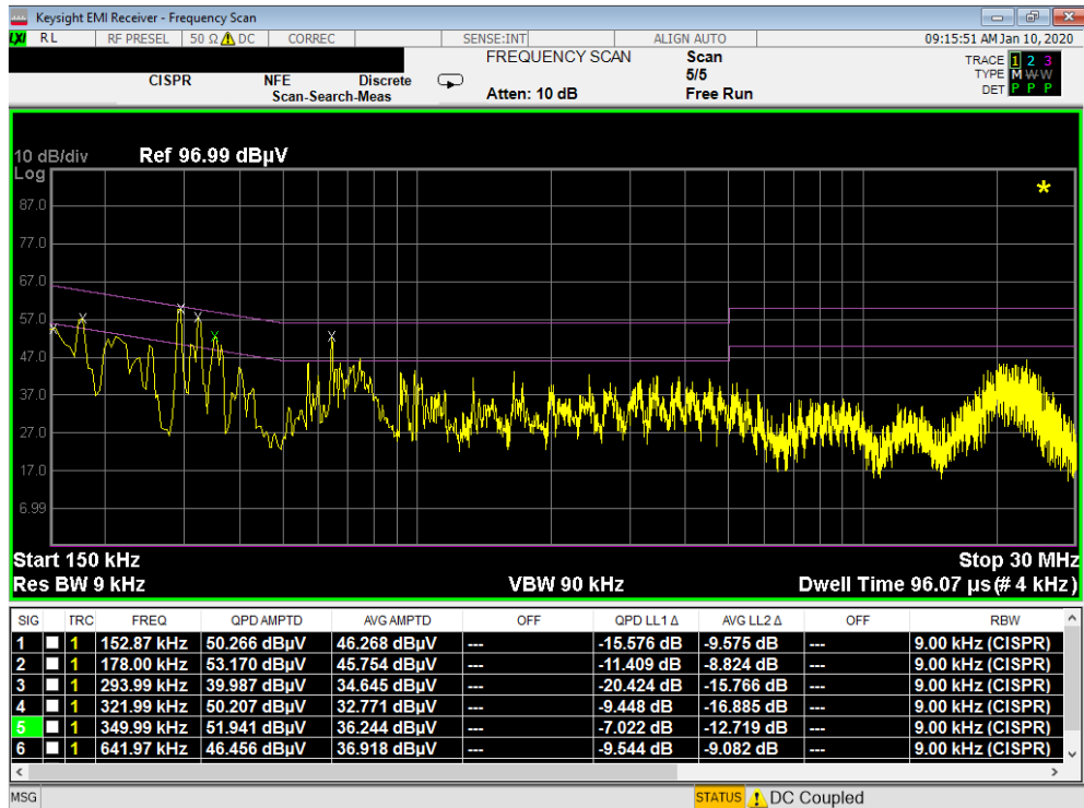
Plot 7-60. Line Conducted Plot with Bluetooth LE (N) – CLOSED with WCP
