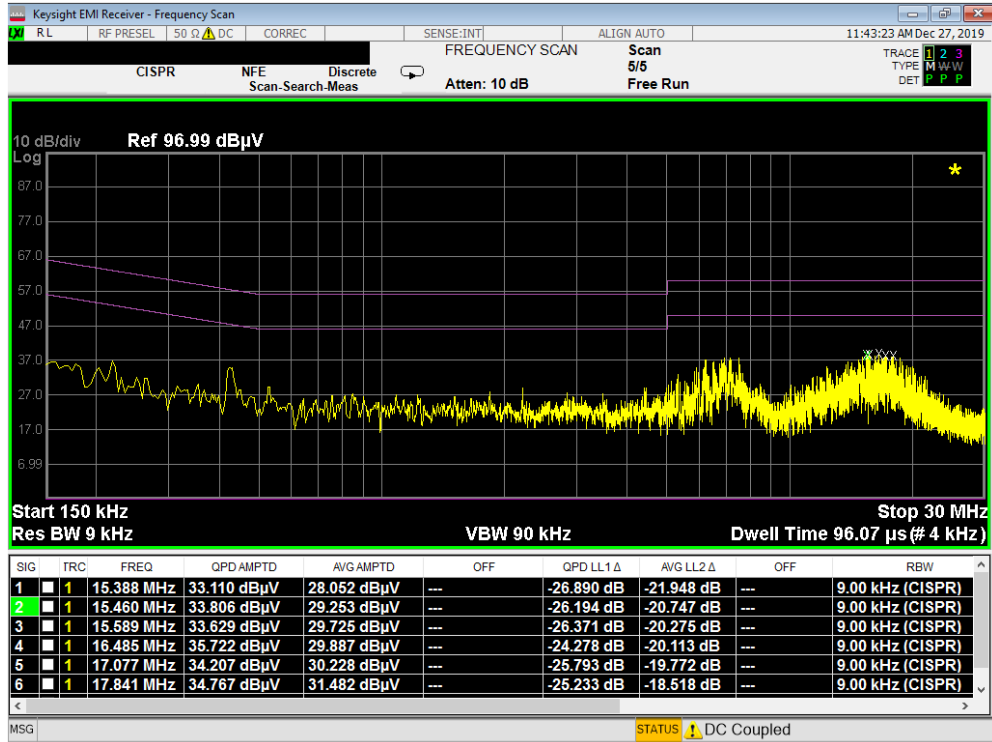
Plot 7-55. Line Conducted Plot with Bluetooth LE (L1) – CLOSED
