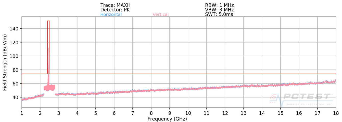
Plot 7-47. Radiated Spurious Plot above 1GHz (BT- Ch. 78) – CLOSED
