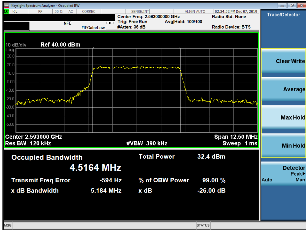
Plot 7-76. Occupied Bandwidth Plot (Band 41 PC3 - 5.0MHz QPSK - Full RB Configuration)
