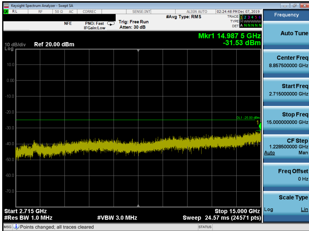
Plot 7-137. Conducted Spurious Plot (Band 41 PC3 - 20.0MHz QPSK - RB Size 1, RB Offset 0 - High Channel)
