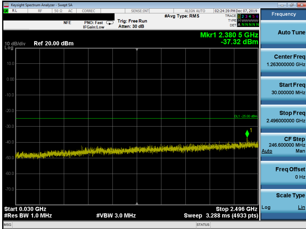
Plot 7-136. Conducted Spurious Plot (Band 41 PC3 - 20.0MHz QPSK - RB Size 1, RB Offset 0 - High Channel)
