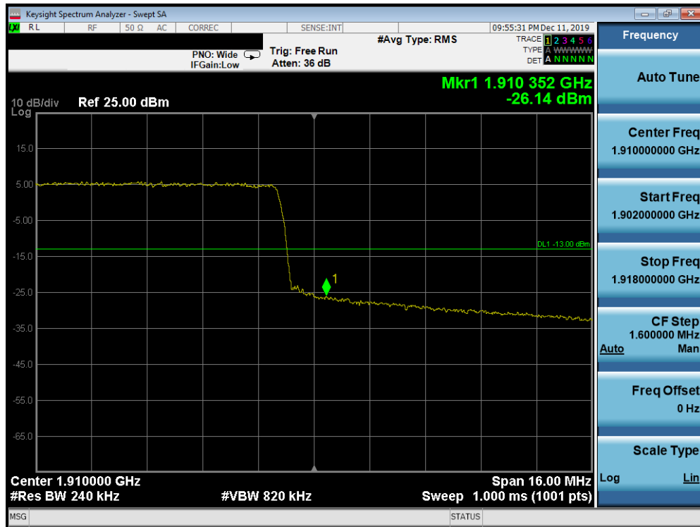
Plot 7-235. Upper Band Edge Plot (Band 2 – 20.0MHz QPSK - Full RB Configuration)
