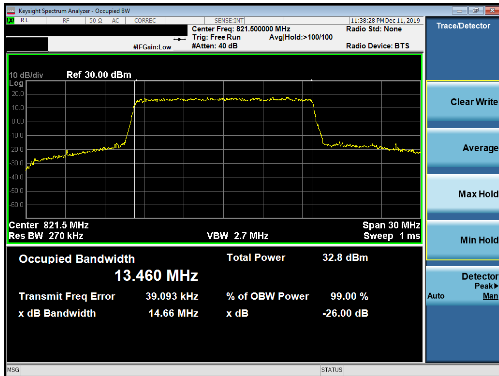
Plot 7-13. Occupied Bandwidth Plot (LTE Band 26 - 15MHz QPSK - Full RB Configuration)
