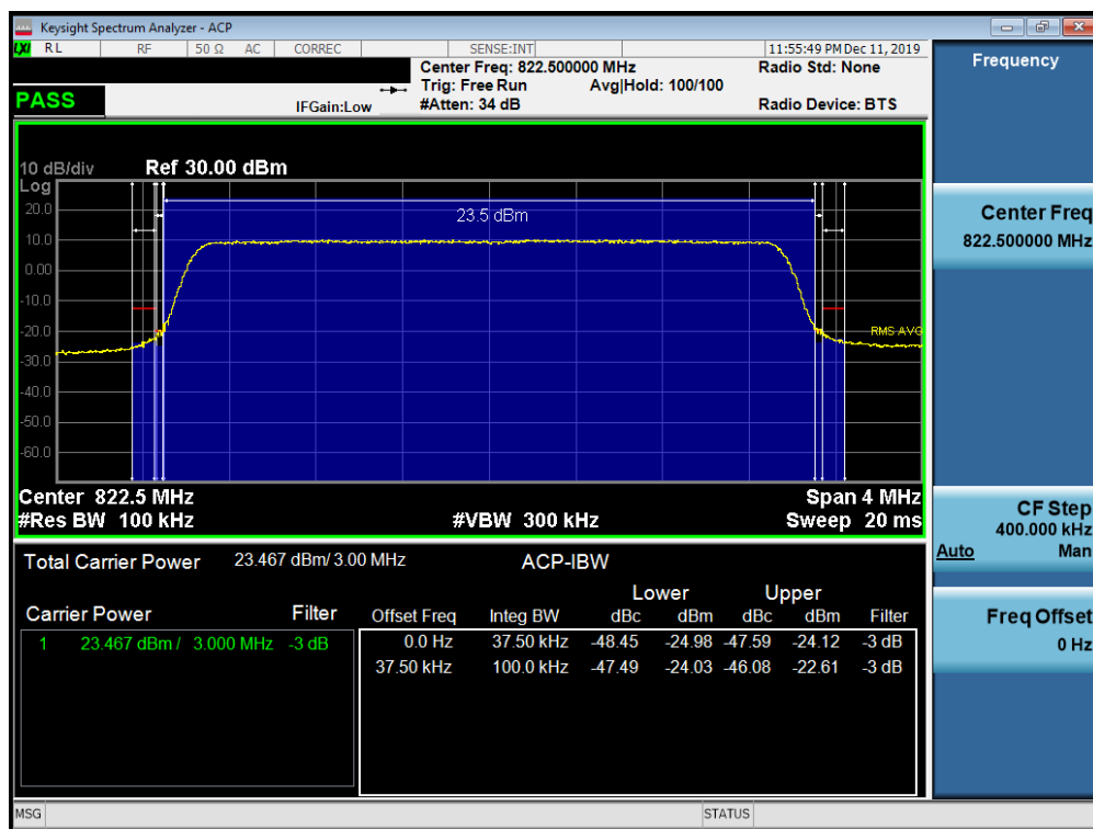
Plot 7-22. Channel Edge Plot (LTE Band 26 - 3MHz QPSK - High Channel)
