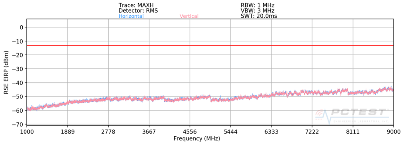
Plot 7-27. Radiated Spurious Plot (Band 26) - OPEN
