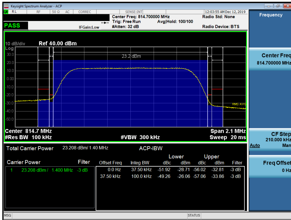
Plot 7-19. Channel Edge Plot (LTE Band 26 - 1.4MHz QPSK - Low Channel)
