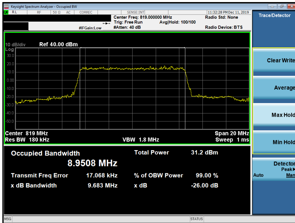
Plot 7-11. Occupied Bandwidth Plot (LTE Band 26 - 10MHz 16-QAM - Full RB Configuration)
