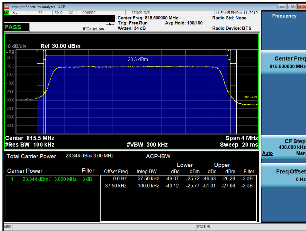
Plot 7-21. Channel Edge Plot (LTE Band 26 - 3MHz QPSK - Low Channel)
