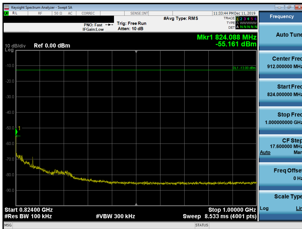
Plot 7-17. Conducted Spurious Plot (LTE Band 26 - 10MHz QPSK - RB Size 1, RB Offset 0 - Mid Channel)
