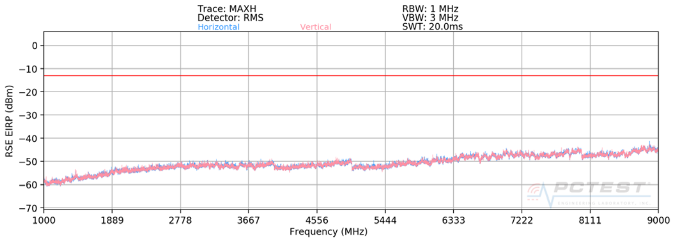
Plot 7-28. Radiated Spurious Plot (Band 26) - CLOSED
