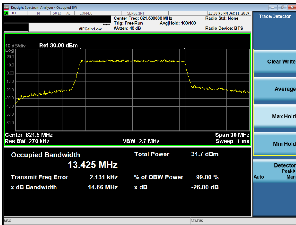
Plot 7-14. Occupied Bandwidth Plot (LTE Band 26 - 15MHz 16-QAM - Full RB Configuration)
