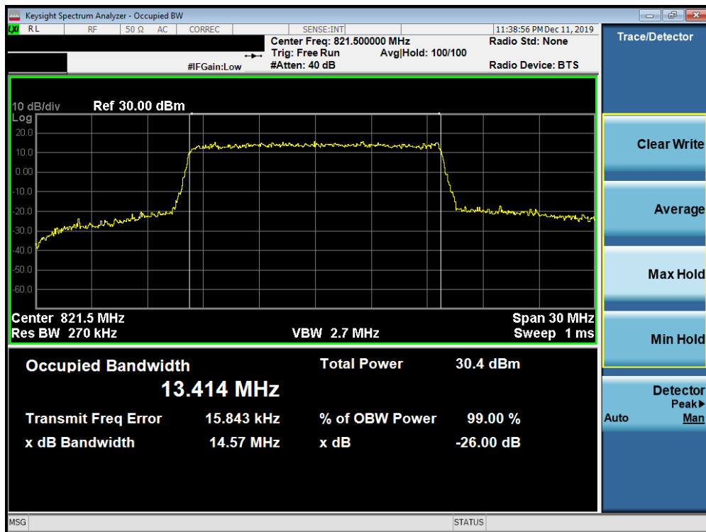
Plot 7-15. Occupied Bandwidth Plot (LTE Band 26 - 15MHz 64-QAM - Full RB Configuration)
