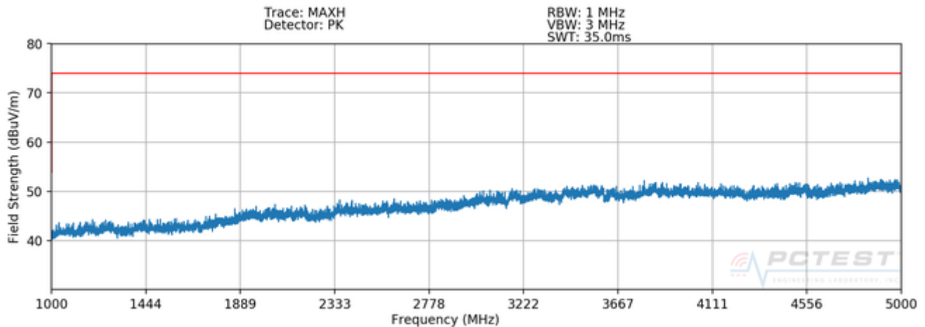
Plot 7-6. Radiated Spurious Plot above 1GHz – V – OPEN
