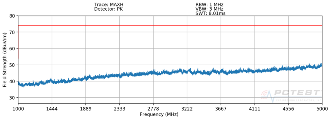
Plot 7-8. Radiated Spurious Plot above 1GHz – V – CLOSED
