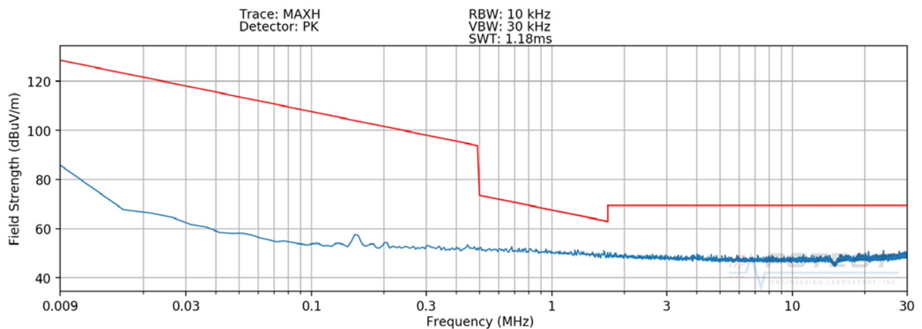
Plot 7-5 Radiated Spurious Plot 9kHz – 30MHz (Pol. Y – Device to Device WPT – CLOSED)
