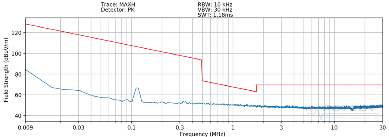
Plot 7-3. Radiated Spurious Plot 9kHz – 30MHz (Pol. Z – Device to Device WPT – OPEN)
