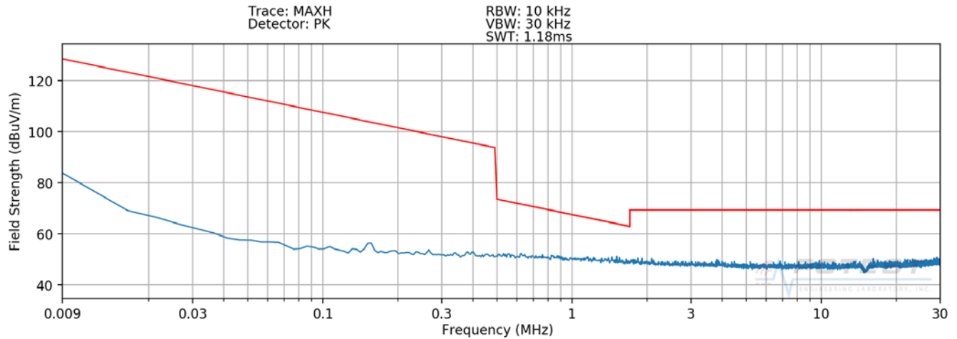
Plot 7-6. Radiated Spurious Plot 9kHz – 30MHz (Pol. Z – Device to Device WPT – CLOSED)
