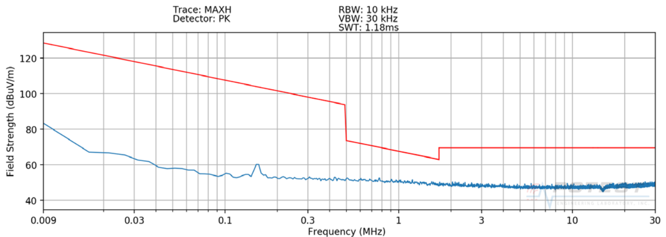
Plot 7-4. Radiated Spurious Plot 9kHz – 30MHz (Pol. X – Device to Device WPT – CLOSED)
