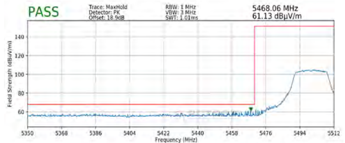
Plot 7-196. Radiated Lower Band Edge Plot SISO ANT1 (Peak - UNII Band 2C)
