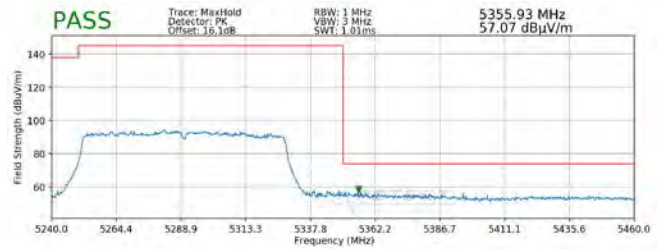
Plot 7-259. Radiated Band Edge Plot MIMO (Peak – WCP)
