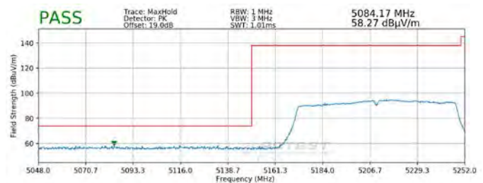
Plot 7-227. Radiated Lower Band Edge Plot SISO ANT2 (Peak - UNII Band 1)
