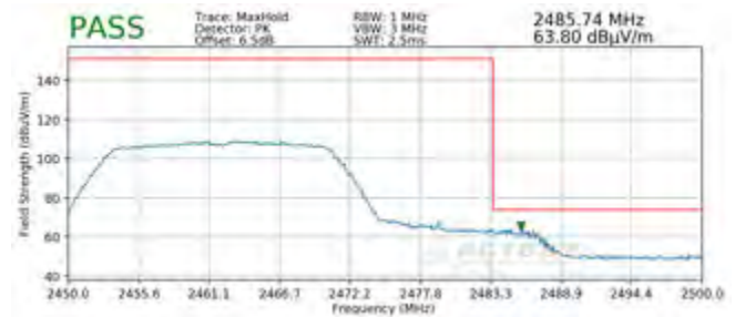
Plot 7-104. Radiated Restricted Upper Band Edge Measurement SISO ANT1 (Peak)
