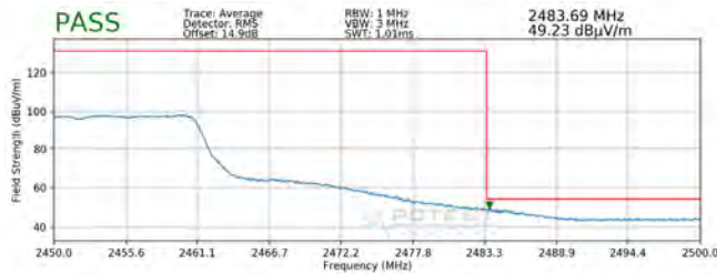
Plot 7-115. Radiated Restricted Upper Band Edge Measurement SISO ANT2 (Average)
