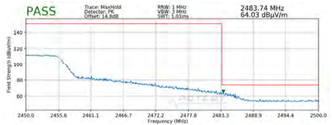
Plot 7-130. Radiated Restricted Upper Band Edge Measurement MIMO (Peak)
