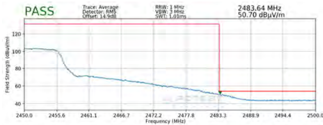
Plot 7-129. Radiated Restricted Upper Band Edge Measurement MIMO (Average)
