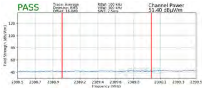
Plot 7-125. Radiated Restricted Lower Band Edge Measurement MIMO (Average)
