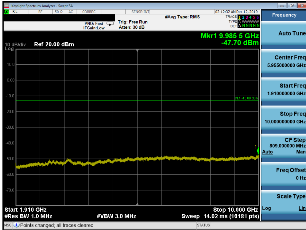
Plot 7-13. Conducted Spurious Plot (PCS WCDMA Mode - Mid Channel)
