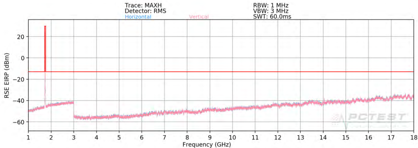
Plot 7-107. Radiated Spurious Plot above 1GHz (AWS WCDMA Mode) – OPEN
