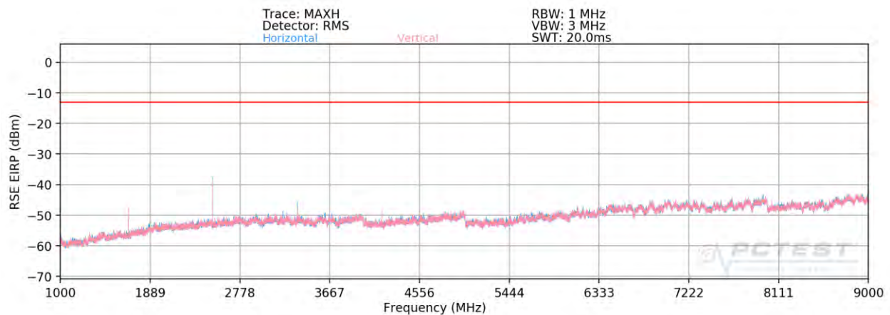
Plot 7-103. Radiated Spurious Plot above 1GHz (Cellular GPRS Mode) – CLOSED
