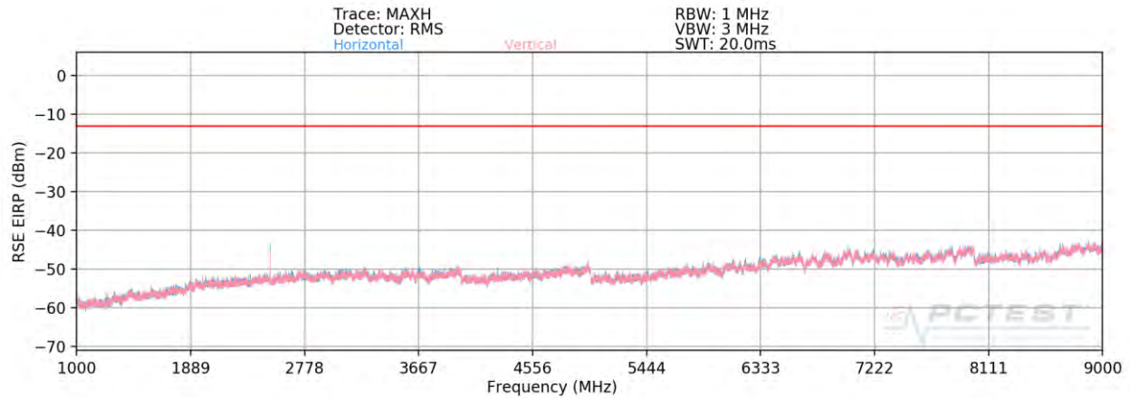
Plot 7-102. Radiated Spurious Plot above 1GHz (Cellular GPRS Mode) – OPEN
