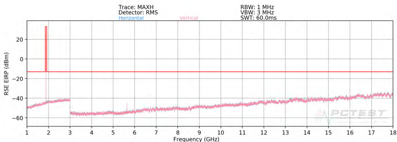
Plot 7-110. Radiated Spurious Plot above 1GHz (PCS GPRS Mode) – CLOSED
