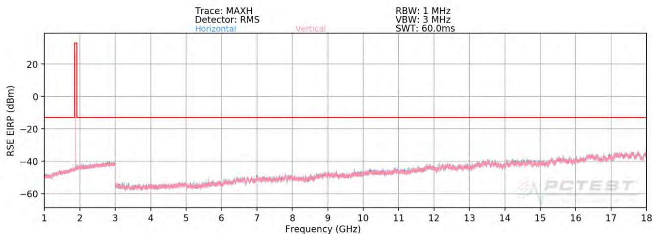
Plot 7-109. Radiated Spurious Plot above 1GHz (PCS GPRS Mode) – OPEN
