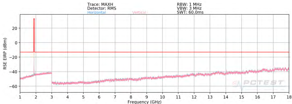
Plot 7-112. Radiated Spurious Plot above 1GHz (PCS CDMA Mode) – CLOSED
