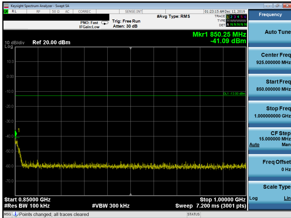
Plot 7-5. Conducted Spurious Plot (Cellular GPRS Mode - High Channel)
