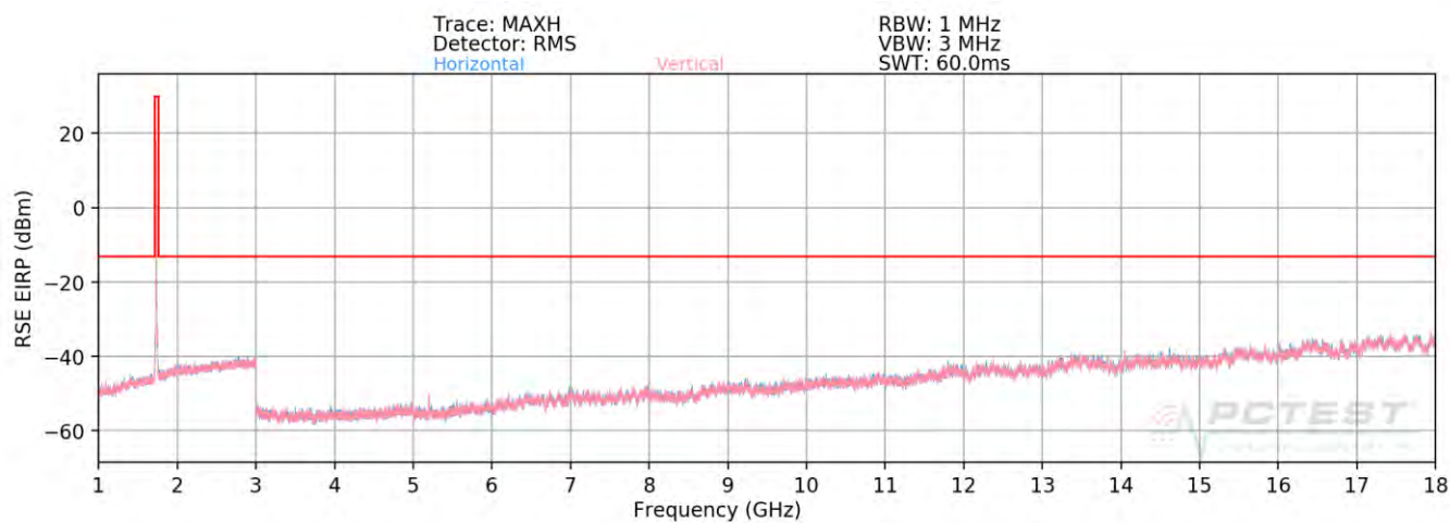
Plot 7-108. Radiated Spurious Plot above 1GHz (AWS WCDMA Mode) – CLOSED
