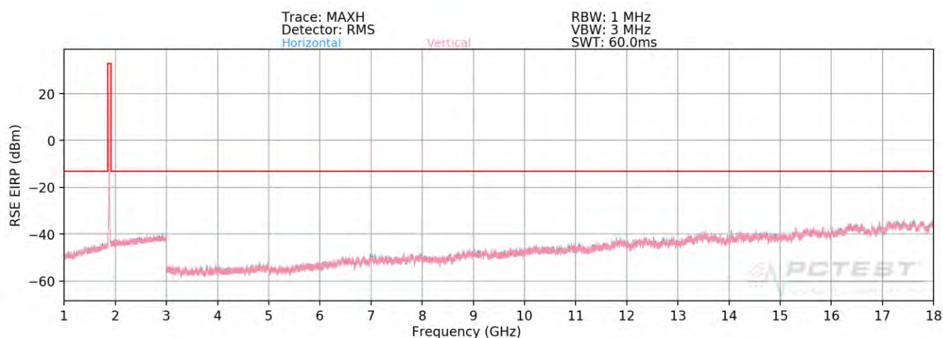
Plot 7-114. Radiated Spurious Plot above 1GHz (PCS WCDMA Mode) – CLOSED
