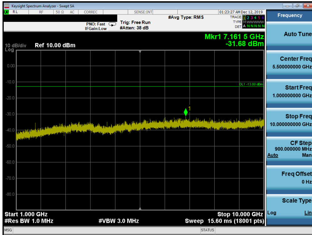
Plot 7-6. Conducted Spurious Plot (Cellular GPRS Mode - High Channel)
