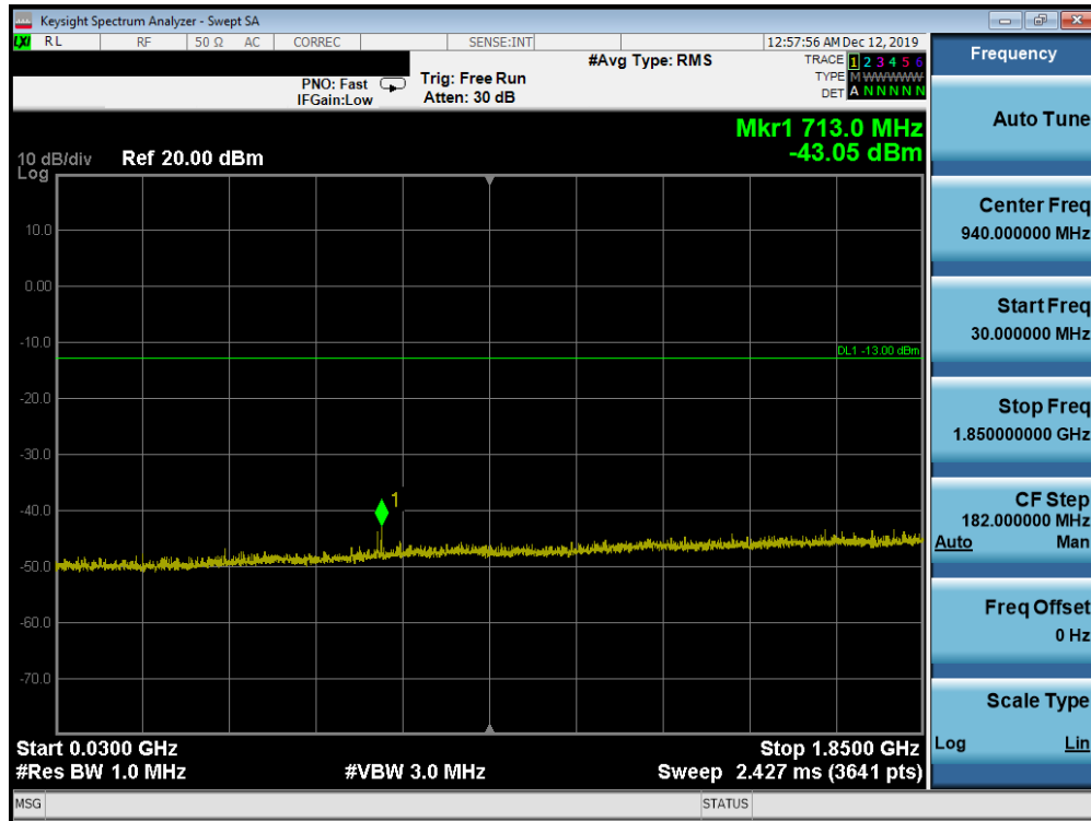
Plot 7-10. Conducted Spurious Plot (PCS GPRS Mode - High Channel)
