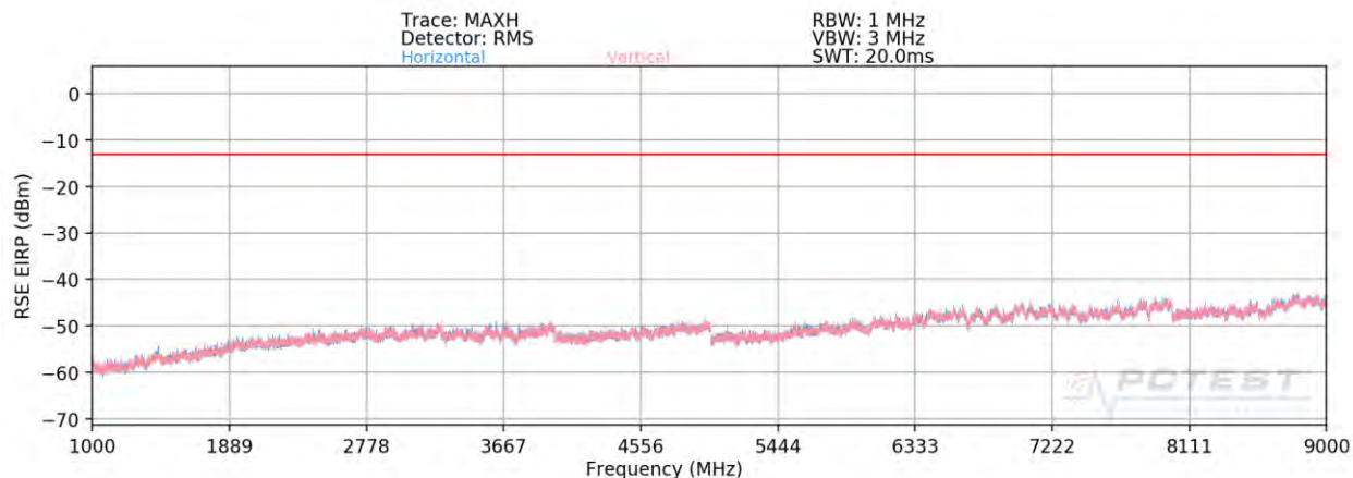
Plot 7-106. Radiated Spurious Plot above 1GHz (Cellular WCDMA Mode) – OPEN
