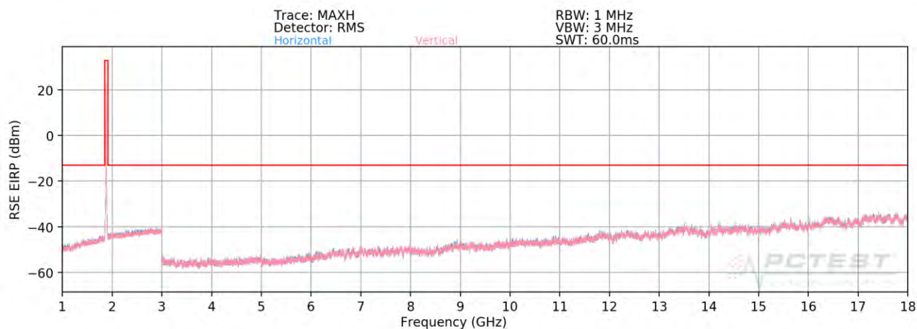
Plot 7-113. Radiated Spurious Plot above 1GHz (PCS WCDMA Mode) – OPEN
