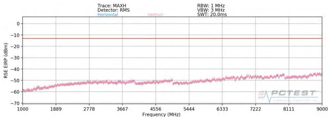
Plot 7-104. Radiated Spurious Plot above 1GHz (Cellular CDMA Mode) – OPEN
