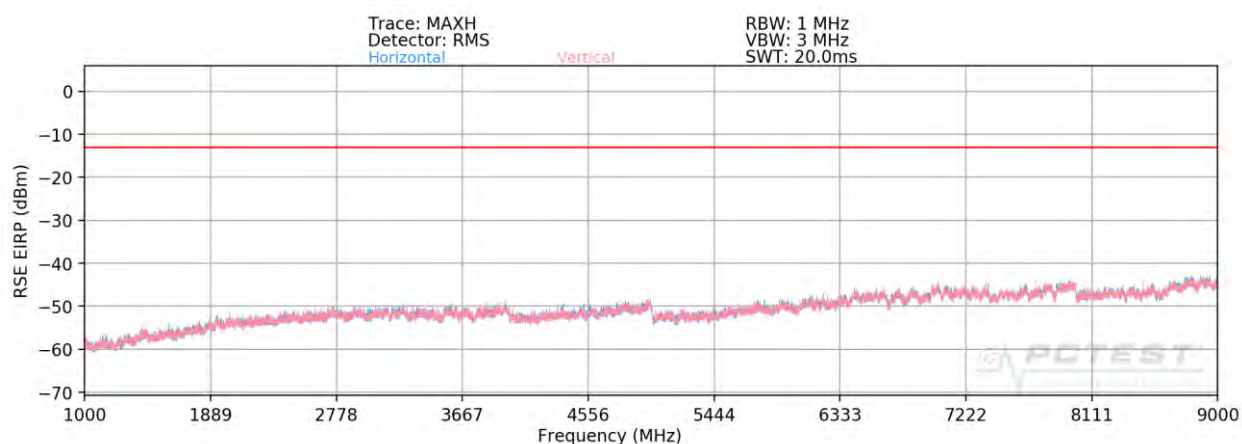
Plot 7-105. Radiated Spurious Plot above 1GHz (Cellular CDMA Mode) – CLOSED
