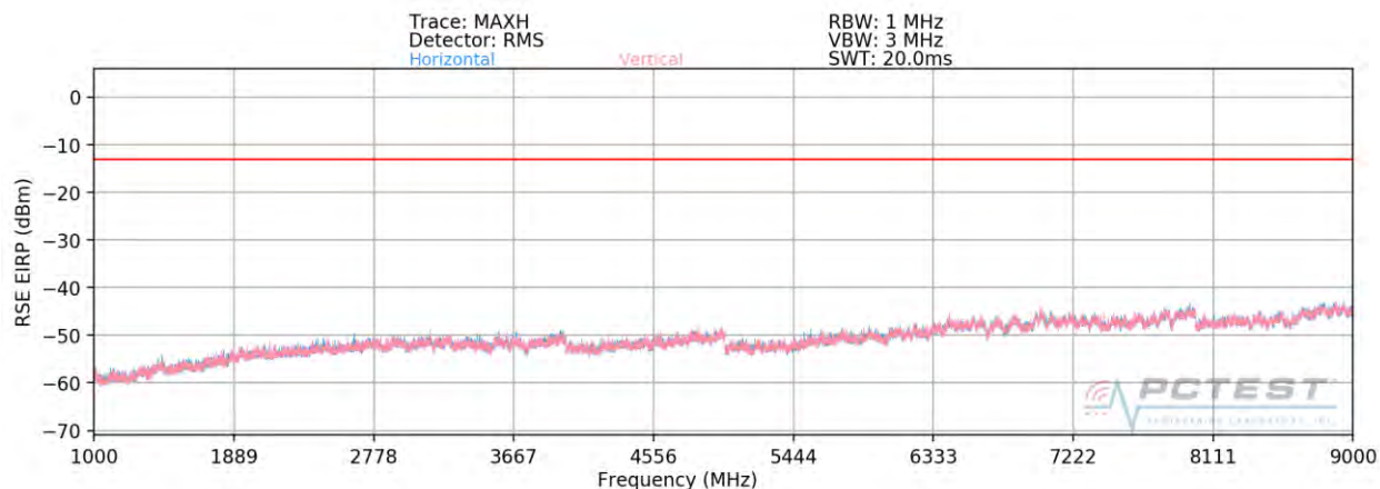
Plot 7-107. Radiated Spurious Plot above 1GHz (Cellular WCDMA Mode) – CLOSED
