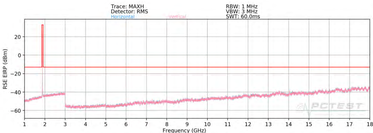
Plot 7-111. Radiated Spurious Plot above 1GHz (PCS CDMA Mode) – OPEN
