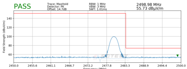
Plot 7-5. Radiated Restricted Upper Band Edge Measurement (Peak)
