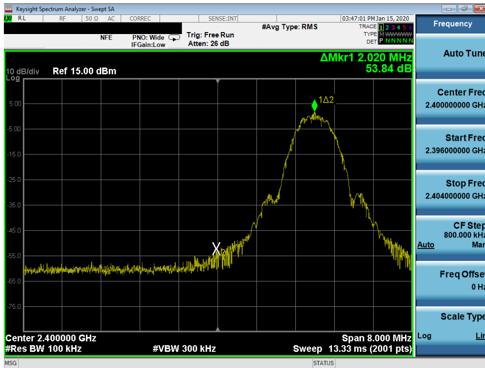
Plot 7-39. Band Edge Plot (Bluetooth (LE), 500kbps – Ch. 0)
