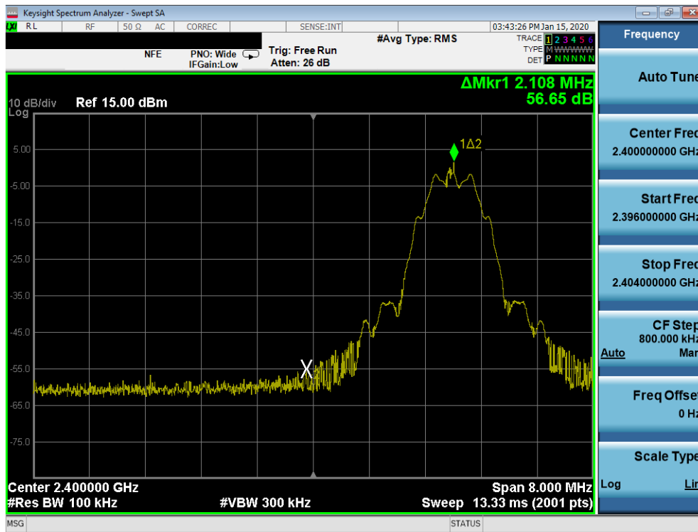
Plot 7-37. Band Edge Plot (Bluetooth (LE), 125kbps – Ch. 0)
