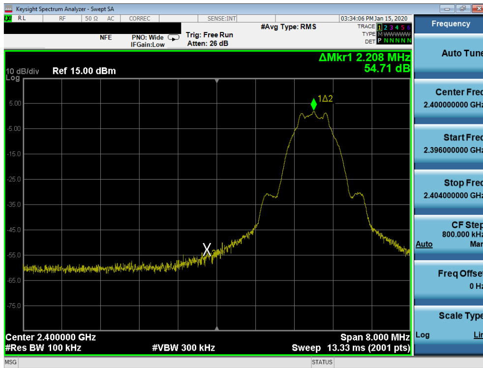
Plot 7-41. Band Edge Plot (Bluetooth (LE), 1Mbps – Ch. 0)
