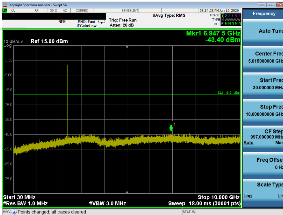
Plot 7-45. Conducted Spurious Plot (Bluetooth (LE), 1Mbps – Ch. 0)
