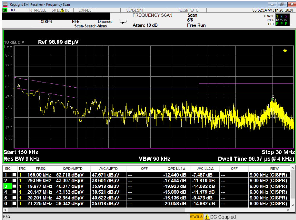
Plot 7-60. Line-Conducted Test Plot (L1) – OPEN with WCP
