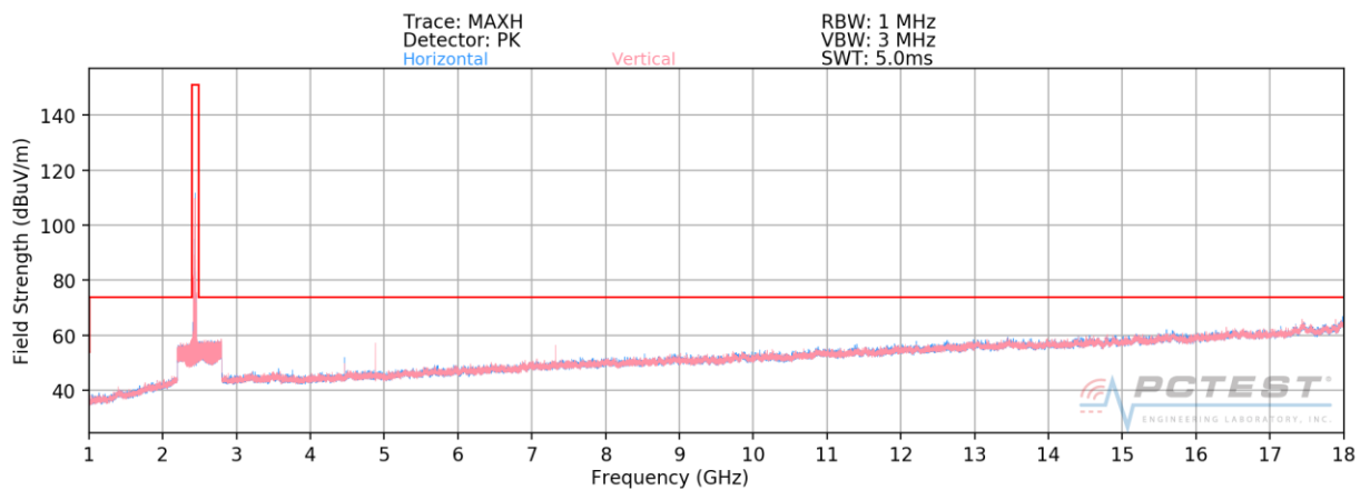
Plot 7-46. Radiated Spurious Plot above 1GHz (BT- Ch. 39) – CLOSED
