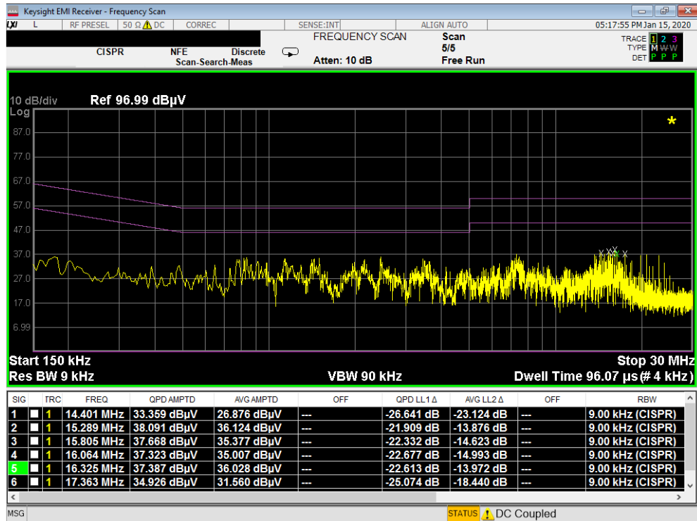
Plot 7-62. Line-Conducted Test Plot (L1) – CLOSED with WCP
