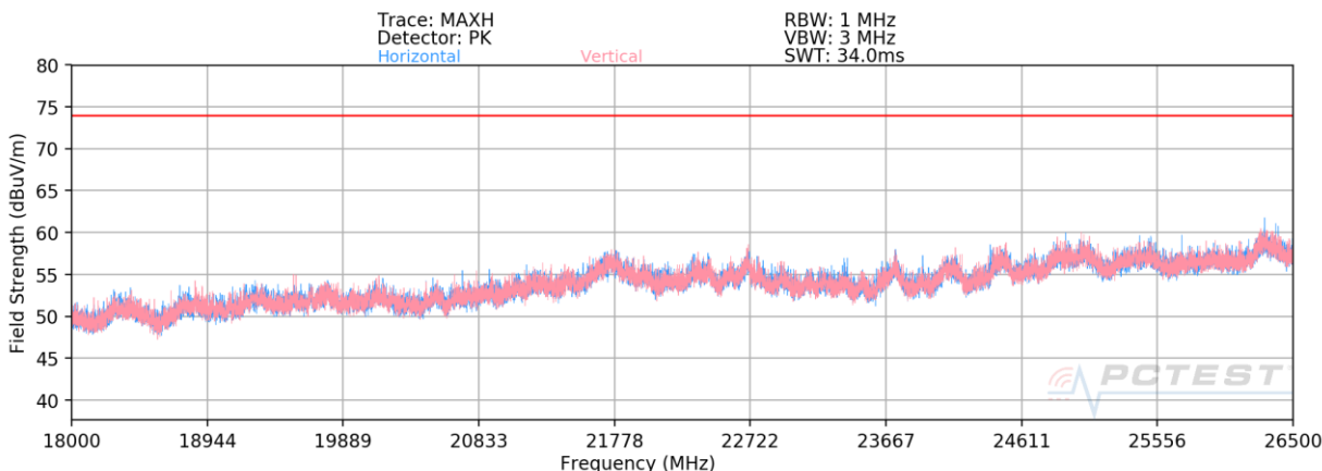
Plot 7-47. Radiated Spurious Plot above 18GHz – OPEN
