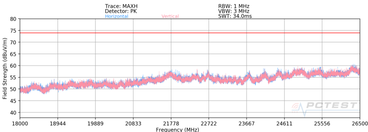
Plot 7-48. Radiated Spurious Plot above 18GHz – CLOSED
