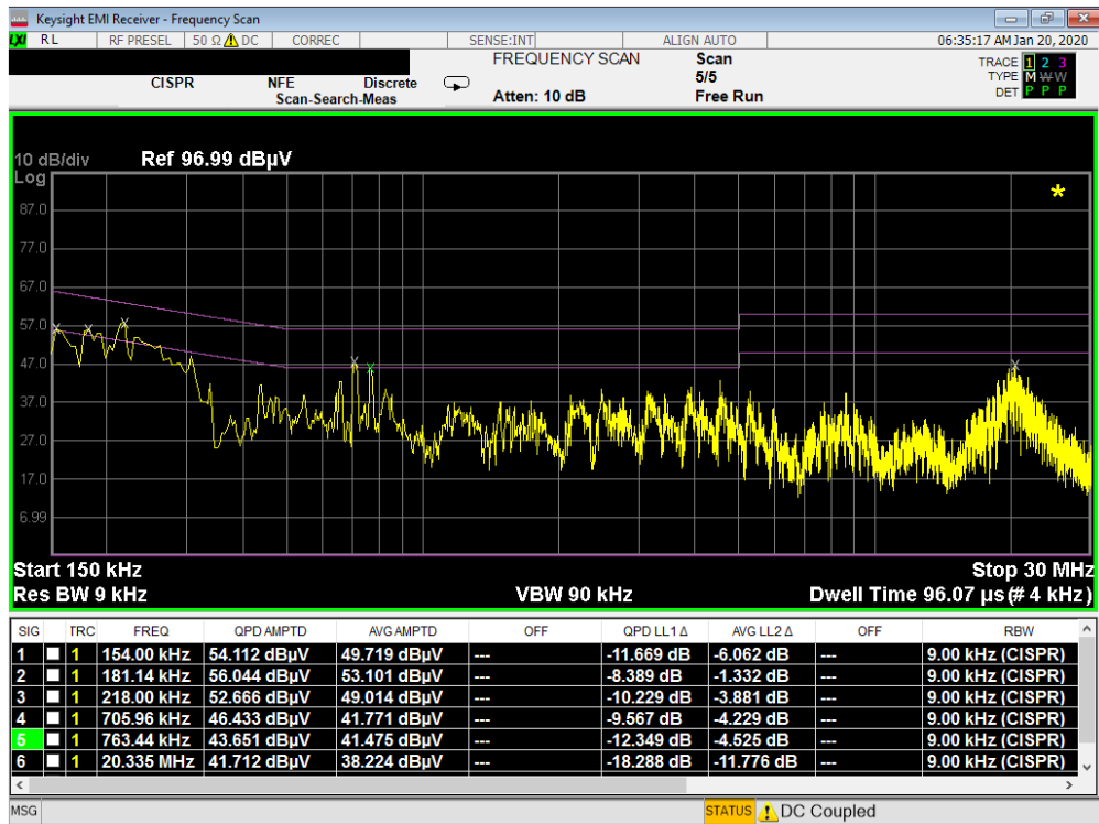
Plot 7-56. Line-Conducted Test Plot (L1) – OPEN
