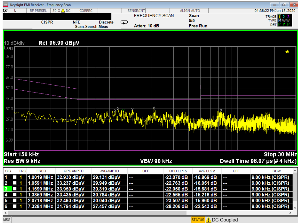
Plot 7-58. Line-Conducted Test Plot (L1) – CLOSED
