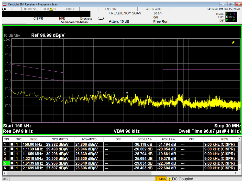
Plot 7-59. Line-Conducted Test Plot (N) – CLOSED
