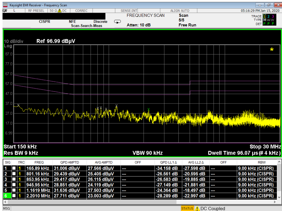
Plot 7-63. Line-Conducted Test Plot (N) – CLOSED with WCP
