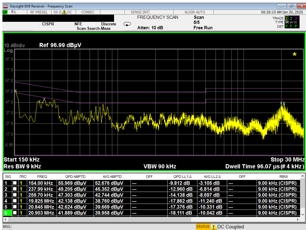
Plot 7-57. Line-Conducted Test Plot (N) – OPEN
