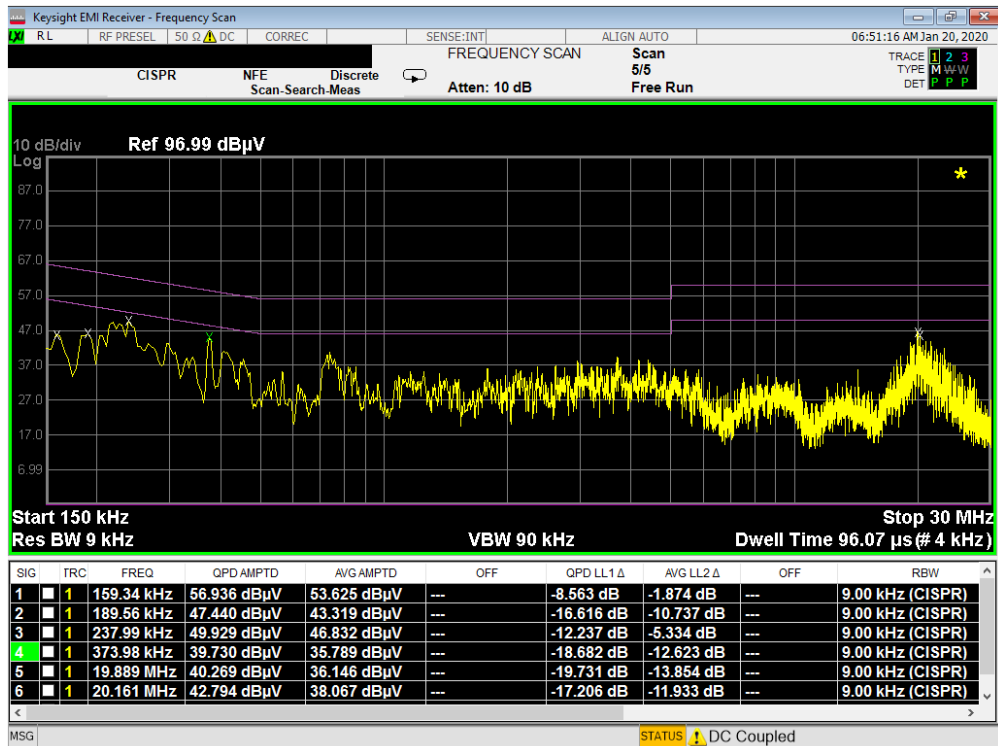
Plot 7-61. Line-Conducted Test Plot (N) – OPEN with WCP
