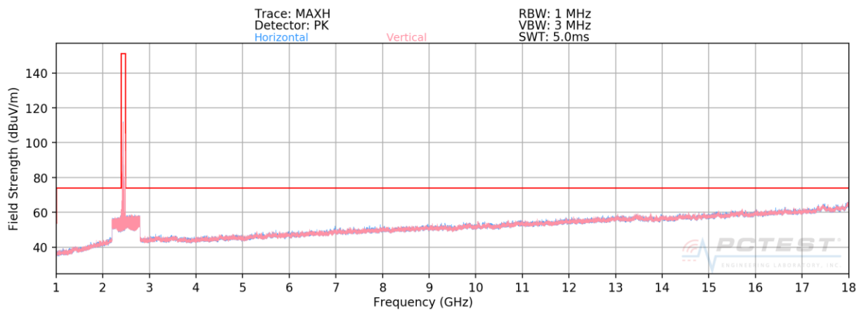
Plot 7-46. Radiated Spurious Plot above 1GHz (BT- Ch. 78) – CLOSED
