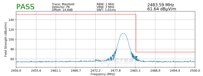
Plot 7-50. Radiated Restricted Upper Band Edge Measurement with WCP (Peak)
