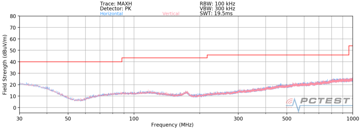
Plot 7-54. Radiated Spurious Plot below 1GHz – OPEN
