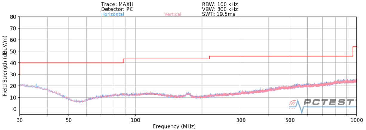
Plot 7-55. Radiated Spurious Plot below 1GHz – CLOSED
