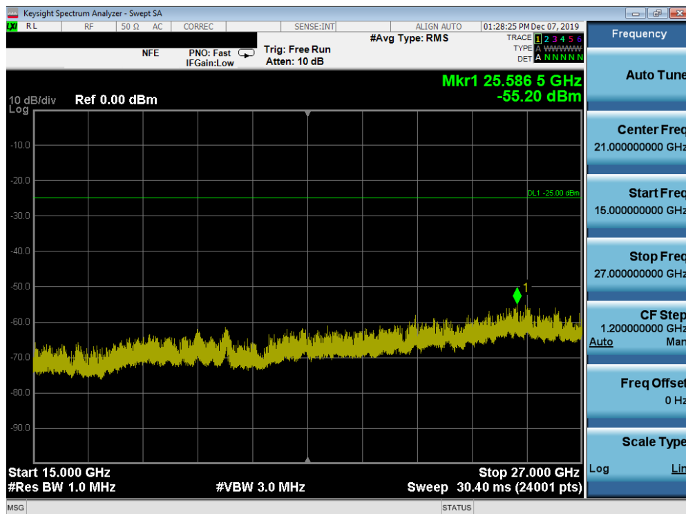
Plot 7-159. Conducted Spurious Plot (Band 7 - 20.0MHz QPSK - RB Size 1, RB Offset 0 - Low Channel)
