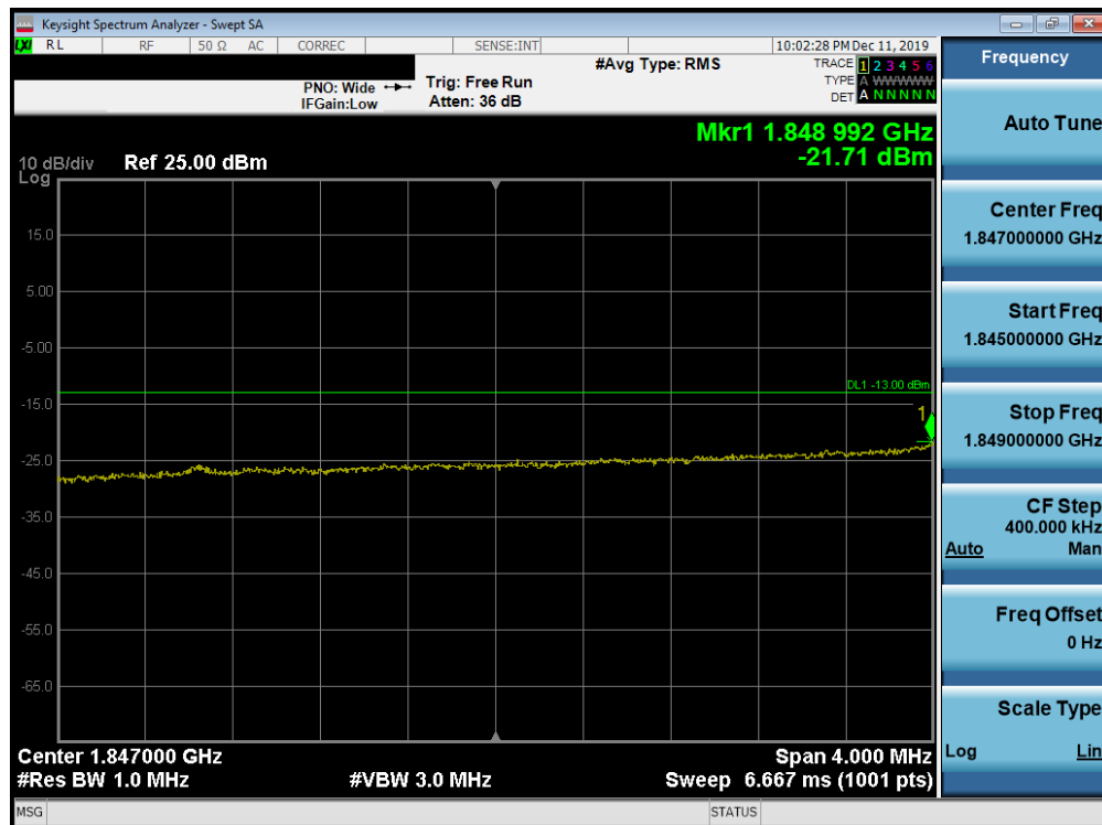
Plot 7-206. Lower Extended Band Edge Plot (Band 25/2 - 10.0MHz QPSK - Full RB Configuration)
