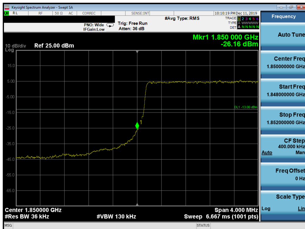
Plot 7-193. Lower Band Edge Plot (Band 25/2 - 3.0MHz QPSK - Full RB Configuration)
