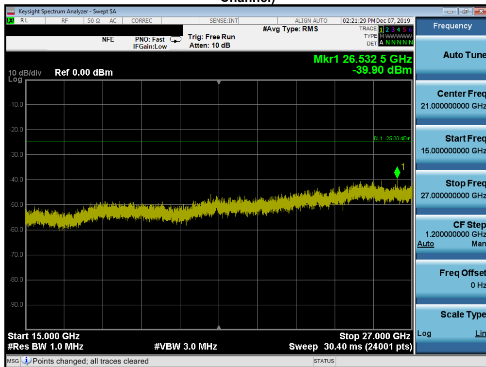
Plot 7-170. Conducted Spurious Plot (Band 41 PC3 - 20.0MHz QPSK - RB Size 1, RB Offset 0 - Mid Channel)
