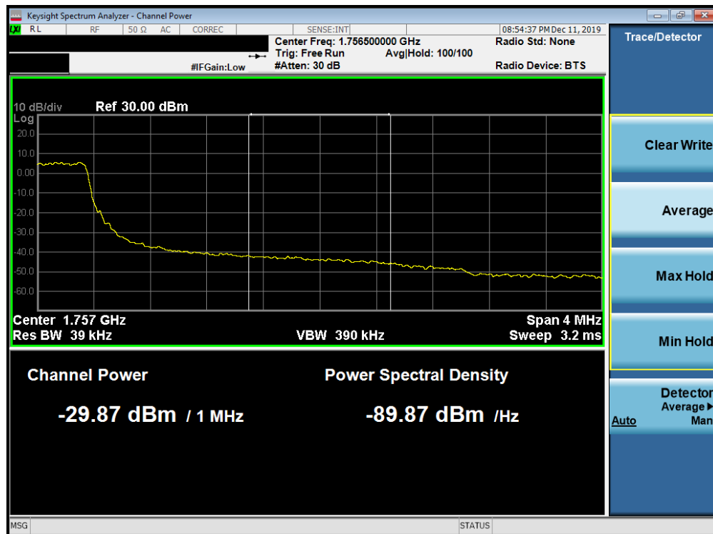
Plot 7-241. Upper Extended Band Edge Plot (Band 4 - 3.0MHz QPSK - Full RB Configuration)
