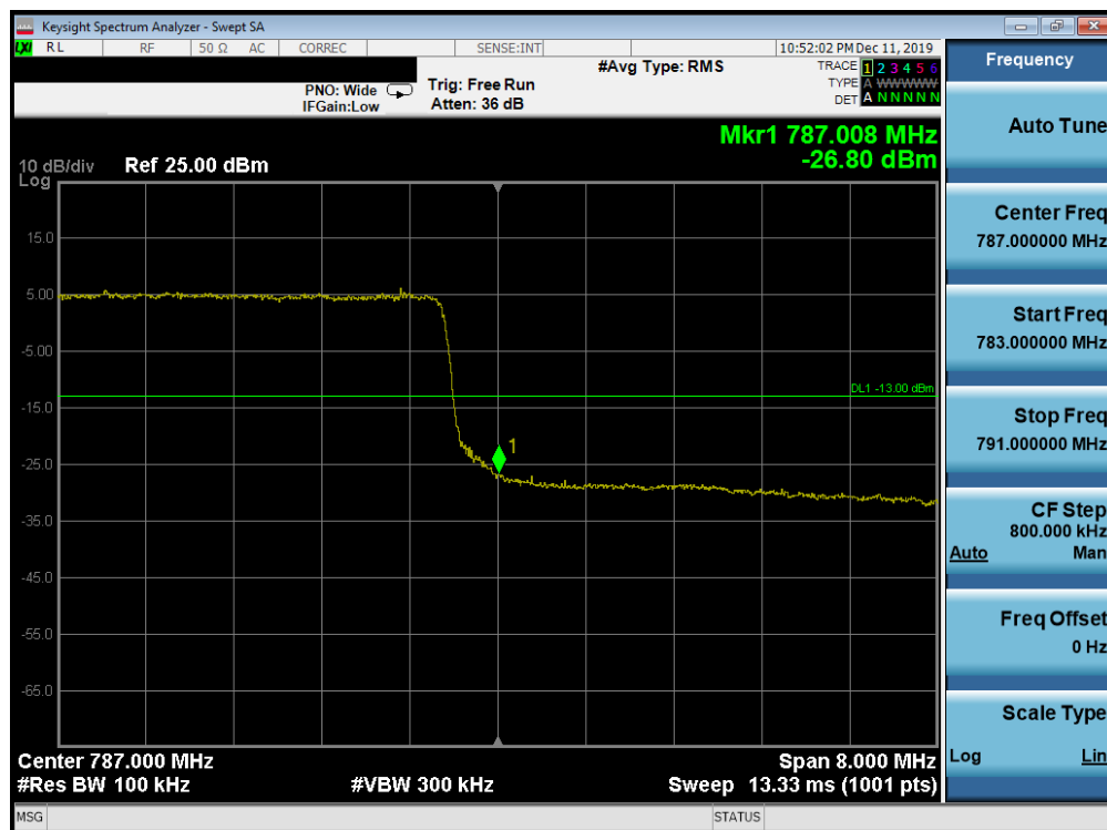
Plot 7-221. Upper Band Edge Plot (Band 13 - 10.0MHz QPSK - Full RB Configuration)
