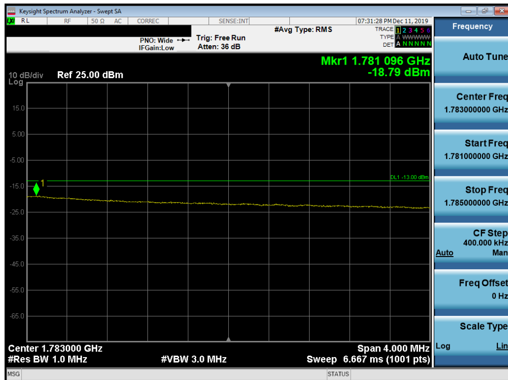
Plot 7-186. Upper Extended Band Edge Plot (Band 66 - 20.0MHz QPSK - Full RB Configuration)
