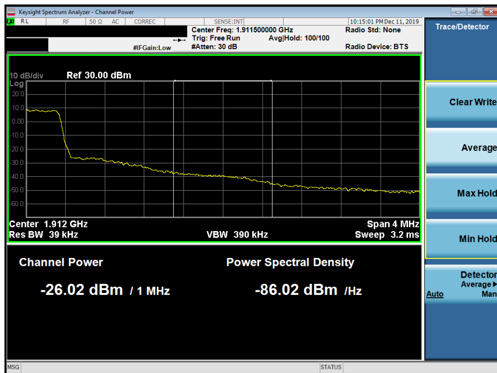
Plot 7-190. Upper Extended Band Edge Plot (Band 2 - 1.4MHz QPSK - Full RB Configuration)
