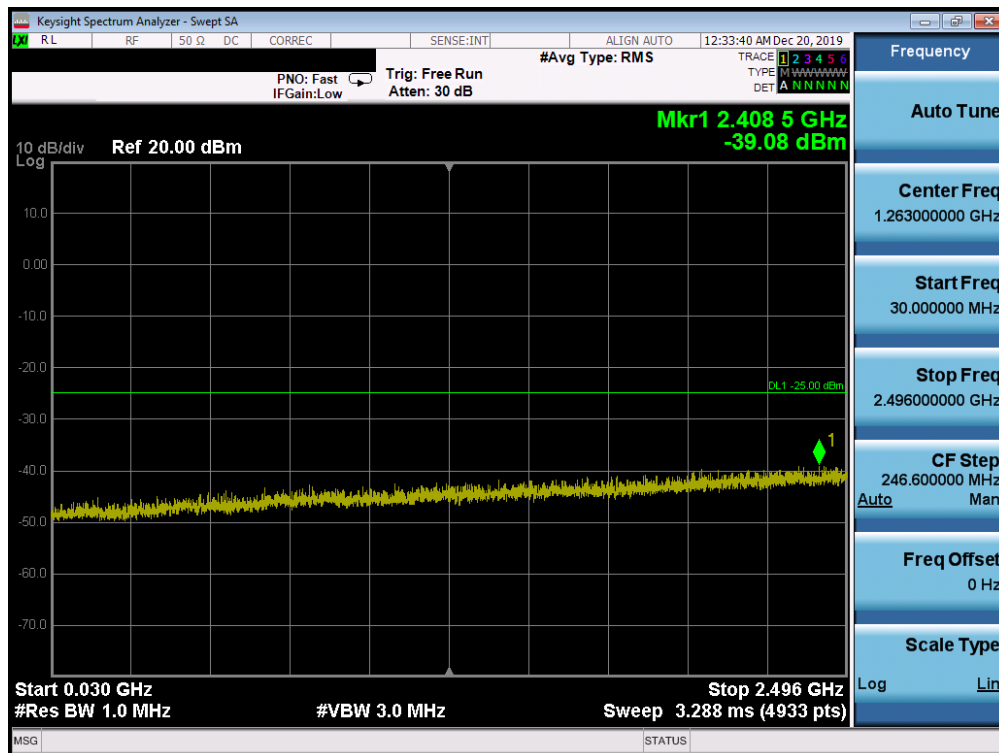
Plot 7-190. Conducted Spurious Plot (Band 41 PC2 - 20.0MHz QPSK - RB Size 1, RB Offset 99 - High Channel)
