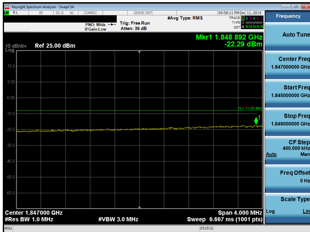
Plot 7-212. Lower Extended Band Edge Plot (Band 25/2 - 15.0MHz QPSK - Full RB Configuration)
