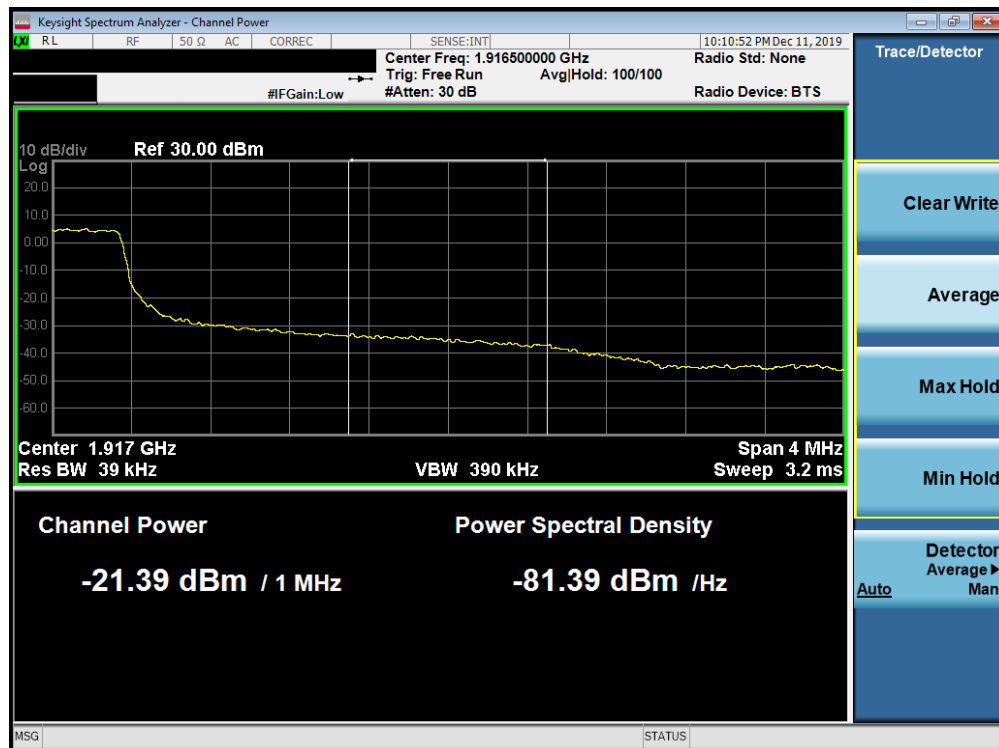
Plot 7-198. Upper Extended Band Edge Plot (Band 25 - 3.0MHz QPSK - Full RB Configuration)
