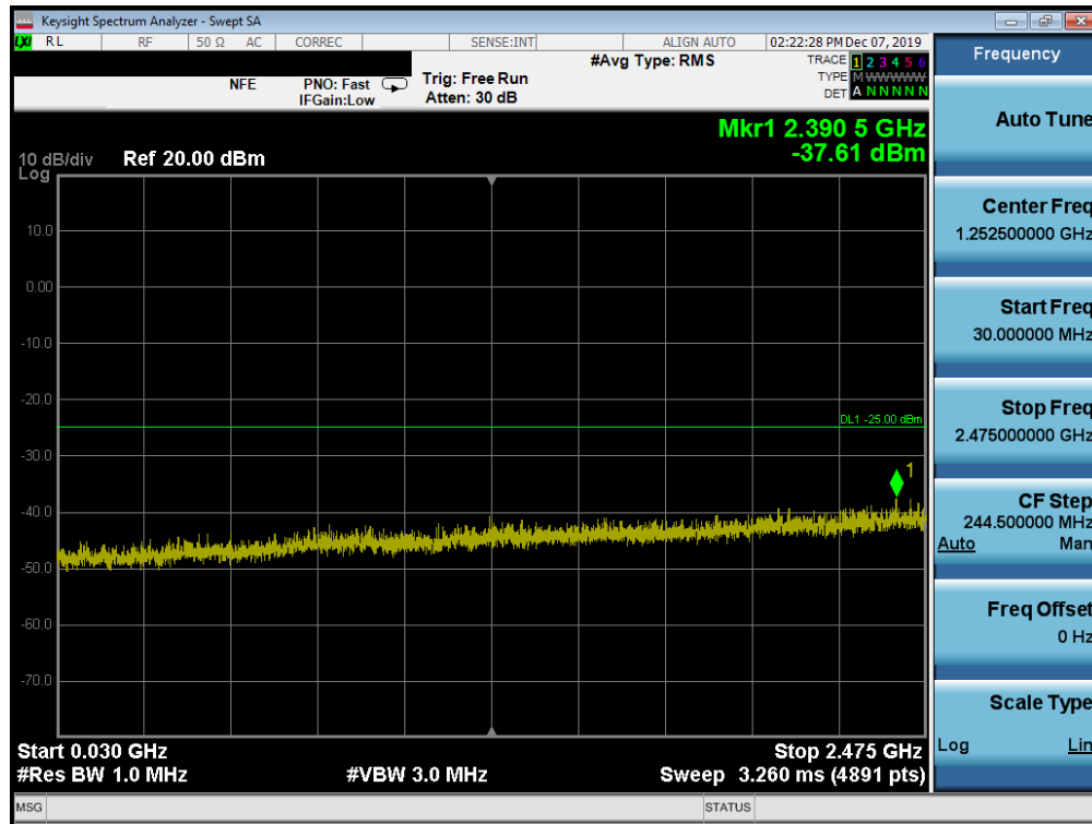
Plot 7-193. Conducted Spurious Plot (Band 41 PC3 - 20.0MHz QPSK - RB Size 1, RB Offset 0 - Low Channel)
