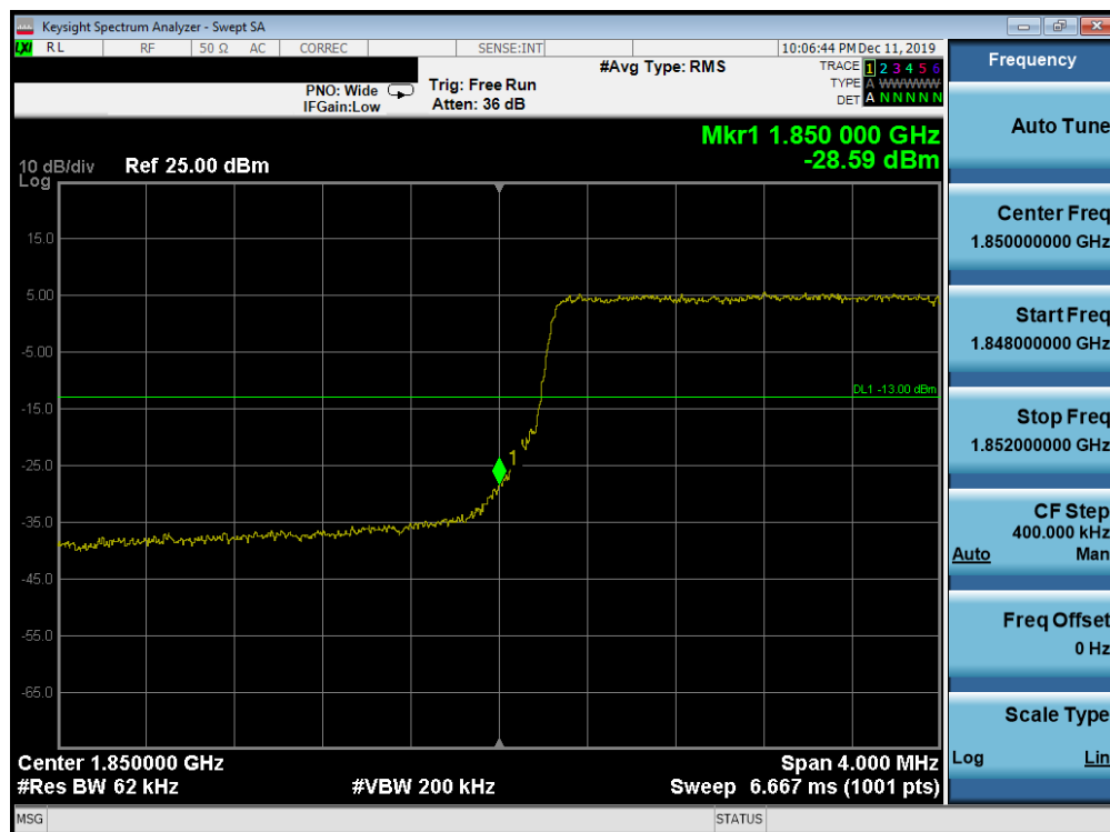
Plot 7-199. Lower Band Edge Plot (Band 25/2 - 5.0MHz QPSK - Full RB Configuration)
