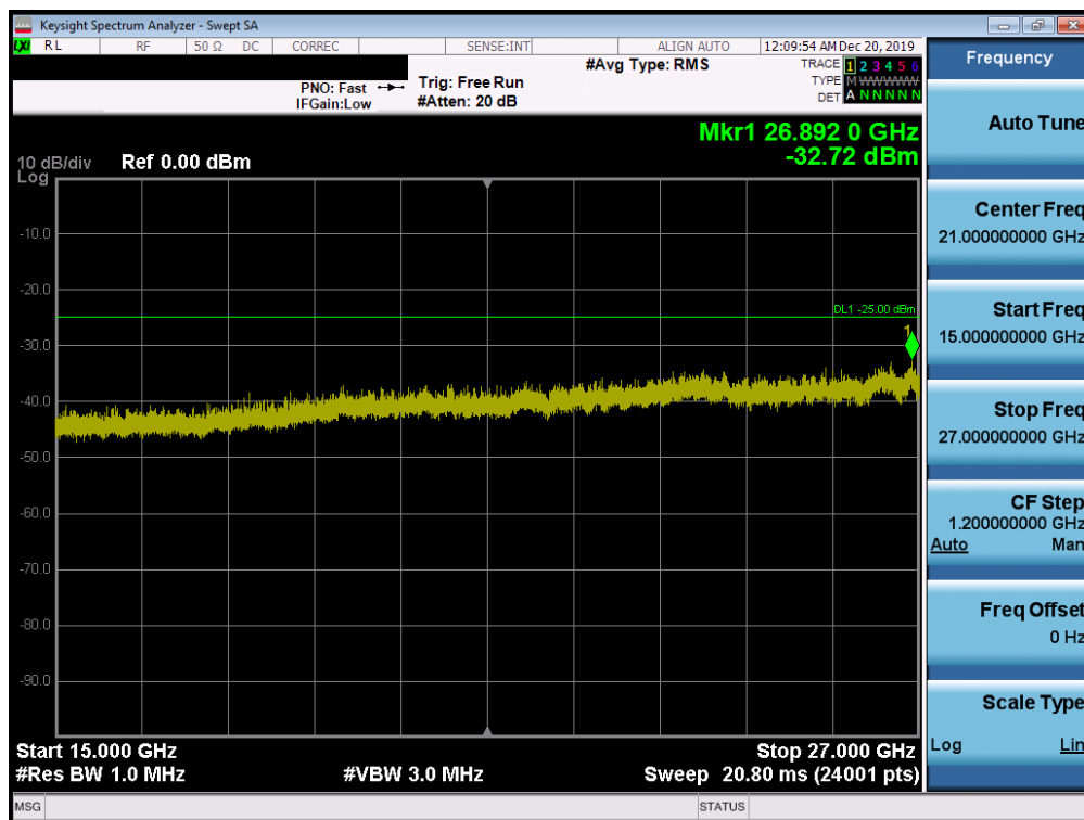
Plot 7-189. Conducted Spurious Plot (Band 41 PC2 - 20.0MHz QPSK - RB Size 1, RB Offset 0 - Mid Channel)
