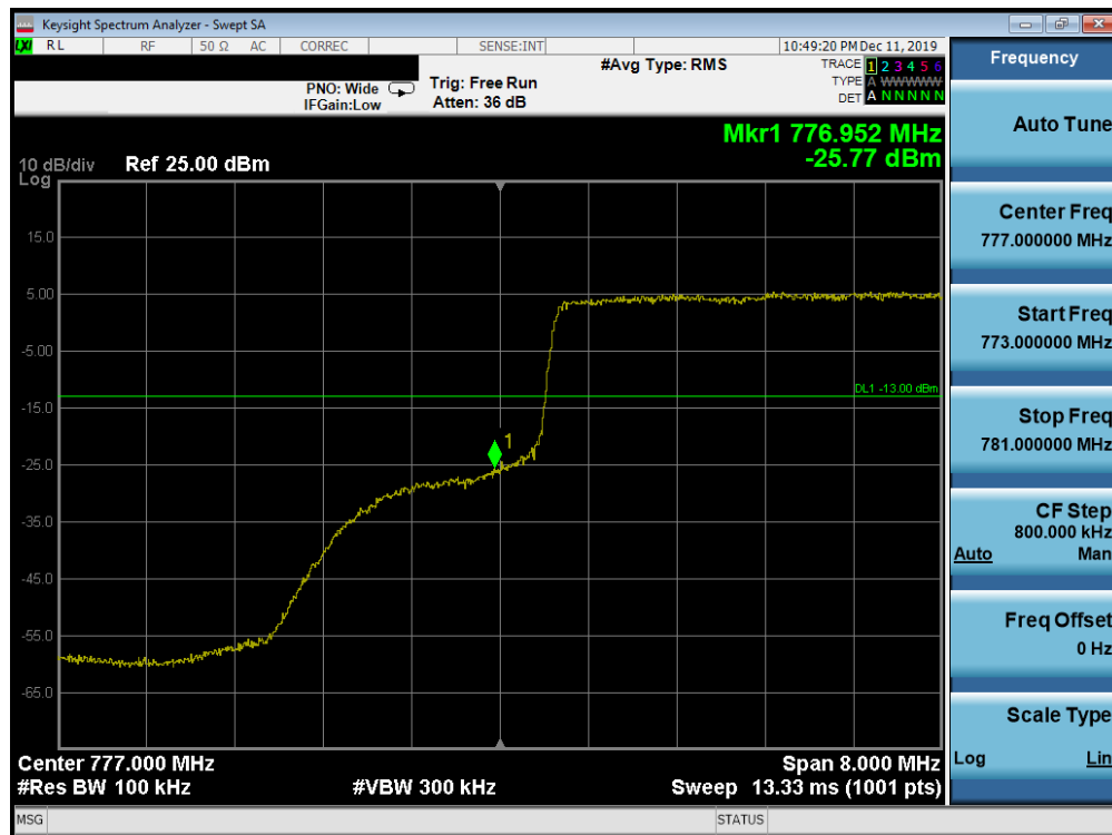
Plot 7-220. Lower Band Edge Plot (Band 13 - 10.0MHz QPSK - Full RB Configuration)
