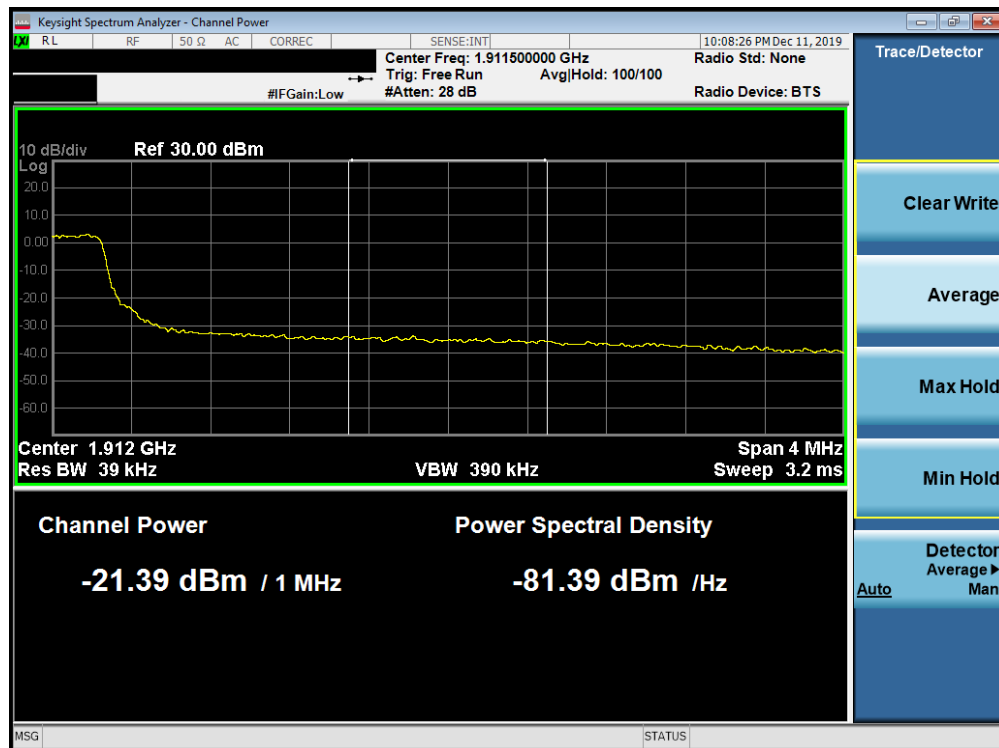
Plot 7-2023. Upper Extended Band Edge Plot (Band 2 - 5.0MHz QPSK - Full RB Configuration)
