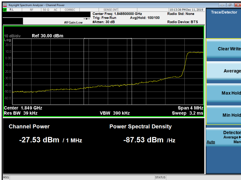
Plot 7-188. Lower Extended Band Edge Plot (Band 25/2 - 1.4MHz QPSK - Full RB Configuration)
