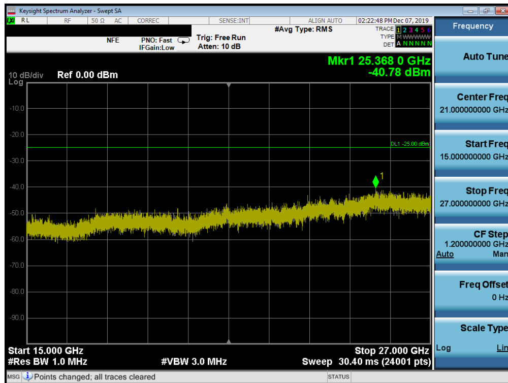
Plot 7-167. Conducted Spurious Plot (Band 41 PC3 - 20.0MHz QPSK - RB Size 1, RB Offset 0 - Low Channel)
