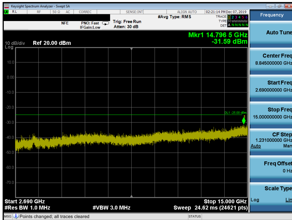
Plot 7-169. Conducted Spurious Plot (Band 41 PC3 - 20.0MHz QPSK - RB Size 1, RB Offset 0 - Mid Channel)
