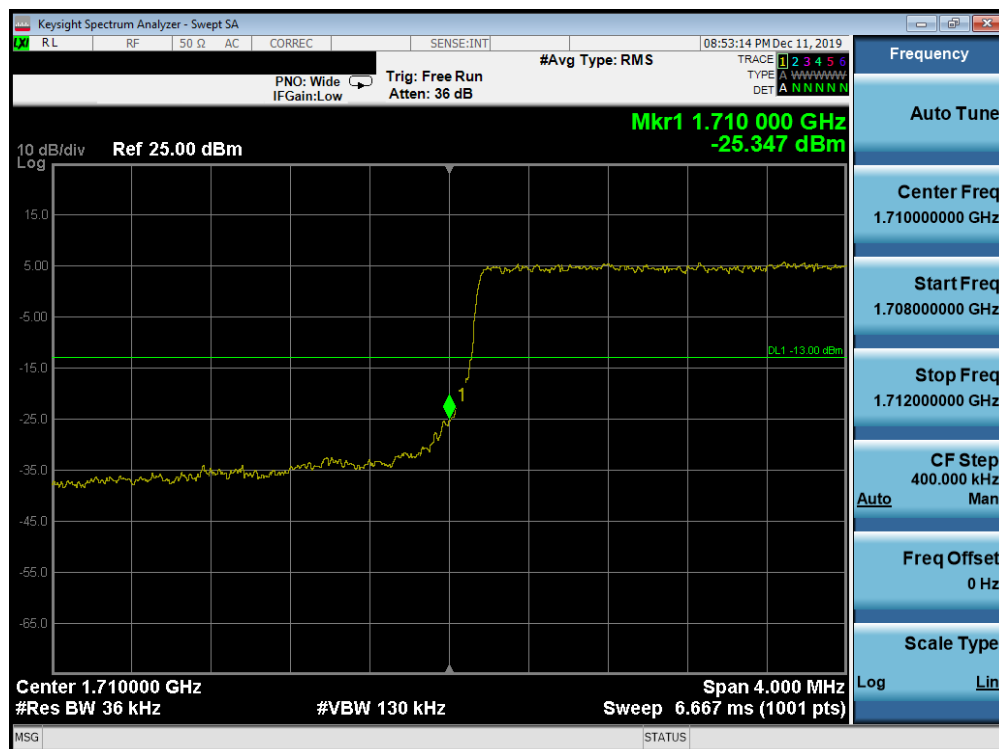
Plot 7-238. Lower Band Edge Plot (Band 66/4 - 3.0MHz QPSK - Full RB Configuration)
