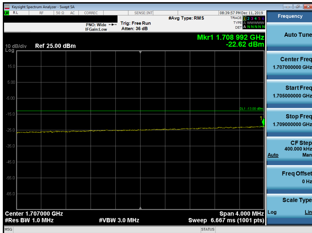
Plot 7-176. Lower Extended Band Edge Plot (Band 66/4 - 15.0MHz QPSK - Full RB Configuration)
