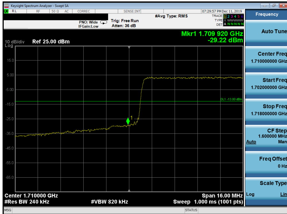
Plot 7-181. Lower Band Edge Plot (Band 66/4 - 20.0MHz QPSK - Full RB Configuration)
