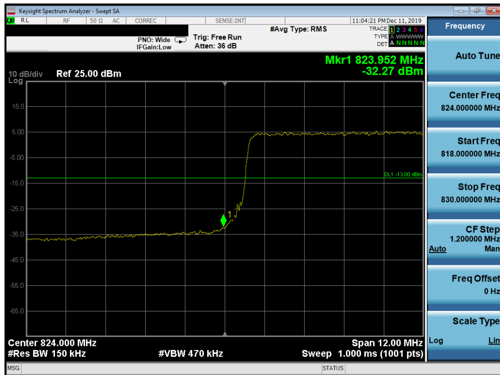
Plot 7-230. Lower Band Edge Plot (Band 26 - 15.0MHz QPSK - Full RB Configuration)
