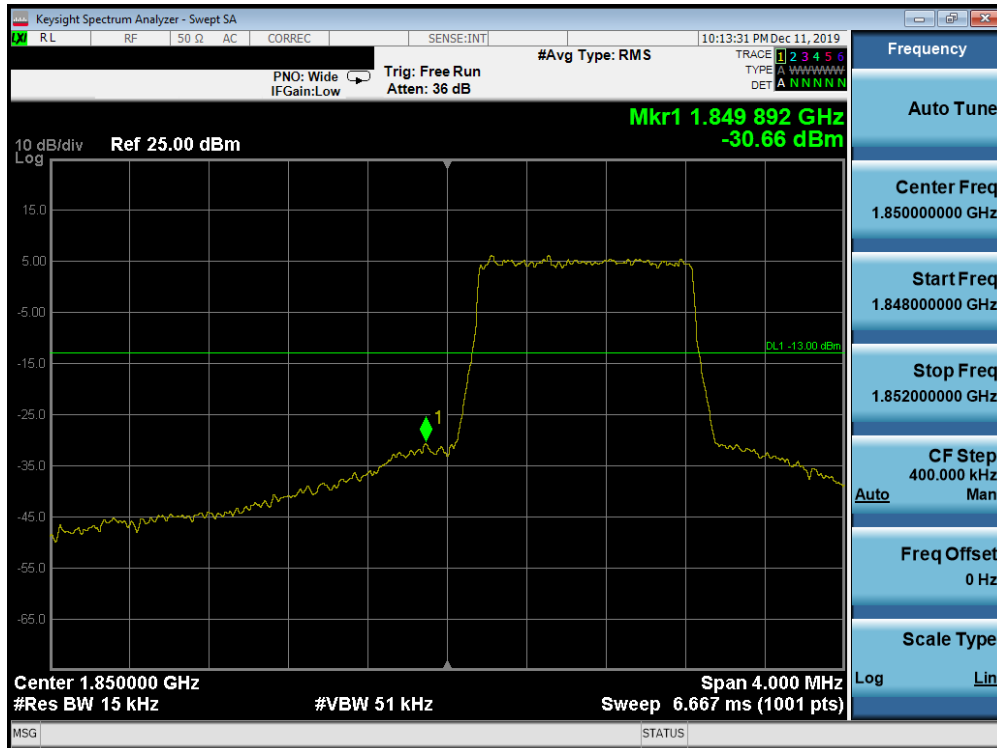
Plot 7-187. Lower Band Edge Plot (Band 25/2 - 1.4MHz QPSK - Full RB Configuration)
