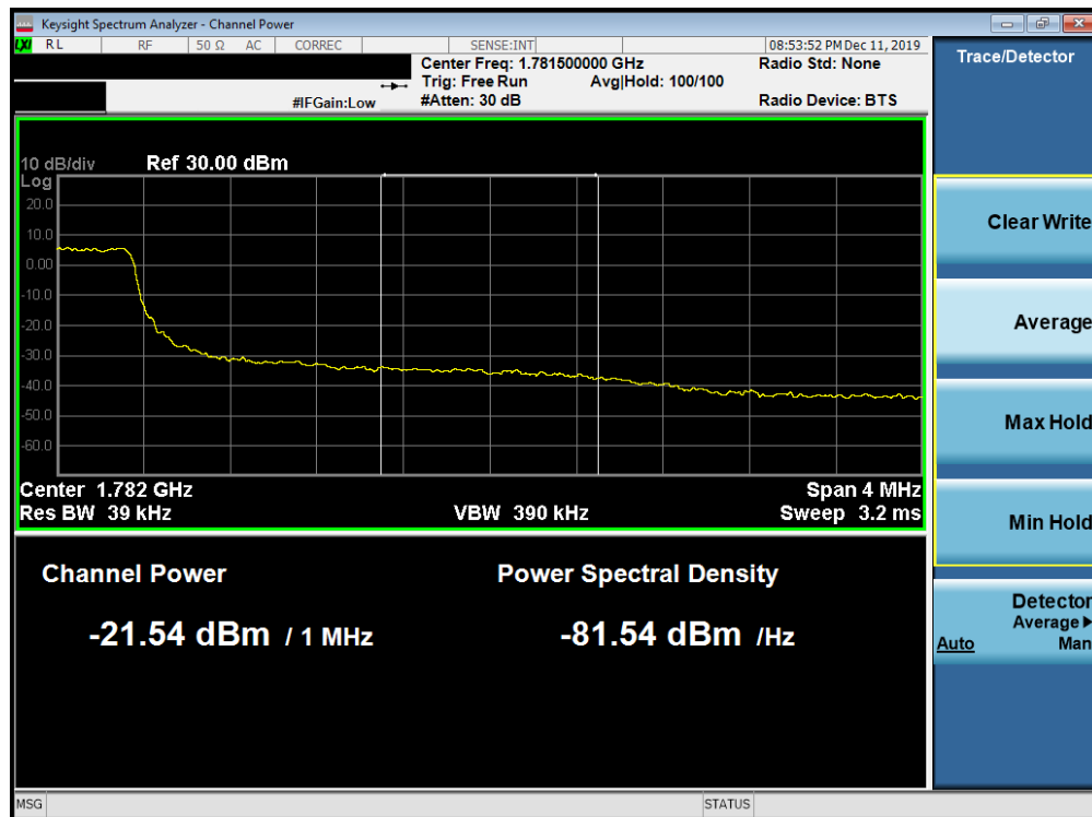
Plot 7-243. Upper Extended Band Edge Plot (Band 66 - 3.0MHz QPSK - Full RB Configuration)
