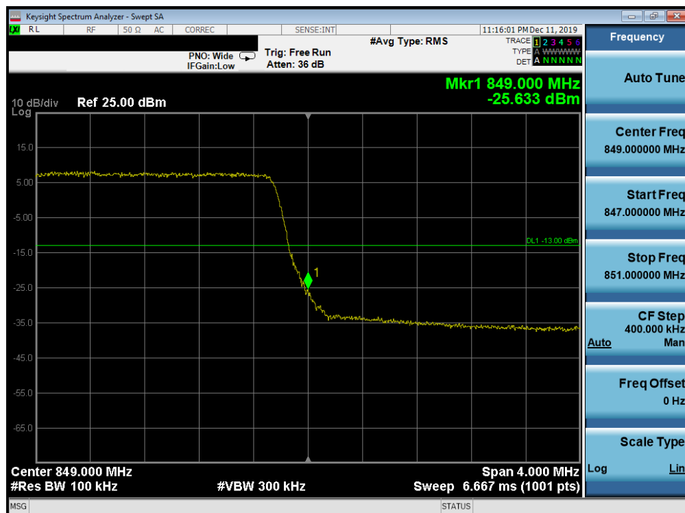
Plot 7-227. Upper Band Edge Plot (Band 26/5 - 5.0MHz QPSK - Full RB Configuration)
