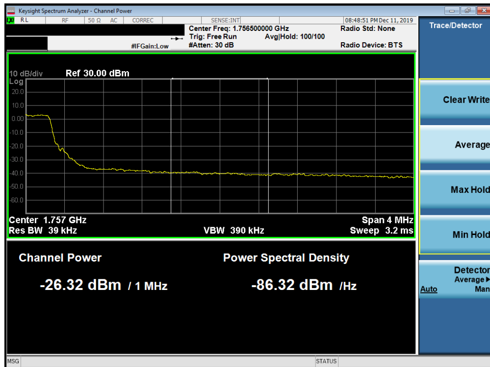
Plot 7-247. Upper Extended Band Edge Plot (Band 4 - 5.0MHz QPSK - Full RB Configuration)
