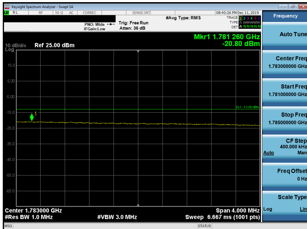
Plot 7-180. Upper Extended Band Edge Plot (Band 66 - 15.0MHz QPSK - Full RB Configuration)
