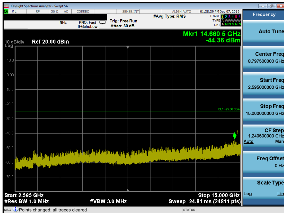
Plot 7-164. Conducted Spurious Plot (Band 7 - 20.0MHz QPSK - RB Size 1, RB Offset 0 - High Channel)
