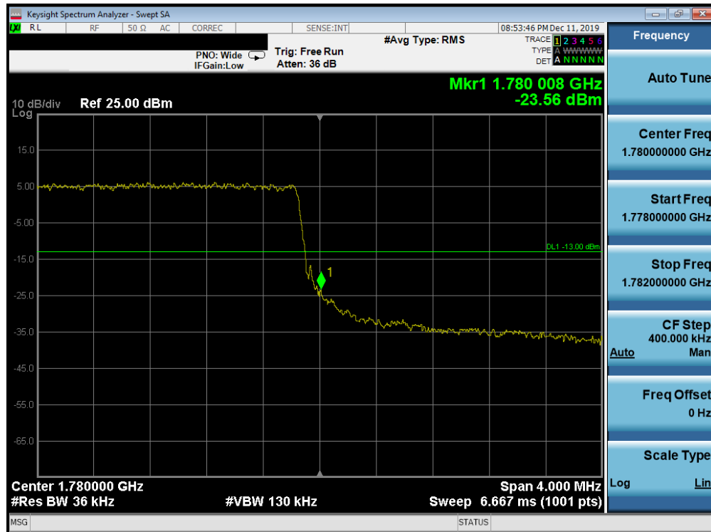
Plot 7-242. Upper Band Edge Plot (Band 66 - 3.0MHz QPSK - Full RB Configuration)
