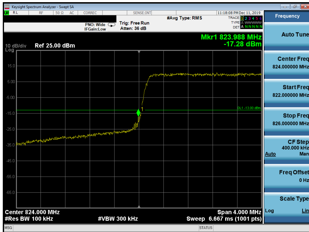
Plot 7-224. Lower Band Edge Plot (Band 26/5 - 3.0MHz QPSK - Full RB Configuration)
