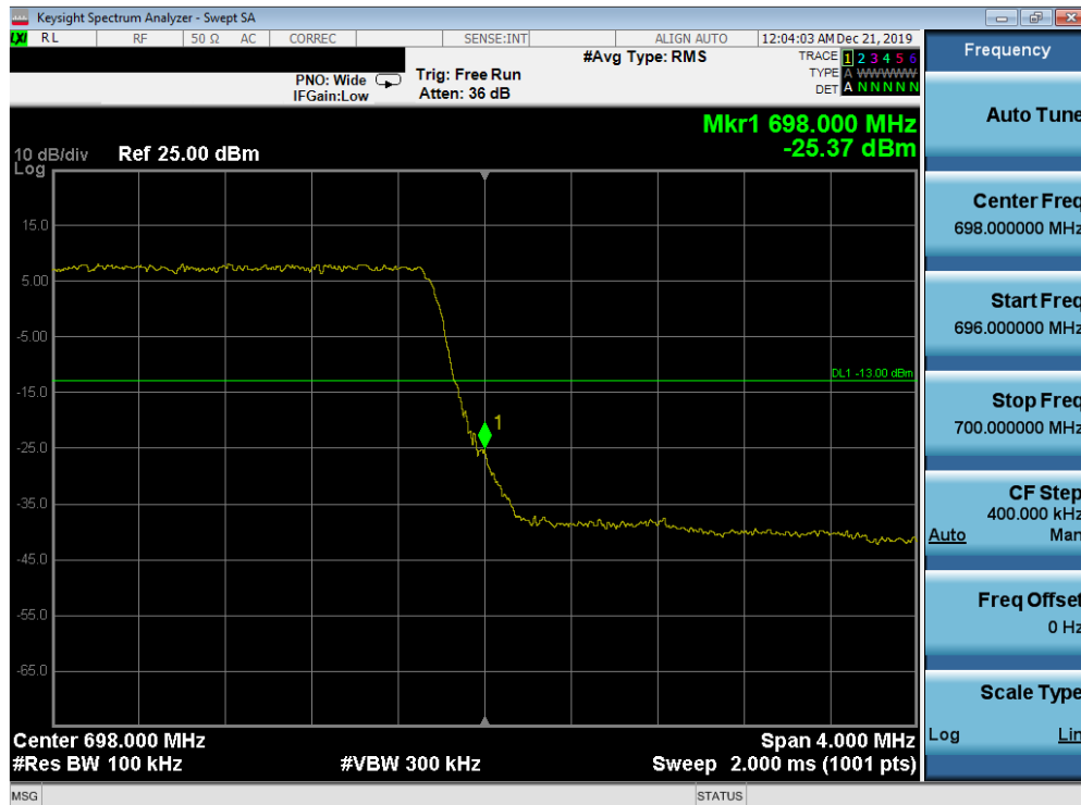
Plot 7-203. Upper Band Edge Plot (Band 71 - 5.0MHz QPSK - Full RB Configuration)
