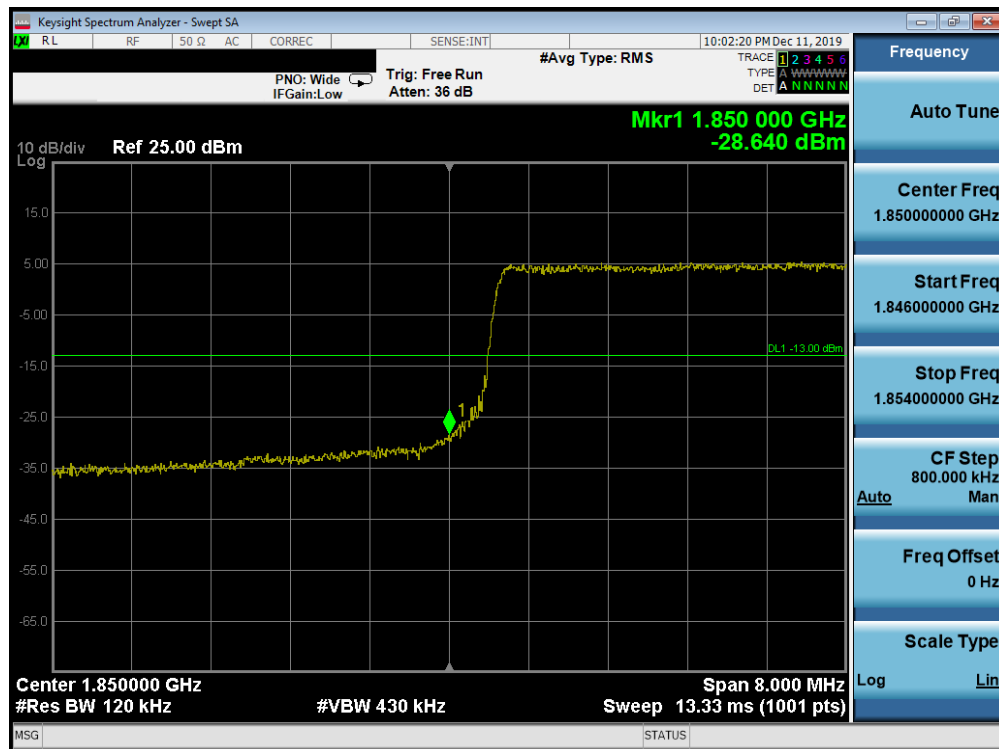
Plot 7-2056. Lower Band Edge Plot (Band 25/2 - 10.0MHz QPSK - Full RB Configuration)
