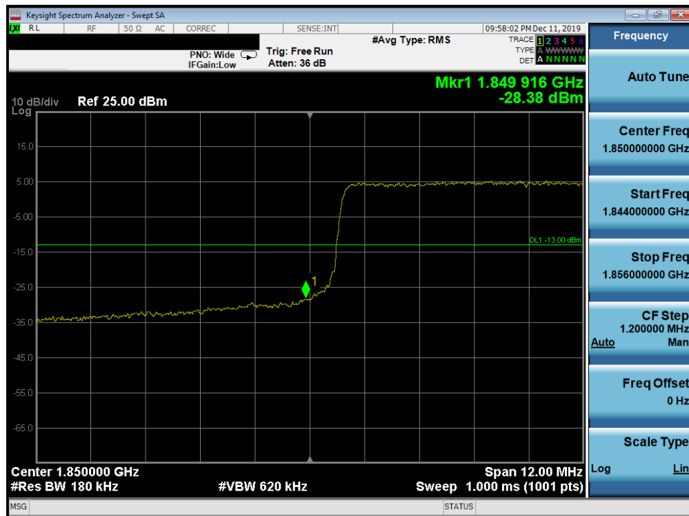
Plot 7-2112. Lower Band Edge Plot (Band 25/2 - 15.0MHz QPSK - Full RB Configuration)
