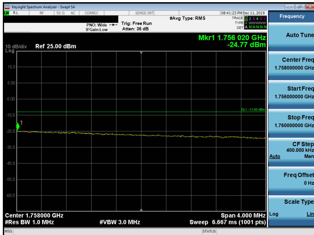
Plot 7-178. Upper Extended Band Edge Plot (Band 4 - 15.0MHz QPSK - Full RB Configuration)
