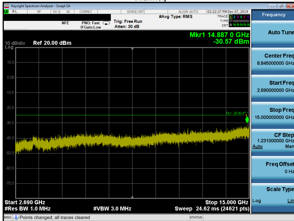
Plot 7-166. Conducted Spurious Plot (Band 41 PC3 - 20.0MHz QPSK - RB Size 1, RB Offset 0 - Low Channel)
