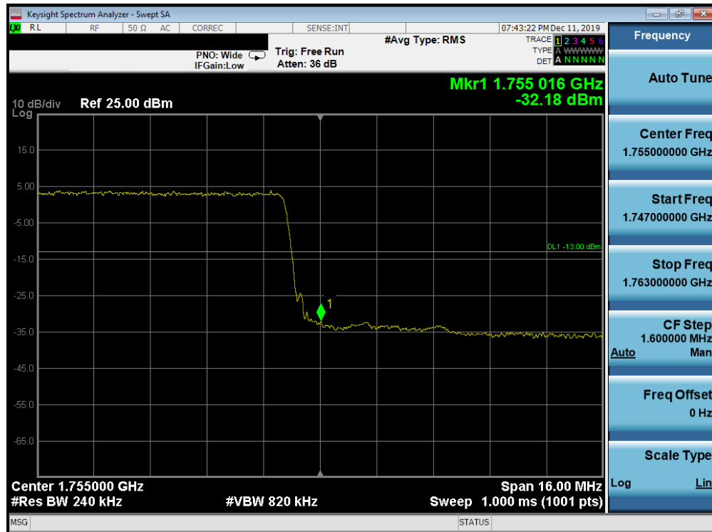
Plot 7-183. Upper Band Edge Plot (Band 4 - 20.0MHz QPSK - Full RB Configuration)
