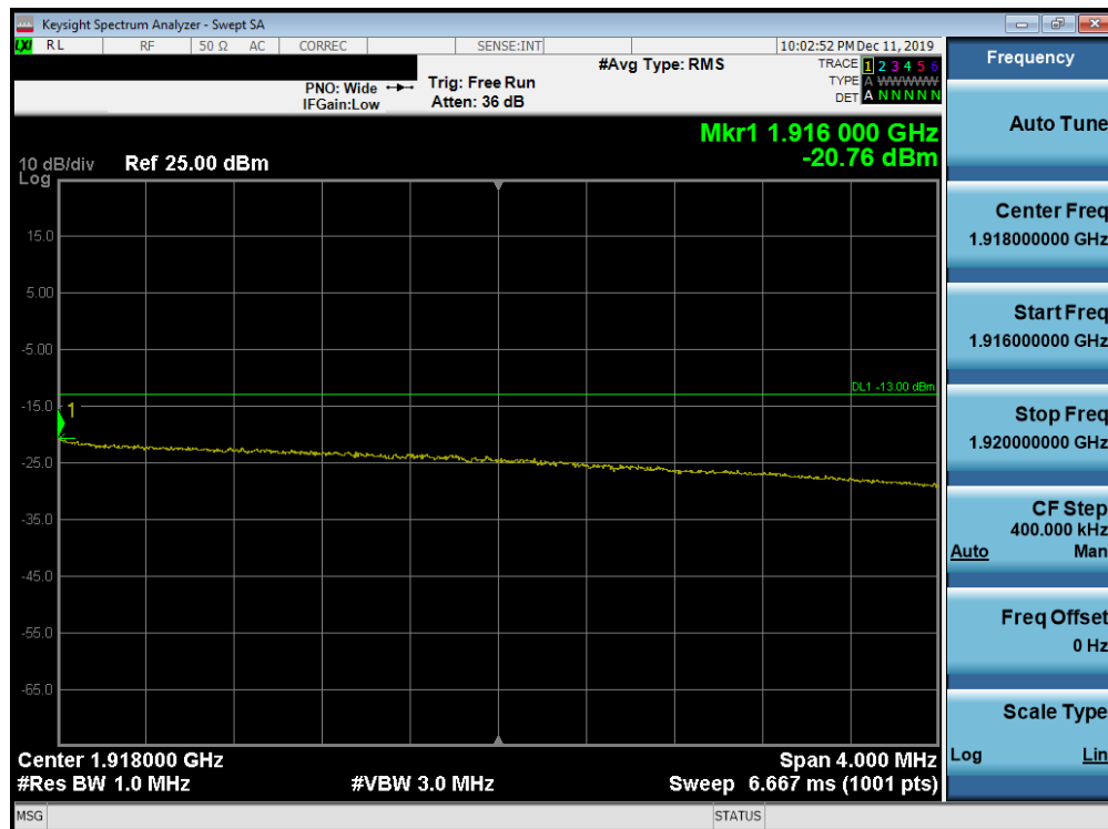
Plot 7-2101. Upper Extended Band Edge Plot (Band 25 - 10.0MHz QPSK - Full RB Configuration)
