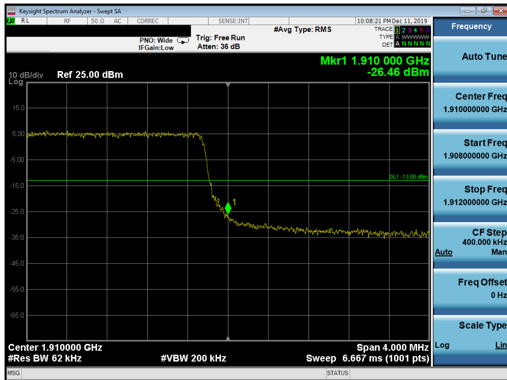
Plot 7-201. Upper Band Edge Plot (Band 2 - 5.0MHz QPSK - Full RB Configuration)
