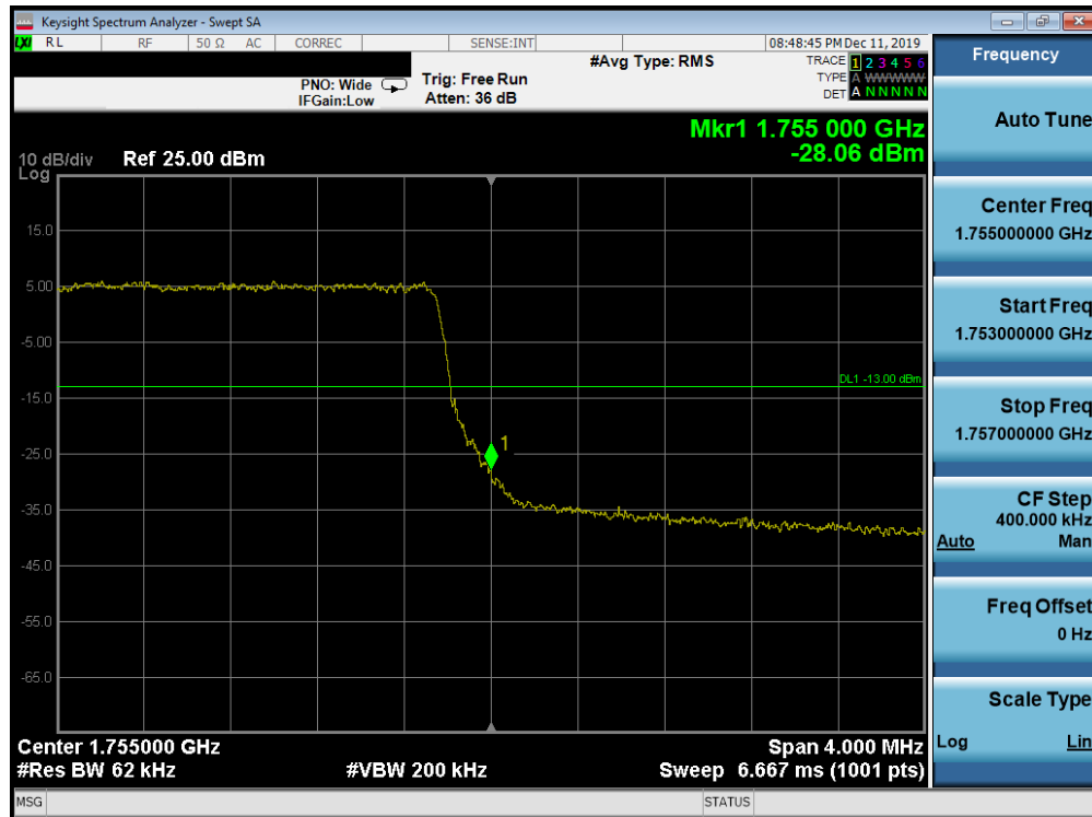
Plot 7-246. Upper Band Edge Plot (Band 4 - 5.0MHz QPSK - Full RB Configuration)
