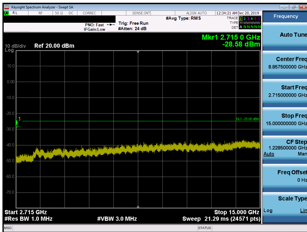
Plot 7-191. Conducted Spurious Plot (Band 41 PC2 - 20.0MHz QPSK - RB Size 1, RB Offset 99 - High Channel)
