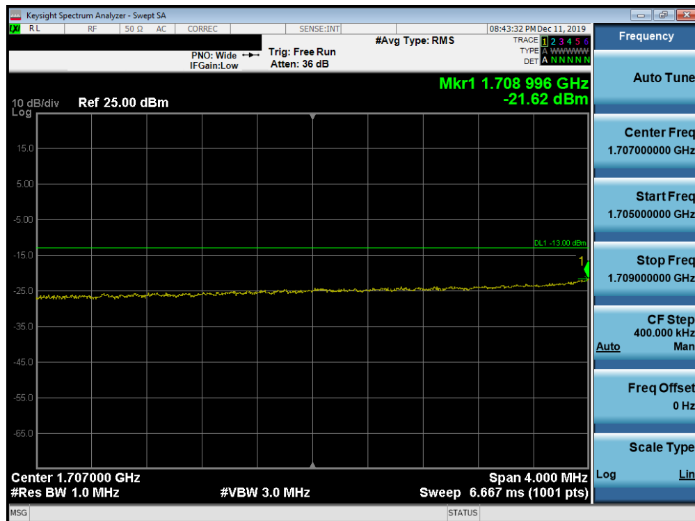
Plot 7-251. Lower Extended Band Edge Plot (Band 66/4 - 10.0MHz QPSK - Full RB Configuration)
