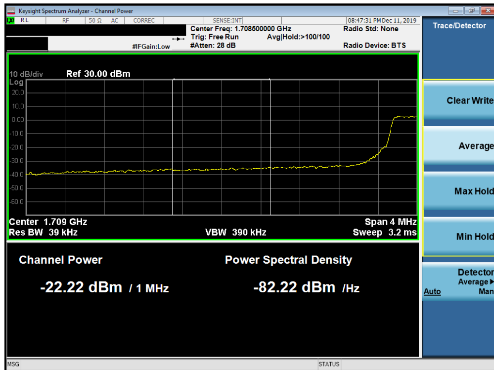
Plot 7-245. Lower Extended Band Edge Plot (Band 66/4 - 5.0MHz QPSK - Full RB Configuration)
