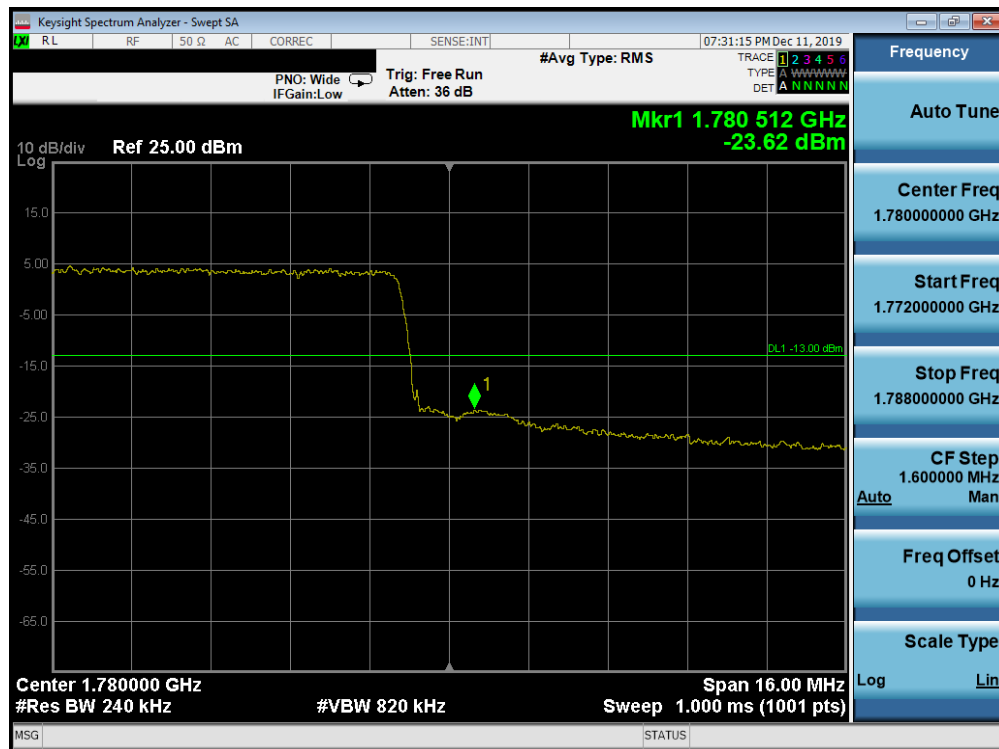
Plot 7-185. Upper Band Edge Plot (Band 66 - 20.0MHz QPSK - Full RB Configuration)
