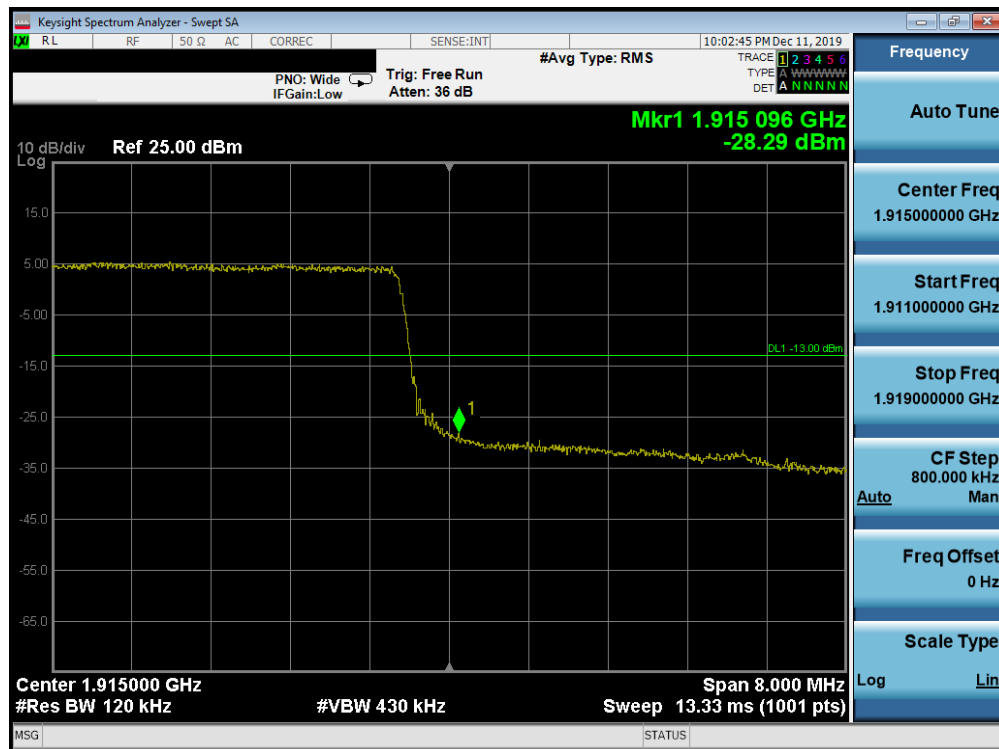
Plot 7-2090. Upper Band Edge Plot (Band 25 - 10.0MHz QPSK - Full RB Configuration)
