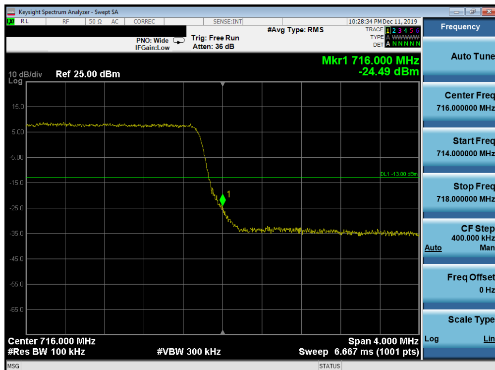
Plot 7-215. Upper Band Edge Plot (Band 12 - 5.0MHz QPSK - Full RB Configuration)
