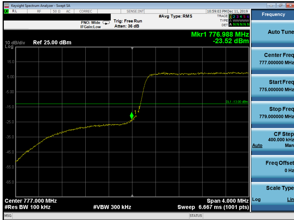
Plot 7-218. Lower Band Edge Plot (Band 13 - 5.0MHz QPSK - Full RB Configuration)
