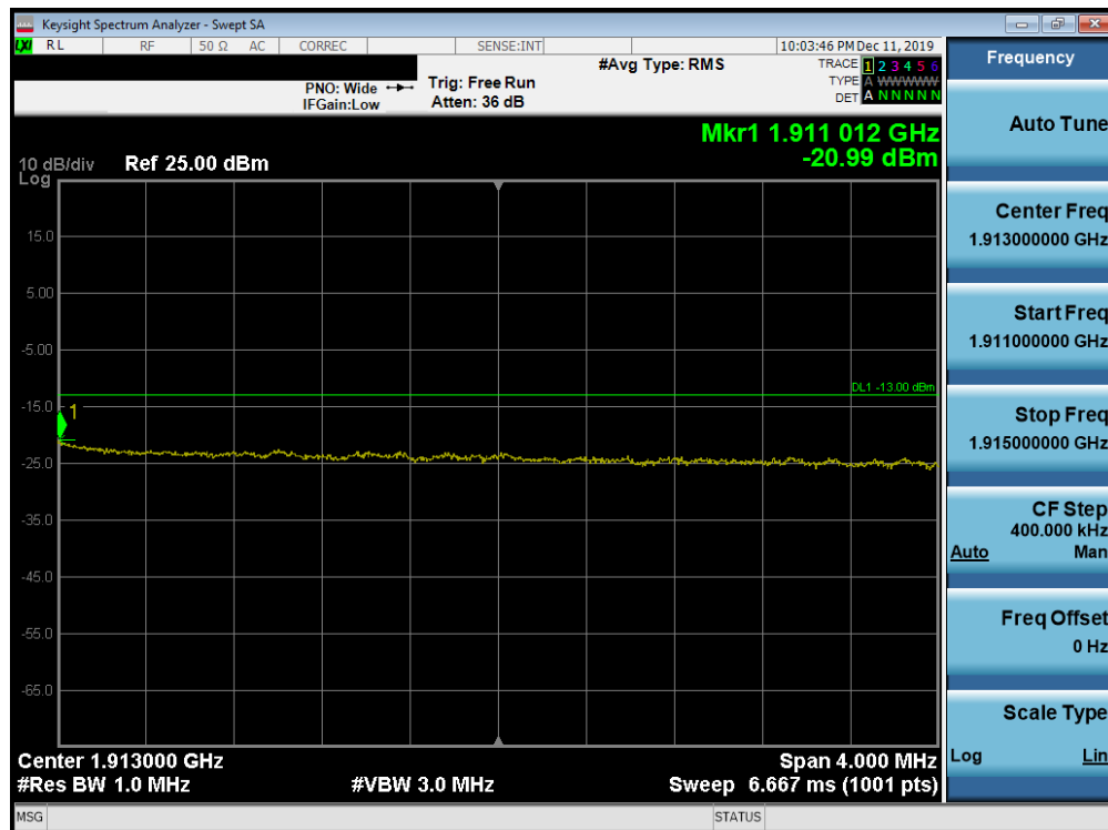
Plot 7-2089. Upper Extended Band Edge Plot (Band 2 - 10.0MHz QPSK - Full RB Configuration)
