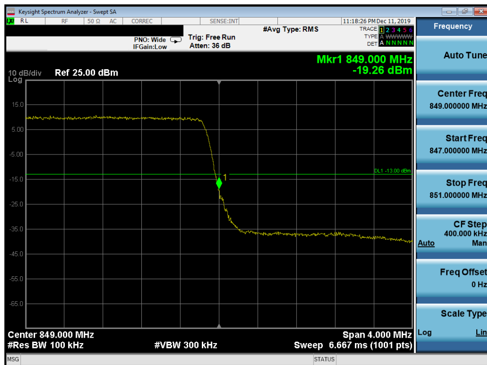
Plot 7-173. Upper Band Edge Plot (Band 26/5 - 3.0MHz QPSK - Full RB Configuration)
