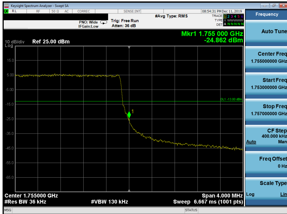
Plot 7-240. Upper Band Edge Plot (Band 4 - 3.0MHz QPSK - Full RB Configuration)
