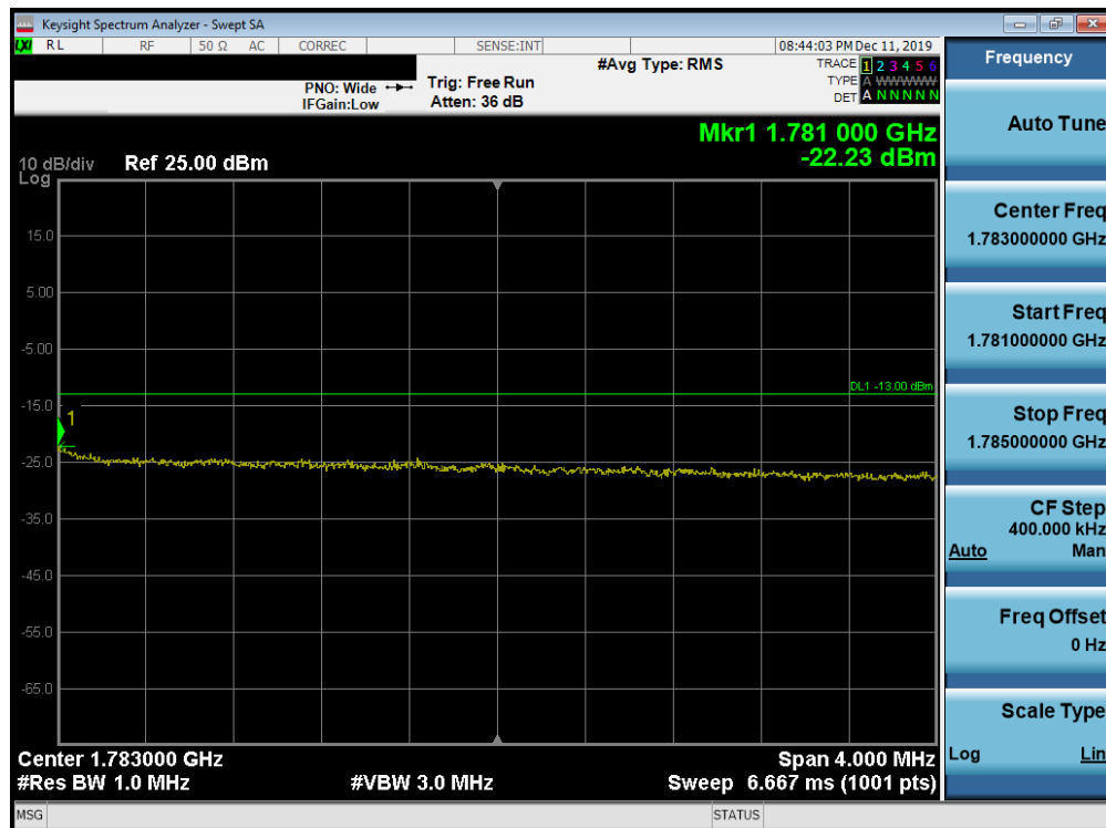
Plot 7-174. Upper Extended Band Edge Plot (Band 66 - 10.0MHz QPSK - Full RB Configuration)
