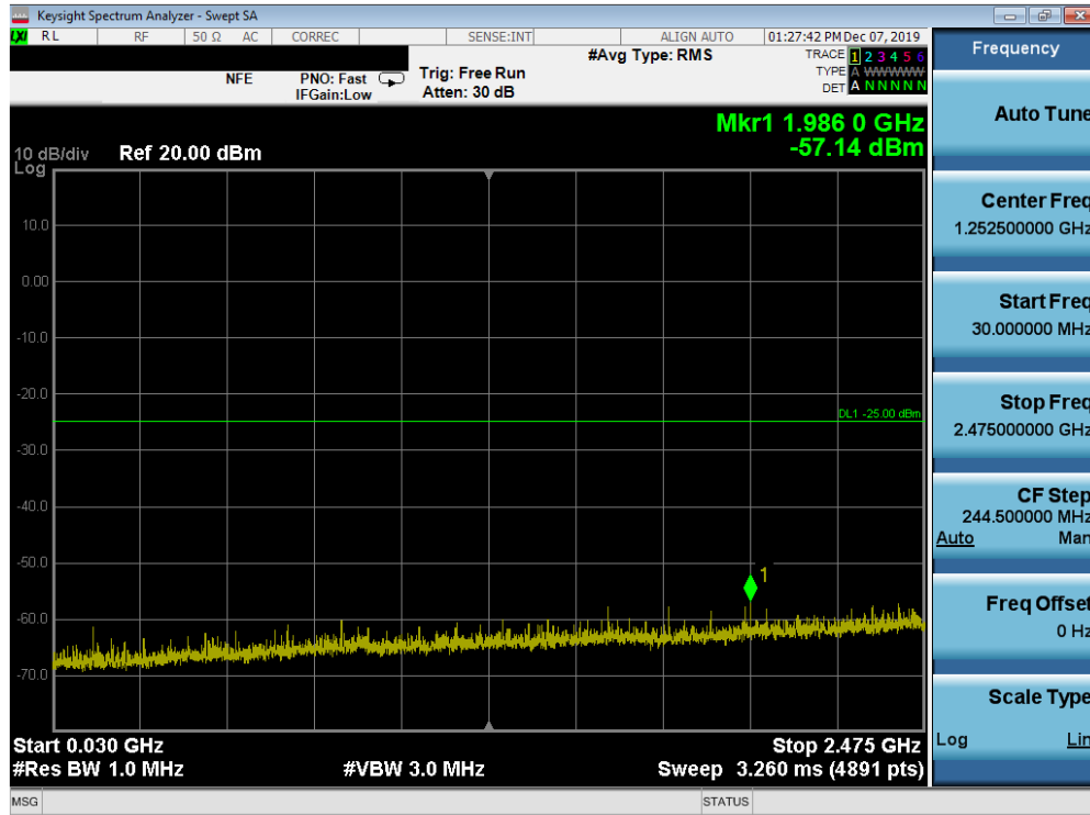
Plot 7-157. Conducted Spurious Plot (Band 7 - 20.0MHz QPSK - RB Size 1, RB Offset 0 - Low Channel)
