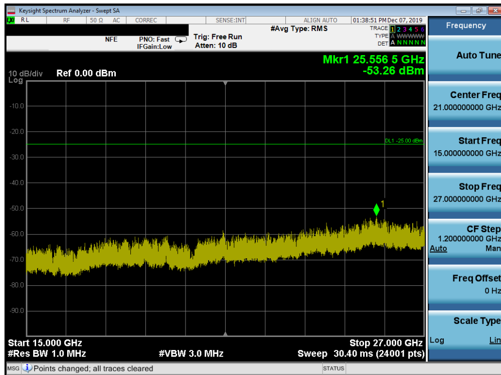
Plot 7-165. Conducted Spurious Plot (Band 7 - 20.0MHz QPSK - RB Size 1, RB Offset 0 - High Channel)
