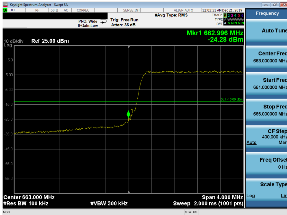
Plot 7-202. Lower Band Edge Plot (Band 71 - 5.0MHz QPSK - Full RB Configuration)
