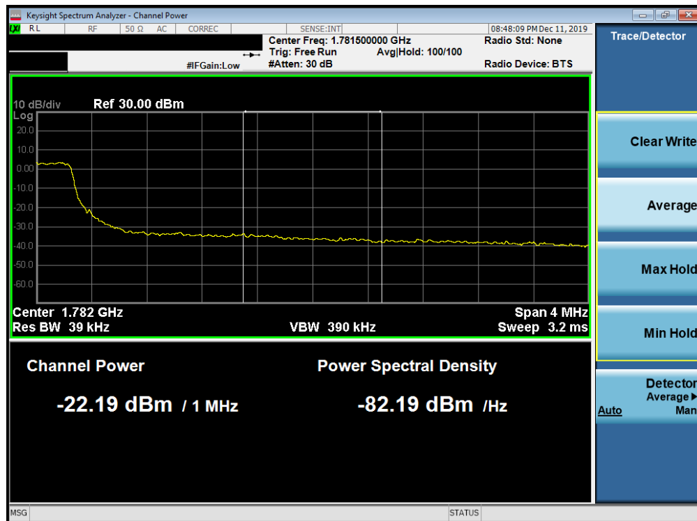
Plot 7-249. Upper Extended Band Edge Plot (Band 66 - 5.0MHz QPSK - Full RB Configuration)
