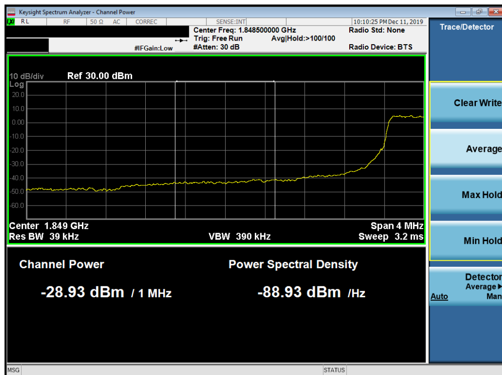
Plot 7-194. Lower Extended Band Edge Plot (Band 25/2 - 3.0MHz QPSK - Full RB Configuration)
