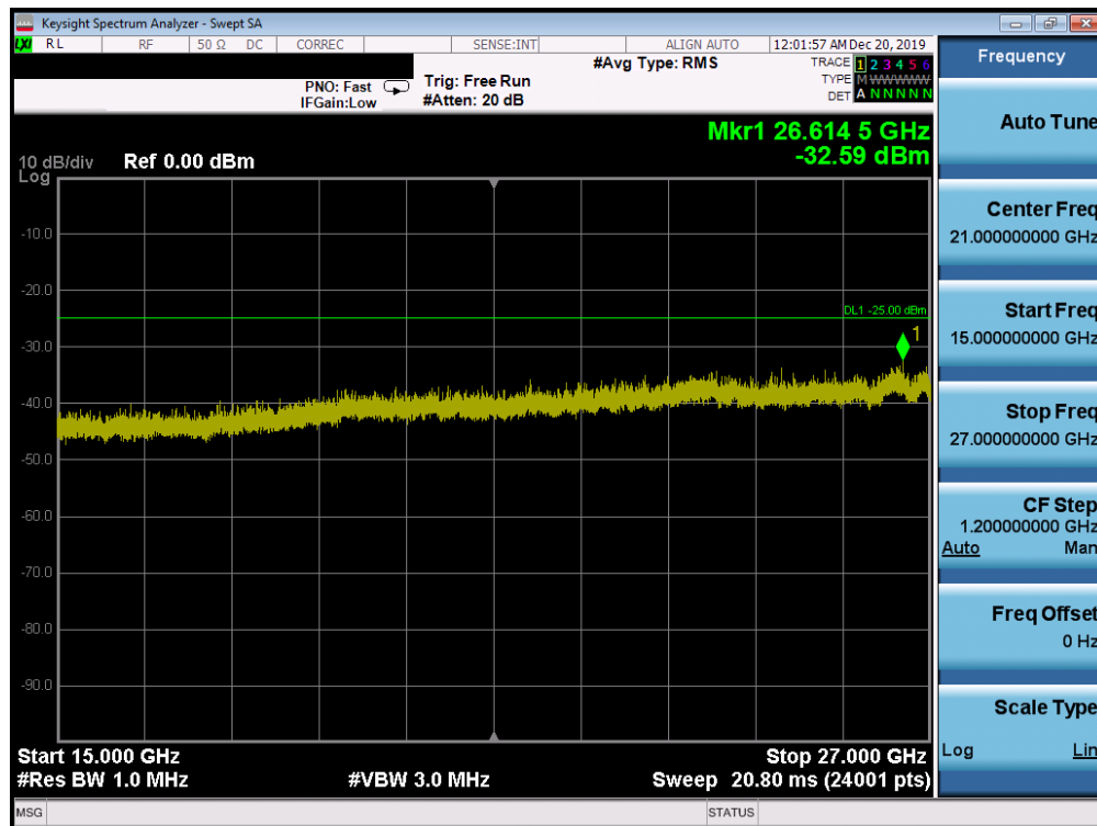
Plot 7-186. Conducted Spurious Plot (Band 41 PC2 - 20.0MHz QPSK - RB Size 1, RB Offset 0 - Low Channel)
