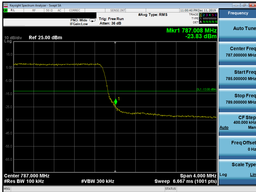
Plot 7-219. Upper Band Edge Plot (Band 13 - 5.0MHz QPSK - Full RB Configuration)
