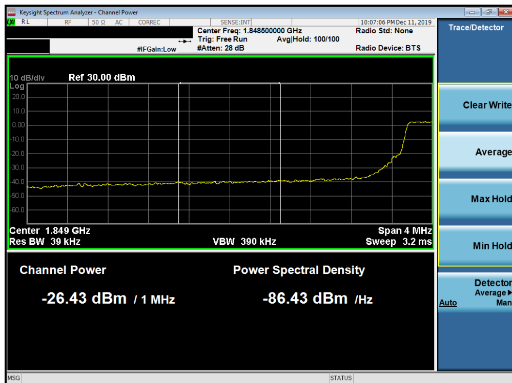
Plot 7-200. Lower Extended Band Edge Plot (Band 25/2 - 5.0MHz QPSK - Full RB Configuration)
