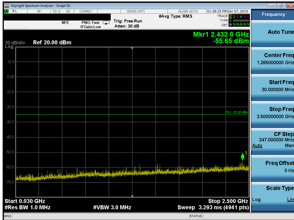
Plot 7-163. Conducted Spurious Plot (Band 7 - 20.0MHz QPSK - RB Size 1, RB Offset 0 - High Channel)
