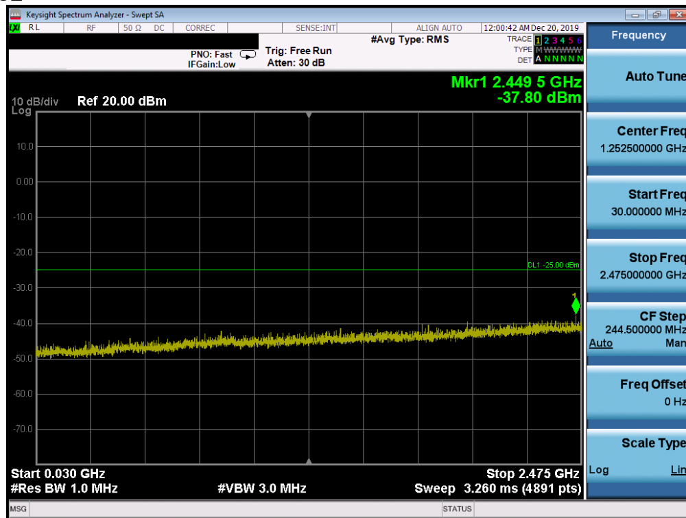
Plot 7-184. Conducted Spurious Plot (Band 41 PC2 - 20.0MHz QPSK - RB Size 1, RB Offset 0 - Low Channel)
