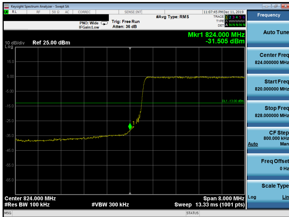
Plot 7-228 Lower Band Edge Plot (Band 26/5 - 10.0MHz QPSK - Full RB Configuration)
