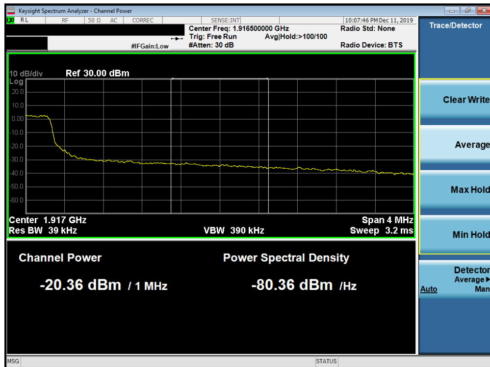
Plot 7-204. Upper Extended Band Edge Plot (Band 25 - 5.0MHz QPSK - Full RB Configuration)
