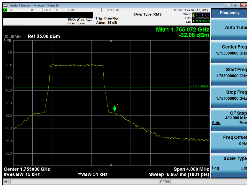
Plot 7-234. Upper Band Edge Plot (Band 4 - 1.4MHz QPSK - Full RB Configuration)
