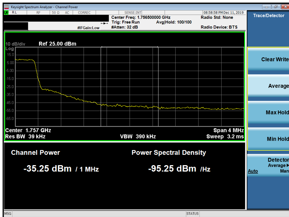
Plot 7-235. Upper Extended Band Edge Plot (Band 4 - 1.4MHz QPSK - Full RB Configuration)
