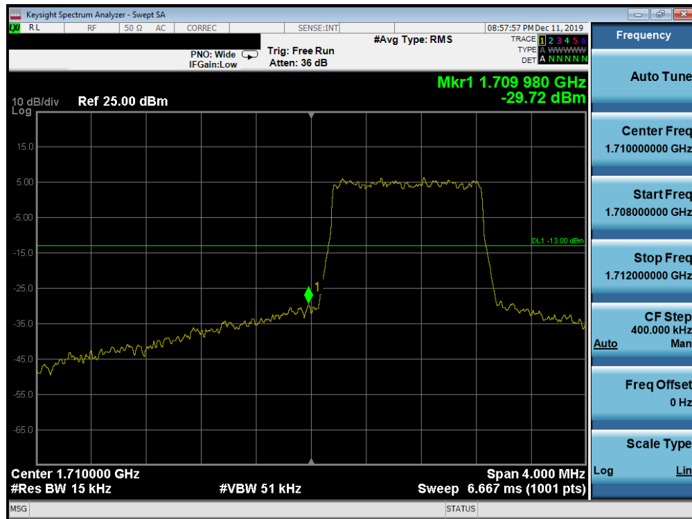
Plot 7-232. Lower Band Edge Plot (Band 66/4 - 1.4MHz QPSK - Full RB Configuration)
