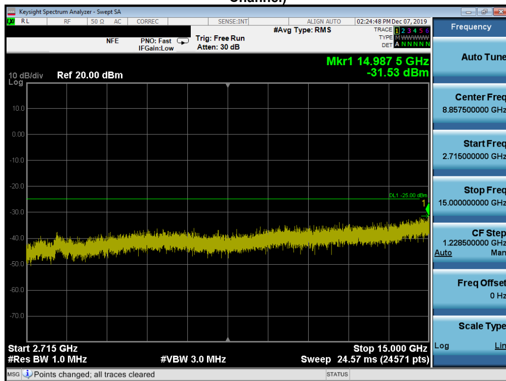
Plot 7-200. Conducted Spurious Plot (Band 41 PC3 - 20.0MHz QPSK - RB Size 1, RB Offset 0 - High Channel)
