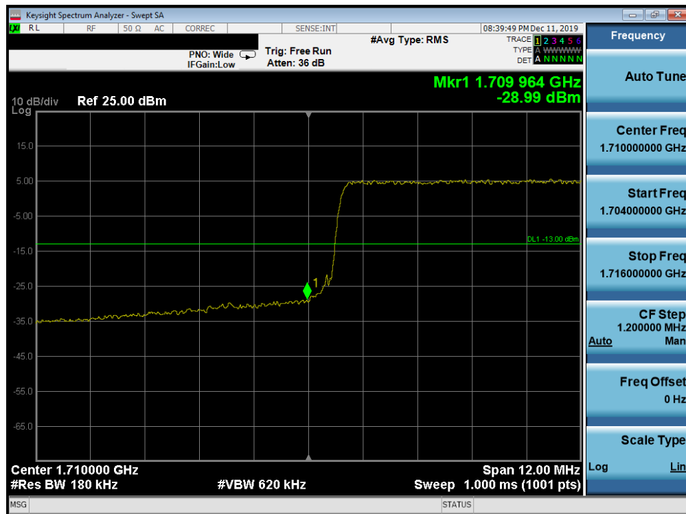
Plot 7-175. Lower Band Edge Plot (Band 66/4 - 15.0MHz QPSK - Full RB Configuration)
