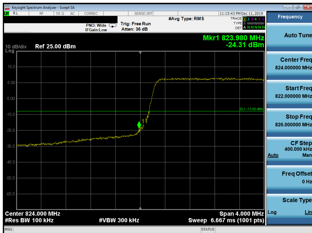
Plot 7-226. Lower Band Edge Plot (Band 26/5 - 5.0MHz QPSK - Full RB Configuration)
