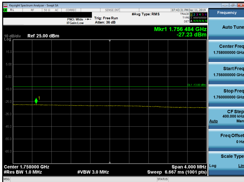
Plot 7-184. Upper Extended Band Edge Plot (Band 4 - 20.0MHz QPSK - Full RB Configuration)
