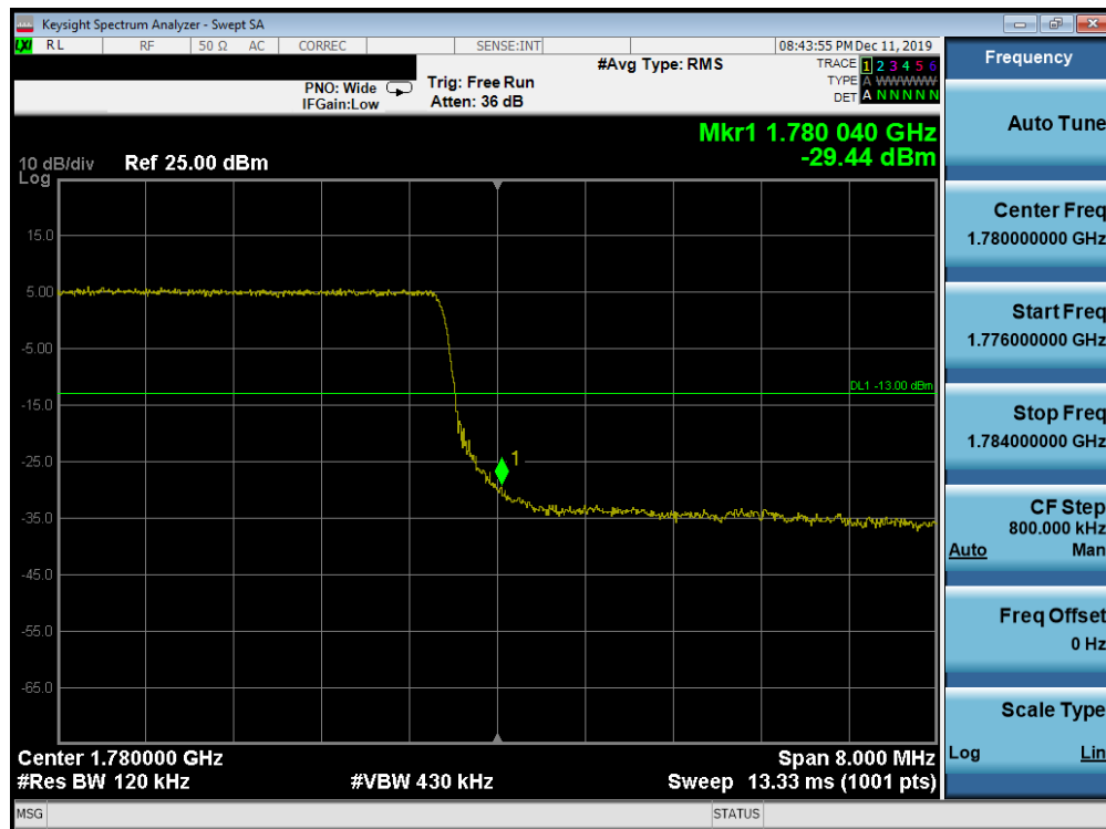
Plot 7-254. Upper Band Edge Plot (Band 66 - 10.0MHz QPSK - Full RB Configuration)
