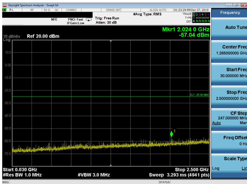
Plot 7-160. Conducted Spurious Plot (Band 7 - 20.0MHz QPSK - RB Size 1, RB Offset 0 - Mid Channel)
