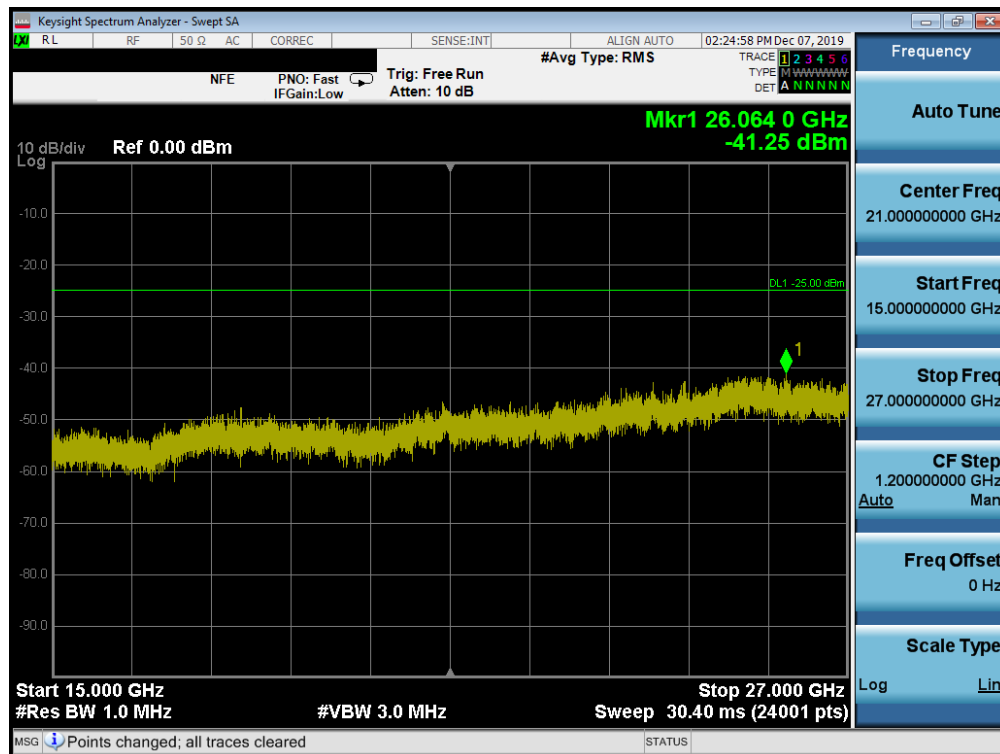
Plot 7-172. Conducted Spurious Plot (Band 41 PC3 - 20.0MHz QPSK - RB Size 1, RB Offset 0 - High Channel)
