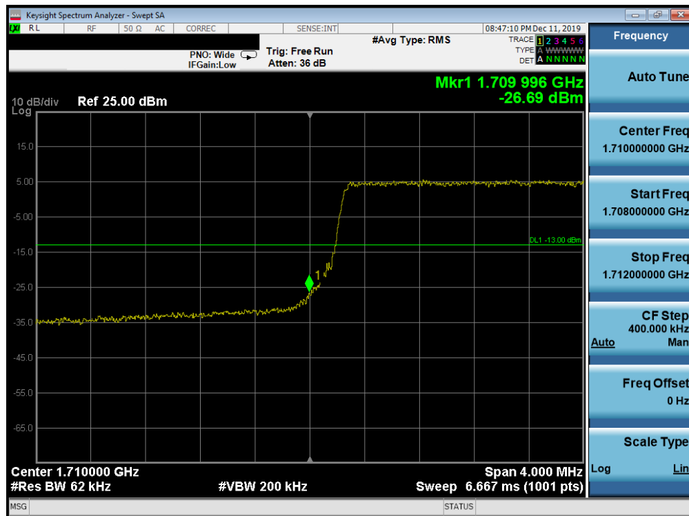
Plot 7-244. Lower Band Edge Plot (Band 66/4 - 5.0MHz QPSK - Full RB Configuration)
