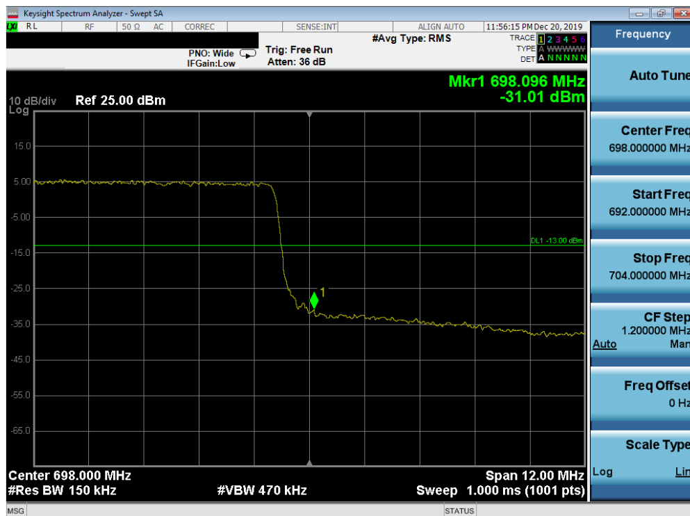
Plot 7-207. Upper Band Edge Plot (Band 71 - 15.0MHz QPSK - Full RB Configuration)
