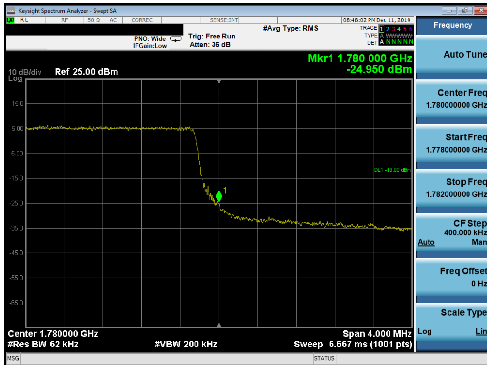
Plot 7-248. Upper Band Edge Plot (Band 66 - 5.0MHz QPSK - Full RB Configuration)
