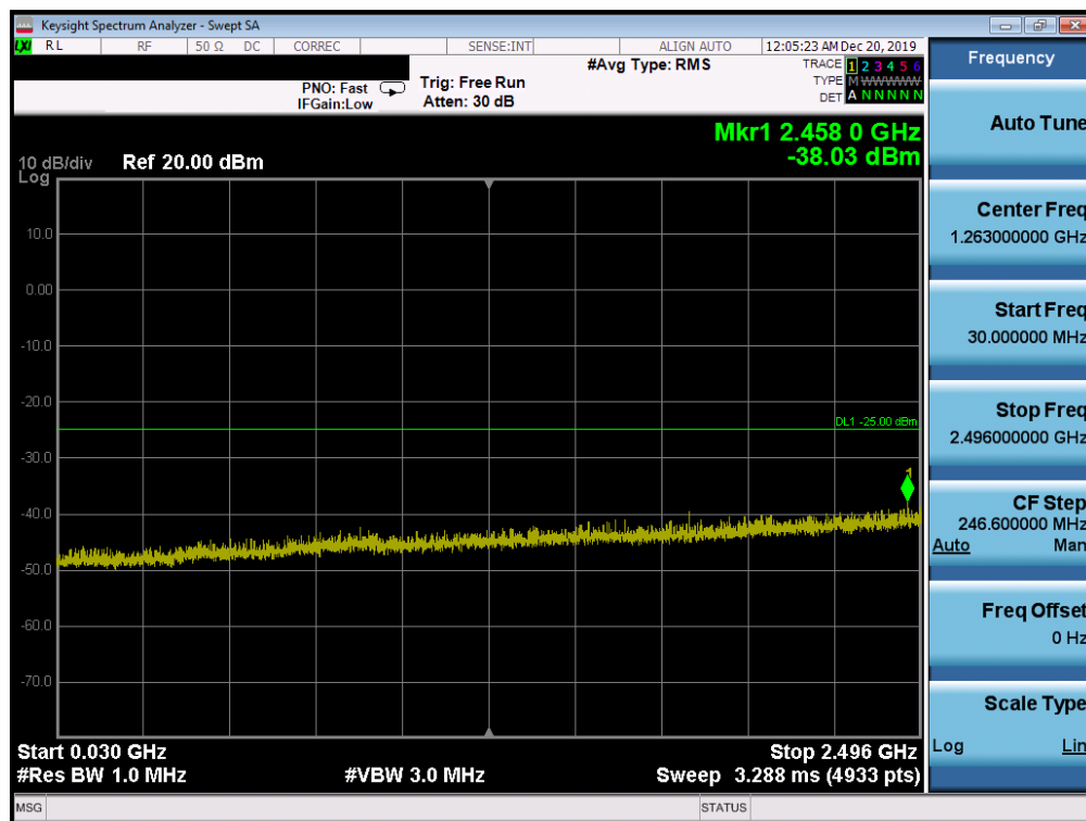
Plot 7-187. Conducted Spurious Plot (Band 41 PC2 - 20.0MHz QPSK - RB Size 1, RB Offset 0 - Mid Channel)
