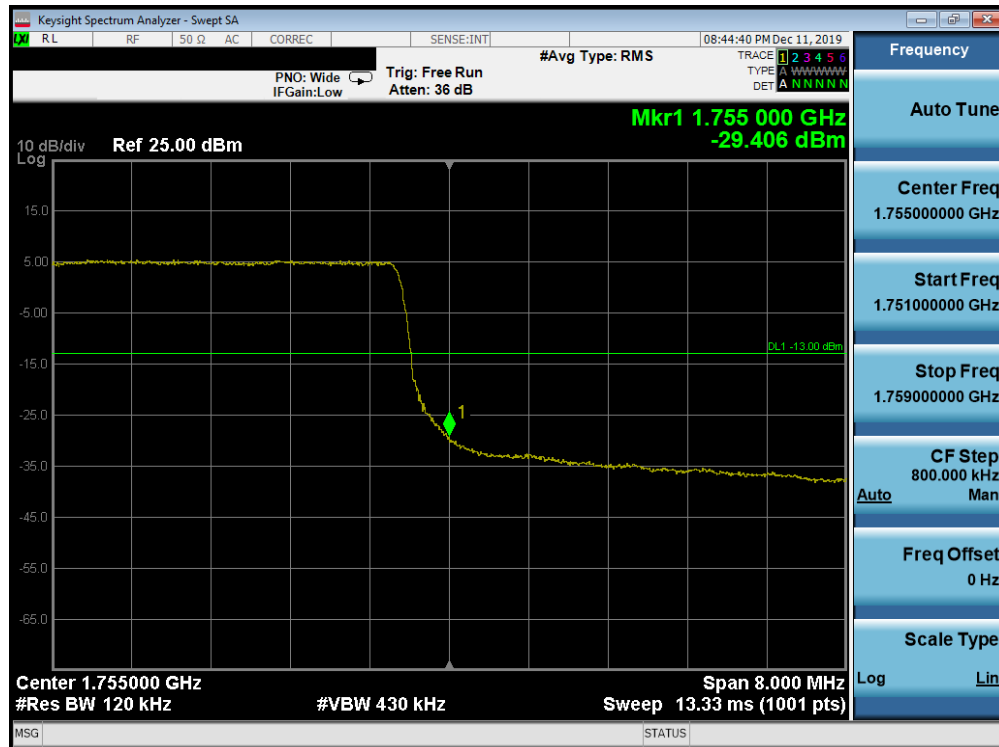
Plot 7-252. Upper Band Edge Plot (Band 4 - 10.0MHz QPSK - Full RB Configuration)
