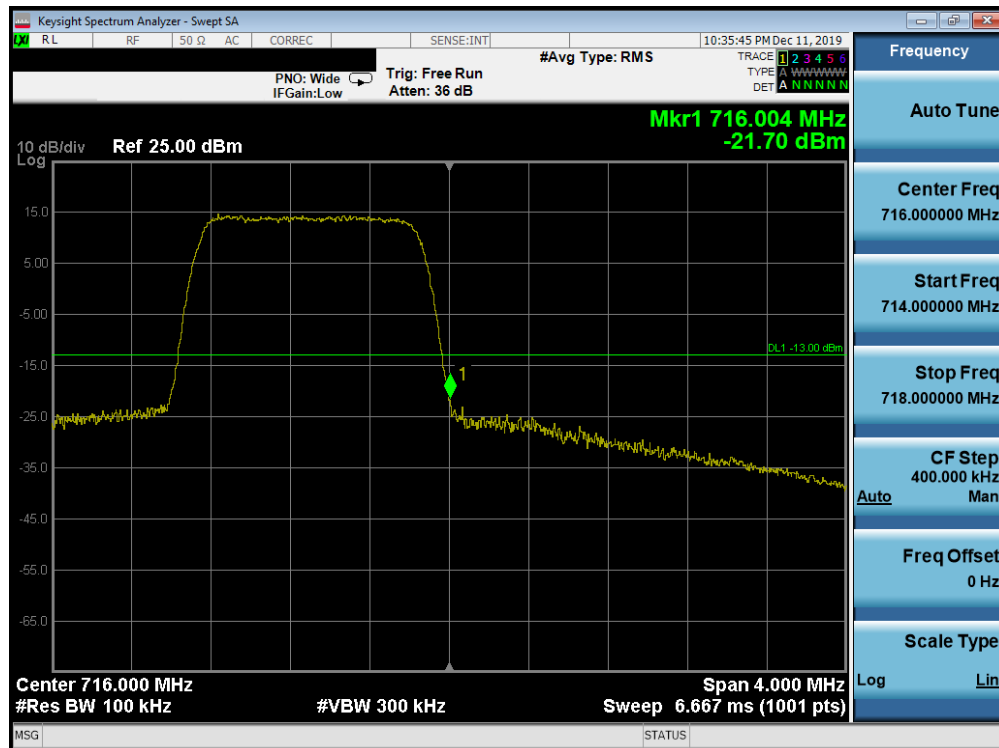
Plot 7-211. Upper Band Edge Plot (Band 12 - 1.4MHz QPSK - Full RB Configuration)
