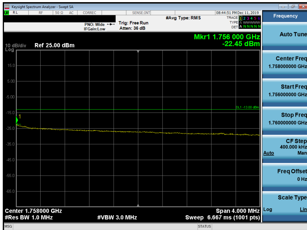
Plot 7-253. Upper Extended Band Edge Plot (Band 4 - 10.0MHz QPSK - Full RB Configuration)
