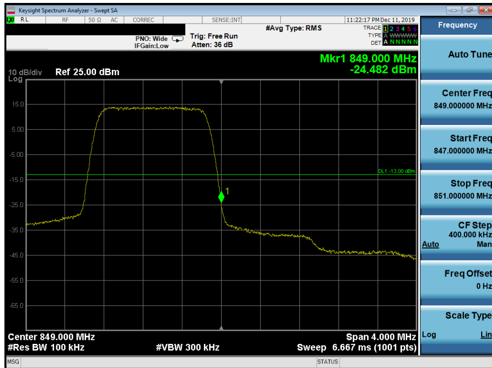
Plot 7-223. Upper Band Edge Plot (Band 26/5 - 1.4MHz QPSK - Full RB Configuration)
