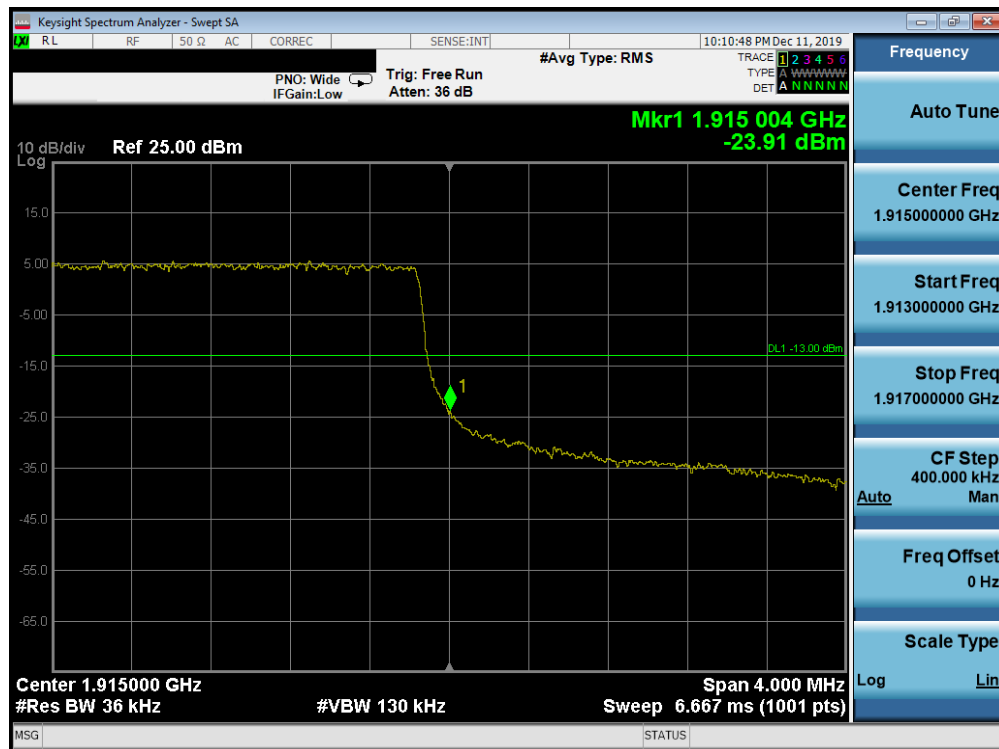
Plot 7-197. Upper Band Edge Plot (Band 25 - 3.0MHz QPSK - Full RB Configuration)
