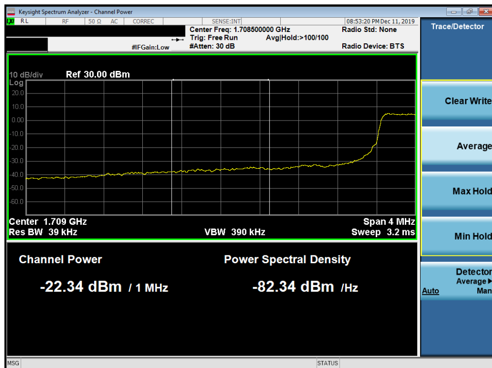
Plot 7-239. Lower Extended Band Edge Plot (Band 66/4 - 3.0MHz QPSK - Full RB Configuration)
