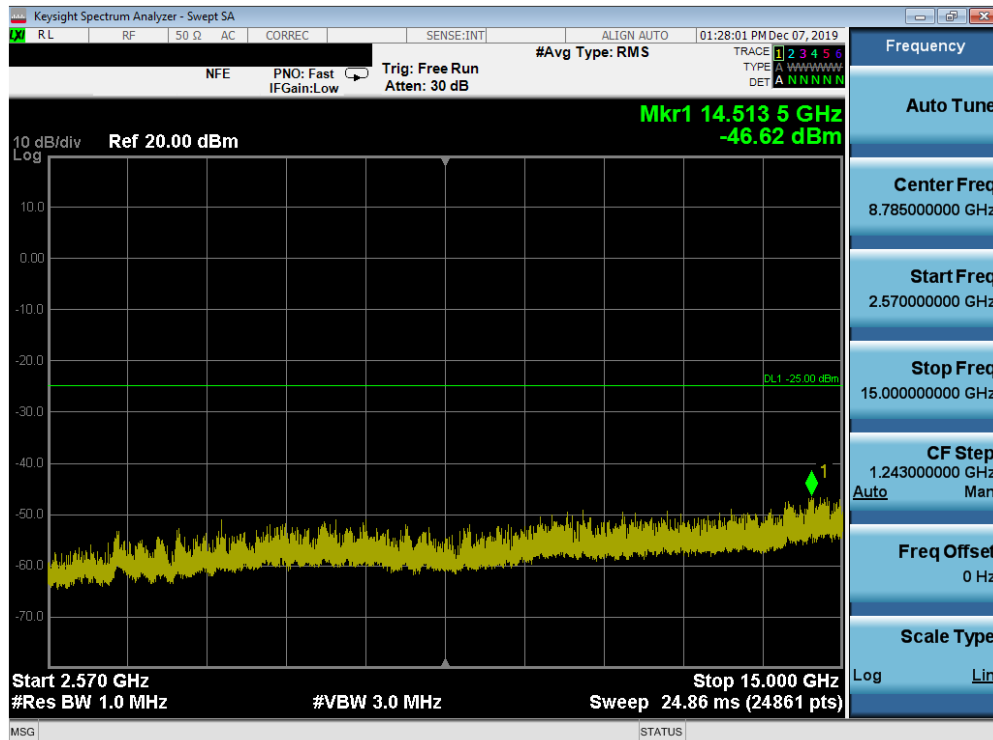
Plot 7-158. Conducted Spurious Plot (Band 7 - 20.0MHz QPSK - RB Size 1, RB Offset 0 - Low Channel)
