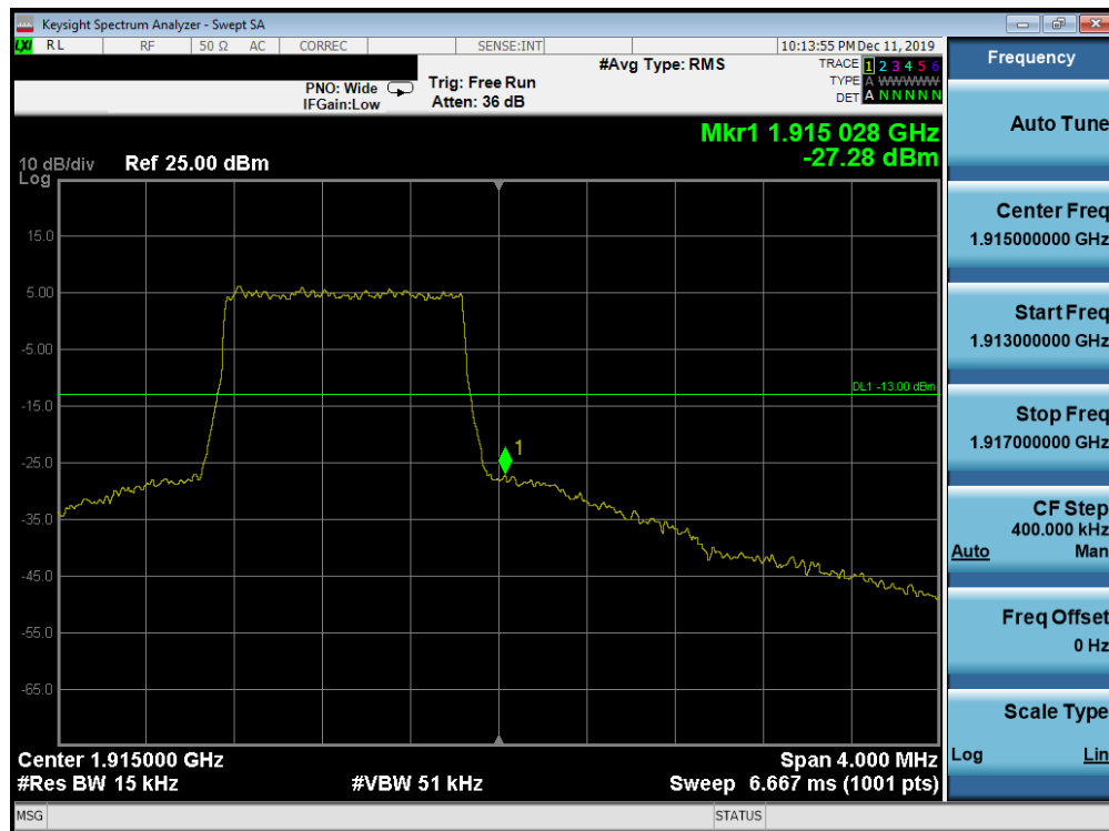
Plot 7-191. Upper Band Edge Plot (Band 25 - 1.4MHz QPSK - Full RB Configuration)
