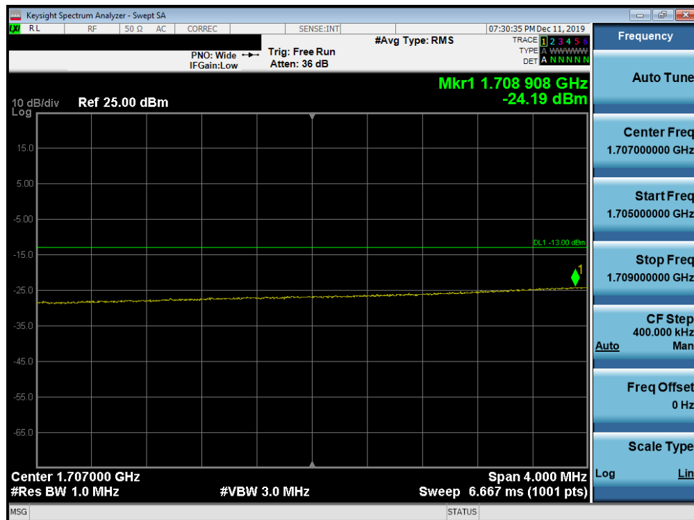
Plot 7-182. Lower Extended Band Edge Plot (Band 66/4 - 20.0MHz QPSK - Full RB Configuration)
