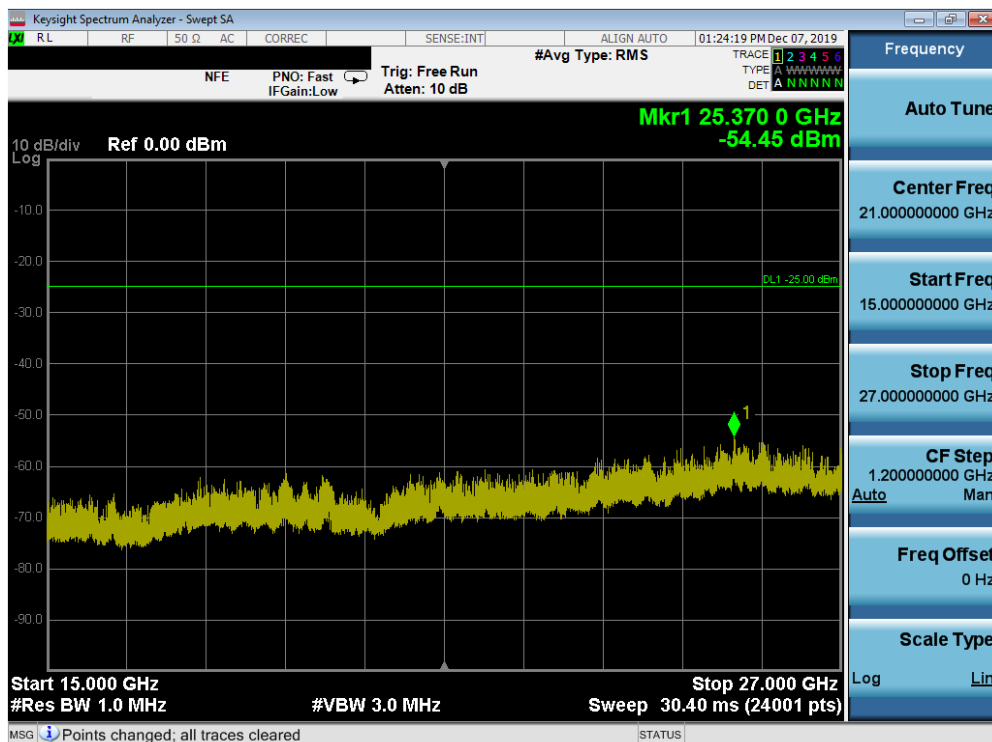
Plot 7-162. Conducted Spurious Plot (Band 7 - 20.0MHz QPSK - RB Size 1, RB Offset 0 - Mid Channel)
