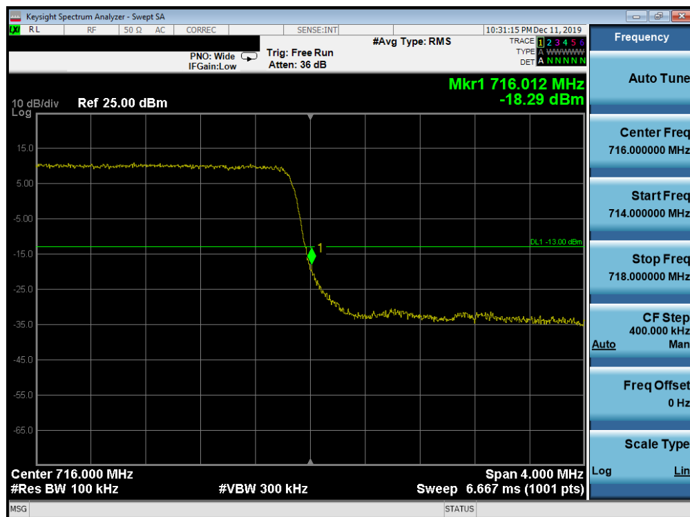
Plot 7-213. Upper Band Edge Plot (Band 12 - 3.0MHz QPSK - Full RB Configuration)
