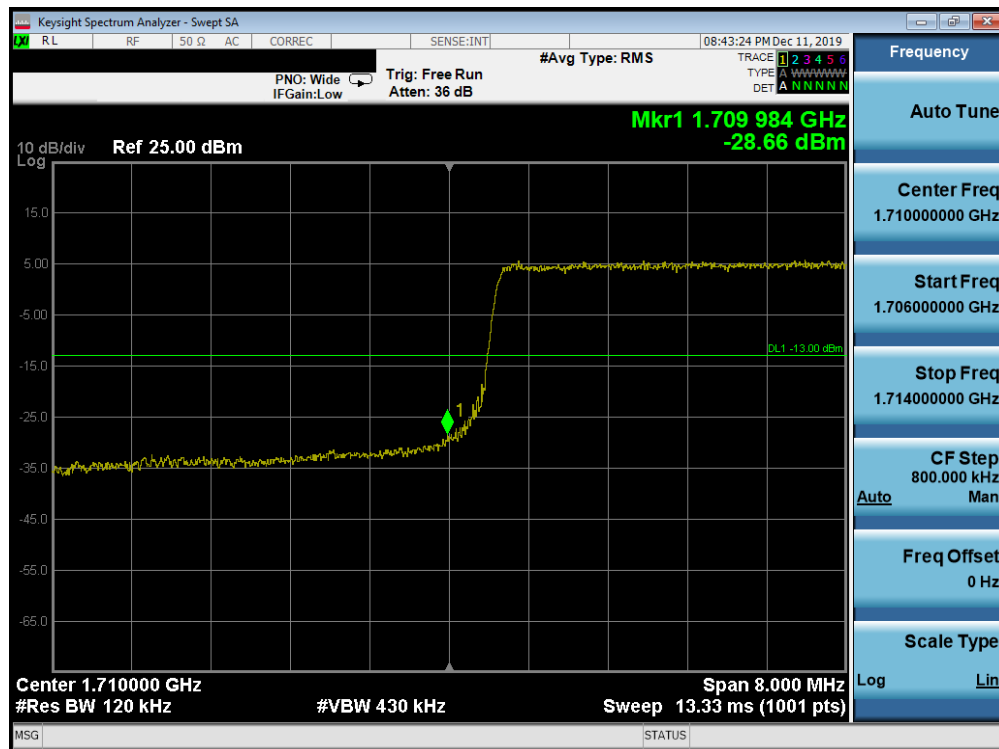
Plot 7-250. Lower Band Edge Plot (Band 66/4 - 10.0MHz QPSK - Full RB Configuration)
