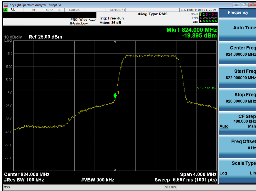
Plot 7-222. Lower Band Edge Plot (Band 26/5 - 1.4MHz QPSK - Full RB Configuration)
