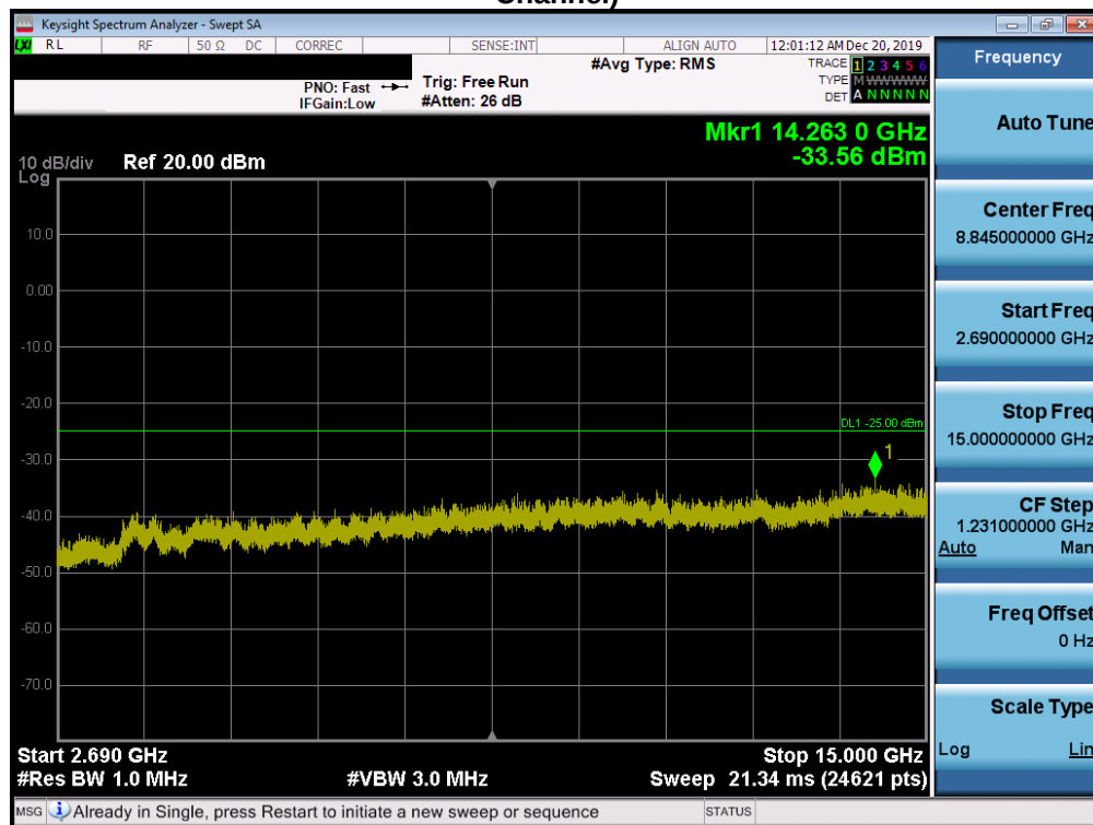
Plot 7-185. Conducted Spurious Plot (Band 41 PC2 - 20.0MHz QPSK - RB Size 1, RB Offset 0 - Low Channel)
