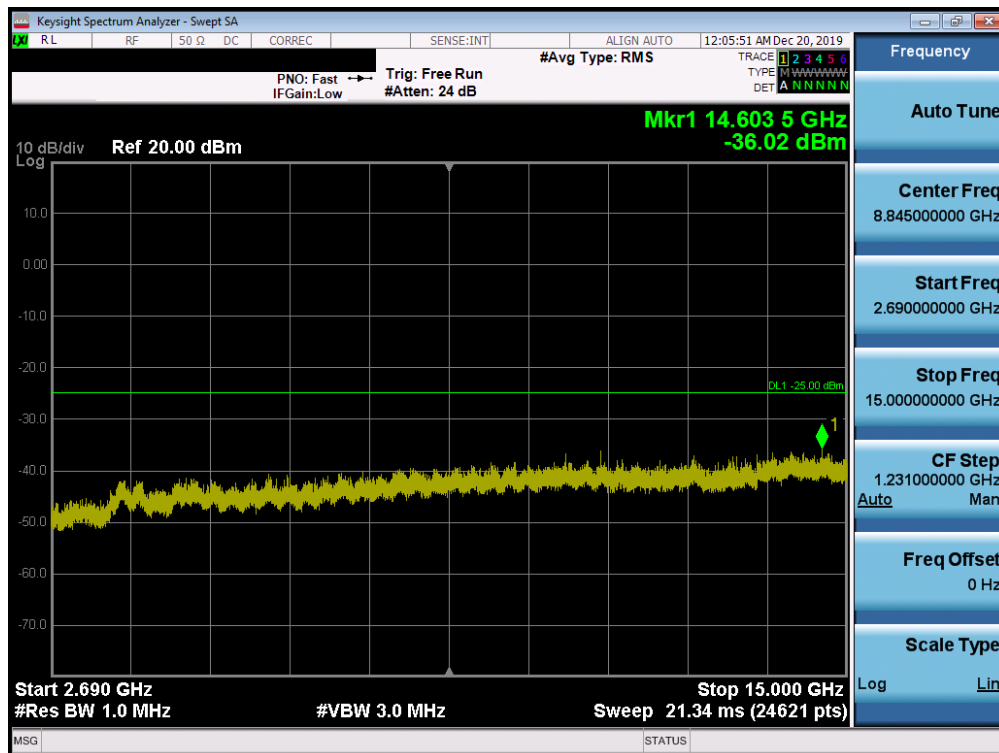
Plot 7-188. Conducted Spurious Plot (Band 41 PC2 - 20.0MHz QPSK - RB Size 1, RB Offset 0 - Mid Channel)
