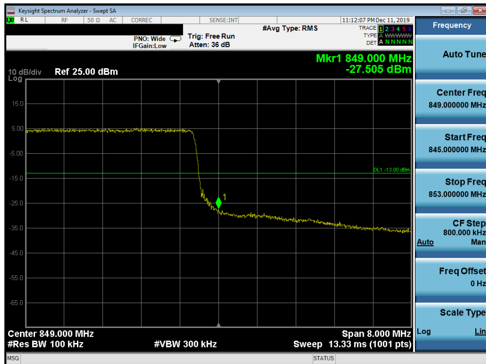
Plot 7-229. Upper Band Edge Plot (Band 26/5 - 10.0MHz QPSK - Full RB Configuration)
