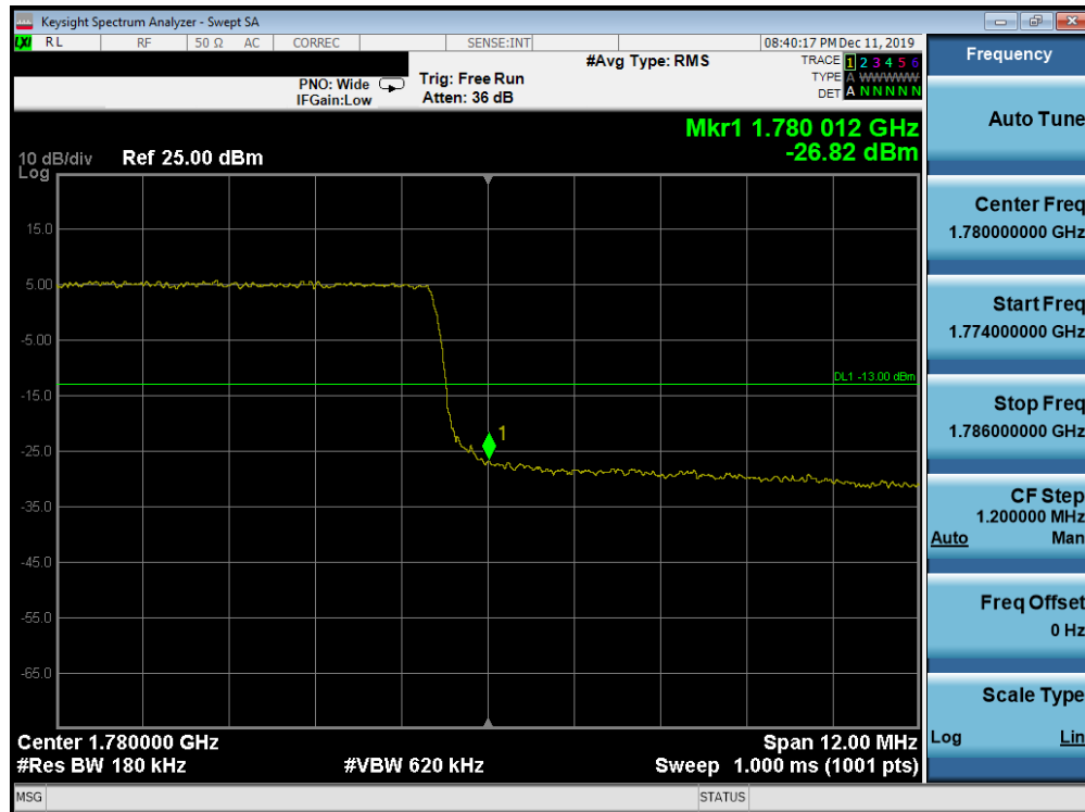
Plot 7-179. Upper Band Edge Plot (Band 66 - 15.0MHz QPSK - Full RB Configuration)
