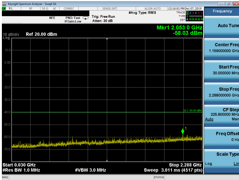
Plot 7-172. Conducted Spurious Plot (Band 30 - 10.0MHz QPSK - RB Size 1, RB Offset 0 - Mid Channel)
