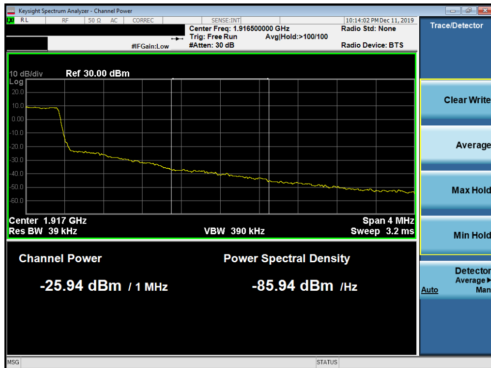
Plot 7-192. Upper Extended Band Edge Plot (Band 25 - 1.4MHz QPSK - Full RB Configuration)
