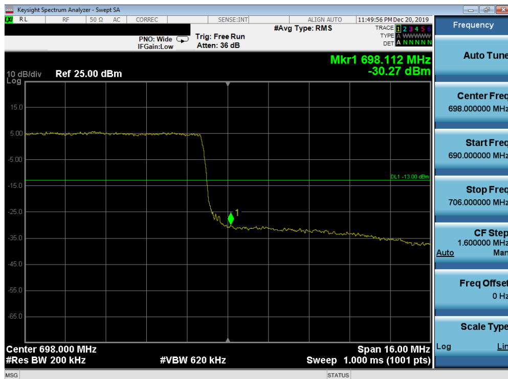
Plot 7-209. Upper Band Edge Plot (Band 71 - 20.0MHz QPSK - Full RB Configuration)
