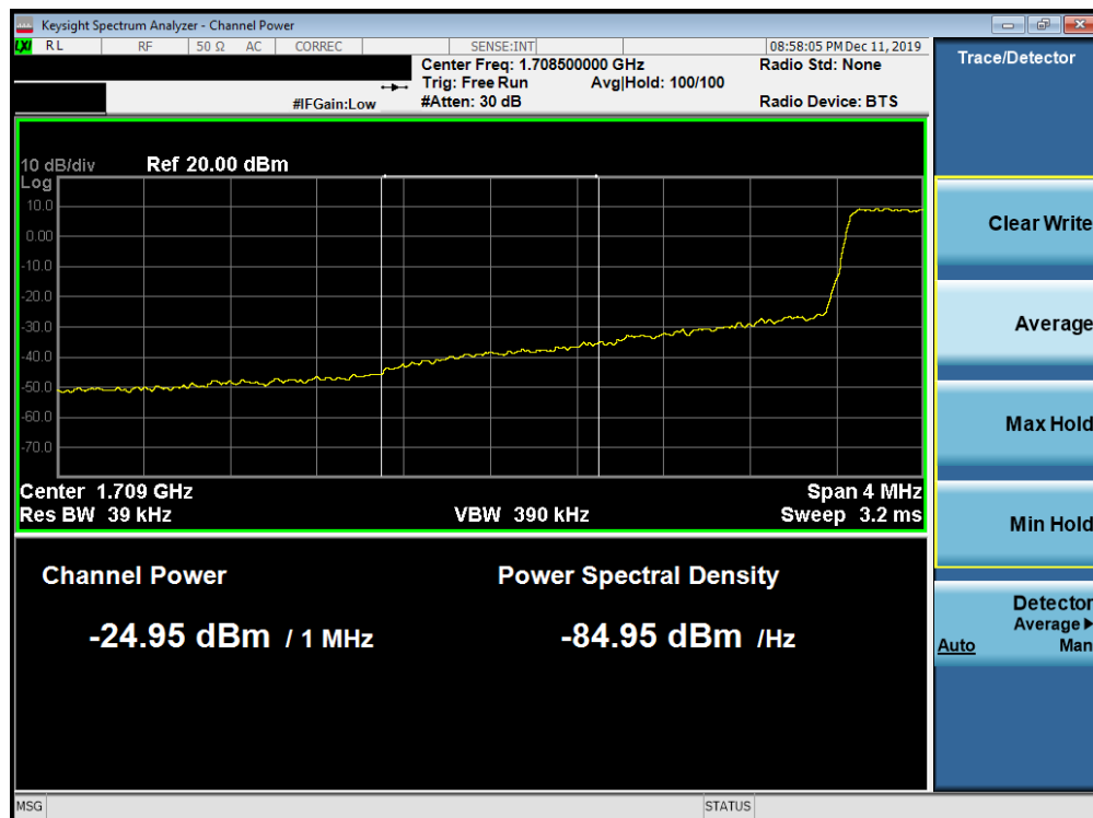
Plot 7-233. Lower Extended Band Edge Plot (Band 66/4 - 1.4MHz QPSK - Full RB Configuration)
