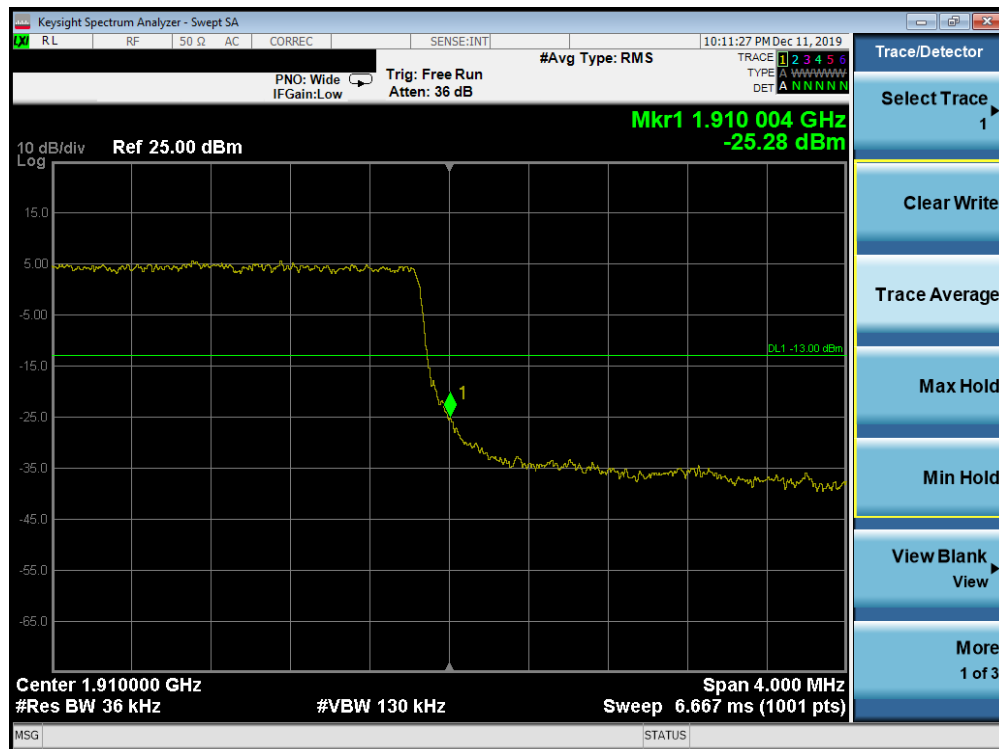
Plot 7-195. Upper Band Edge Plot (Band 2 - 3.0MHz QPSK - Full RB Configuration)
