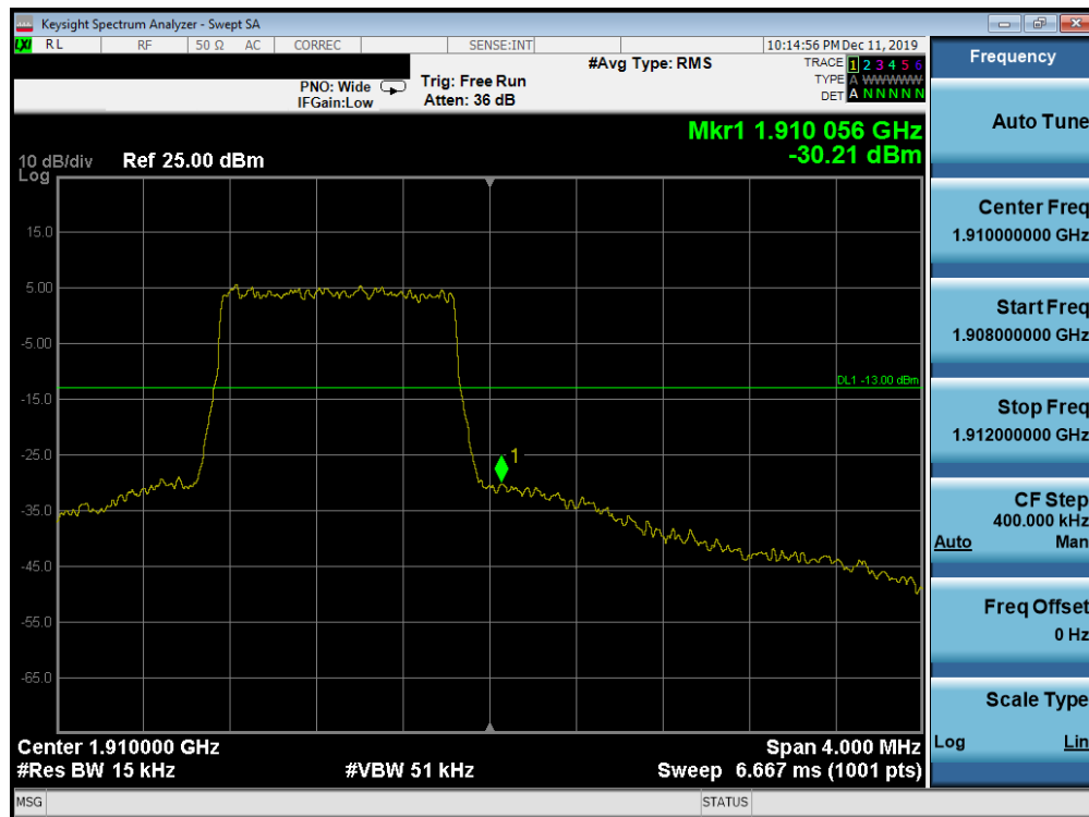
Plot 7-189. Upper Band Edge Plot (Band 2 - 1.4MHz QPSK - Full RB Configuration)
