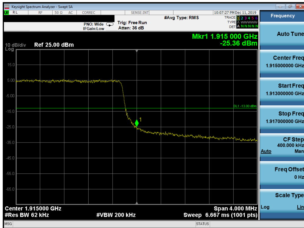
Plot 7-203. Upper Band Edge Plot (Band 25 - 5.0MHz QPSK - Full RB Configuration)
