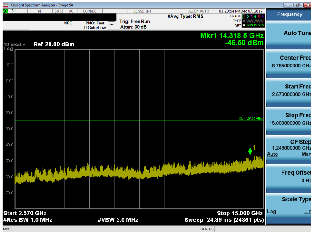
Plot 7-161. Conducted Spurious Plot (Band 7 - 20.0MHz QPSK - RB Size 1, RB Offset 0 - Mid Channel)
