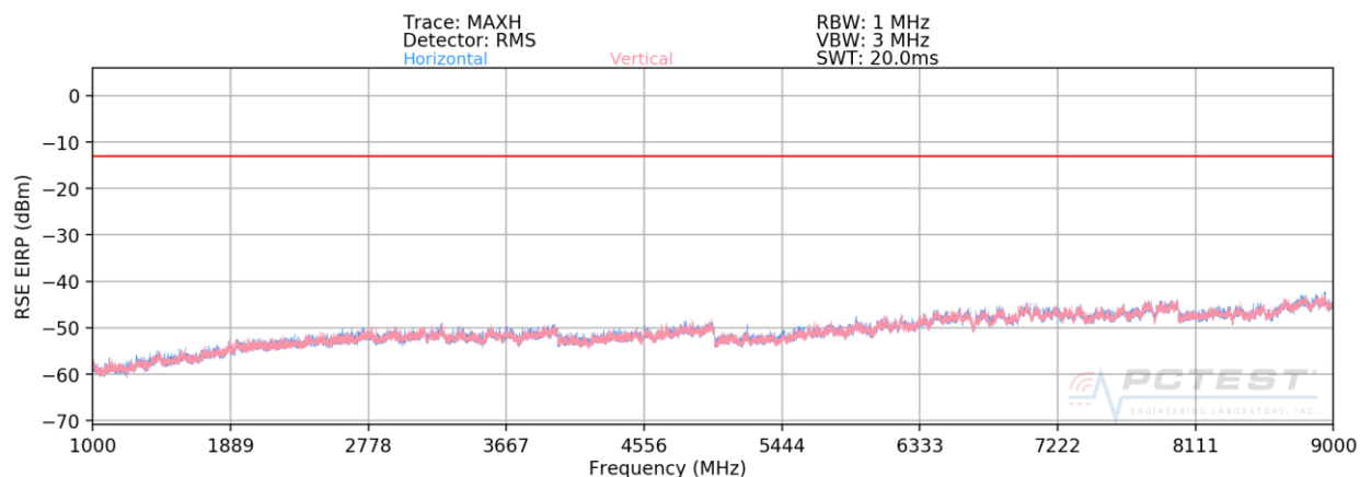
Plot 7-56. Radiated Spurious Plot (Band 26) – OPEN
