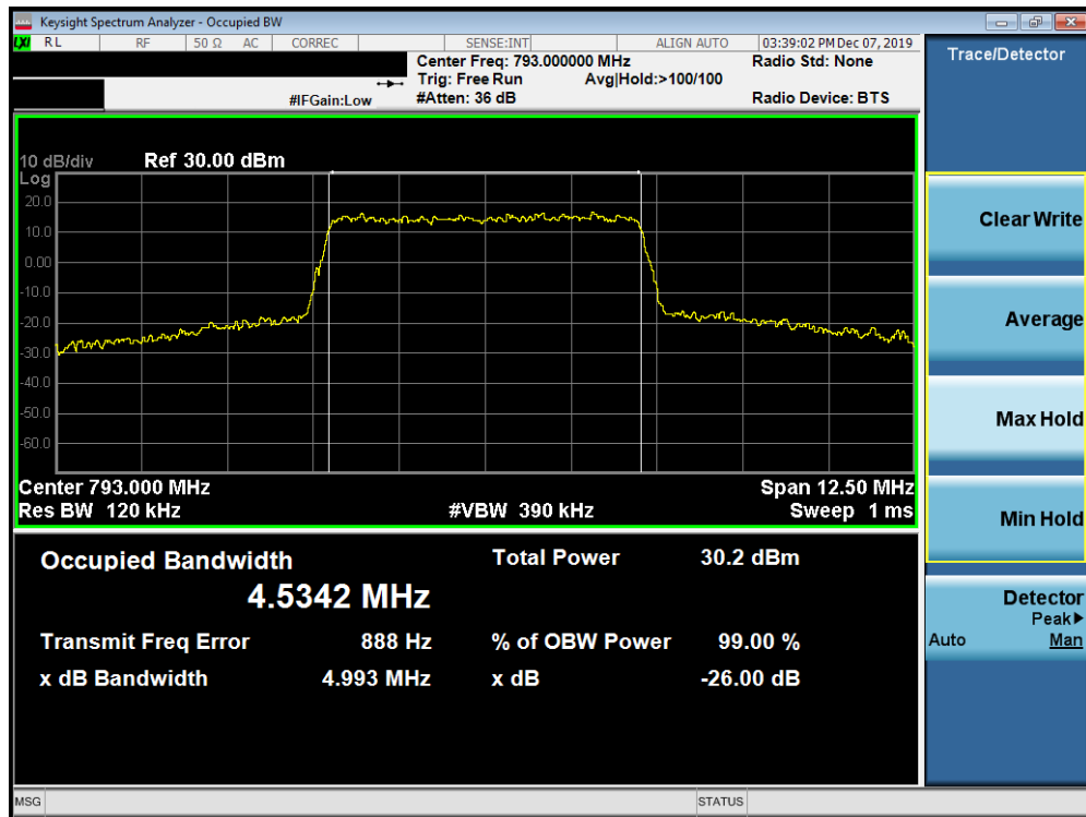
Plot 7-20. Occupied Bandwidth Plot (LTE Band 14 - 5MHz 64-QAM - Full RB Configuration)
