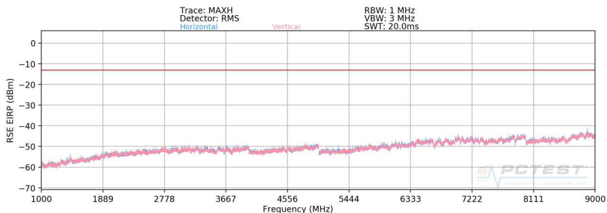
Plot 7-57. Radiated Spurious Plot (Band 26) – CLOSED
