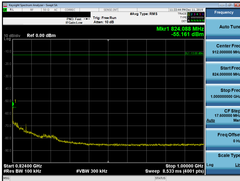
Plot 7-7. Conducted Spurious Plot (LTE Band 26 - 10MHz QPSK - RB Size 1, RB Offset 0 - Mid Channel)
