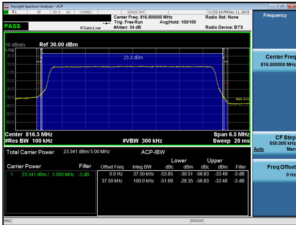
Plot 7-42. Channel Edge Plot (LTE Band 26 - 5MHz QPSK - Low Channel)
