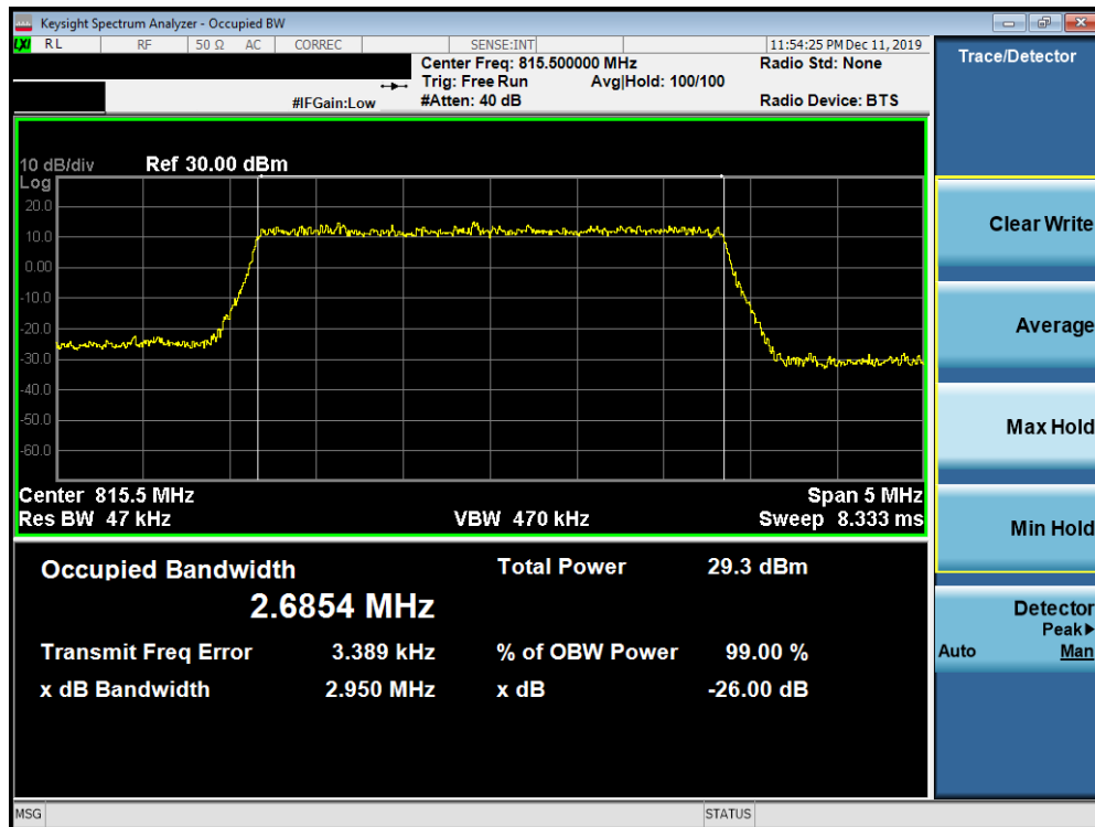
Plot 7-8. Occupied Bandwidth Plot (LTE Band 26 - 3MHz 64-QAM - Full RB Configuration)
