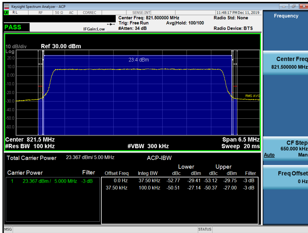
Plot 7-43. Channel Edge Plot (LTE Band 26 - 5MHz QPSK - High Channel)
