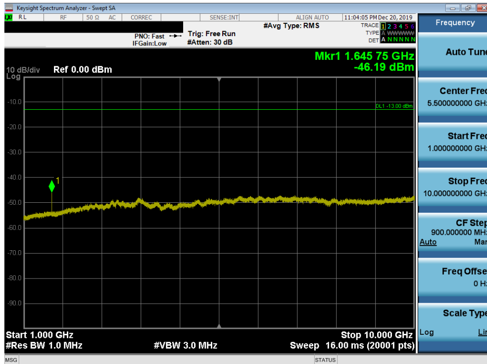
Plot 7-29. Conducted Spurious Plot (CDMA Ch. 684- High Channel)
