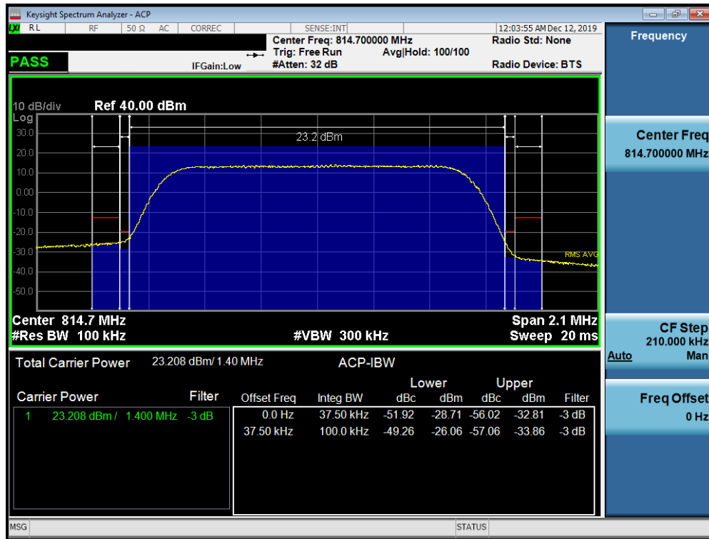
Plot 7-38. Channel Edge Plot (LTE Band 26 - 1.4MHz QPSK - Low Channel)
