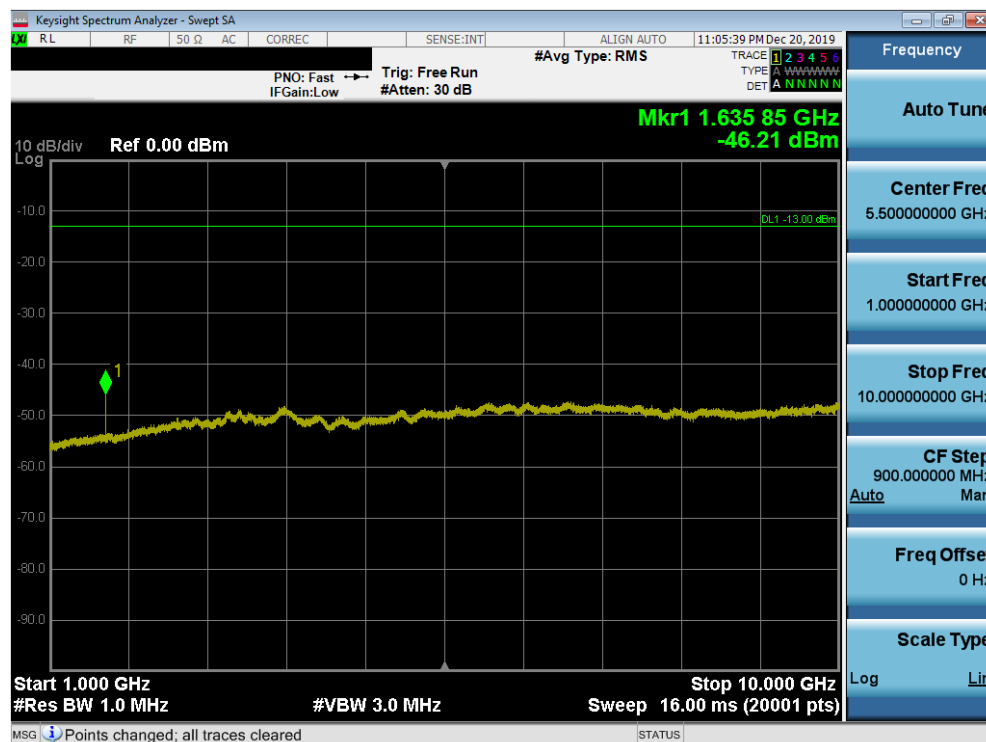
Plot 7-26. Conducted Spurious Plot (CDMA Ch. 476- Low Channel)
