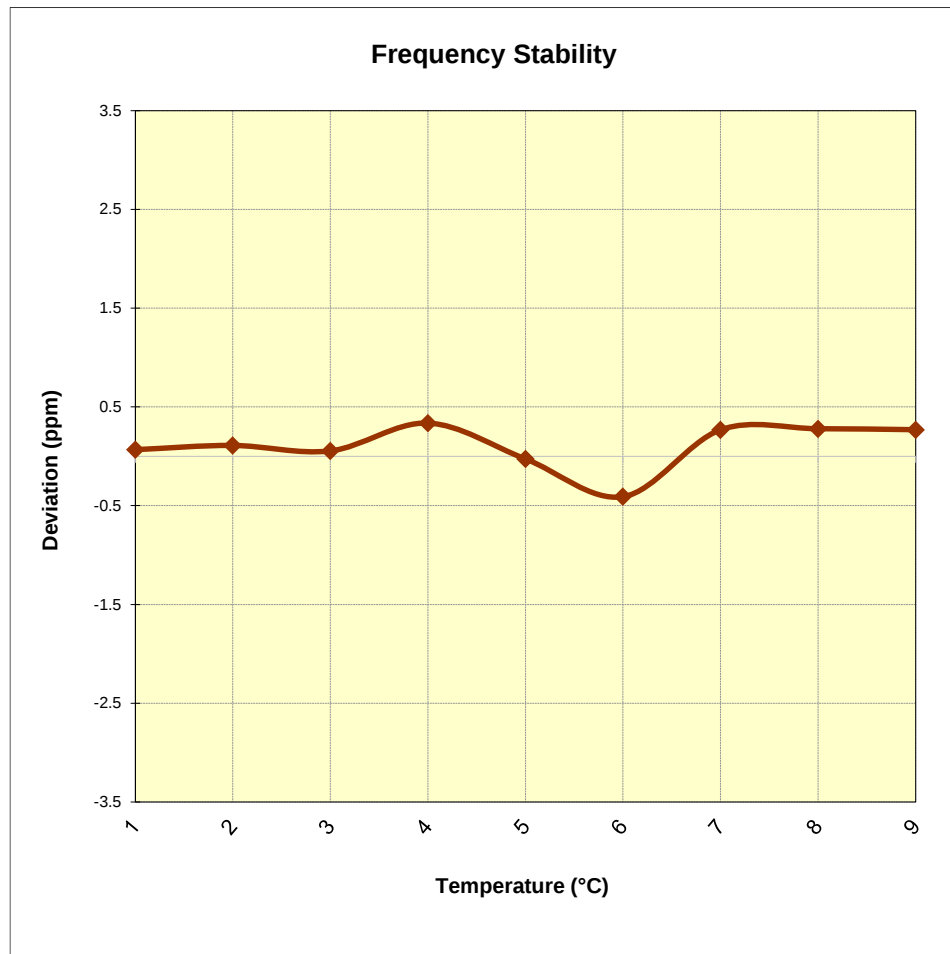
Figure 7-7. LTE Band 14 Frequency Stability Chart
