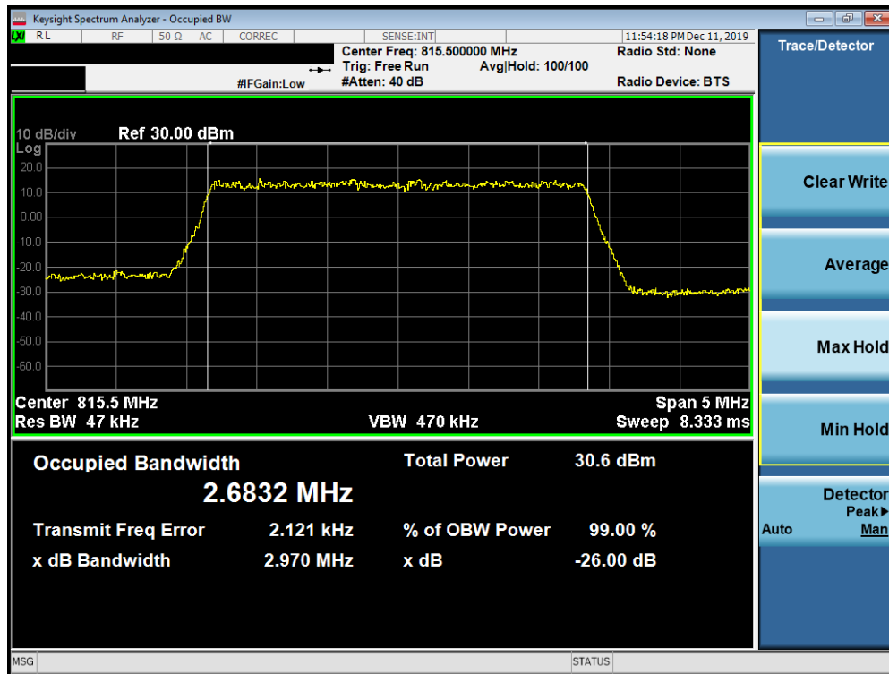
Plot 7-7. Occupied Bandwidth Plot (LTE Band 26 - 3MHz 16-QAM - Full RB Configuration)
