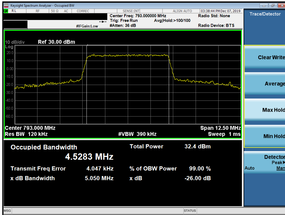
Plot 7-18. Occupied Bandwidth Plot (LTE Band 14 - 5MHz QPSK - Full RB Configuration)
