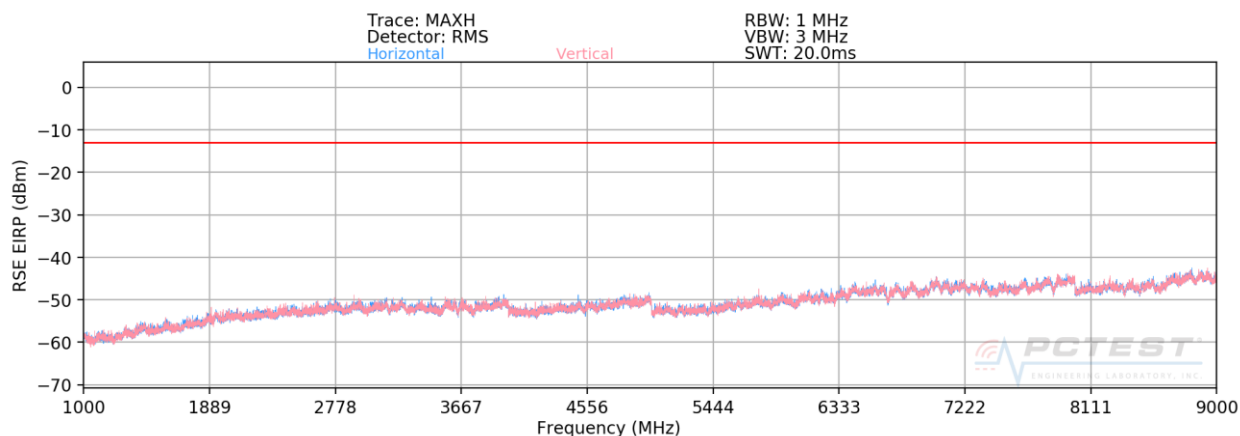
Plot 7-55. Radiated Spurious Plot (CDMA BC10) – CLOSED
