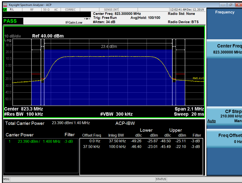
Plot 7-39. Channel Edge Plot (LTE Band 26 - 1.4MHz QPSK - High Channel)
