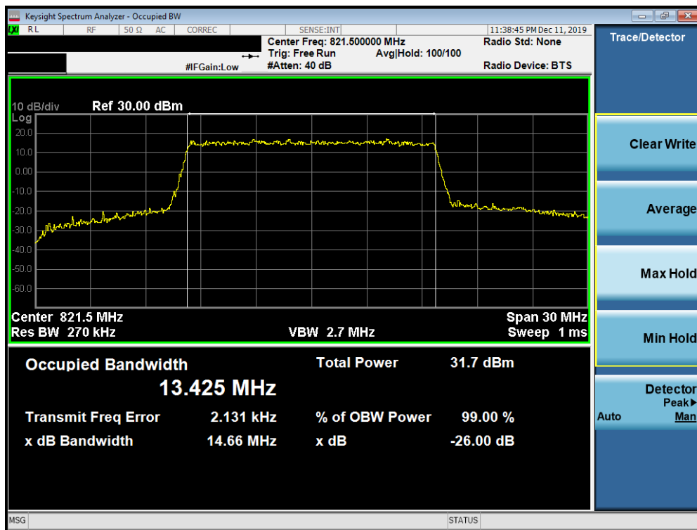
Plot 7-5. Occupied Bandwidth Plot (LTE Band 26 - 15MHz 16-QAM - Full RB Configuration)
