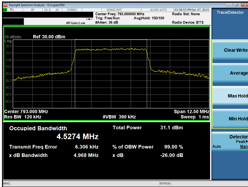
Plot 7-19. Occupied Bandwidth Plot (LTE Band 14 - 5MHz 16-QAM - Full RB Configuration)
