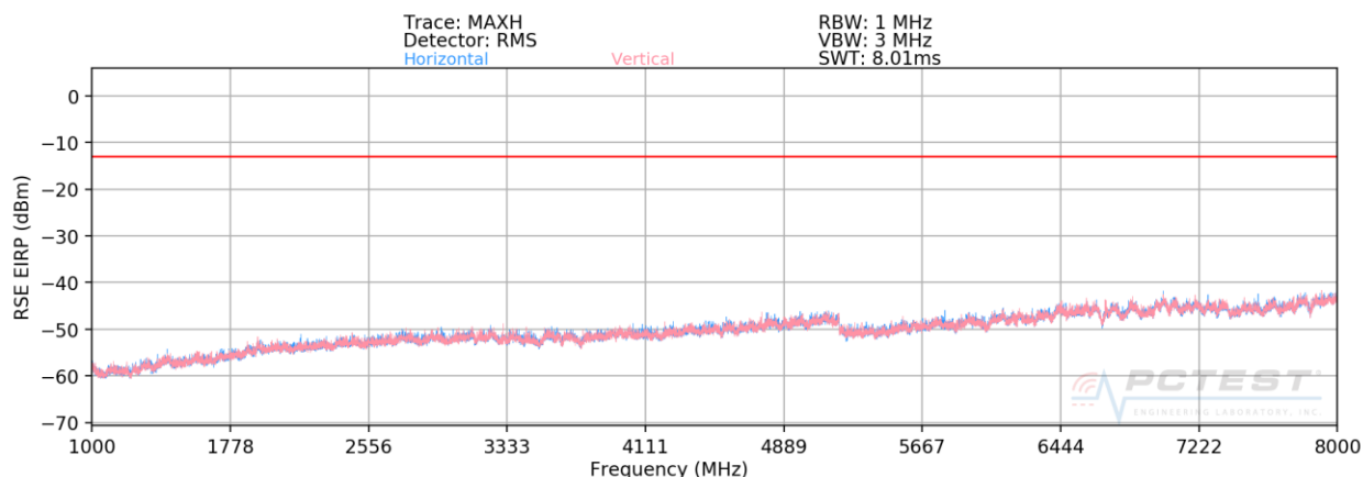
Plot 7-58. Radiated Spurious Plot (Band 14) – OPEN
