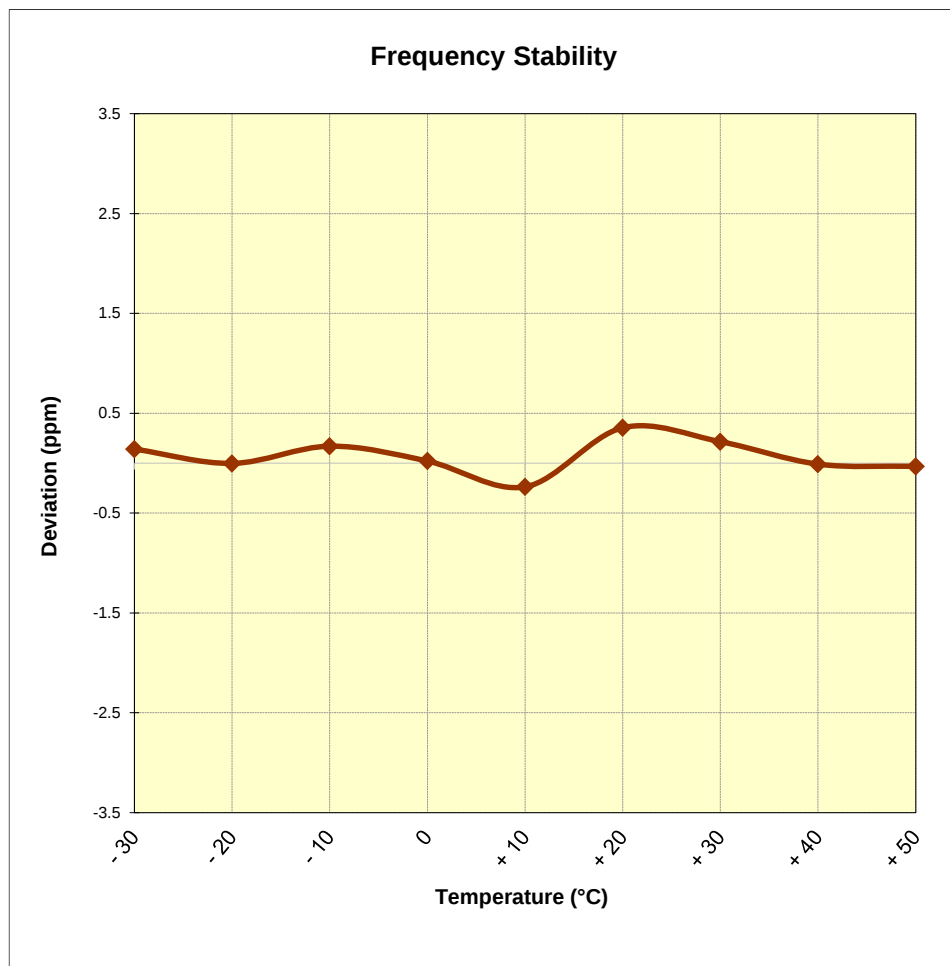
Figure 7-6. LTE Band 26 Frequency Stability Chart
