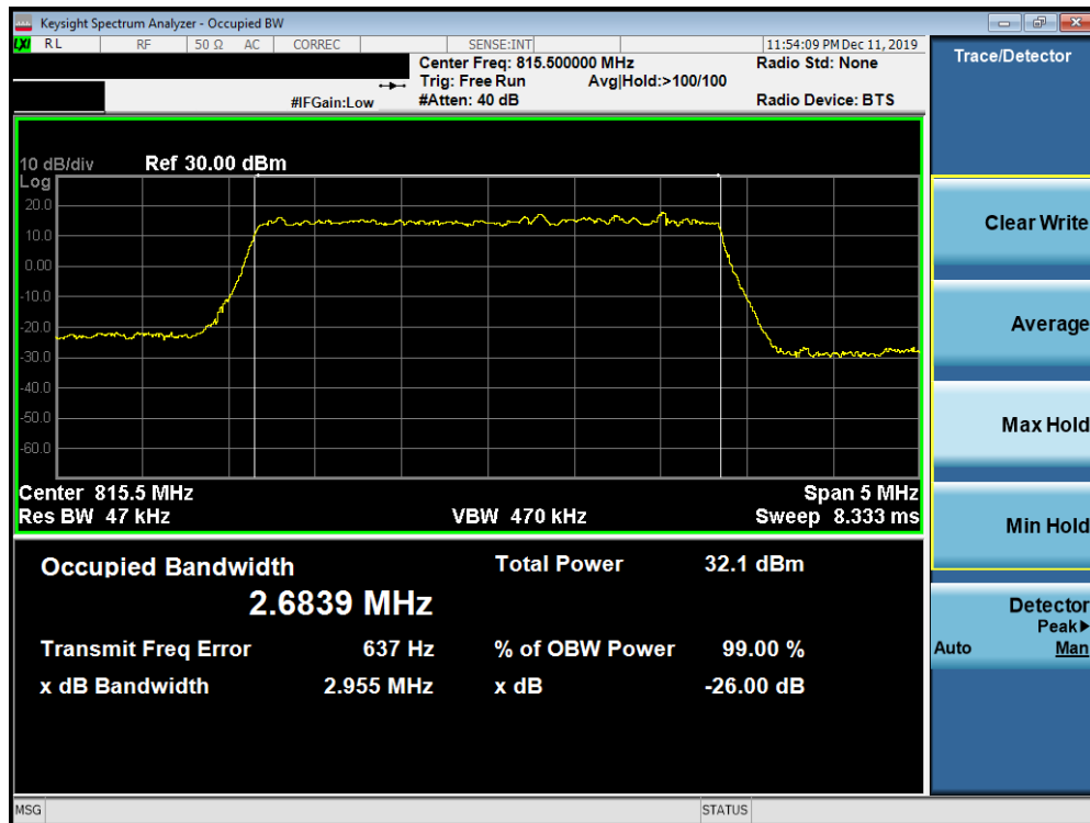
Plot 7-6. Occupied Bandwidth Plot (LTE Band 26 - 3MHz QPSK - Full RB Configuration)
