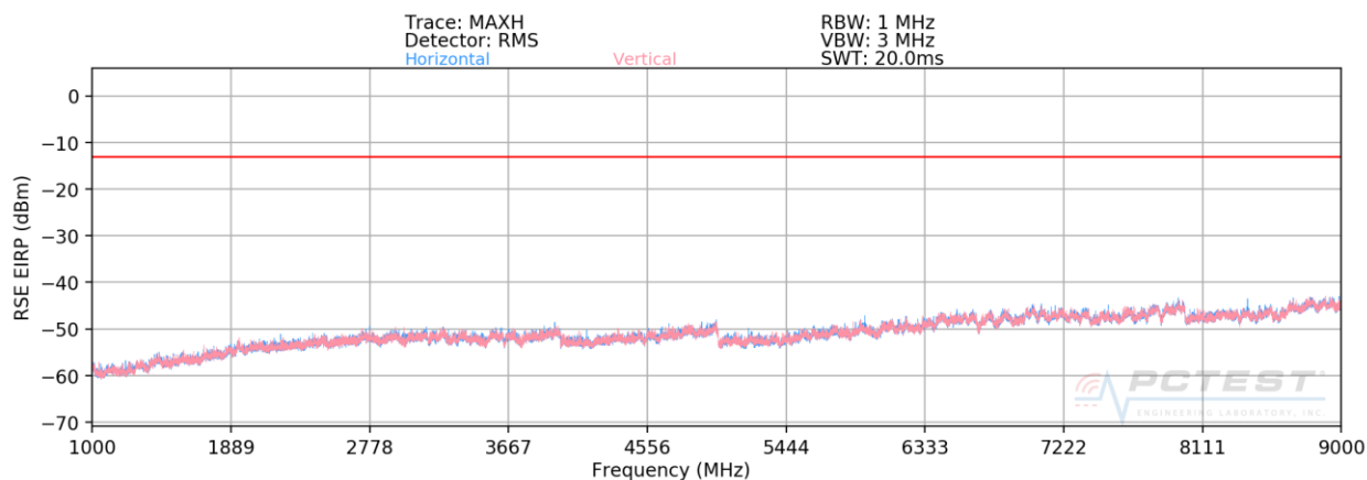
Plot 7-54. Radiated Spurious Plot (CDMA BC10) – OPEN
