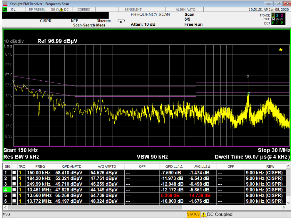
Plot 7-9. Line-Conducted Test Plot (L1) – OPEN
