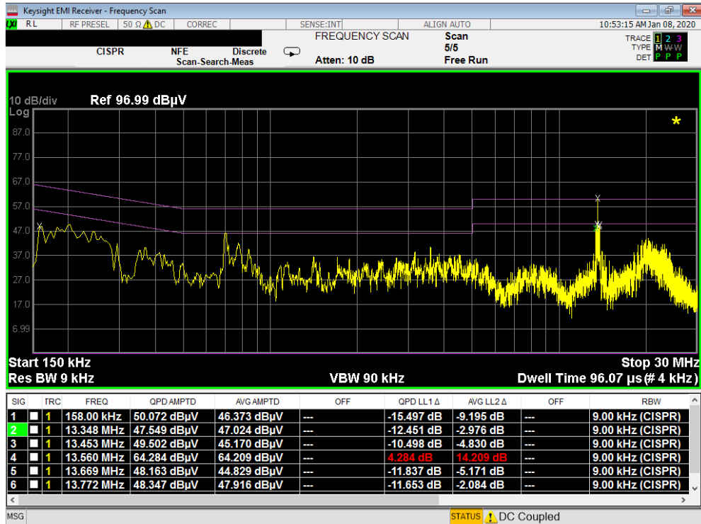
Plot 7-10. Line-Conducted Test Plot (N) – OPEN
