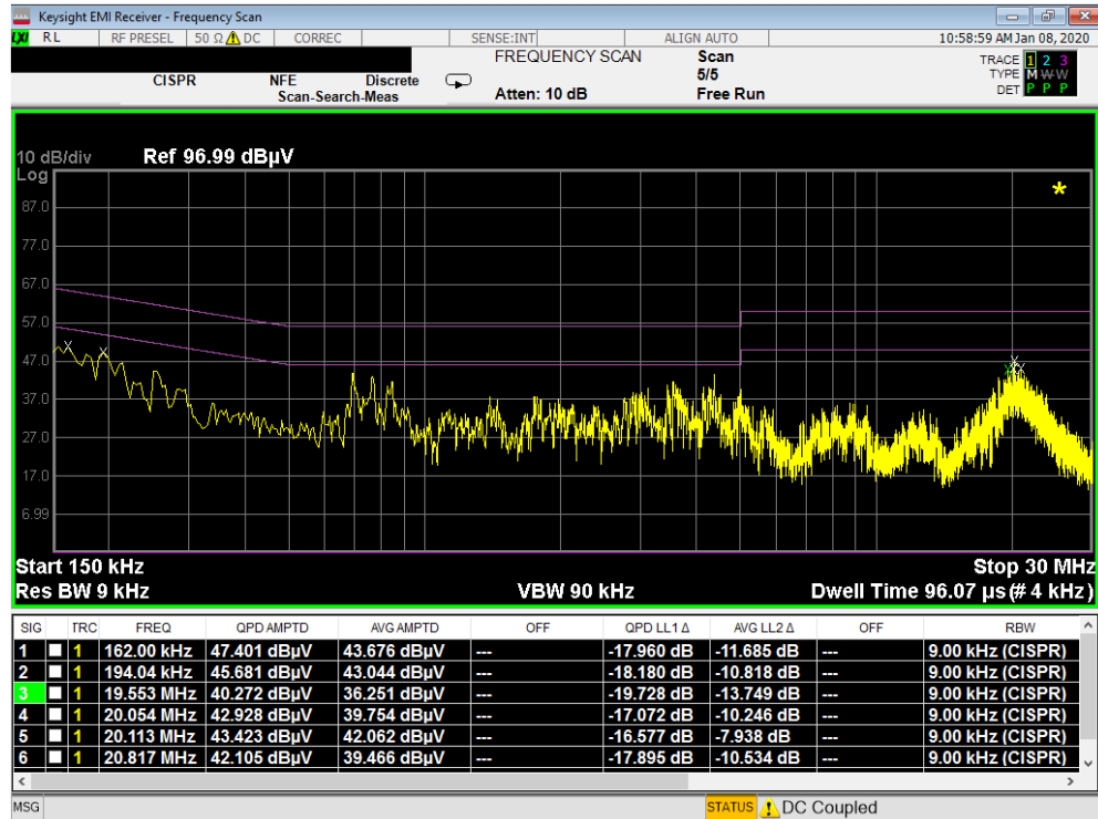
Plot 7-13. Line-Conducted Test Plot Terminated at 50 Ohms(L1) – OPEN
