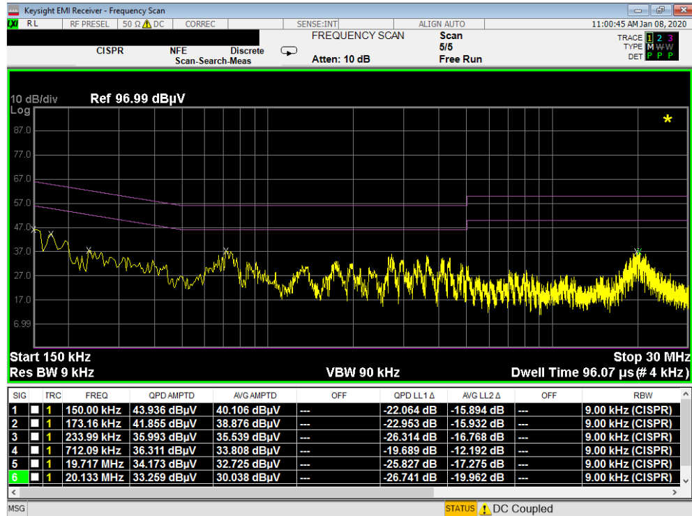
Plot 7-15. Line-Conducted Test Plot Terminated at 50 Ohms(L1) – CLOSED
