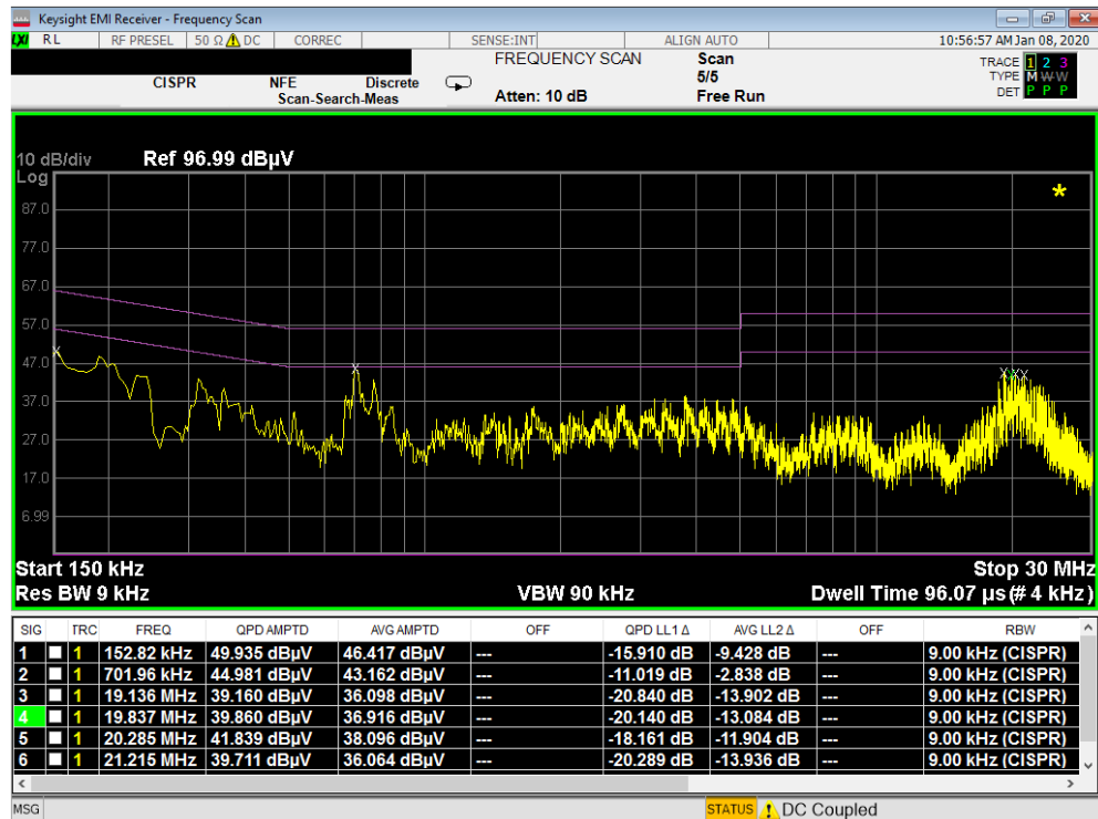
Plot 7-14. Line-Conducted Test Plot Terminated at 50 Ohms (N) – OPEN
