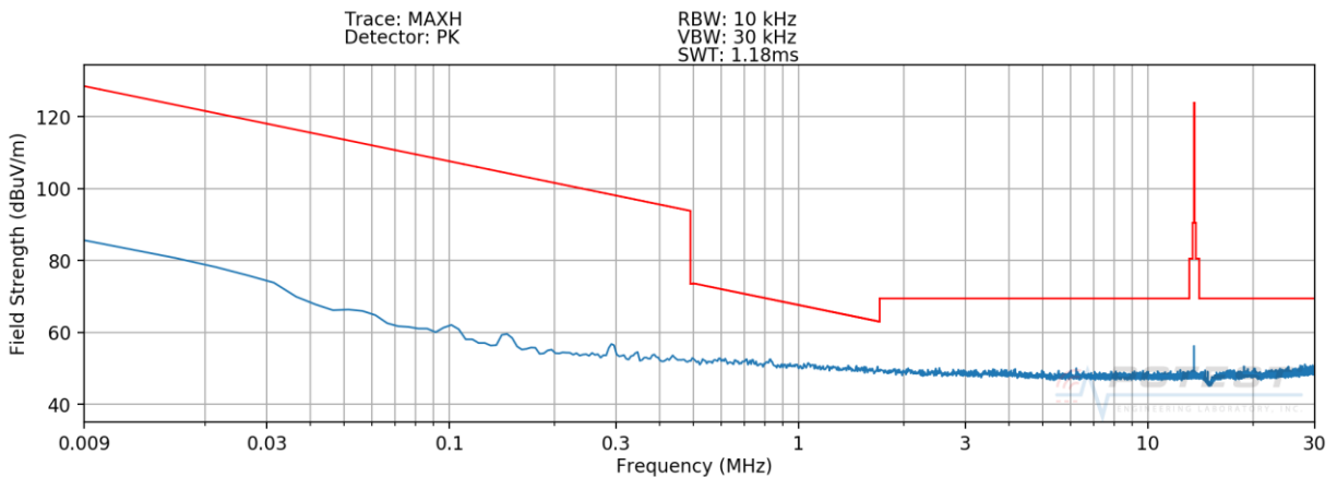
Plot 7-3. Radiated Spurious Plot 9kHz – 30MHz (Pol. Y - CLOSED)
