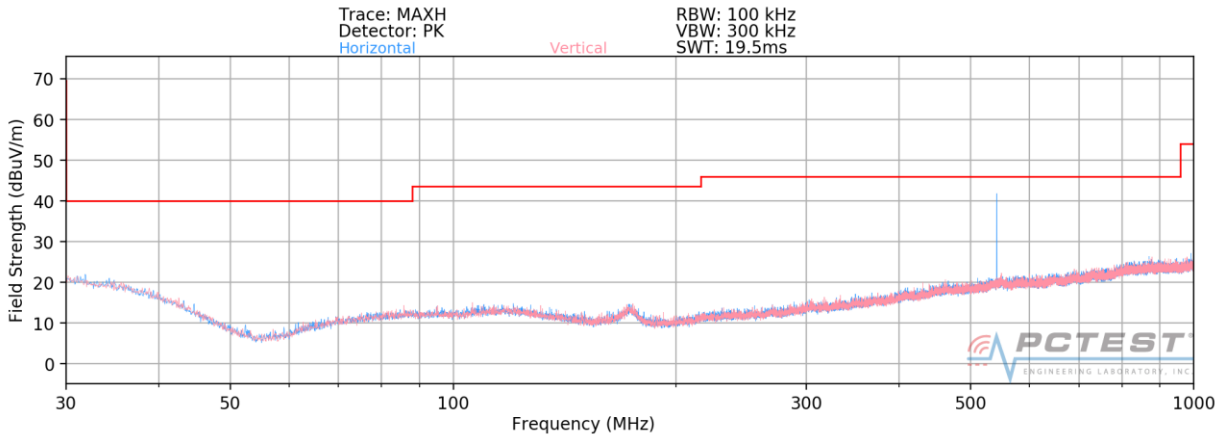
Plot 7-7. Radiated Spurious Plot 30MHz – 1GHz – OPEN
