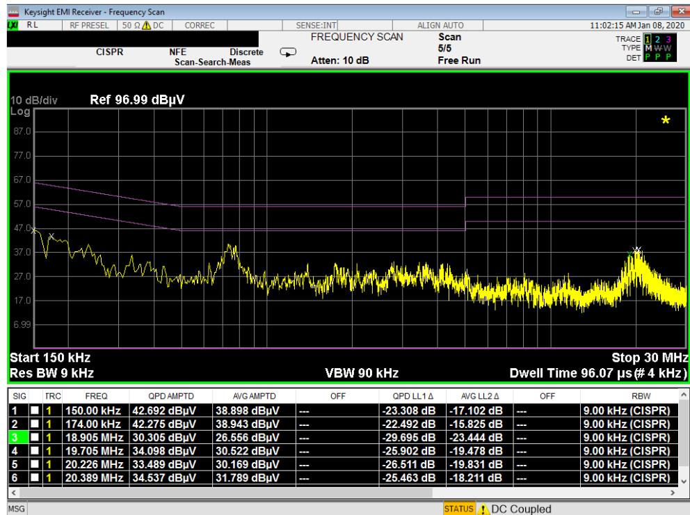
Plot 7-16. Line-Conducted Test Plot Terminated at 50 Ohms (N) – CLOSED
