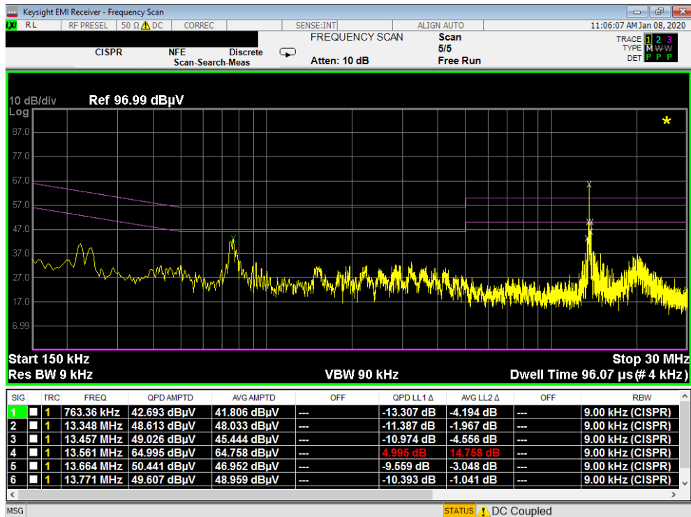
Plot 7-12. Line-Conducted Test Plot (N) – CLOSED
