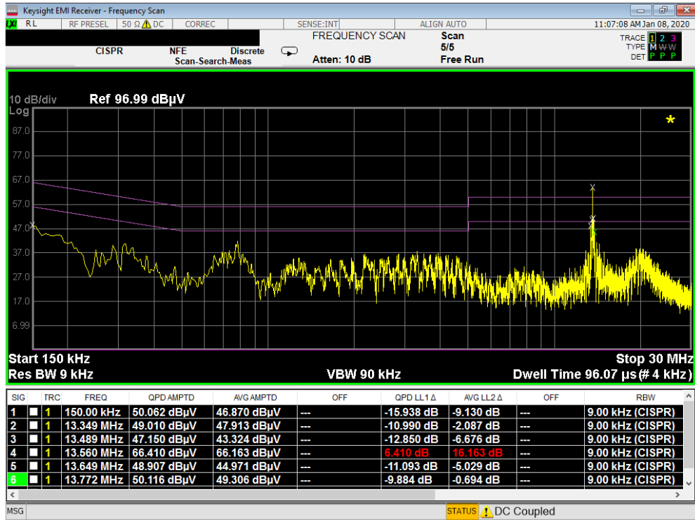
Plot 7-11. Line-Conducted Test Plot (L1) – CLOSED
