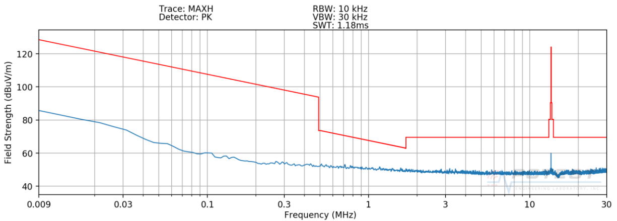
Plot 7-2. Radiated Spurious Plot 9kHz – 30MHz (Pol. X - OPEN)
