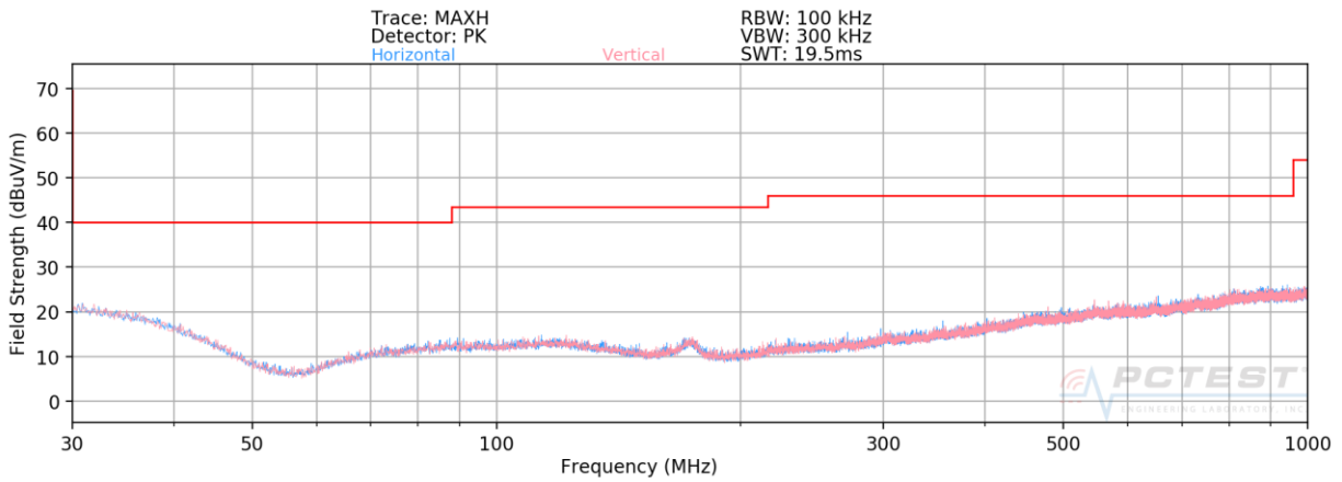
Plot 7-8. Radiated Spurious Plot 30MHz – 1GHz – CLOSED
