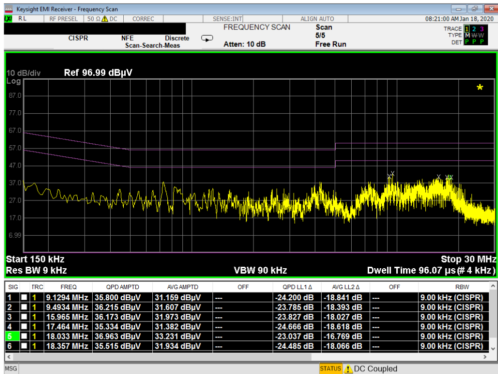
Plot 7-31. Line Conducted Plot (L1 - Closed)
