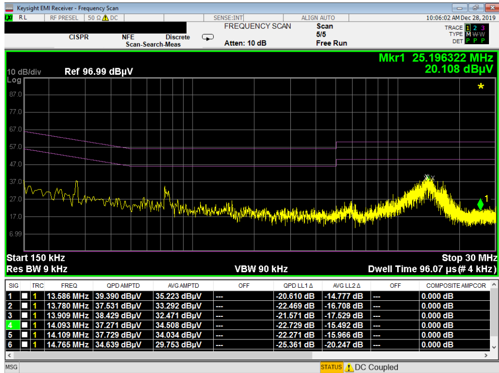
Plot 7-29. Line Conducted Plot (L1 - Open)
