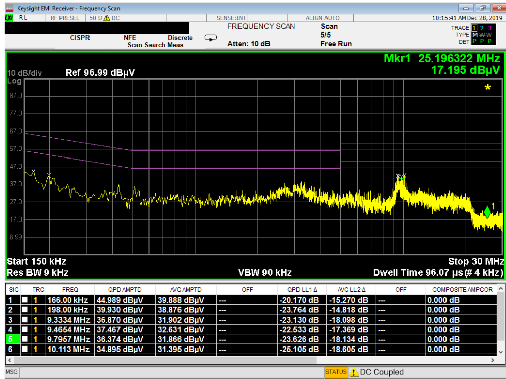
Plot 7-33. Line Conducted Plot (L1 - Open)
