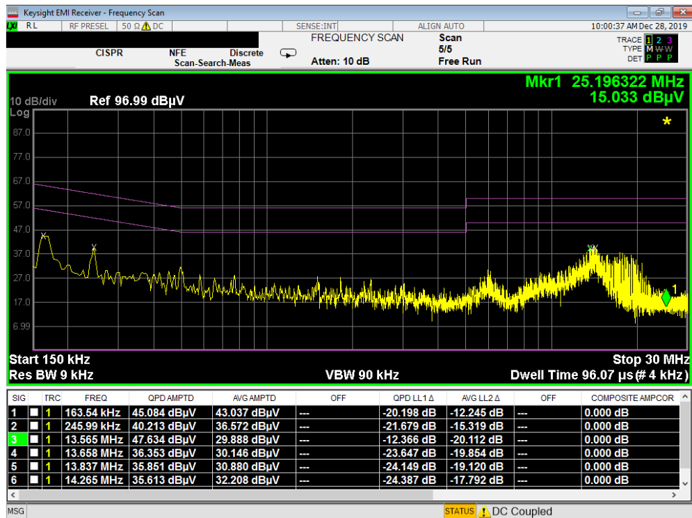
Plot 7-20. Line Conducted Plot (N - Open)
