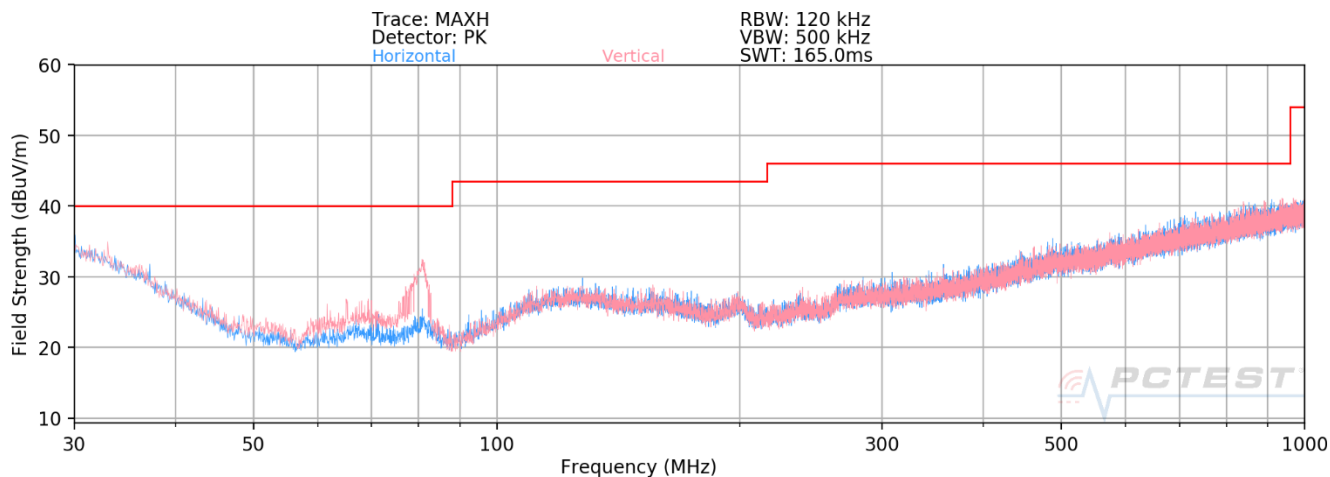
Plot 7-2. Radiated Spurious Plot below 1GHz [Radiated Test Config. 1 – Closed]
