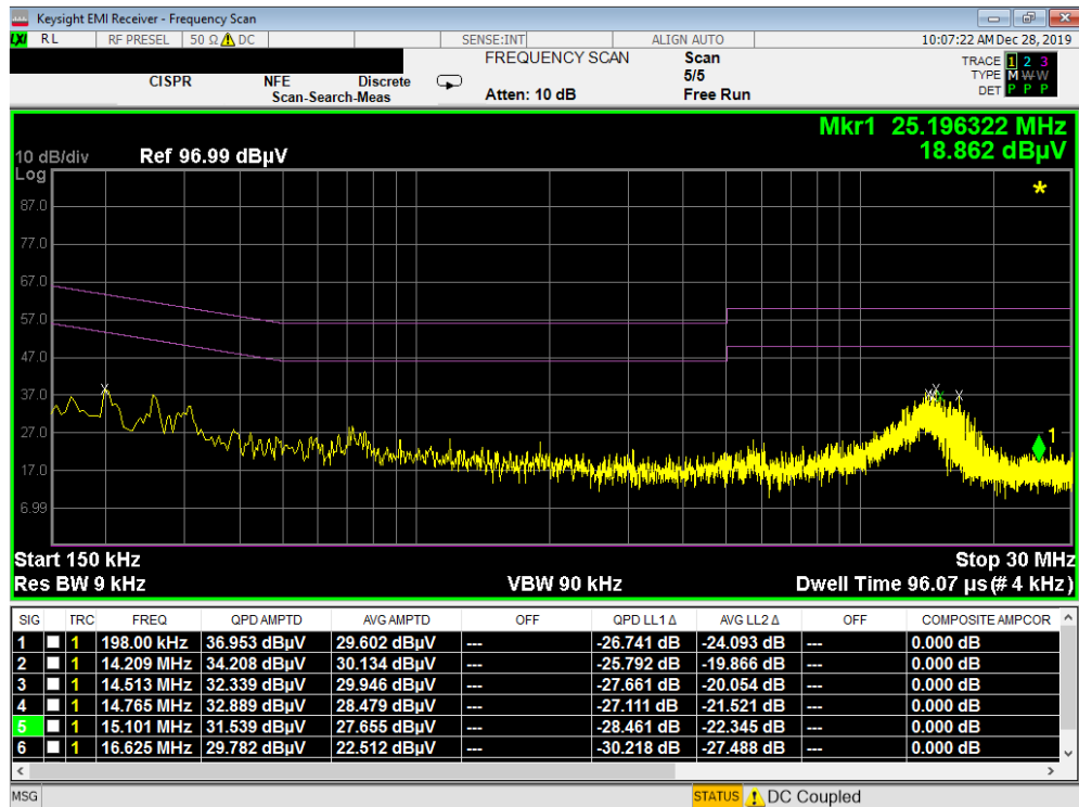
Plot 7-30. Line Conducted Plot (N - Open)
