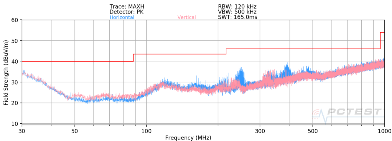
Plot 7-16. Radiated Spurious Plot below 1GHz [Radiated Test Config. 5 - Closed]
