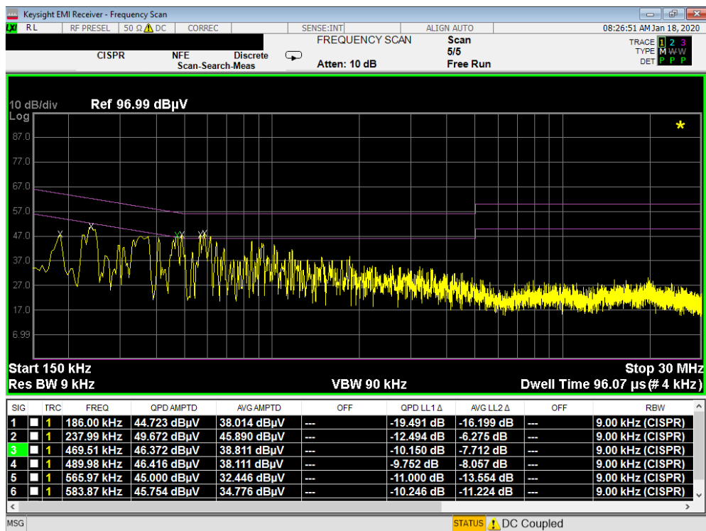
Plot 7-36. Line Conducted Plot (N - Closed)
