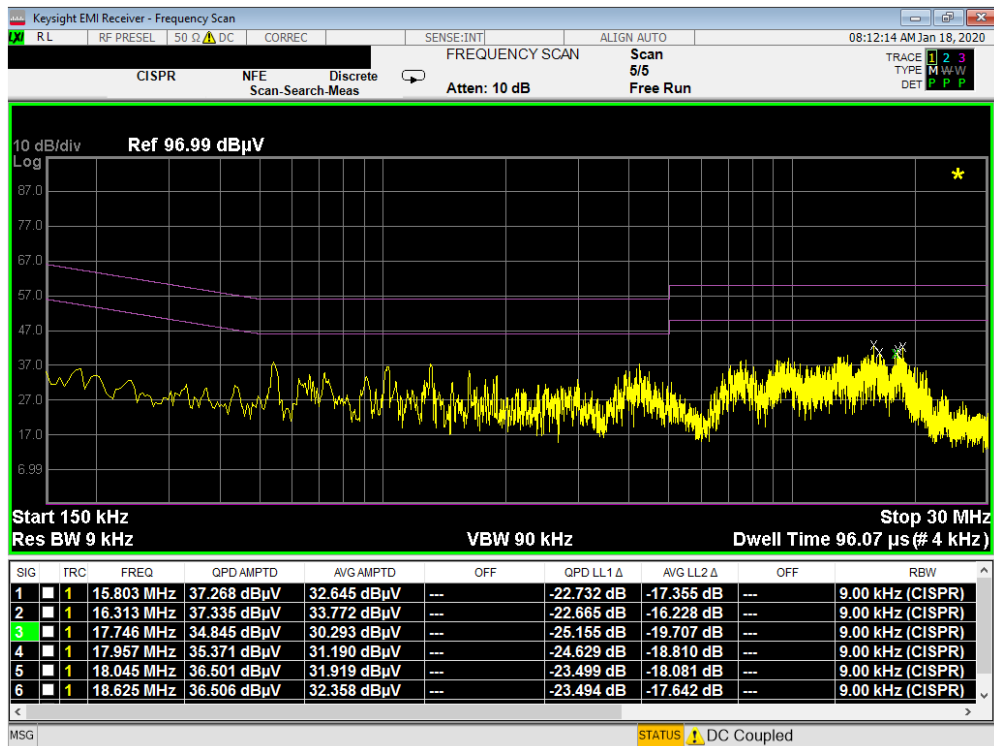
Plot 7-27. Line Conducted Plot (L1 - Closed)
