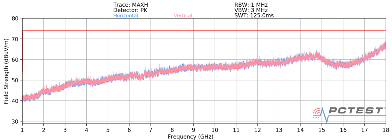
Plot 7-17. Radiated Spurious Plot above 1GHz [Radiated Test Config. 5 - Open]
