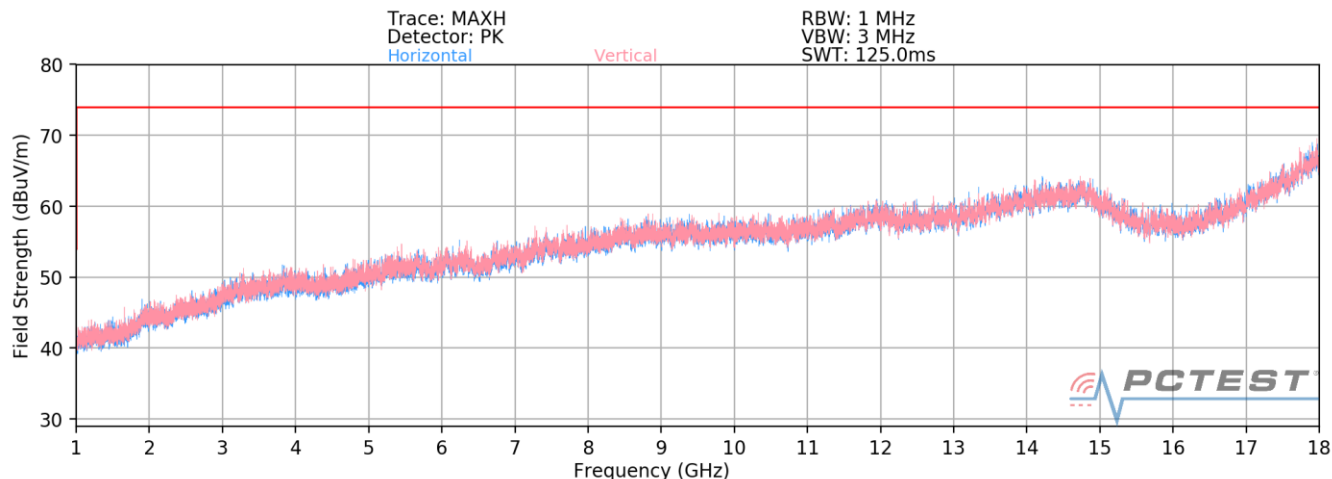
Plot 7-13. Radiated Spurious Plot above 1GHz [Radiated Test Config. 4 - Open]
