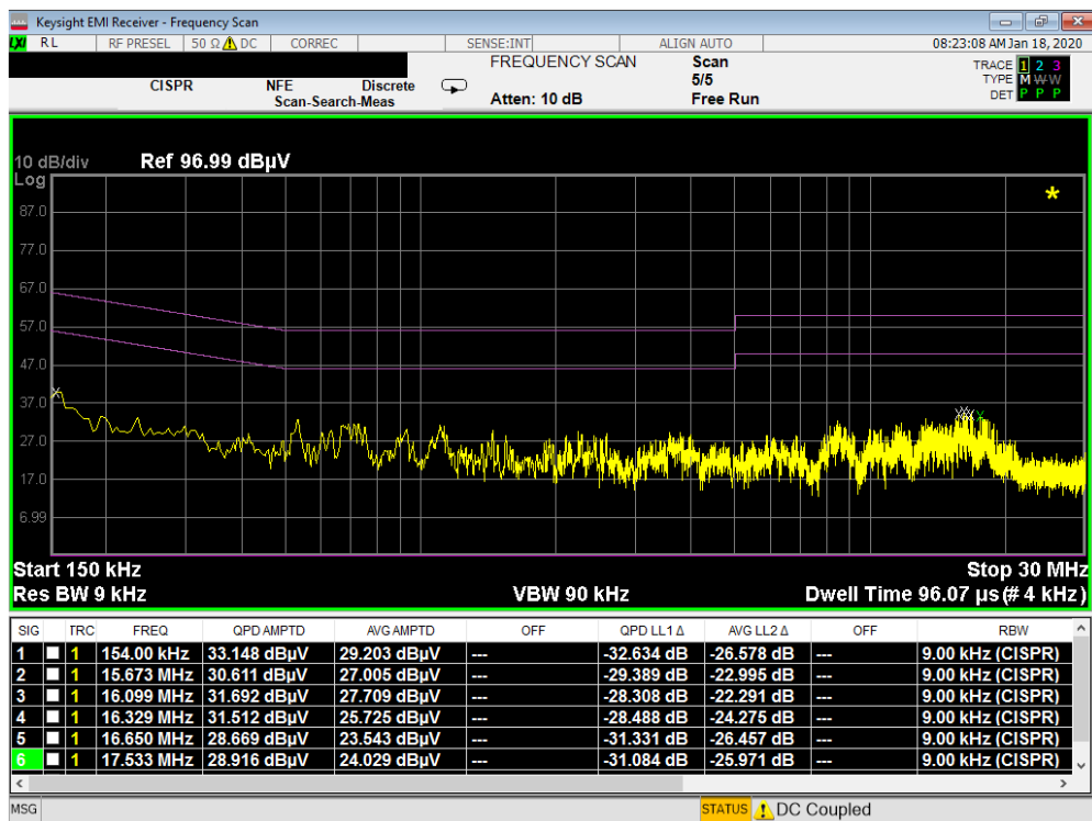
Plot 7-32. Line Conducted Plot (N - Closed)
