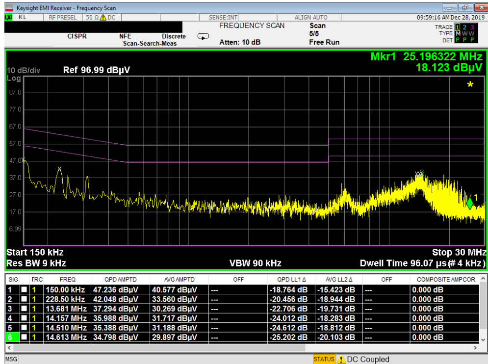
Plot 7-24. Line Conducted Plot (N - Open)
