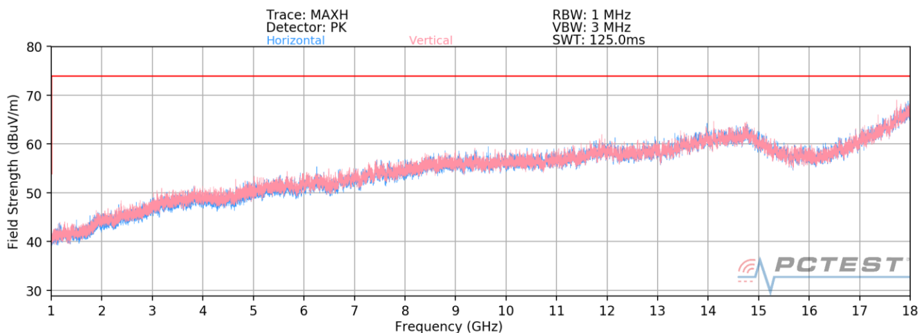
Plot 7-10. Radiated Spurious Plot above 1GHz [Radiated Test Config. 3 - Open]
