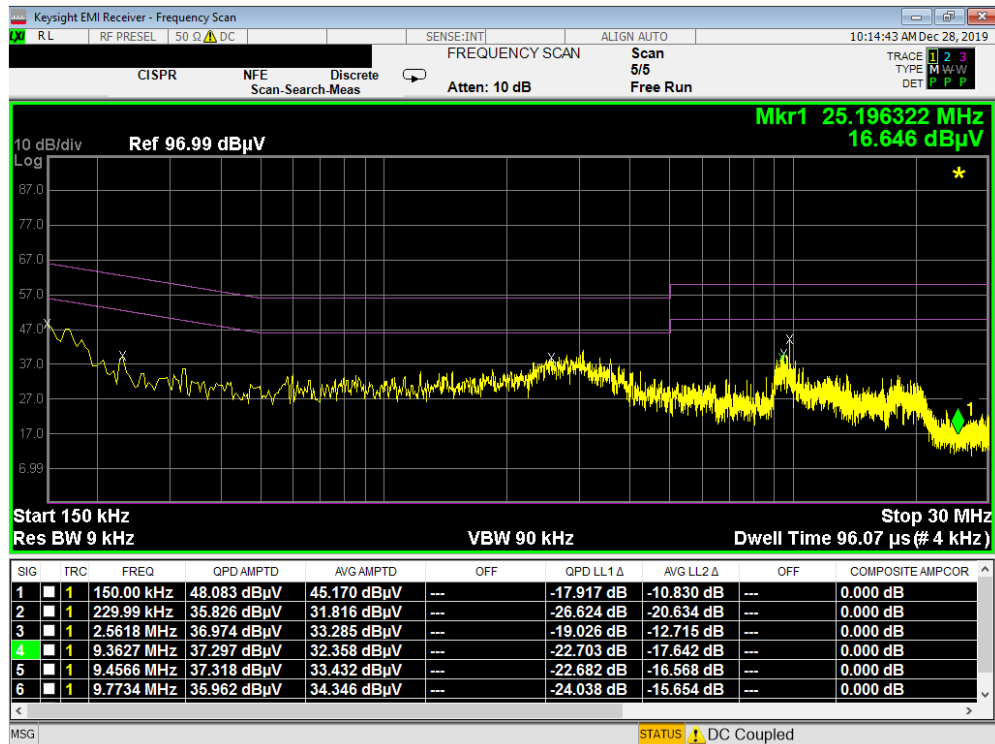
Plot 7-34. Line Conducted Plot (N - Open)
