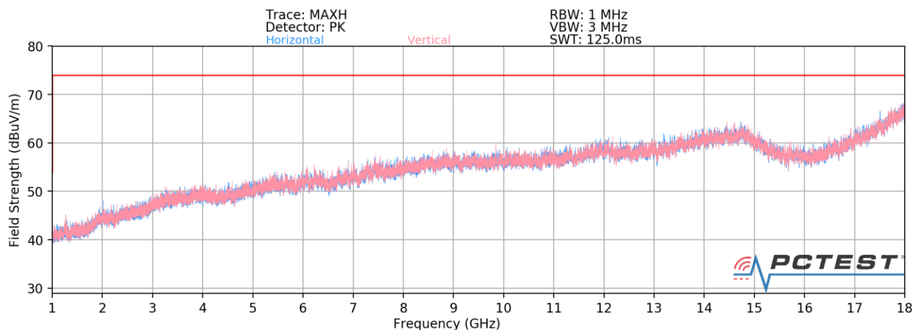
Plot 7-18. Radiated Spurious Plot above 1GHz [Radiated Test Config. 5 - Closed]
