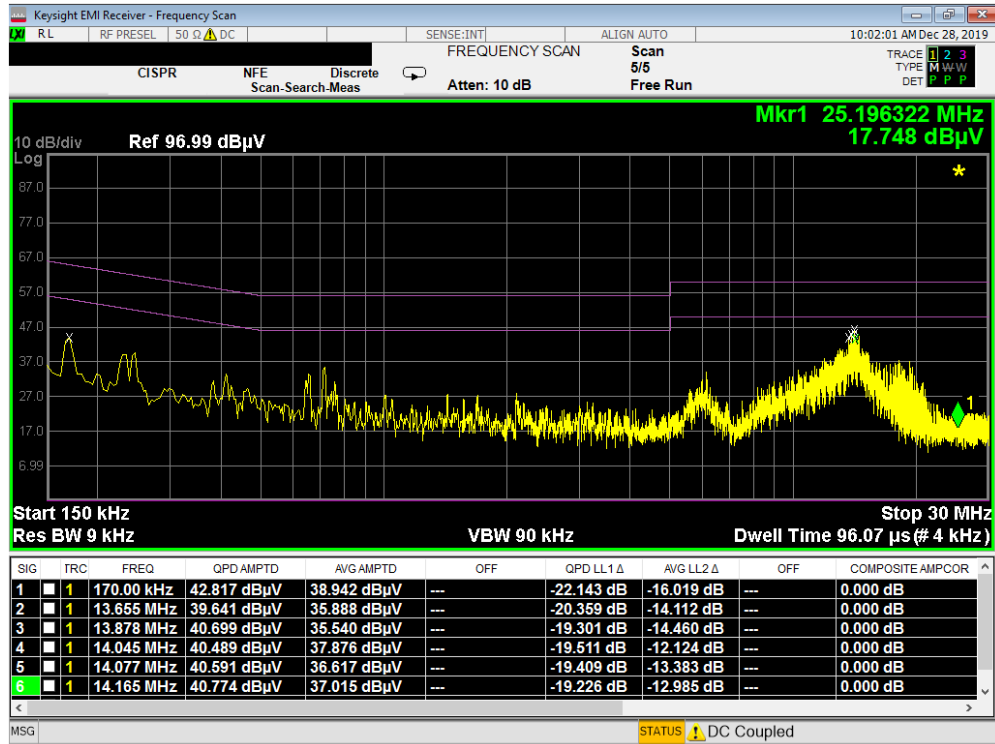
Plot 7-19. Line Conducted Plot (L1 - Open)
