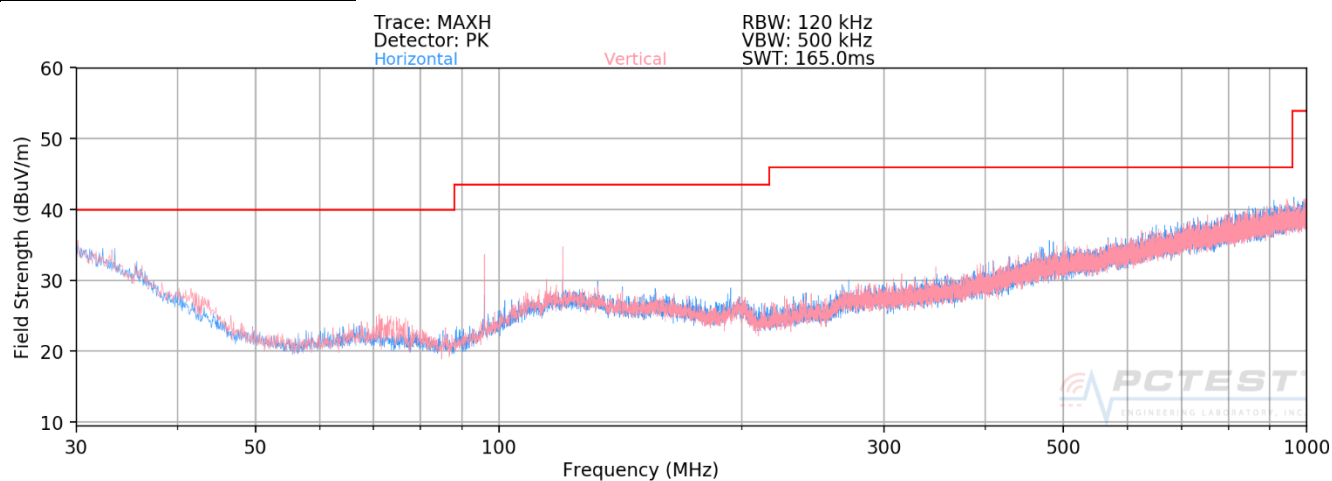
Plot 7-11. Radiated Spurious Plot below 1GHz [Radiated Test Config. 4 - Open]
