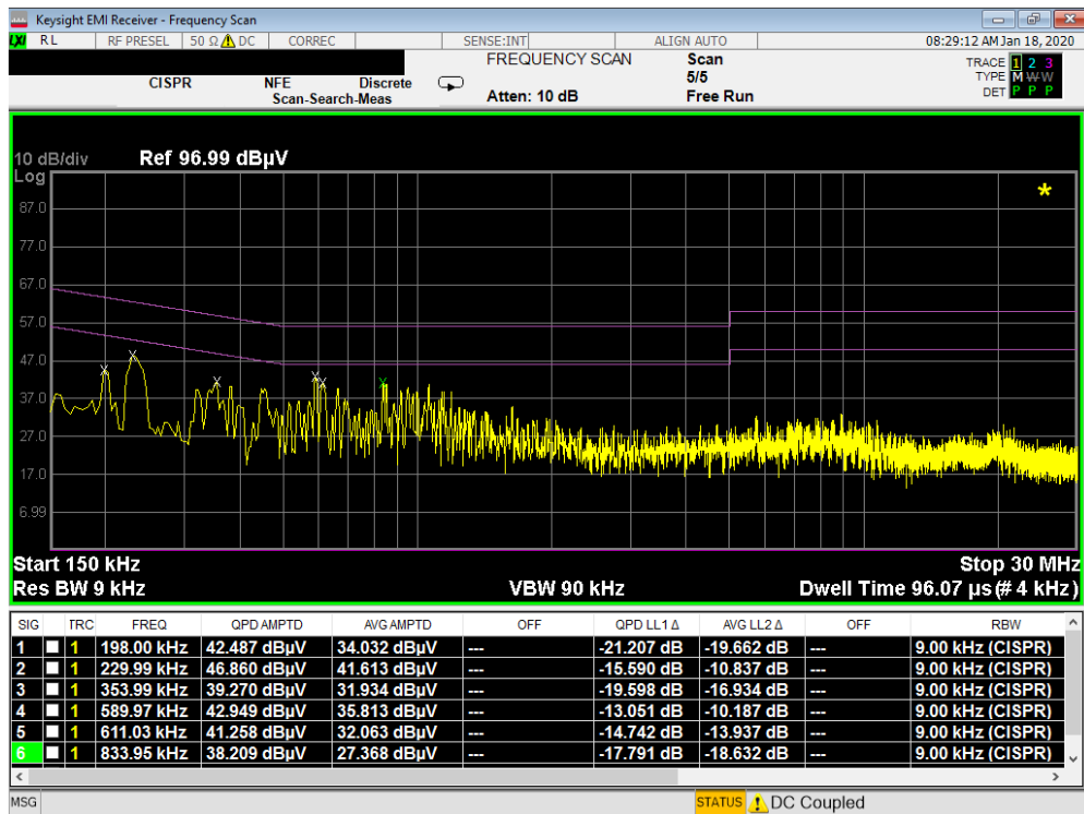
Plot 7-35. Line Conducted Plot (L1 - Closed)
