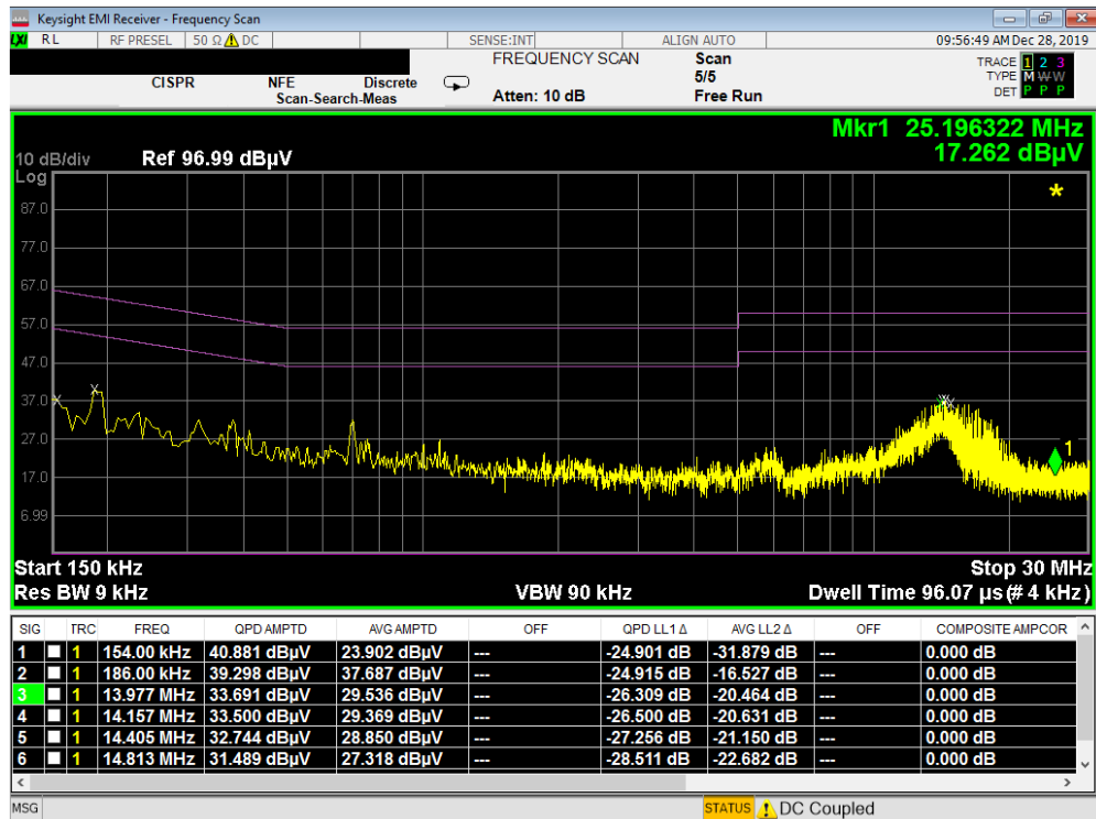
Plot 7-26. Line Conducted Plot (N - Open)
