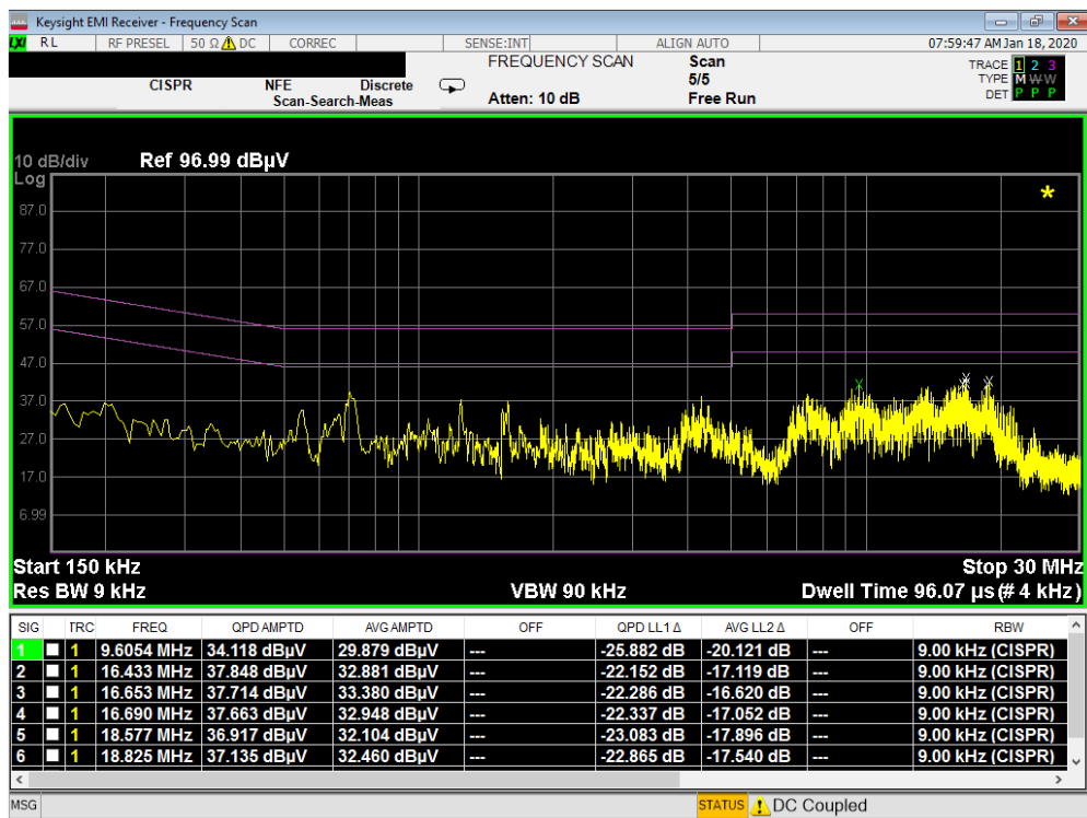
Plot 7-22. Line Conducted Plot (N - Closed)
