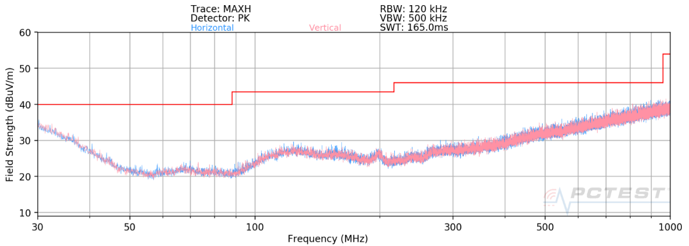
Plot 7-6. Radiated Spurious Plot below 1GHz [Radiated Test Config. 2 – Closed]
