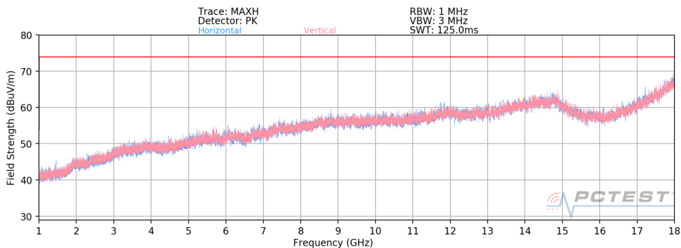
Plot 7-7. Radiated Spurious Plot above 1GHz [Radiated Test Config. 2 - Open]
