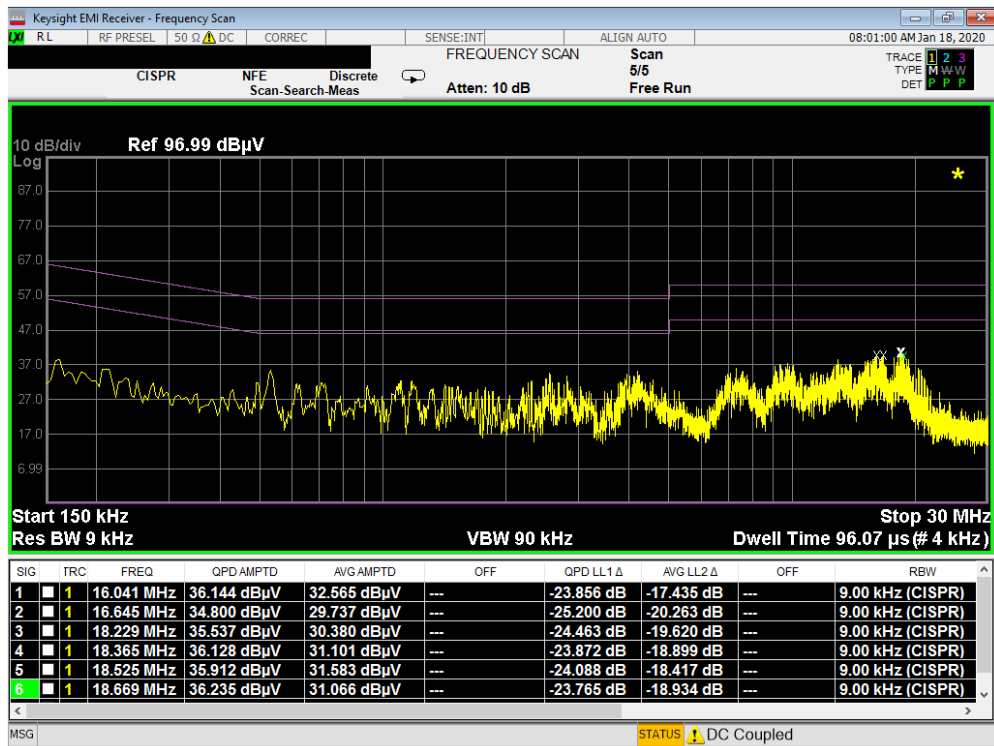
Plot 7-21. Line Conducted Plot (L1 – Closed)
