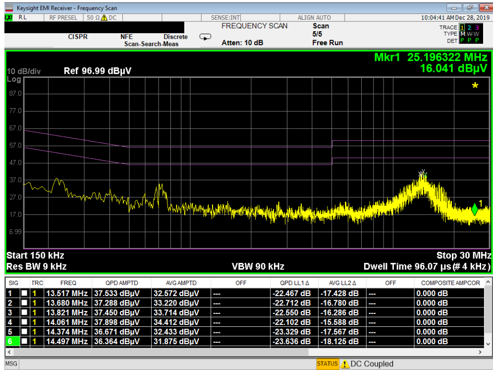
Plot 7-25. Line Conducted Plot (L1 - Open)
