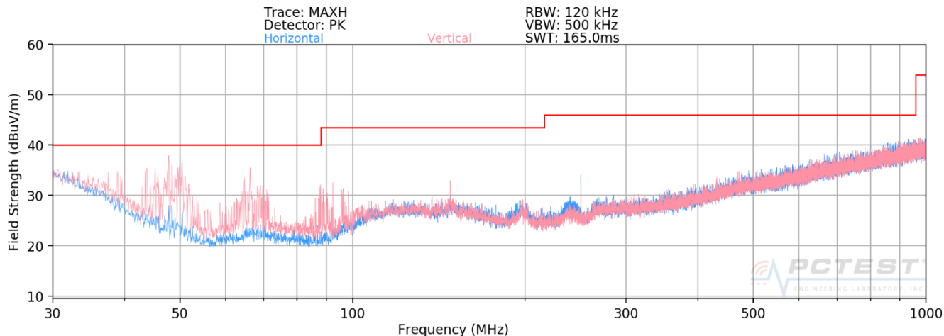
Plot 7-9. Radiated Spurious Plot below 1GHz [Radiated Test Config. 3 - Open]
