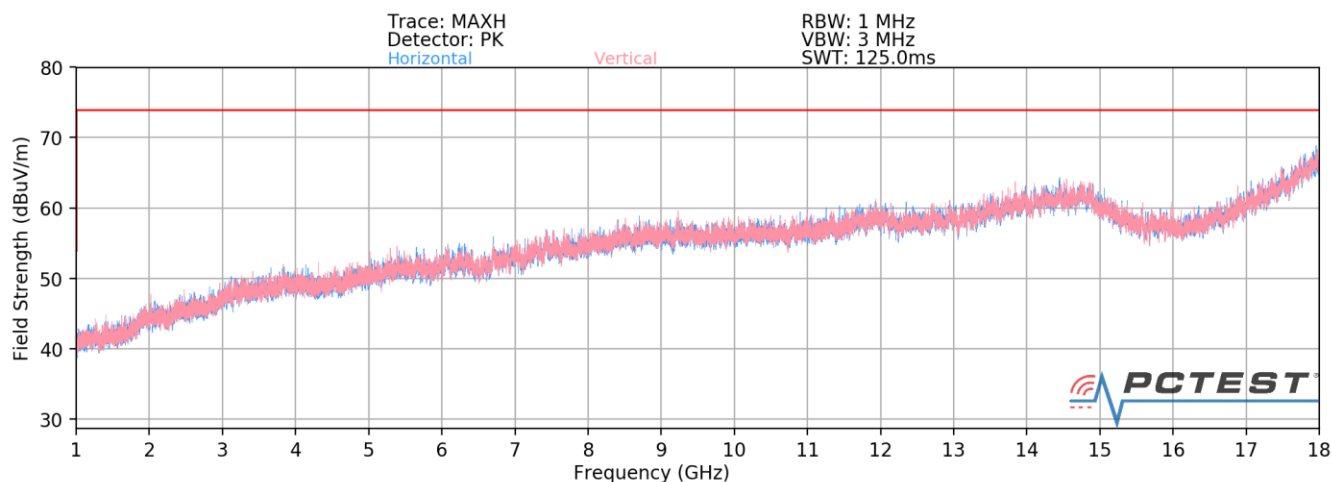
Plot 7-14. Radiated Spurious Plot above 1GHz [Radiated Test Config. 4 - Closed]
