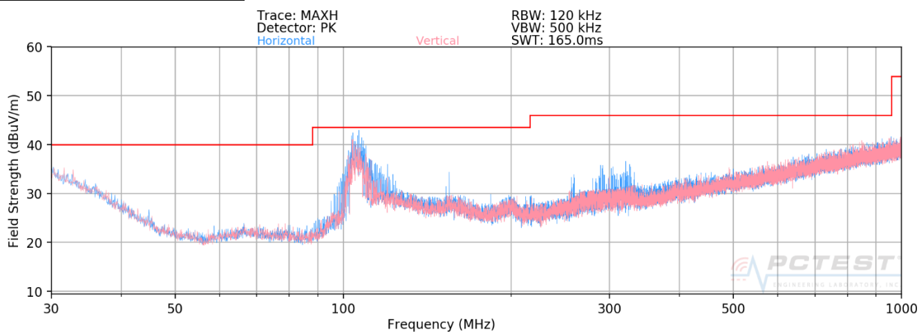
Plot 7-15. Radiated Spurious Plot below 1GHz [Radiated Test Config. 5 - Open]
