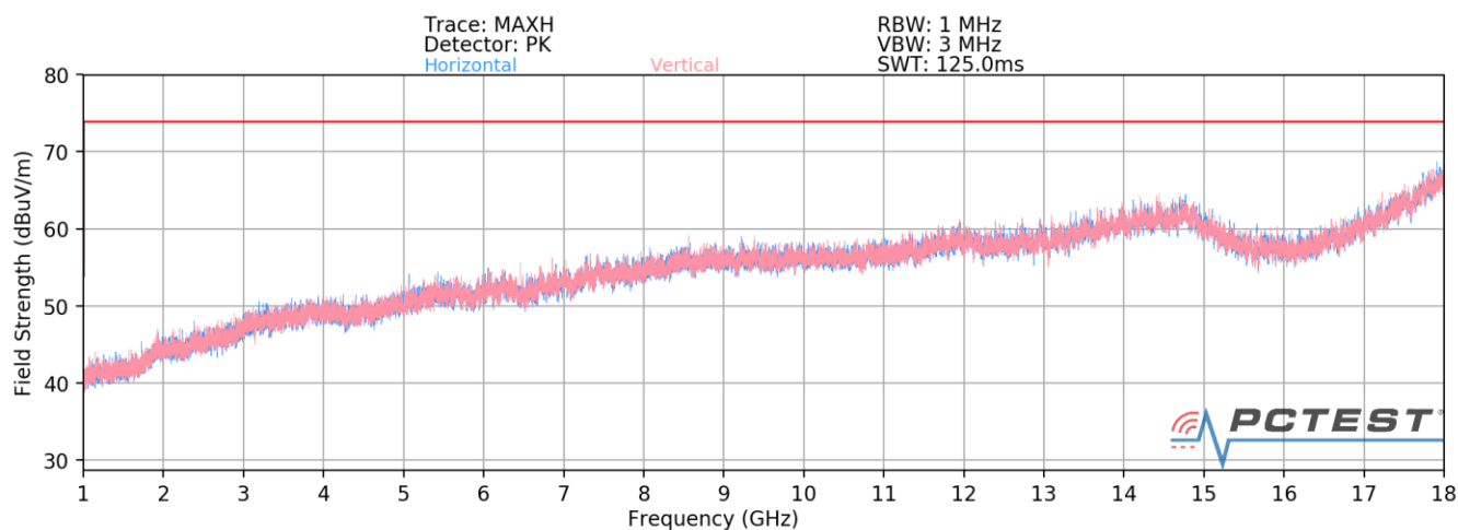
Plot 7-8. Radiated Spurious Plot above 1GHz [Radiated Test Config. 2 - Closed]
