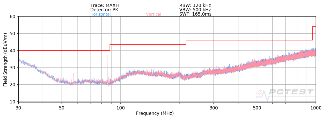
Plot 7-12. Radiated Spurious Plot below 1GHz [Radiated Test Config. 4 - Closed]
