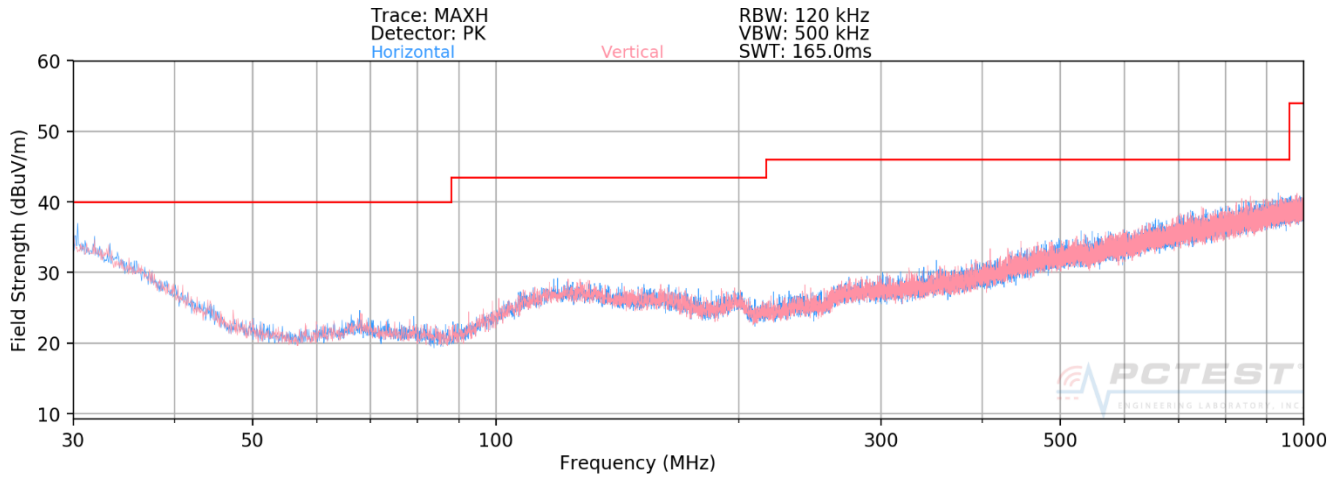
Plot 7-5. Radiated Spurious Plot below 1GHz [Radiated Test Config. 2 - Open]
