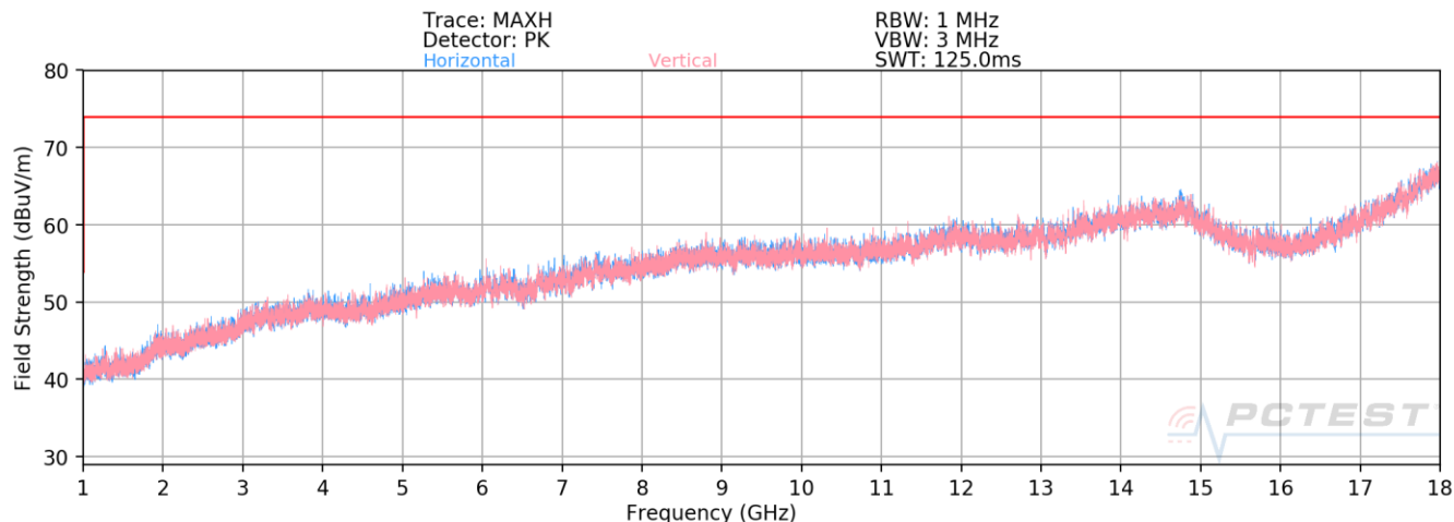
Plot 7-3. Radiated Spurious Plot above 1GHz [Radiated Test Config. 1 - Open]
