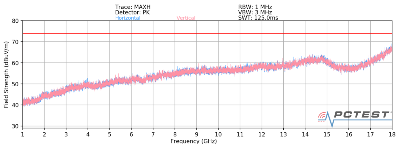
Plot 7-4. Radiated Spurious Plot above 1GHz [Radiated Test Config. 1 - Closed]
