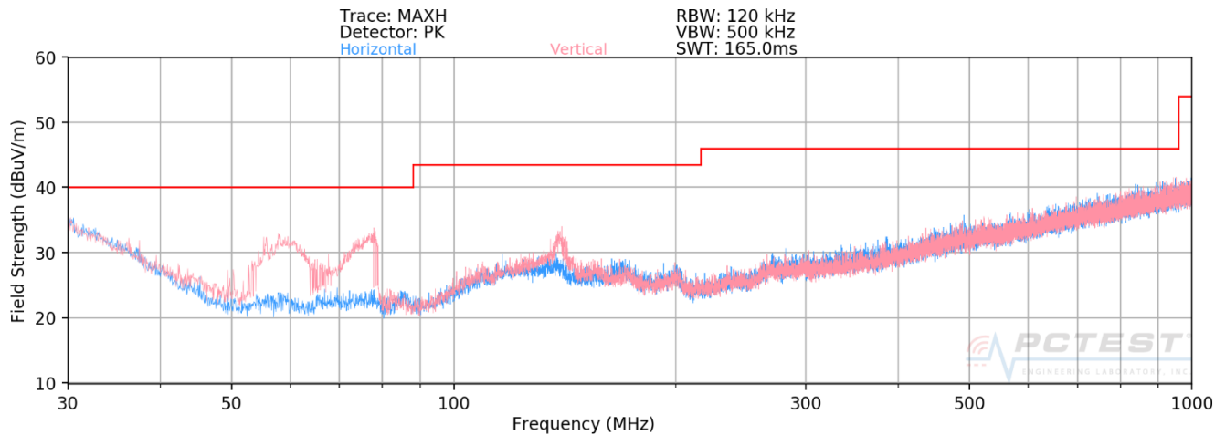
Plot 7-1. Radiated Spurious Plot below 1GHz [Radiated Test Config. 1 - Open]
