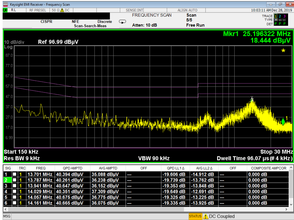
Plot 7-23. Line Conducted Plot (L1 - Open)
