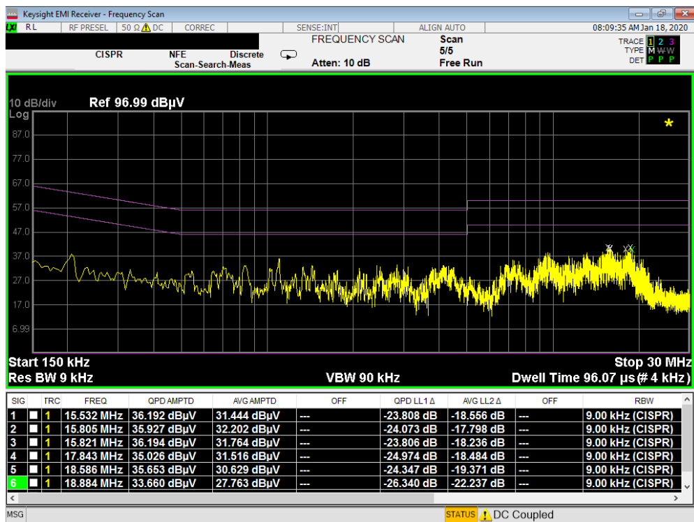
Plot 7-28. Line Conducted Plot (N - Closed)
