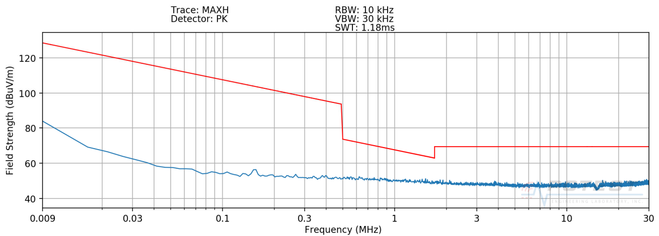
Plot 7-6. Radiated Spurious Plot 9kHz – 30MHz (Pol. Z – Device to Device WPT – CLOSED)
