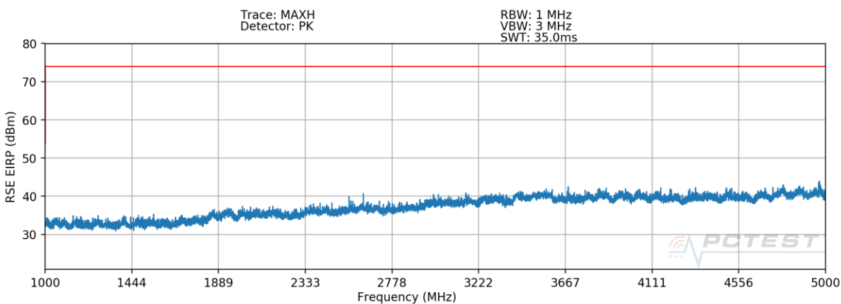
Plot 7-5. Radiated Spurious Plot above 1GHz – H – OPEN
