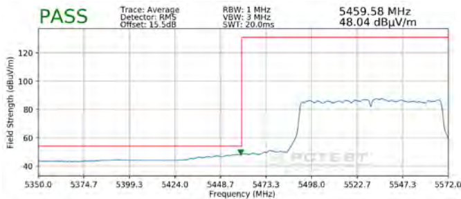
Plot 7-255. Radiated Lower Band Edge Plot MIMO (Average – UNII Band 2C)
