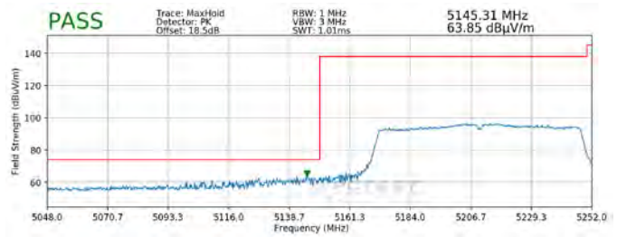
Plot 7-206. Radiated Lower Band Edge Plot SISO ANT1 (Peak – UNII Band 1)
