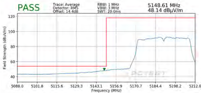
Plot 7-242. Radiated Lower Band Edge Plot MIMO (Average – UNII Band 1)
