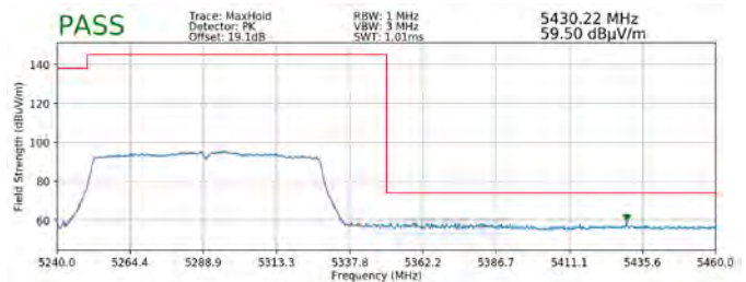
Plot 7-229. Radiated Upper Band Edge Plot SISO ANT2 (Peak – UNII Band 2A)
