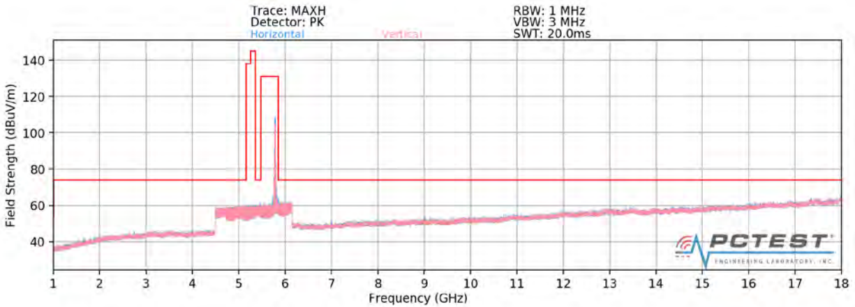
Plot 7-160. Radiated Spurious Plot above 1GHz SISO ANT1 (802.11a - U3 Ch. 157) - OPEN
