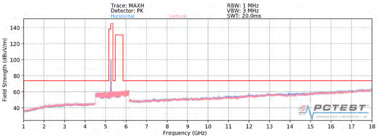
Plot 7-158. Radiated Spurious Plot above 1GHz SISO ANT1 (802.11a – U2A Ch. 56) – OPEN
