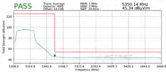
Plot 7-235. Radiated Upper Band Edge Plot MIMO (Average – UNII Band 2A)
