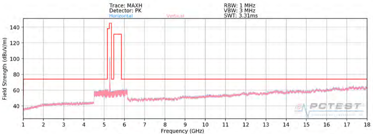
Plot 7-170. Radiated Spurious Plot above 1GHz SISO ANT2 (802.11a – U2A Ch. 56) – OPEN
