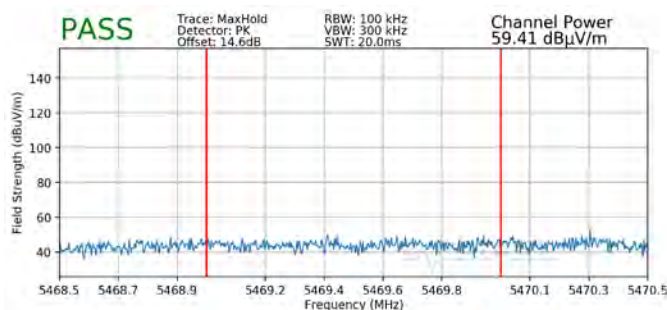
Plot 7-238. Radiated Lower Band Edge Plot CDD (Peak – UNII Band 2C)
