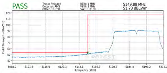
Plot 7-198. Radiated Lower Band Edge Plot SISO ANT1 (Average – UNII Band 1)
