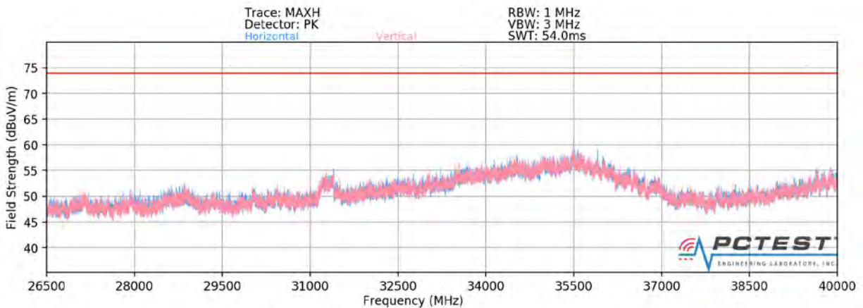
Plot 7-182. Radiated Spurious Plot 26.5GHz - 40GHz MIMO/CDD (802.11a) – OPEN
