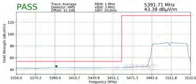
Plot 7-223. Radiated Lower Band Edge Plot SISO ANT2 (Average - UNII Band 2C)
