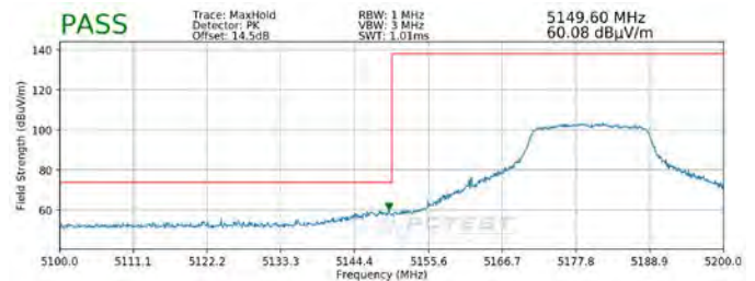
Plot 7-241. Radiated Band Edge Plot MIMO (Peak – WCP)
