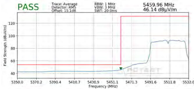
Plot 7-246. Radiated Lower Band Edge Plot MIMO (Average – UNII Band 2C)
