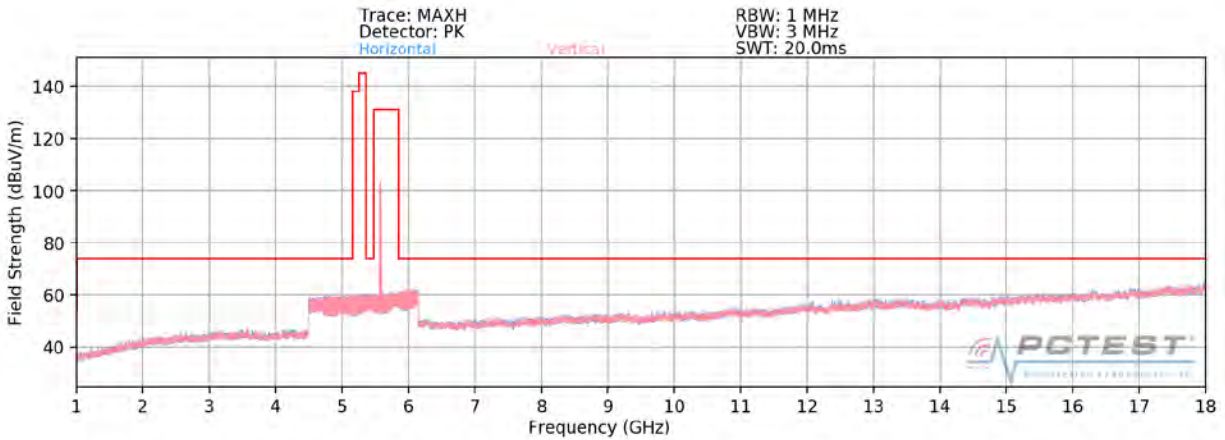
Plot 7-163. Radiated Spurious Plot above 1GHz SISO ANT1 (802.11a – U2C Ch. 120) – CLOSED
