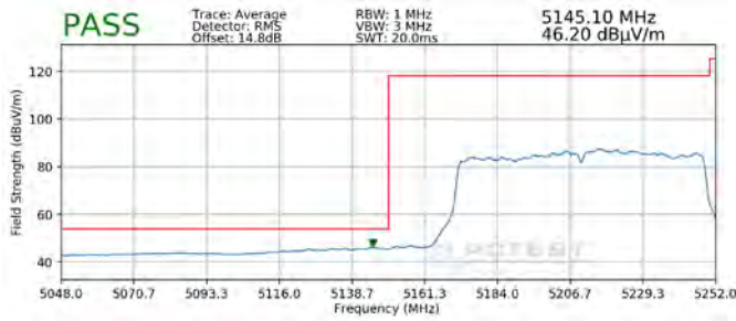
Plot 7-251. Radiated Lower Band Edge Plot MIMO (Average – UNII Band 1)
