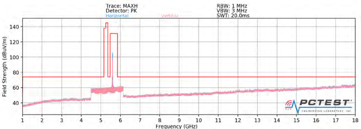
Plot 7-171. Radiated Spurious Plot above 1GHz SISO ANT2 (802.11a – U2C Ch. 120) – OPEN
