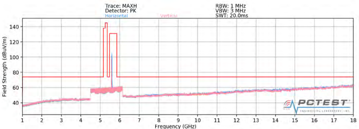
Plot 7-159. Radiated Spurious Plot above 1GHz SISO ANT1 (802.11a – U2C Ch. 120) – OPEN
