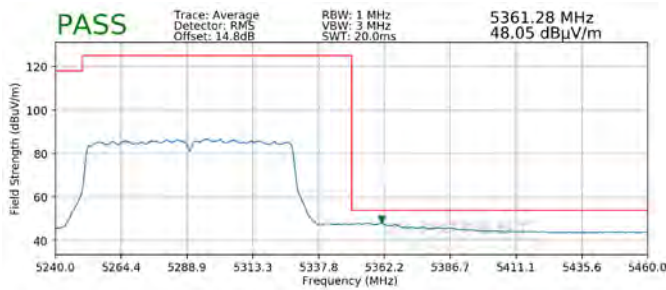
Plot 7-253. Radiated Upper Band Edge Plot MIMO (Average – UNII Band 2A)
