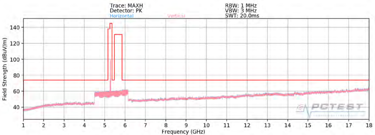
Plot 7-162. Radiated Spurious Plot above 1GHz SISO ANT1 (802.11a - U2A Ch. 56) - CLOSED
