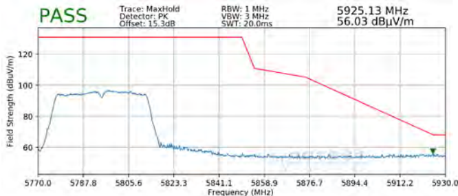
Plot 7-225. Radiated Upper Band Edge Plot SISO ANT2 (Peak - UNII Band 3)
