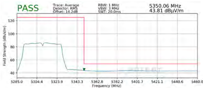
Plot 7-221. Radiated Upper Band Edge Plot SISO ANT2 (Average - UNII Band 2A)
