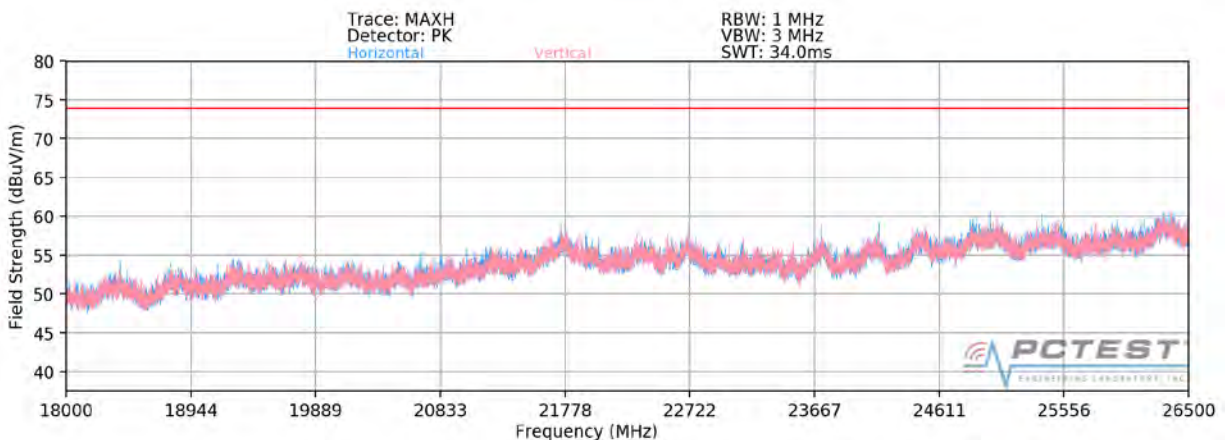
Plot 7-179. Radiated Spurious Plot above 18GHz - 26.5GHz SISO ANT2 (802.11a) – CLOSED
