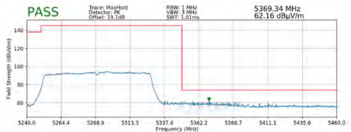
Plot 7-208. Radiated Upper Band Edge Plot SISO ANT1 (Peak – UNII Band 2A)
