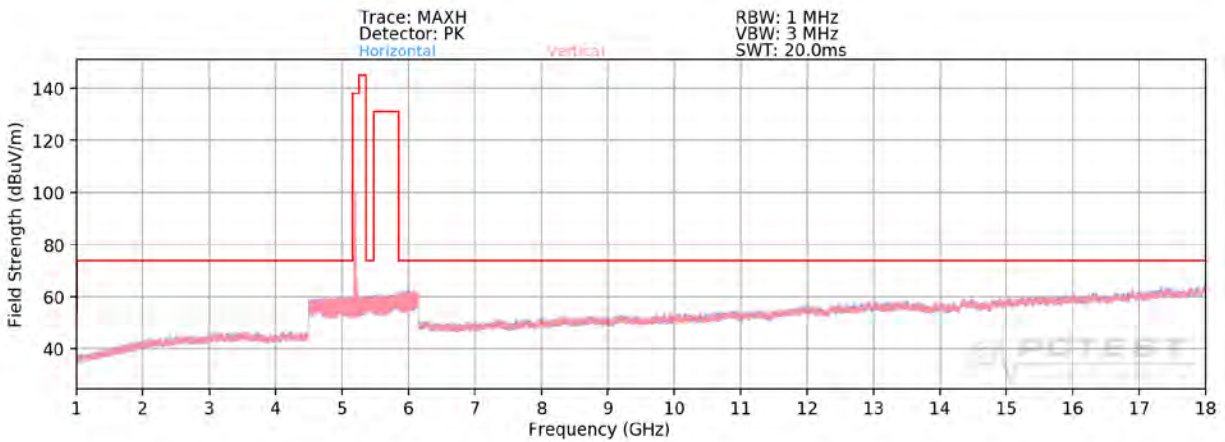
Plot 7-161. Radiated Spurious Plot above 1GHz SISO ANT1 (802.11a - U1 Ch. 40) - CLOSED
