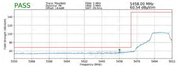
Plot 7-217. Radiated Lower Band Edge Plot SISO ANT2 (Peak - UNII Band 2C)
