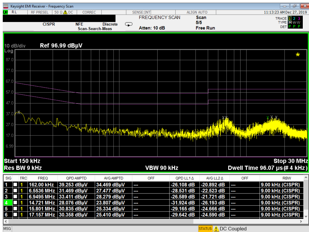
Plot 7-120. Line Conducted Plot with 802.11b (N) – OPEN
