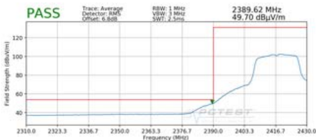
Plot 7-83. Radiated Restricted Upper Band Edge Measurement SISO ANT1 (Average)
