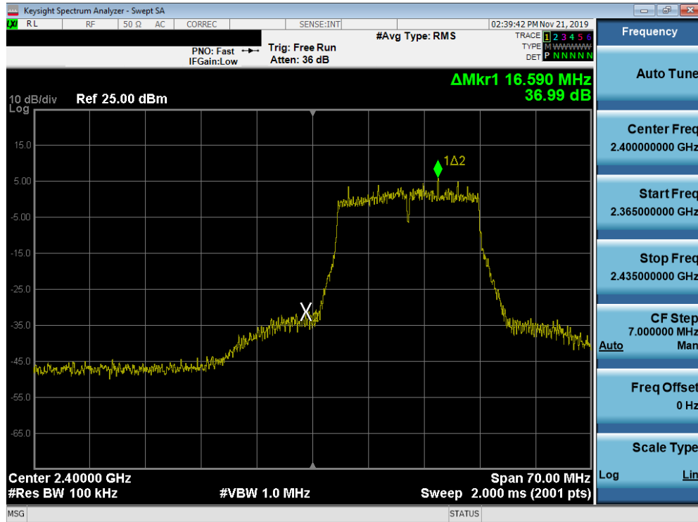
Plot 7-53. Band Edge Plot SISO ANT2 (802.11n (2.4GHz) – Ch. 1)
