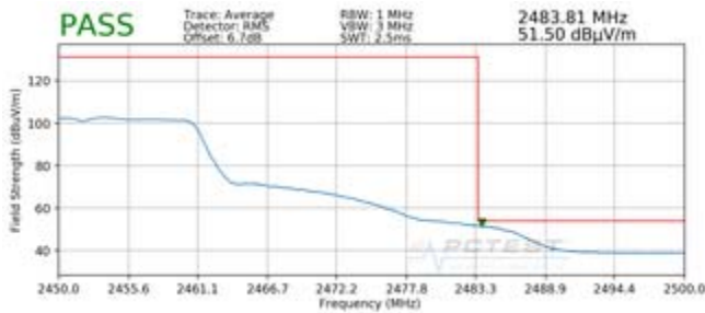
Plot 7-87. Radiated Restricted Upper Band Edge Measurement SISO ANT1 (Average)
