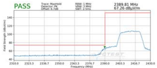
Plot 7-94. Radiated Restricted Lower Band Edge Measurement SISO ANT2 (Peak)
