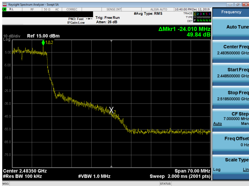
Plot 7-44. Band Edge Plot SISO ANT1 (802.11n (2.4GHz) – Ch. 9)
