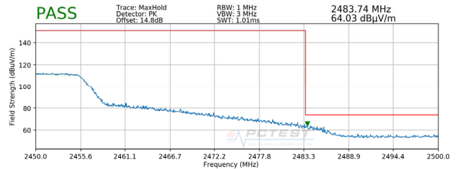
Plot 7-110. Radiated Restricted Upper Band Edge Measurement MIMO (Peak)
