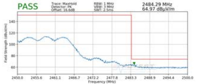
Plot 7-114. Radiated Restricted Upper Band Edge Measurement MIMO (Peak)
