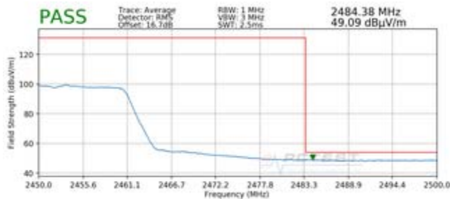
Plot 7-111. Radiated Restricted Upper Band Edge Measurement MIMO (Average)
