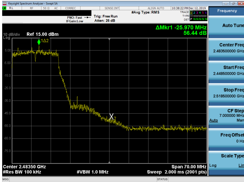
Plot 7-41. Band Edge Plot SISO ANT1 (802.11g – Ch. 10)
