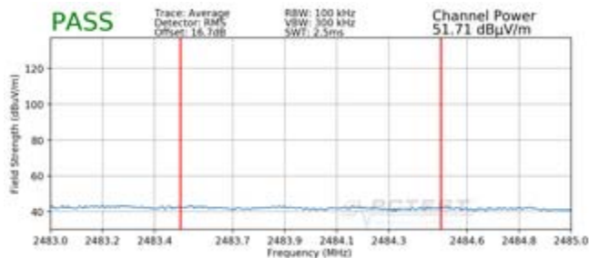
Plot 7-115. Radiated Restricted Upper Band Edge Measurement MIMO (Average)
