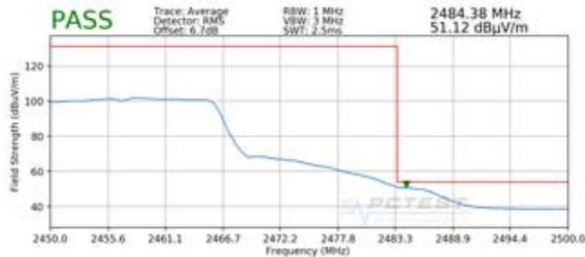
Plot 7-89. Radiated Restricted Upper Band Edge Measurement SISO ANT1 (Average)
