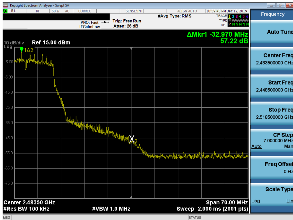
Plot 7-50. Band Edge Plot SISO ANT2 (802.11g - Ch. 9)
