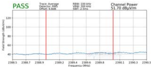
Plot 7-93. Radiated Restricted Lower Band Edge Measurement SISO ANT2 (Average)
