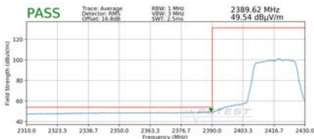
Plot 7-107. Radiated Restricted Lower Band Edge Measurement MIMO (Average)
