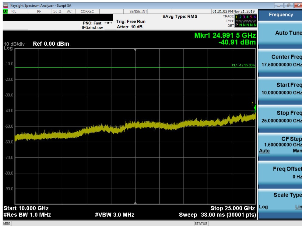
Plot 7-58. Conducted Spurious Plot SISO ANT1 (802.11b – Ch. 1)
