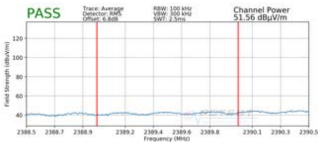
Plot 7-81. Radiated Restricted Lower Band Edge Measurement SISO ANT1 (Average)
