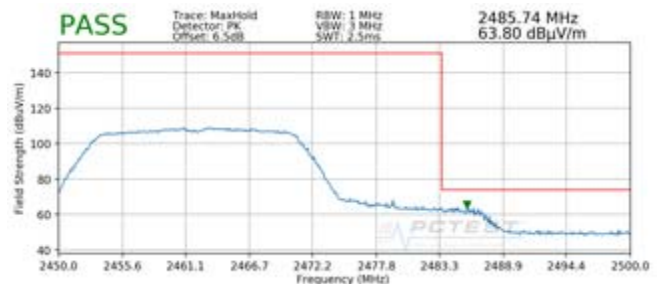
Plot 7-92. Radiated Restricted Upper Band Edge Measurement SISO ANT1 (Peak)
