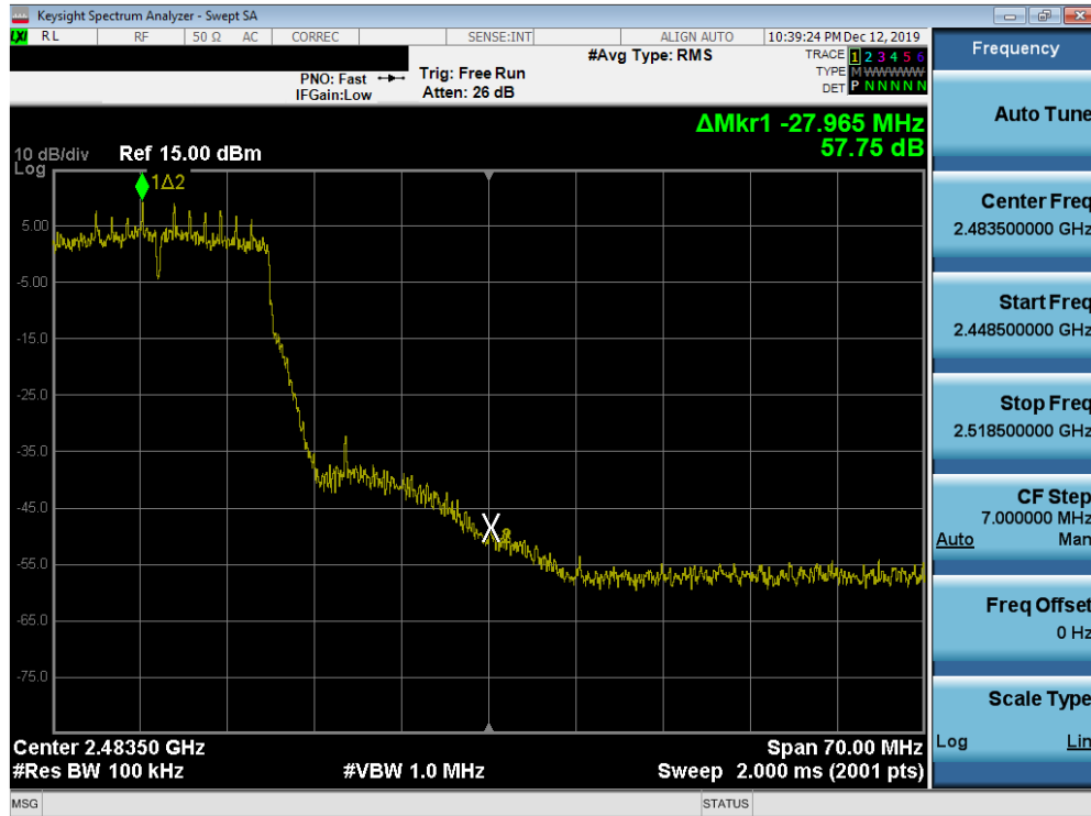
Plot 7-45. Band Edge Plot SISO ANT1 (802.11n (2.4GHz) – Ch. 10)
