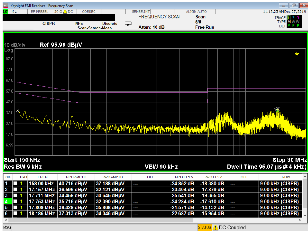
Plot 7-119. Line Conducted Plot with 802.11b (L1) – OPEN
