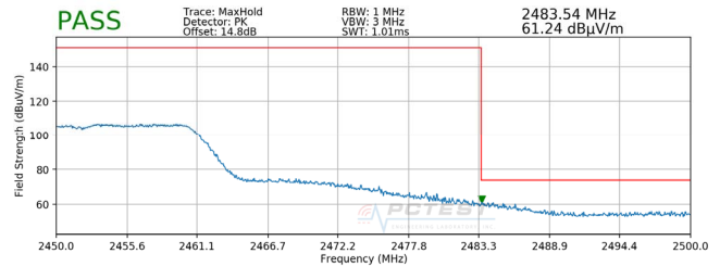
Plot 7-100. Radiated Restricted Upper Band Edge Measurement SISO ANT2 (Peak)
