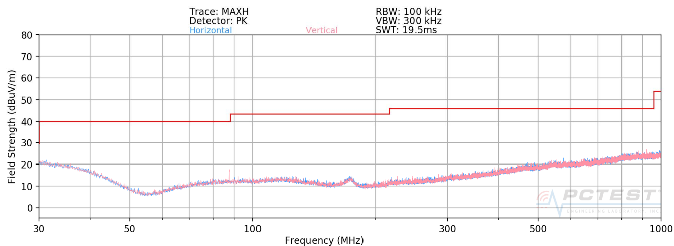
Plot 7-118. Radiated Spurious Plot below 1GHz MIMO (802.11n - Open)
