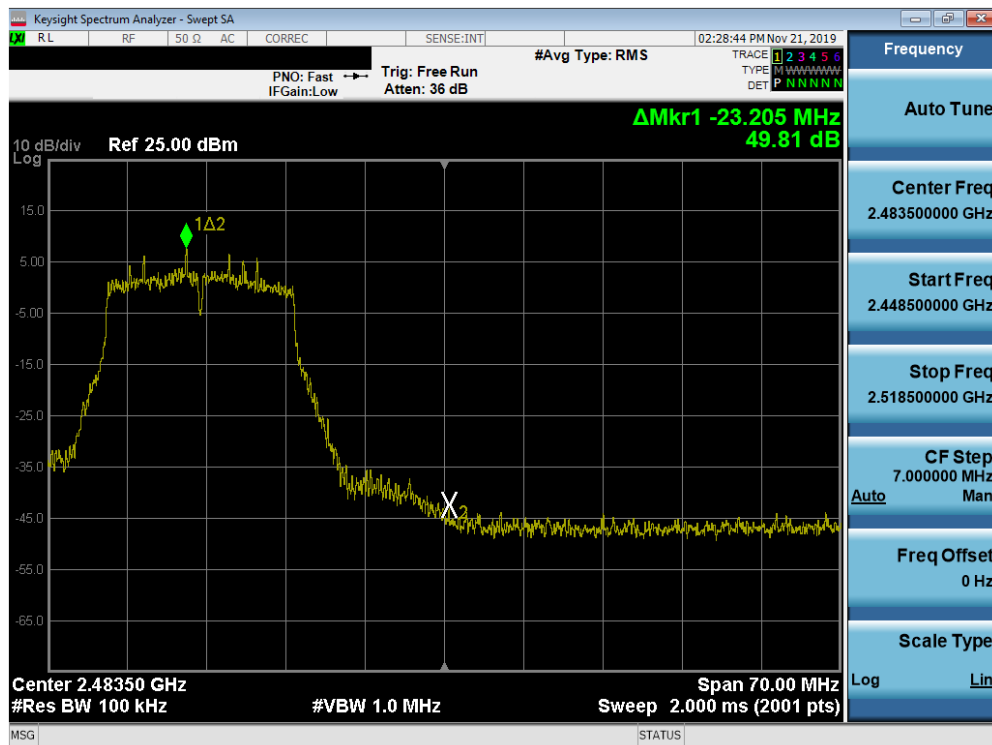
Plot 7-52. Band Edge Plot SISO ANT2 (802.11g – Ch. 11)
