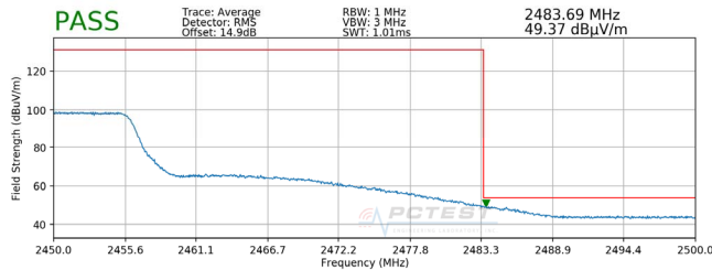
Plot 7-97. Radiated Restricted Upper Band Edge Measurement SISO ANT2 (Average)
