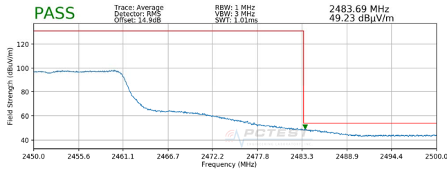
Plot 7-99. Radiated Restricted Upper Band Edge Measurement SISO ANT2 (Average)
