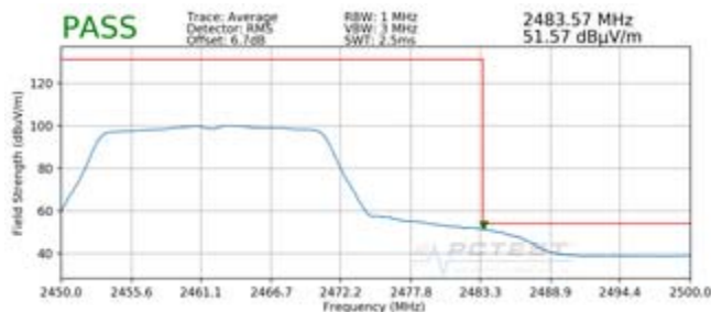
Plot 7-91. Radiated Restricted Upper Band Edge Measurement SISO ANT1 (Average)
