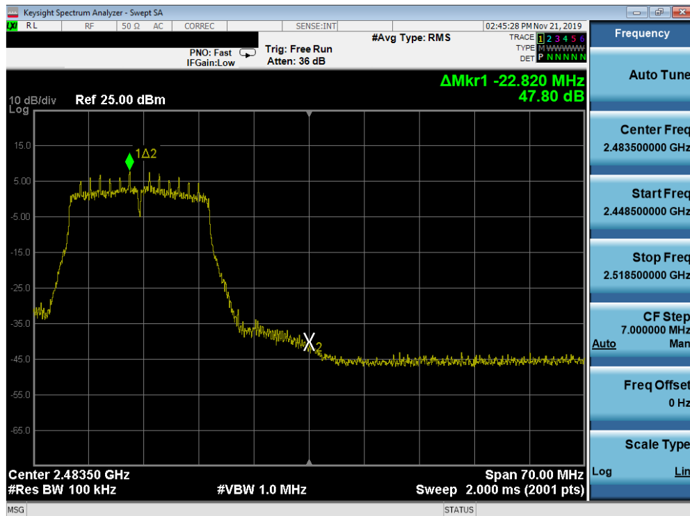
Plot 7-56. Band Edge Plot SISO ANT2 (802.11n (2.4GHz) – Ch. 11)
