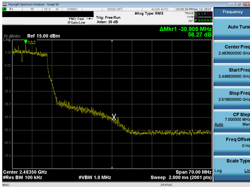
Plot 7-54. Band Edge Plot SISO ANT2 (802.11n (2.4GHz) – Ch. 9)
