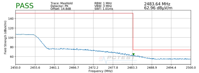
Plot 7-98. Radiated Restricted Upper Band Edge Measurement SISO ANT2 (Peak)
