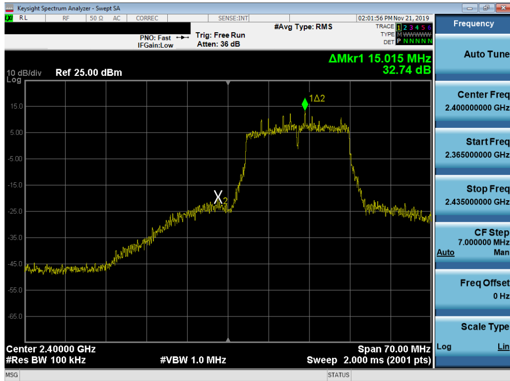
Plot 7-43. Band Edge Plot SISO ANT1 (802.11n (2.4GHz) – Ch. 1)
