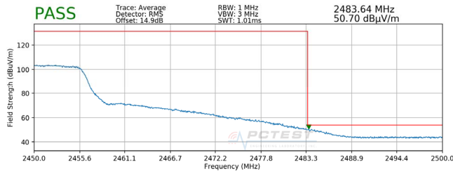
Plot 7-109. Radiated Restricted Upper Band Edge Measurement MIMO (Average)
