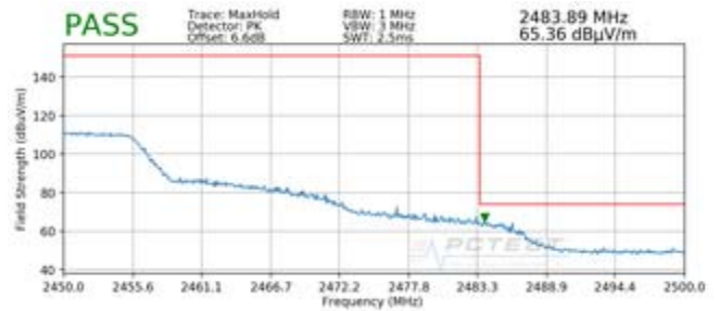
Plot 7-86. Radiated Restricted Upper Band Edge Measurement SISO ANT1 (Peak)
