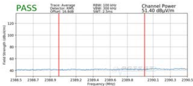
Plot 7-105. Radiated Restricted Lower Band Edge Measurement MIMO (Average)
