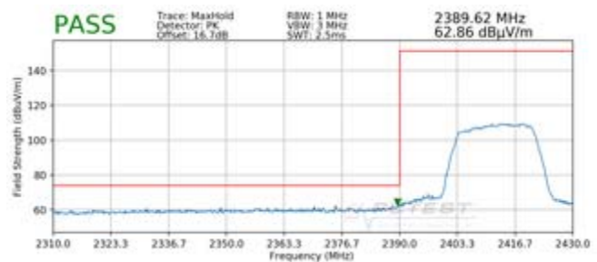
Plot 7-106. Radiated Restricted Lower Band Edge Measurement MIMO (Peak)
