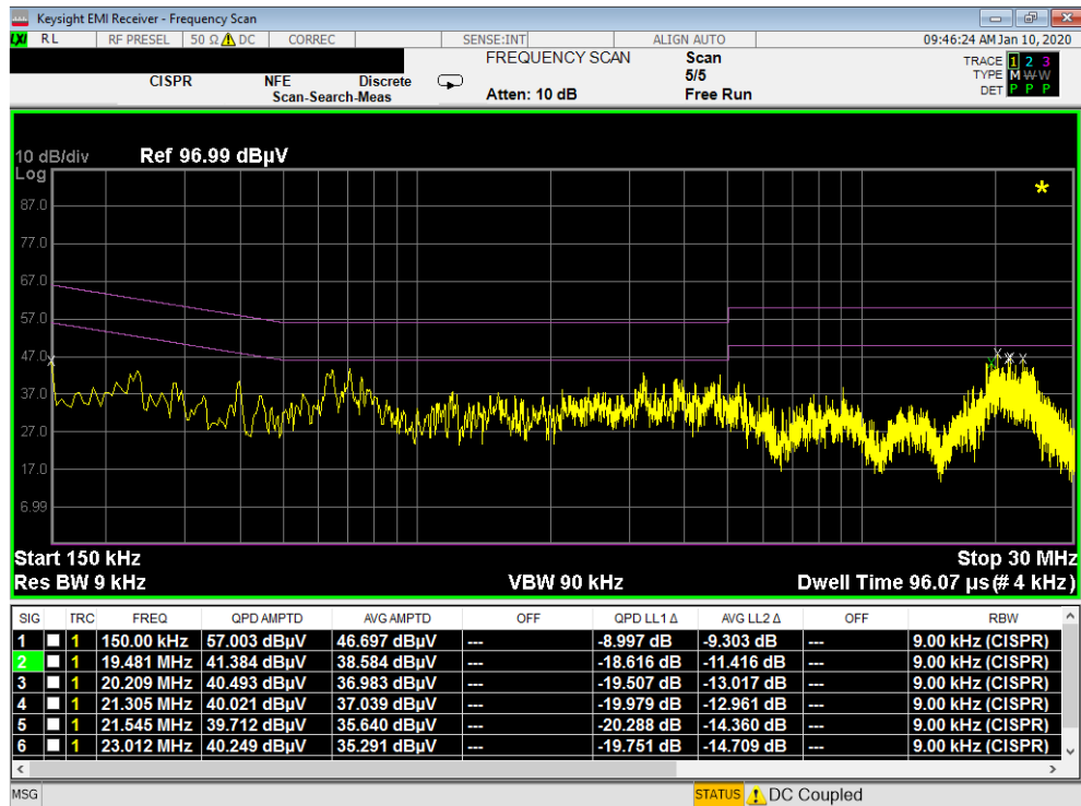
Plot 7-126. Line Conducted Plot with 802.11b (N) – CLOSED with WCP
