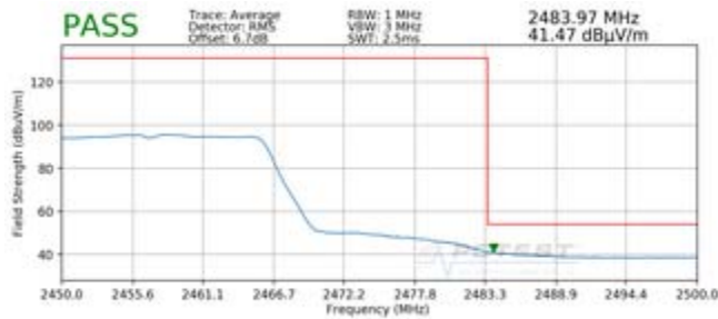
Plot 7-101. Radiated Restricted Upper Band Edge Measurement SISO ANT2 (Average)
