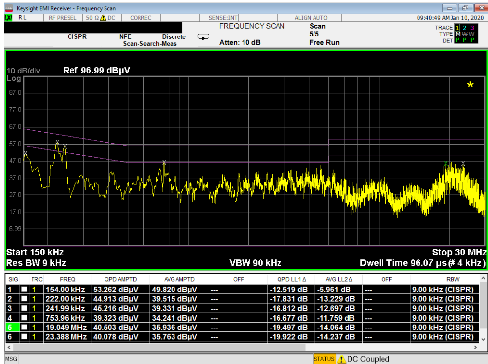
Plot 7-124. Line Conducted Plot with 802.11b (N) – OPEN with WCP
