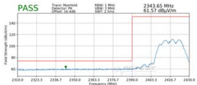
Plot 7-108. Radiated Restricted Lower Band Edge Measurement MIMO (Peak)
