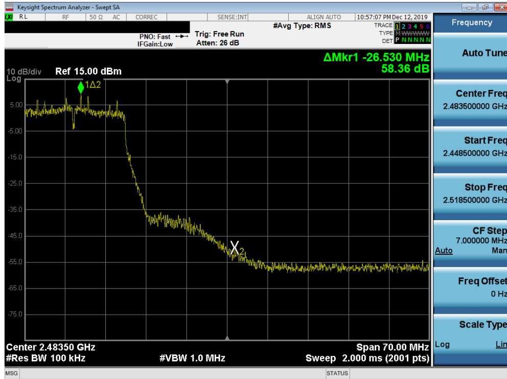
Plot 7-55. Band Edge Plot SISO ANT2 (802.11n (2.4GHz) – Ch. 10)
