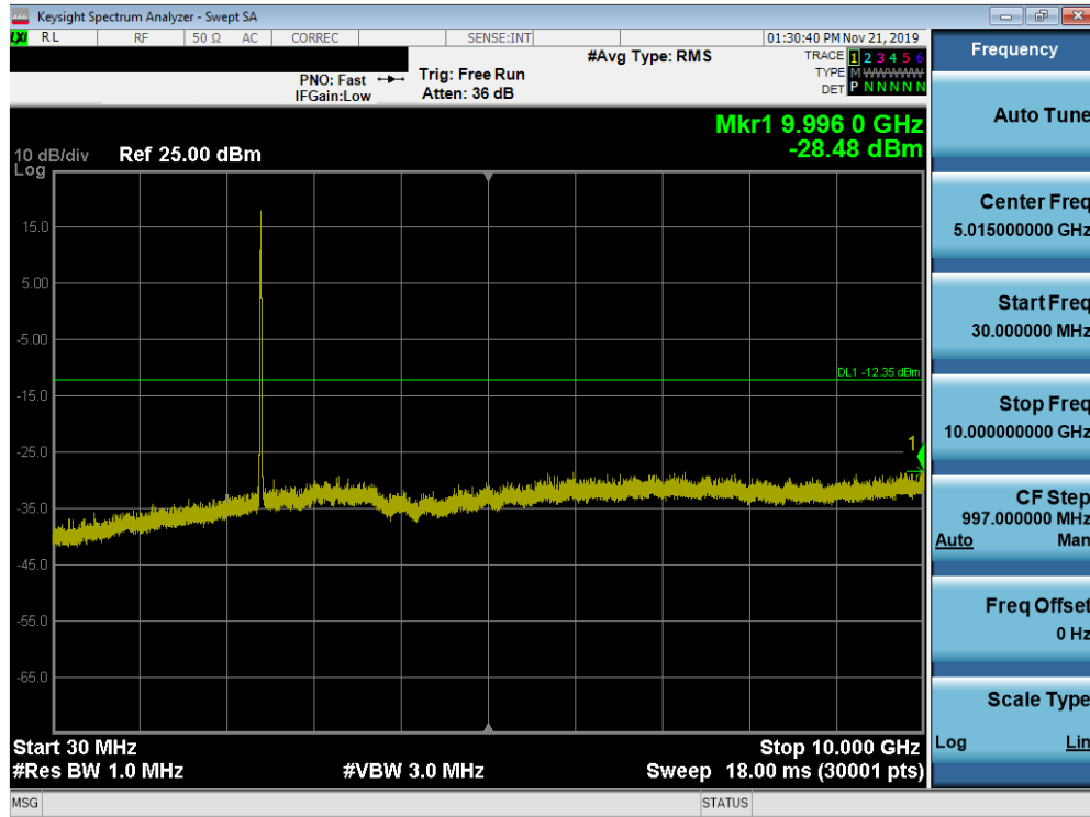
Plot 7-57. Conducted Spurious Plot SISO ANT1 (802.11b – Ch. 1)
