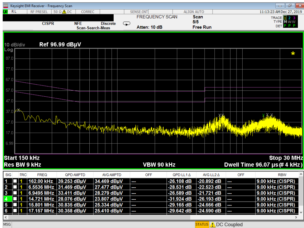
Plot 7-122. Line Conducted Plot with 802.11b (N) – CLOSED
