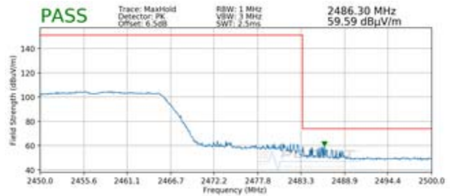
Plot 7-102. Radiated Restricted Upper Band Edge Measurement SISO ANT2 (Peak)
