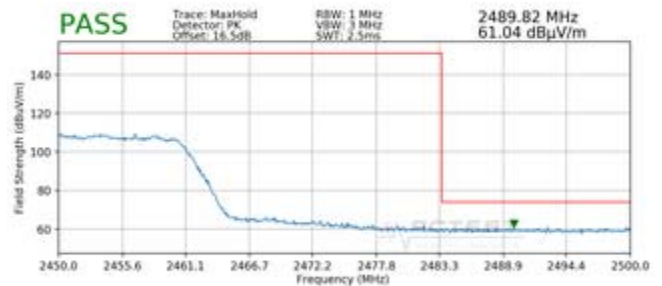
Plot 7-112. Radiated Restricted Upper Band Edge Measurement MIMO (Peak)
