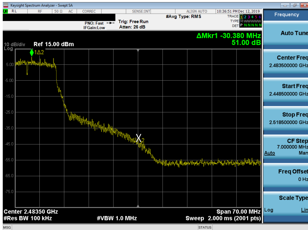
Plot 7-40. Band Edge Plot SISO ANT1 (802.11g - Ch. 9)
