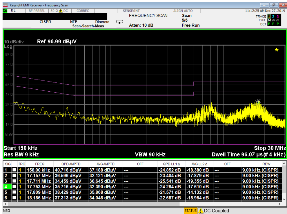
Plot 7-121. Line Conducted Plot with 802.11b (L1) – CLOSED
