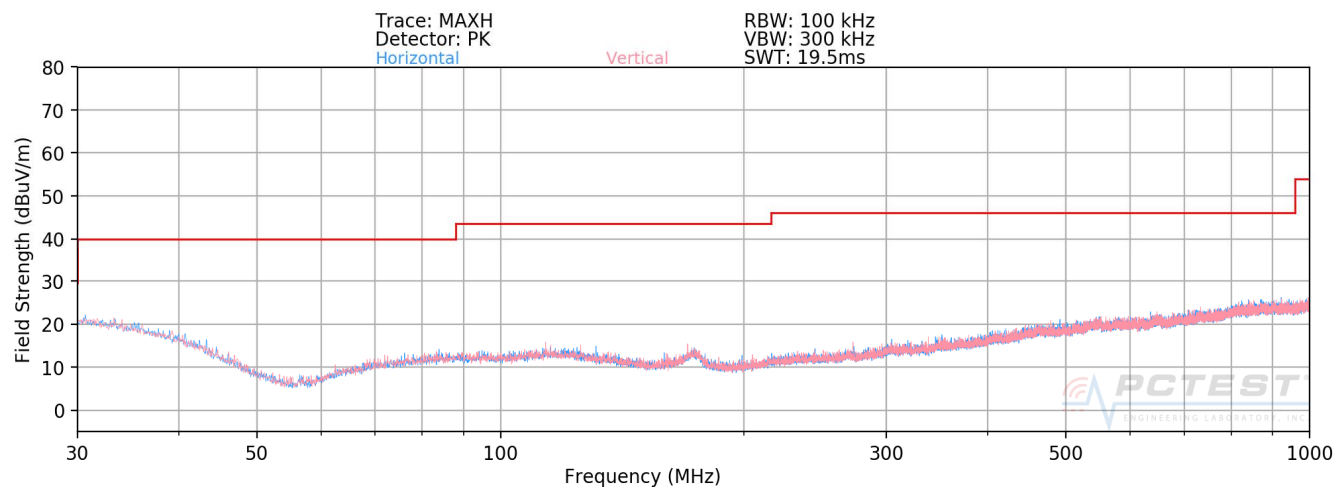
Plot 7-117. Radiated Spurious Plot below 1GHz MIMO (802.11n - Closed)
