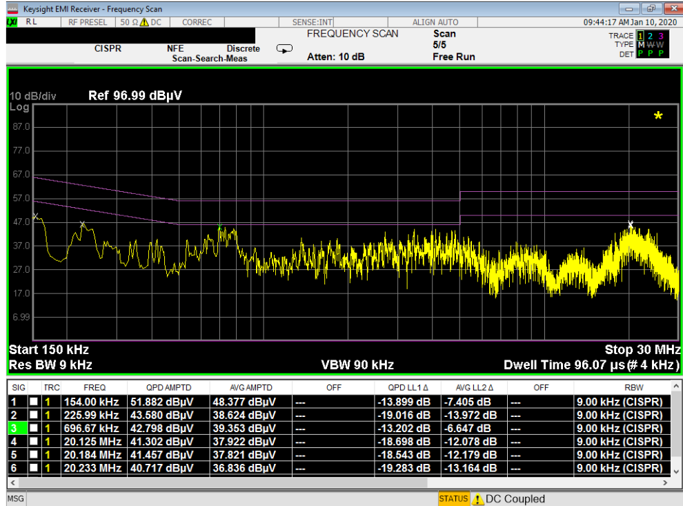
Plot 7-125. Line Conducted Plot with 802.11b (L1) – CLOSED with WCP
