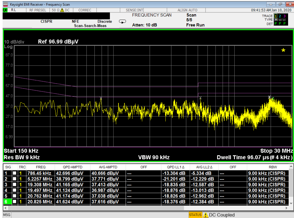
Plot 7-123. Line Conducted Plot with 802.11b (L1) – OPEN with WCP
