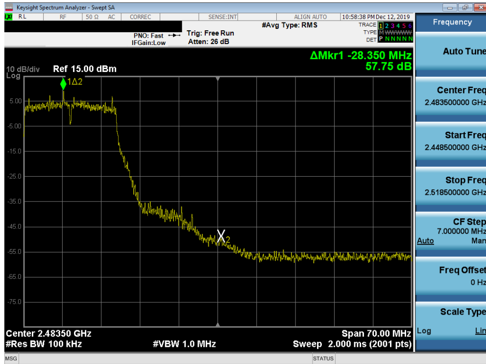
Plot 7-51. Band Edge Plot SISO ANT2 (802.11g – Ch. 10)
