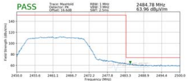
Plot 7-116. Radiated Restricted Upper Band Edge Measurement MIMO (Peak)
