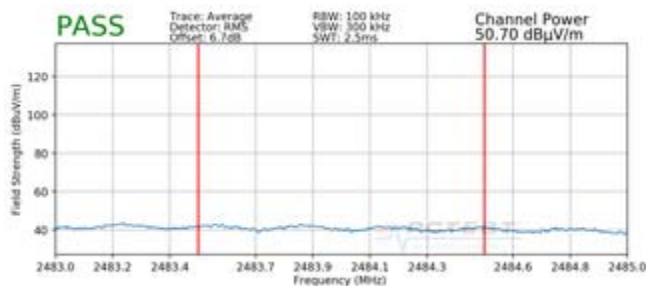
Plot 7-103. Radiated Restricted Upper Band Edge Measurement SISO ANT2 (Average)
