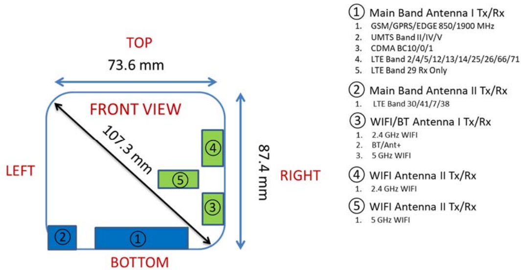
Figure E-3 DUT Antenna Locations Closed Configuration
