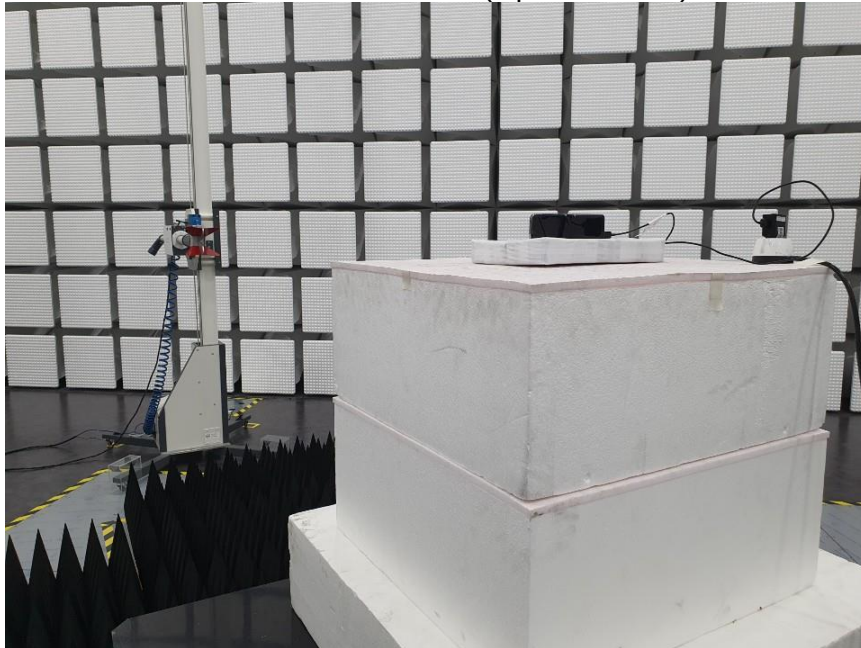
ABOVE 1 GHz REAR TEST PHOTO(Open & Y axis)
