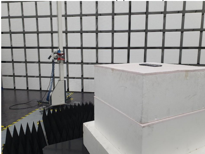
ABOVE 1 GHz REAR TEST PHOTO(Open & X axis)
