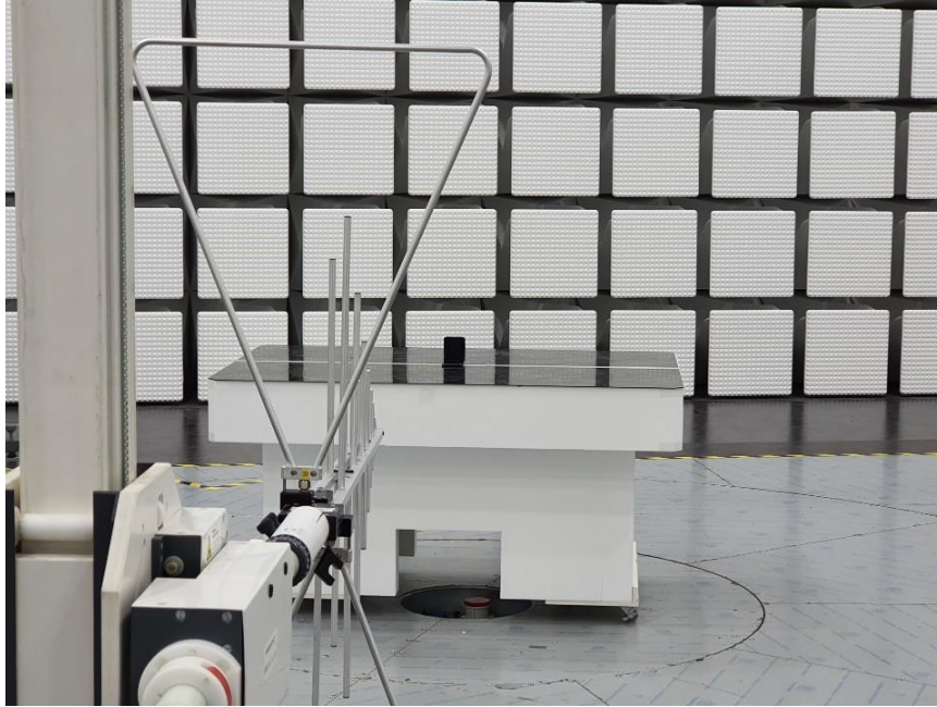
BELOW 1 GHz FRONT TEST PHOTO(Half-Folded & X axis)
