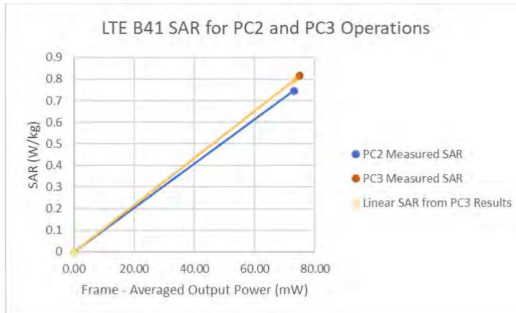
Figure 14-7 LTE Band 41 Phablet Linearity
