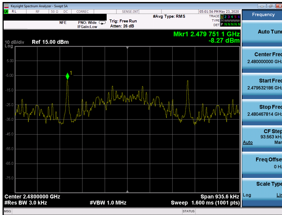
Plot 7-27. Power Spectral Density Plot (Bluetooth (LE), 125kbps – Ch. 39)
