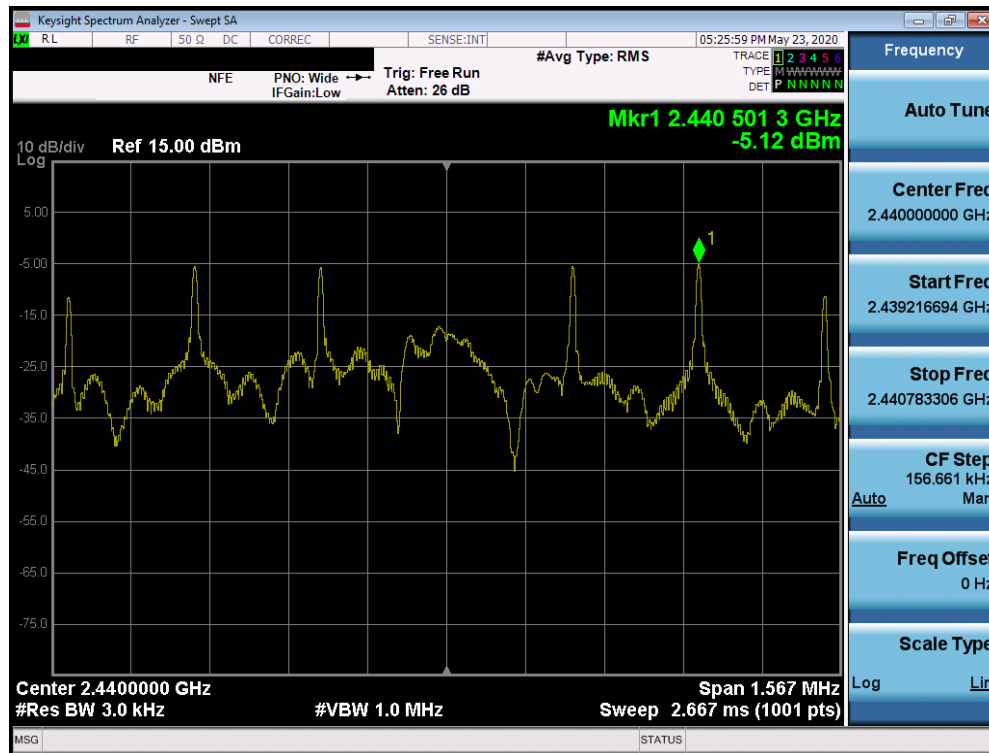
Plot 7-35. Power Spectral Density Plot (Bluetooth (LE), 2Mbps – Ch. 19)
