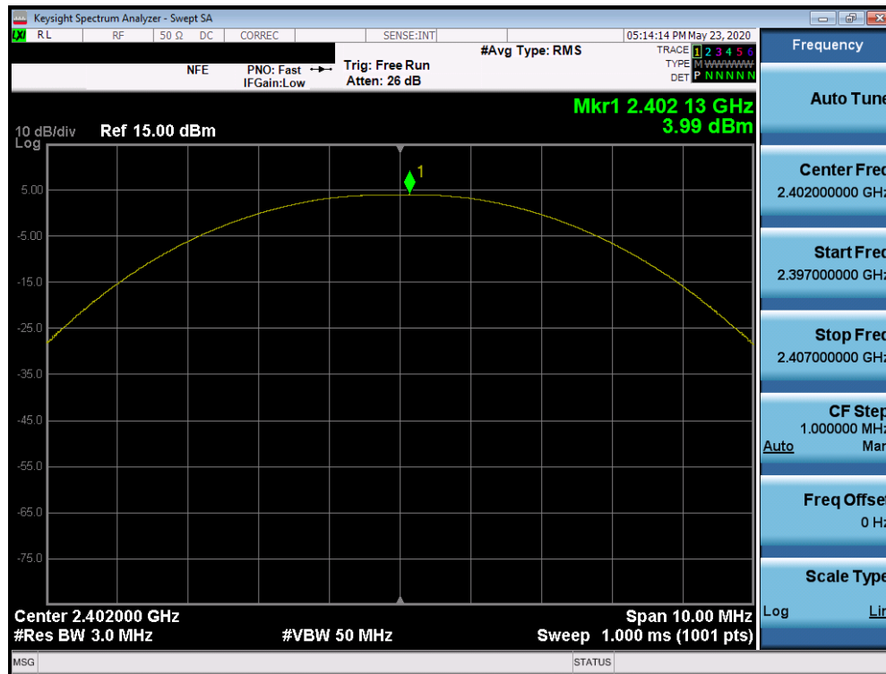
Plot 7-19. Peak Power Plot (Bluetooth (LE), 1Mbps – Ch. 0)
