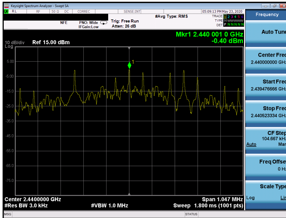
Plot 7-29. Power Spectral Density Plot (Bluetooth (LE), 500kbps – Ch. 19)
