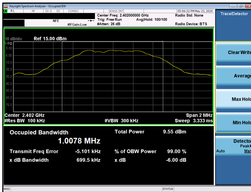
Plot 7-4. 6dB Bandwidth Plot (Bluetooth (LE), 500kbps – Ch. 0)
