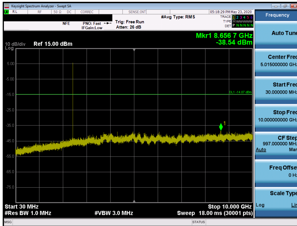
Plot 7-47. Conducted Spurious Plot (Bluetooth (LE), 1Mbps – Ch. 19)
