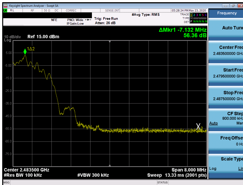
Plot 7-44. Band Edge Plot (Bluetooth (LE), 2Mbps - Ch. 39)
