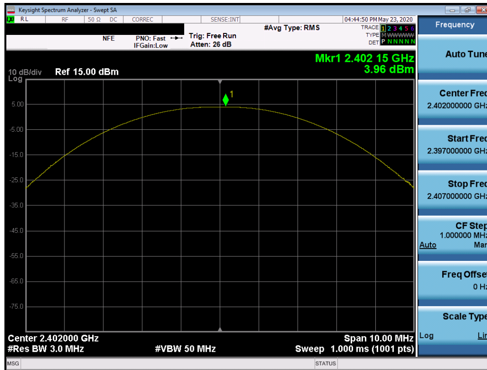
Plot 7-13. Peak Power Plot (Bluetooth (LE), 125kbps – Ch. 0)
