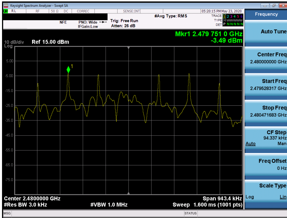
Plot 7-33. Power Spectral Density Plot (Bluetooth (LE), 1Mbps – Ch. 39)
