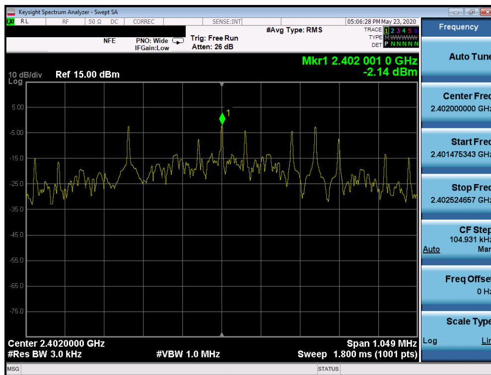
Plot 7-28. Power Spectral Density Plot (Bluetooth (LE), 500kbps – Ch. 0)
