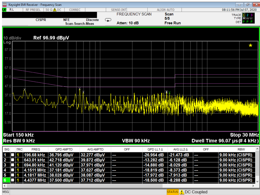
Plot 7-57. Line Conducted Plot with Bluetooth LE (N) with WCP
