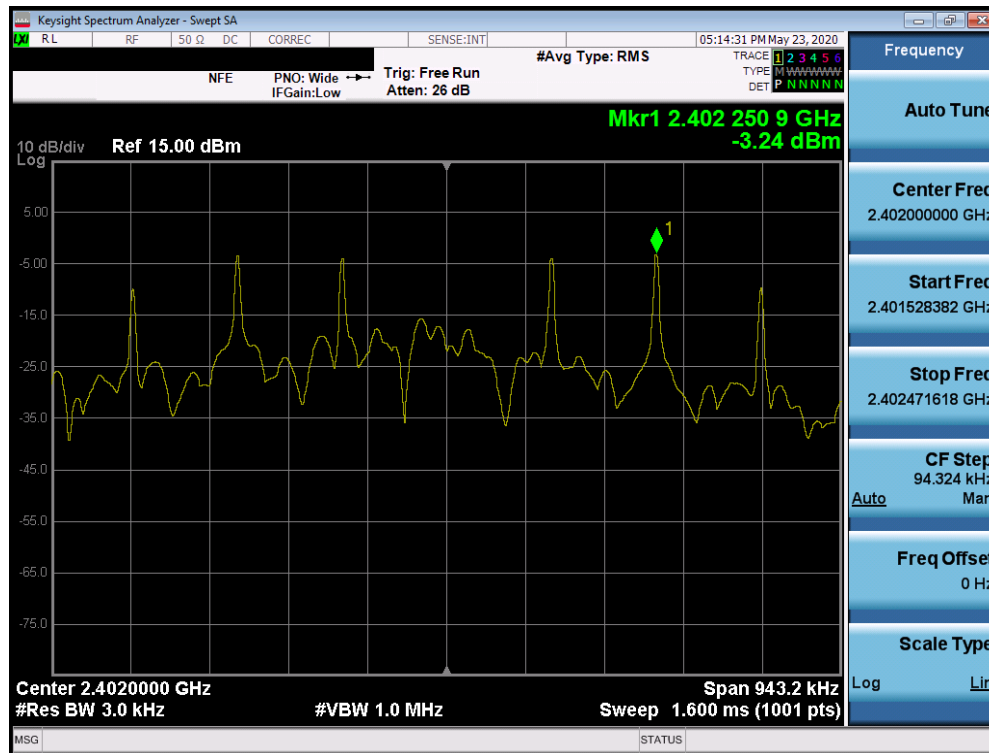
Plot 7-31. Power Spectral Density Plot (Bluetooth (LE), 1Mbps - Ch. 0)
