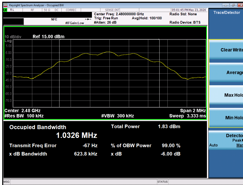
Plot 7-3. 6dB Bandwidth Plot (Bluetooth (LE), 125kbps – Ch. 39)
