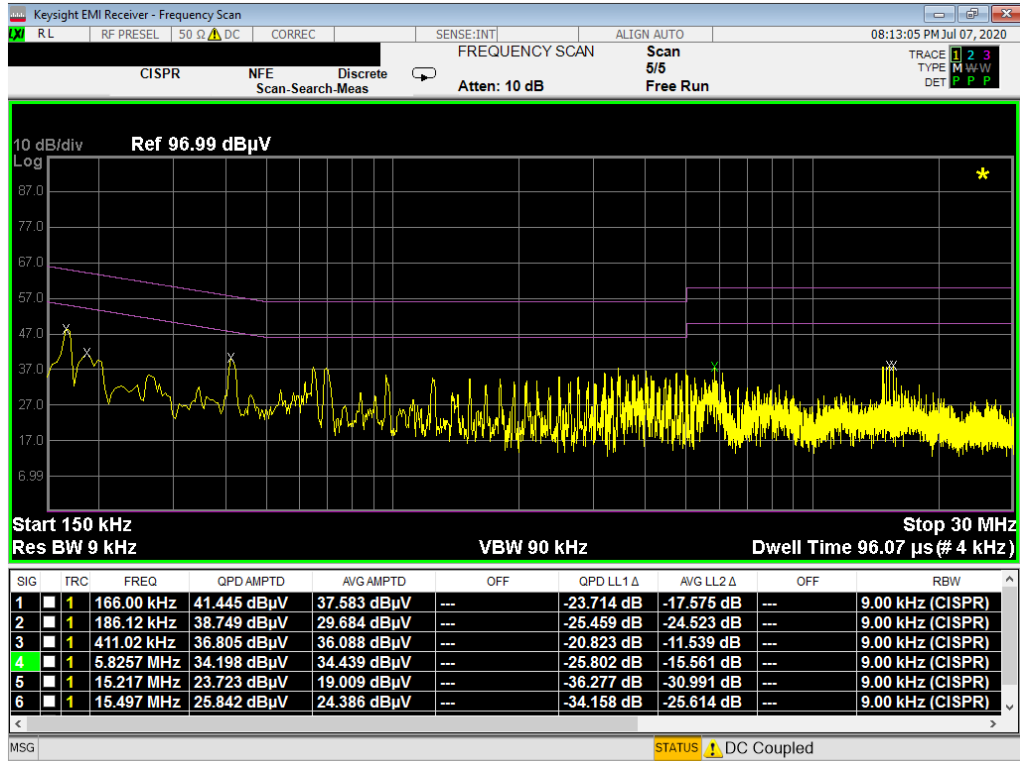
Plot 7-56. Line Conducted Plot with Bluetooth LE (L1) with WCP
