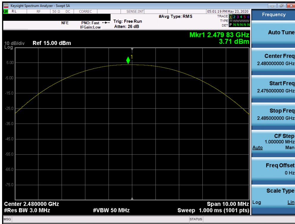
Plot 7-15. Peak Power Plot (Bluetooth (LE), 125kbps – Ch. 39)
