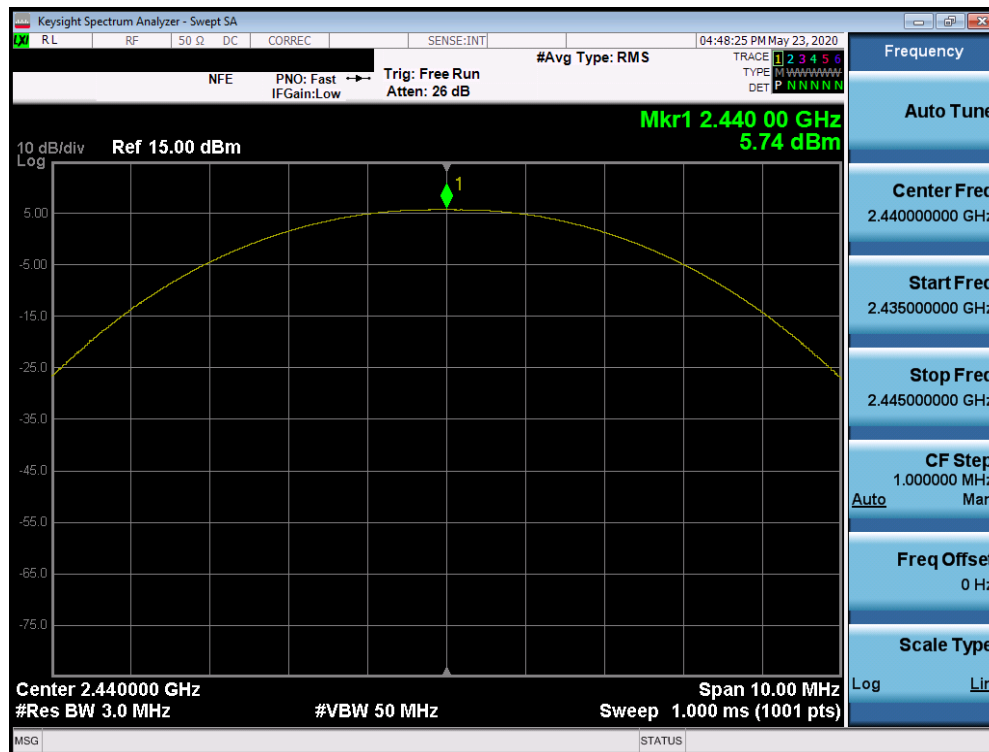
Plot 7-14. Peak Power Plot (Bluetooth (LE), 125kbps – Ch. 19)
