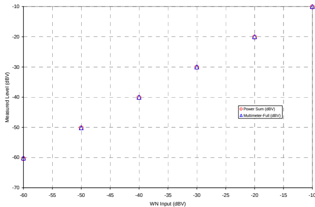
Figure 4-9 ABM2 Power Sum Validation
