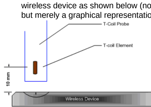
Figure 4-10 Measurement Distance
