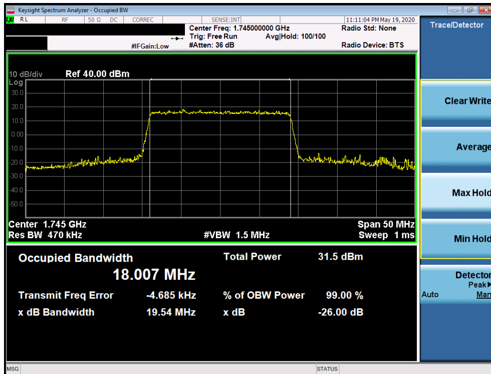
Plot 7-122. Occupied Bandwidth Plot (Band 66/4 - 20.0MHz 16-QAM - Full RB Configuration)
