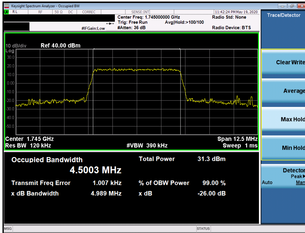
Plot 7-111. Occupied Bandwidth Plot (Band 66/4 - 5.0MHz 64-QAM - Full RB Configuration)
