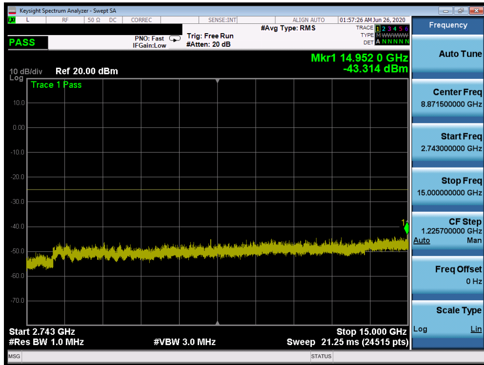
Plot 7-379. Conducted Spurious Plot (n41 - 100MHz DFT-s-OFDM-QPSK - RB Size 1, RB Offset 1 - Mid Channel)
