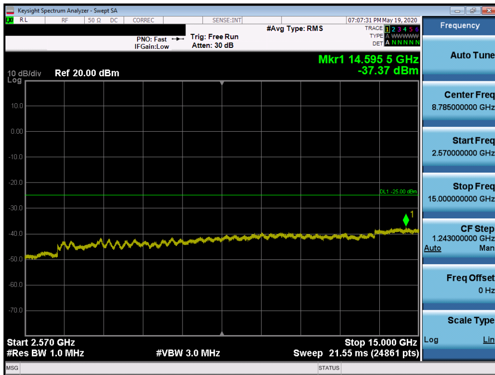
Plot 7-358. Conducted Spurious Plot (Band 7 - 20.0MHz QPSK - RB Size 1, RB Offset 0 - Low Channel)
