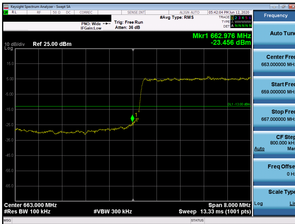
Plot 7-394. Lower Band Edge Plot (n71 - 10MHz DFT-s-OFDM-QPSK - Full RB Configuration)
