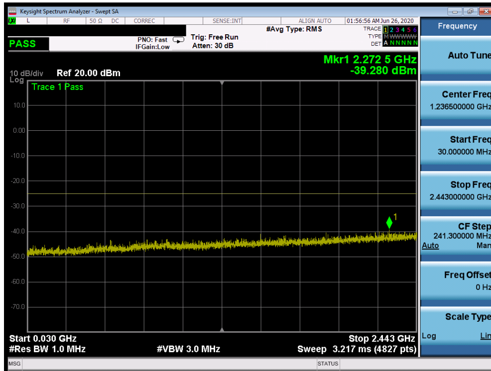
Plot 7-378. Conducted Spurious Plot (n41 - 100MHz DFT-s-OFDM-QPSK - RB Size 1, RB Offset 1 - Mid Channel)
