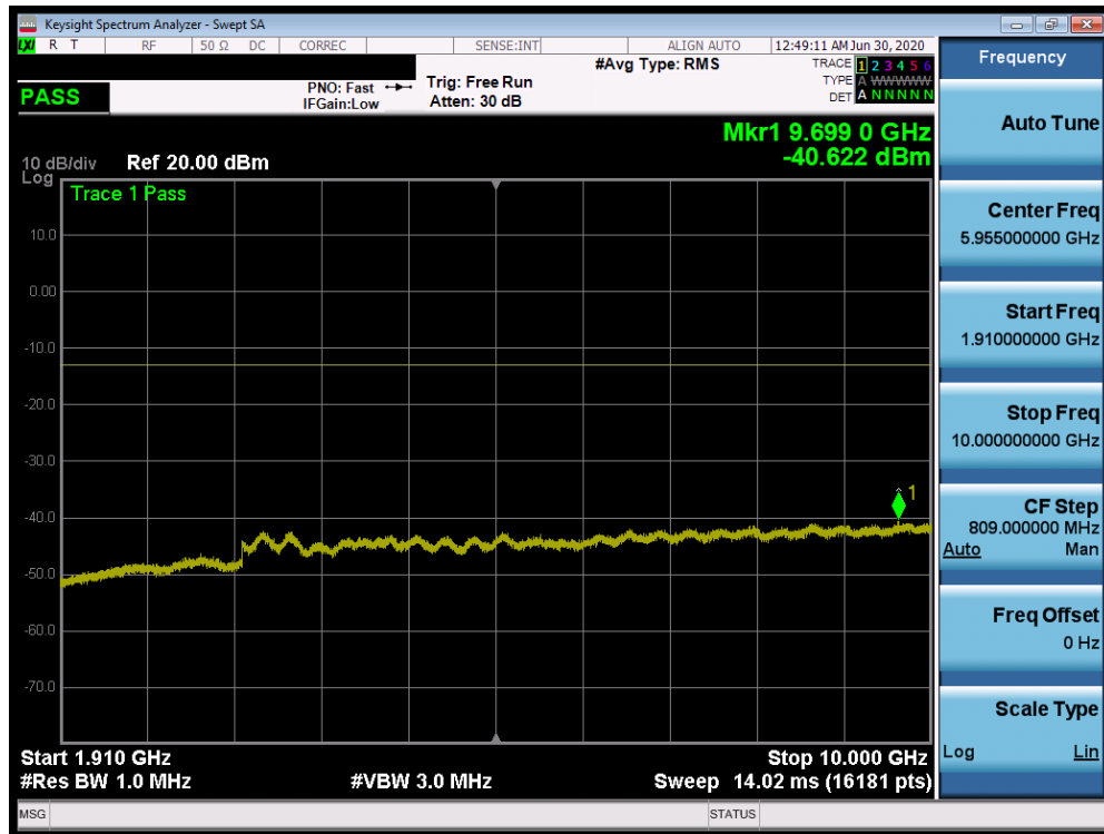
Plot 7-343. Conducted Spurious Plot (n25/2 - 20MHz DFT-s-OFDM-QPSK - RB Size 1, RB Offset 1 - Mid Channel)
