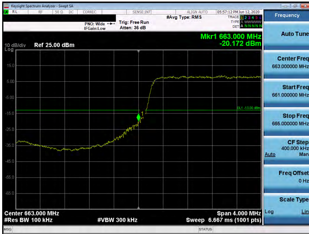
Plot 7-392. Lower Band Edge Plot (n71 - 5MHz DFT-s-OFDM-QPSK - Full RB Configuration)
