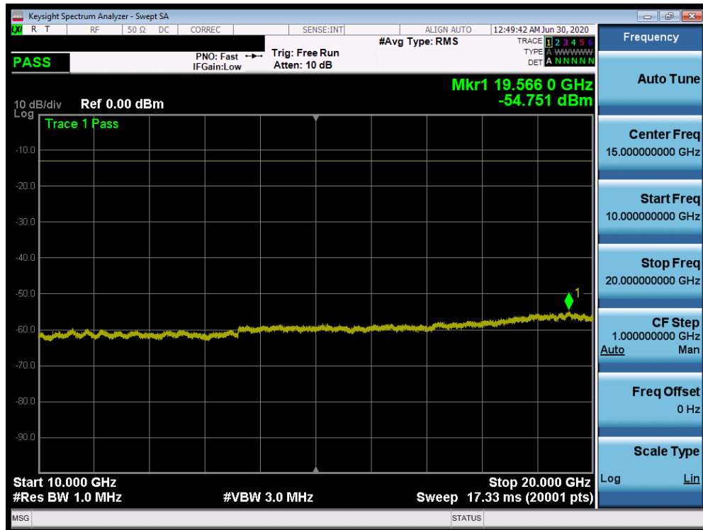
Plot 7-344. Conducted Spurious Plot (n25/2 - 20MHz DFT-s-OFDM-QPSK - RB Size 1, RB Offset 1 - Mid Channel)
