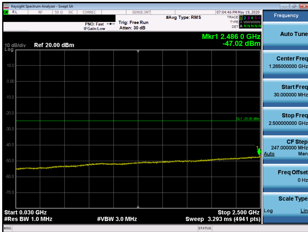
Plot 7-360. Conducted Spurious Plot (Band 7 - 20.0MHz QPSK - RB Size 1, RB Offset 0 - Mid Channel)
