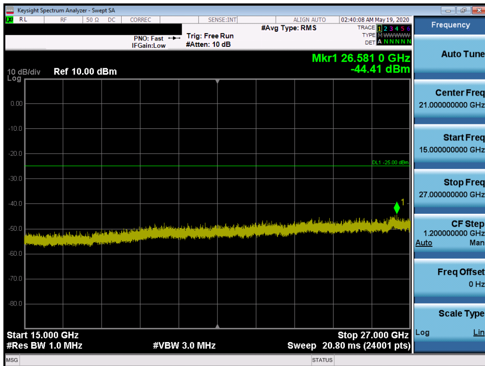
Plot 7-371. Conducted Spurious Plot (Band 41 PC2 - 20.0MHz QPSK - RB Size 1, RB Offset 0 - Mid Channel)
