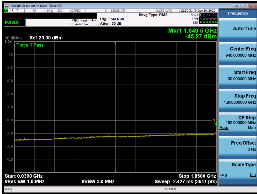
Plot 7-339. Conducted Spurious Plot (n25/2 - 20MHz DFT-s-OFDM-QPSK - RB Size 1, RB Offset 1 - Low Channel)
