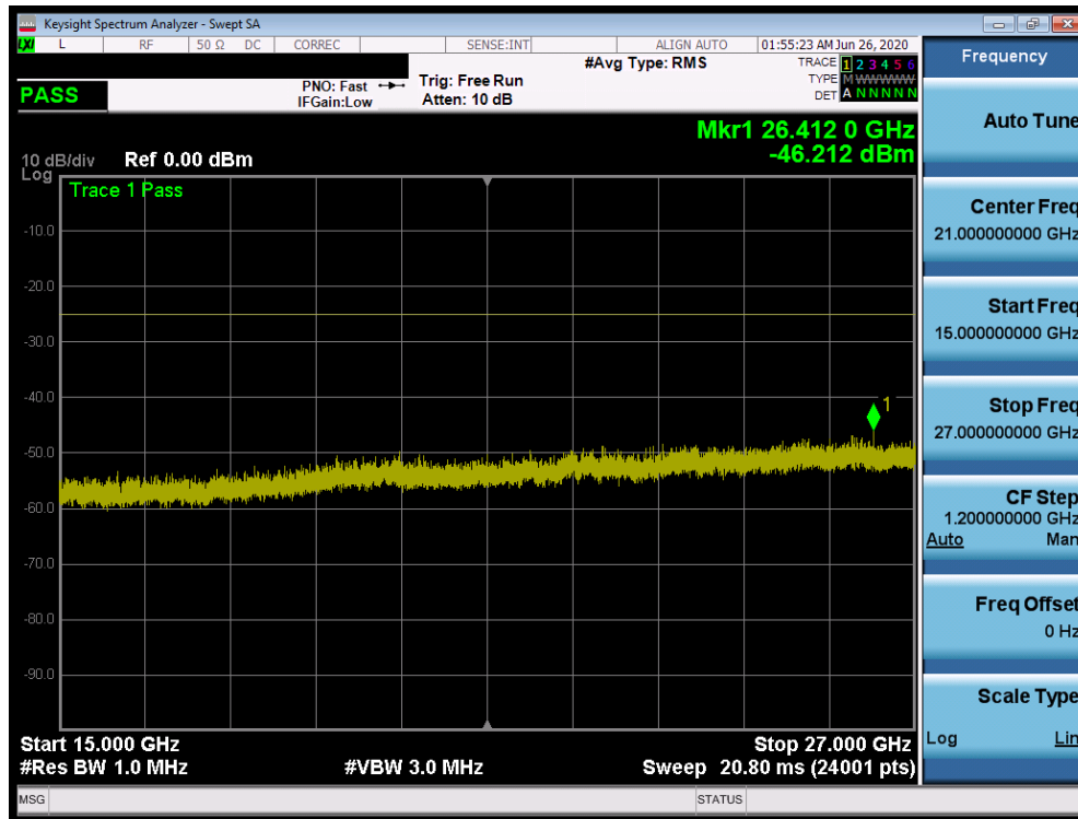
Plot 7-377. Conducted Spurious Plot (n41 - 100MHz DFT-s-OFDM-QPSK - RB Size 1, RB Offset 1 - Low Channel)
