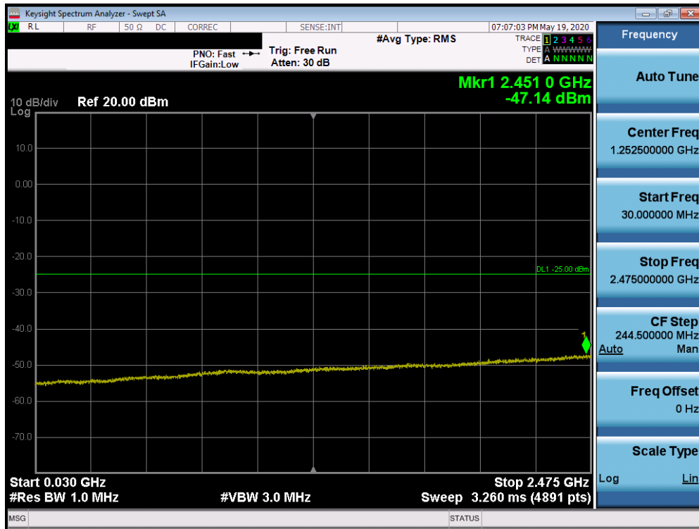
Plot 7-357. Conducted Spurious Plot (Band 7 - 20.0MHz QPSK - RB Size 1, RB Offset 0 - Low Channel)
