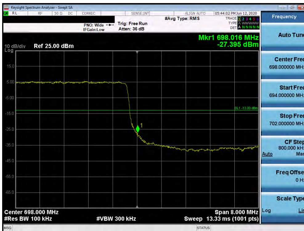
Plot 7-395. Upper Band Edge Plot (n71 - 10MHz DFT-s-OFDM-QPSK - Full RB Configuration)
