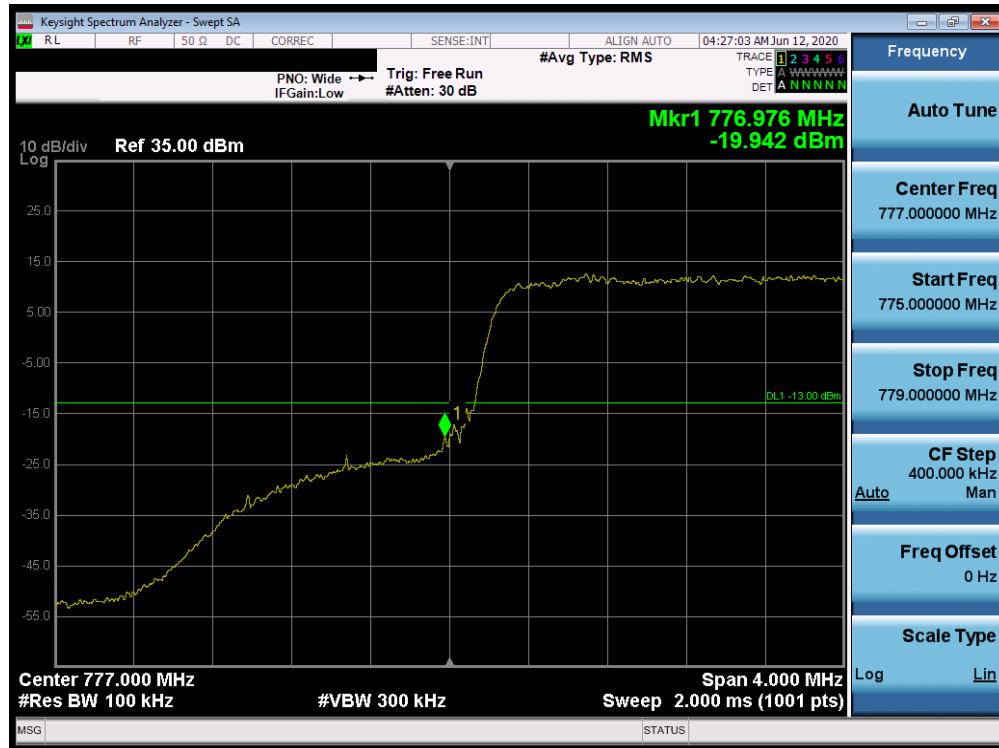
Plot 7-408. Lower Band Edge Plot (Band 13 - 5.0MHz QPSK - Full RB Configuration)
