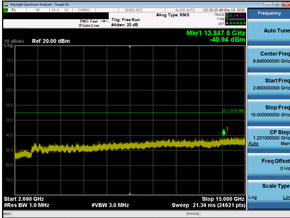
Plot 7-370. Conducted Spurious Plot (Band 41 PC2 - 20.0MHz QPSK - RB Size 1, RB Offset 0 - Mid Channel)
