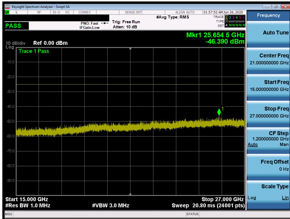
Plot 7-380. Conducted Spurious Plot (n41 - 100MHz DFT-s-OFDM-QPSK - RB Size 1, RB Offset 1 - Mid Channel)
