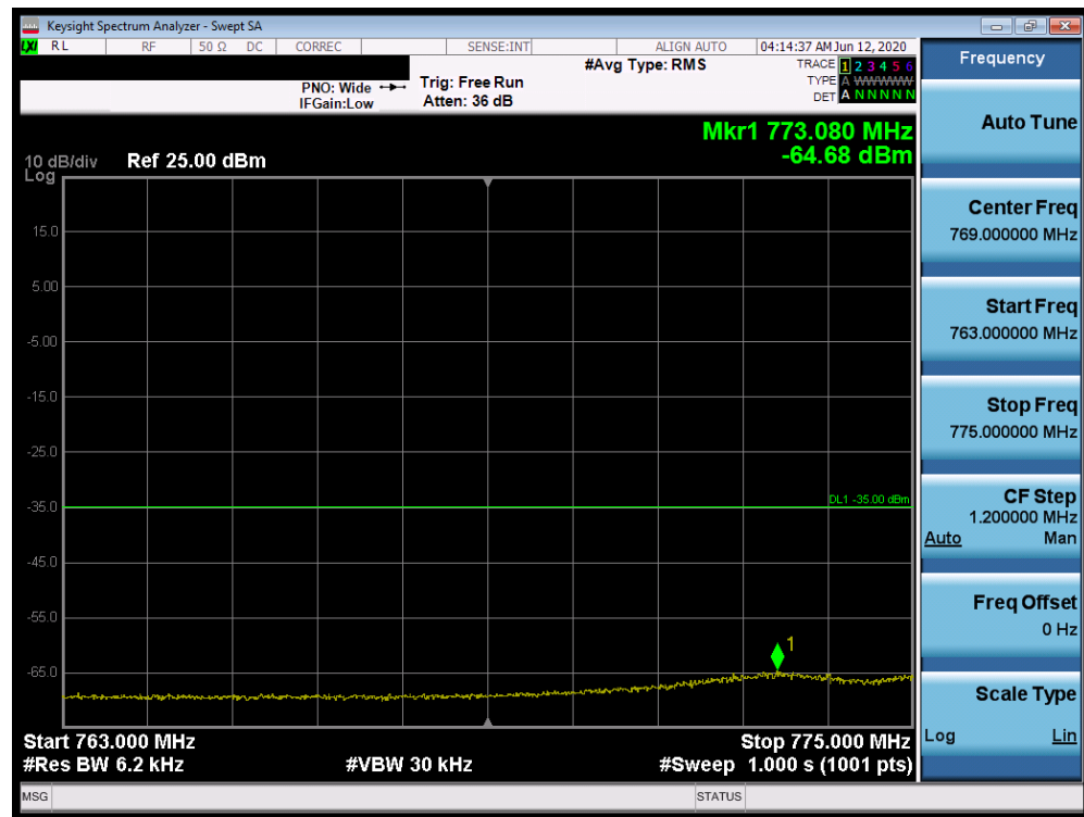
Plot 7-413. Lower Emission Mask Plot (Band 13 - 10.0MHz QPSK - Full RB Configuration)
