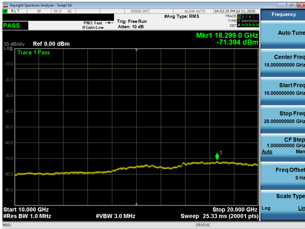
Plot 7-347. Conducted Spurious Plot (n25/2 - 20MHz DFT-s-OFDM-QPSK - RB Size 1, RB Offset 1 - High Channel)
