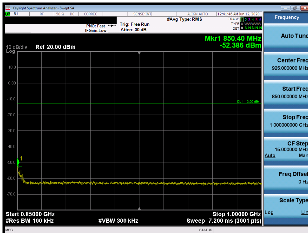
Plot 7-687. Conducted Spurious Plot (Band 5 - 10.0MHz QPSK - PCC 1/0 SCC 1/49 - High Channel)
