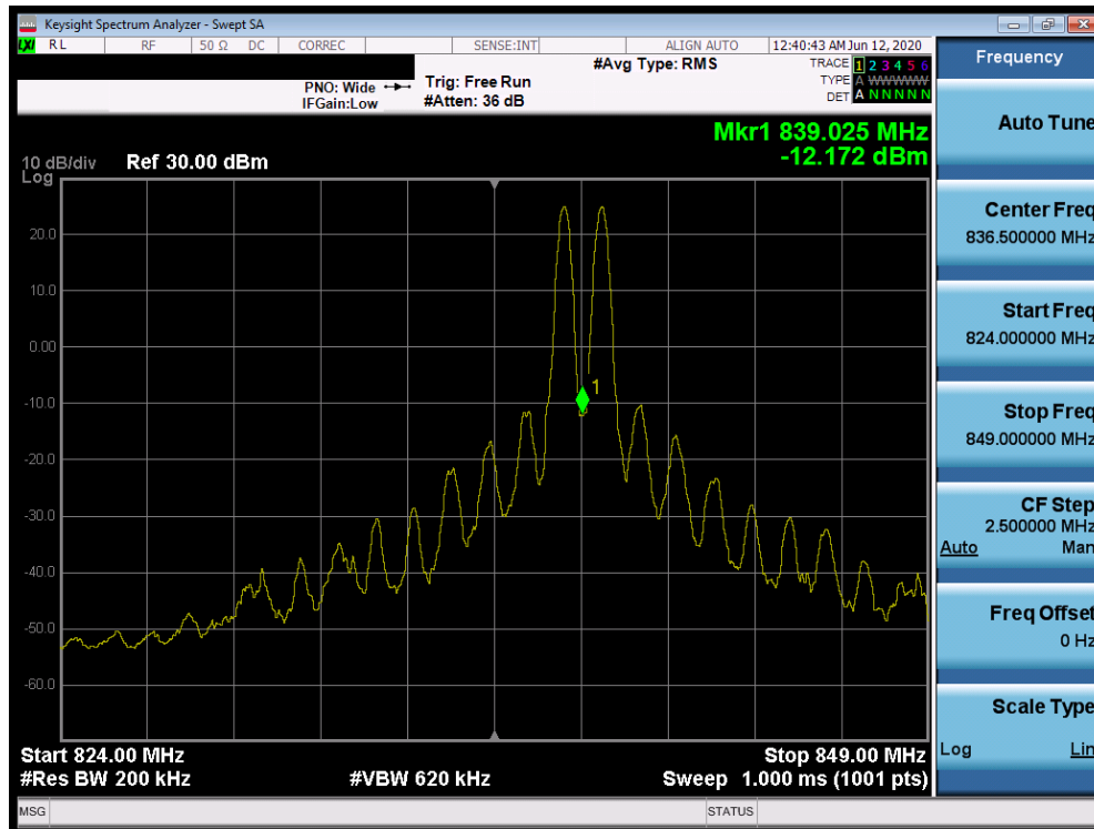
Plot 7-686. Conducted Spurious Plot (Band 5 - 10.0MHz QPSK - PCC 1/0 SCC 1/49 - High Channel)
