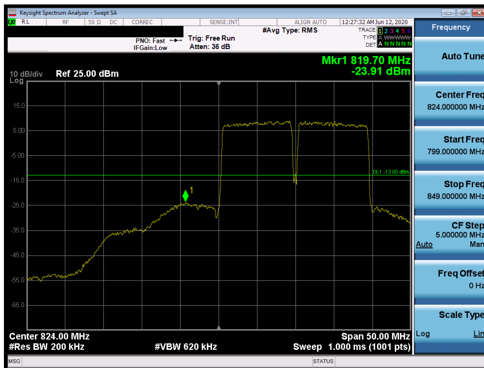
Plot 7-689. Lower Band Edge Plot (Band 5 QPSK – PCC:10 MHz SCC:10 MHz – Full RB)
