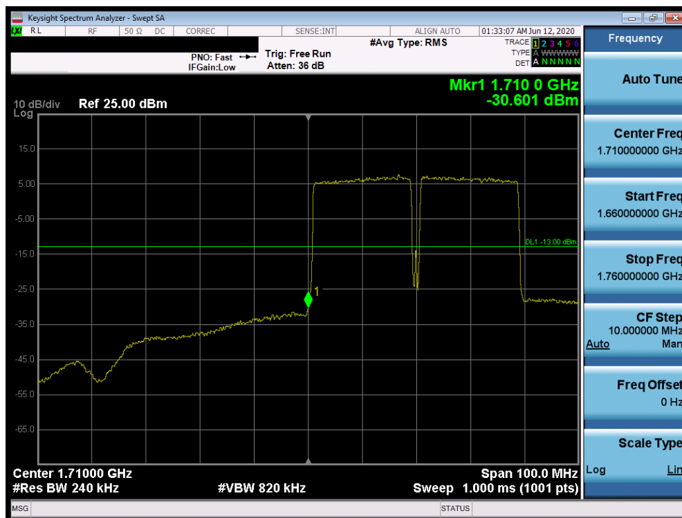
Plot 7-703. Lower Band Edge Plot (Band 66 QPSK – PCC:20 MHz SCC:20 MHz – Full RB)
