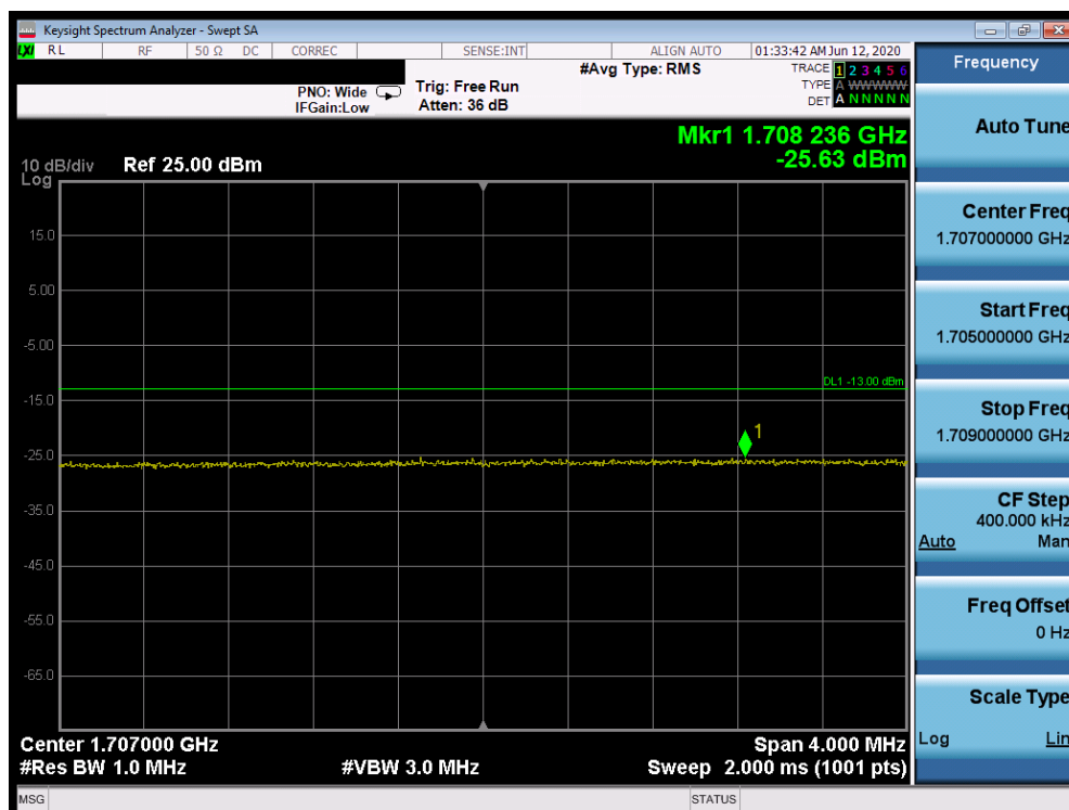
Plot 7-704. Extended Lower Band Edge Plot (Band 66 QPSK – PCC:20 MHz SCC:20 MHz – Full RB)
