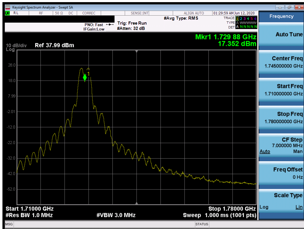
Plot 7-692. Conducted Spurious Plot (Band 66 – 20.0MHz QPSK – PCC 1/99 SCC 1/0 – Low Channel)
