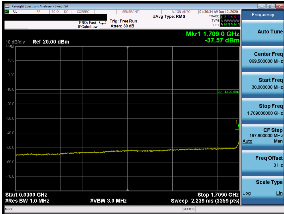
Plot 7-691. Conducted Spurious Plot (Band 66 – 20.0MHz QPSK – PCC 1/99 SCC 1/0 – Low Channel)
