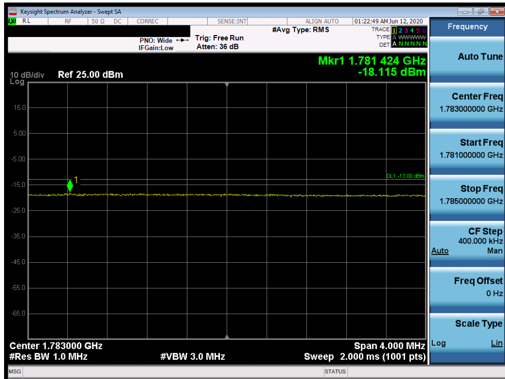
Plot 7-706. Extended Upper Band Edge Plot (Band 66 QPSK – PCC:20 MHz SCC:20 MHz – Full RB)
