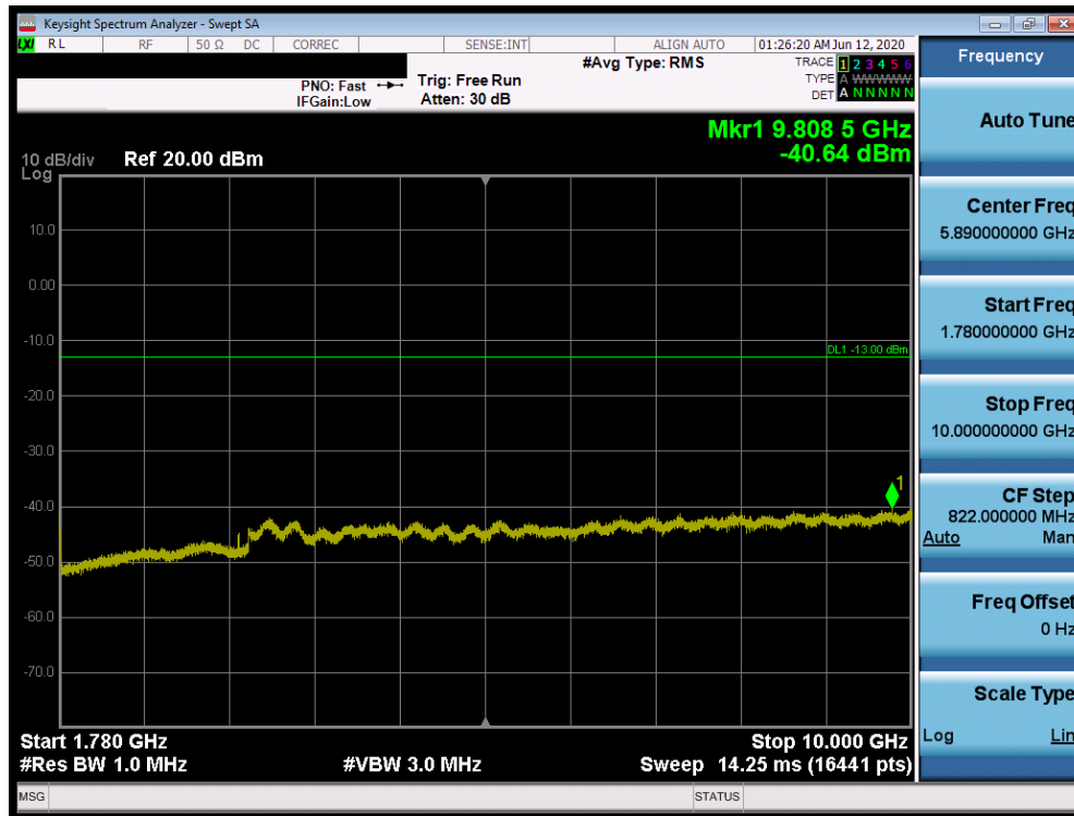
Plot 7-697. Conducted Spurious Plot (Band 66 – 20.0MHz QPSK – PCC 1/99 SCC 1/0 – Mid Channel)
