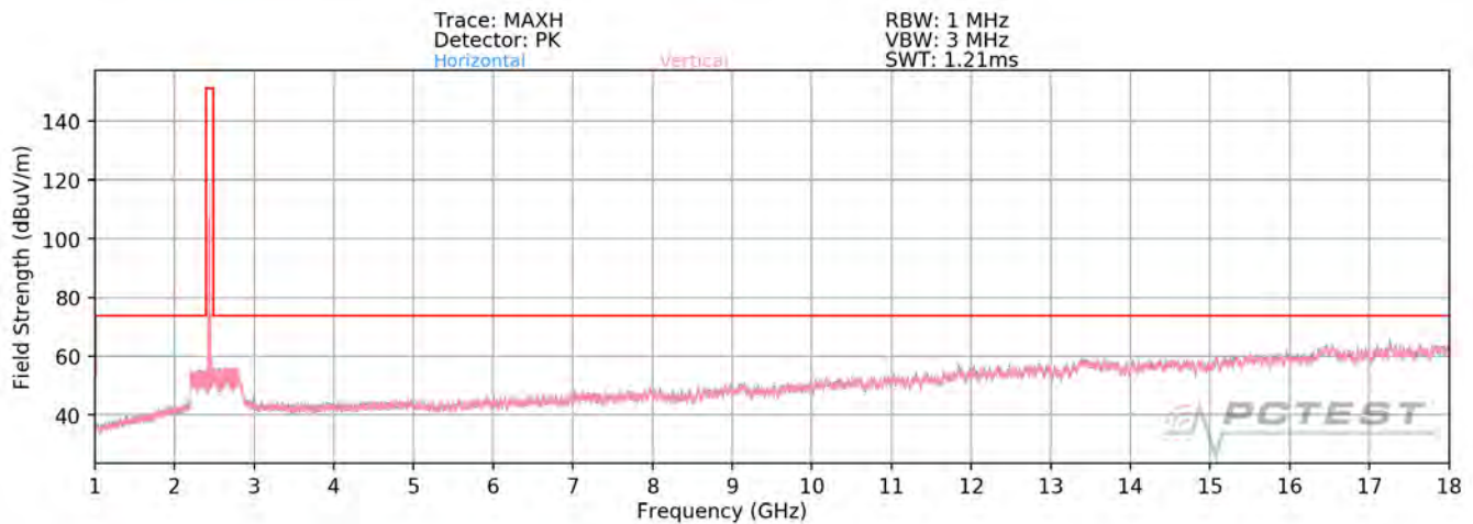
Plot 7-78. Radiated Spurious Plot above 1GHz MIMO (802.11ax OFDMA – 26 Tones – Ch. 6)
