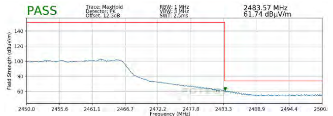
Plot 7-110. Radiated Restricted Upper Band Edge Measurement SISO ANT2 (Peak - 242 Tones)
