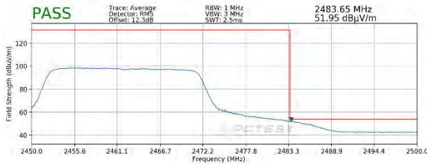
Plot 7-125. Radiated Restricted Upper Band Edge Measurement MIMO (Average – 242 Tones)
