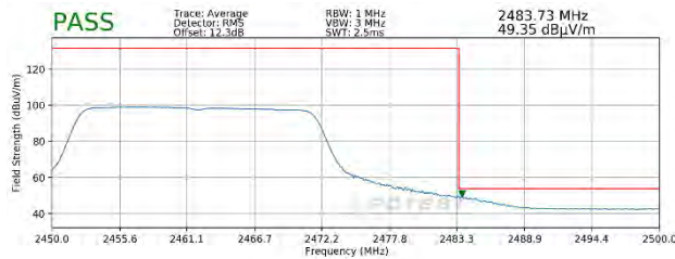
Plot 7-97. Radiated Restricted Upper Band Edge Measurement SISO ANT1 (Average – 242 Tones)
