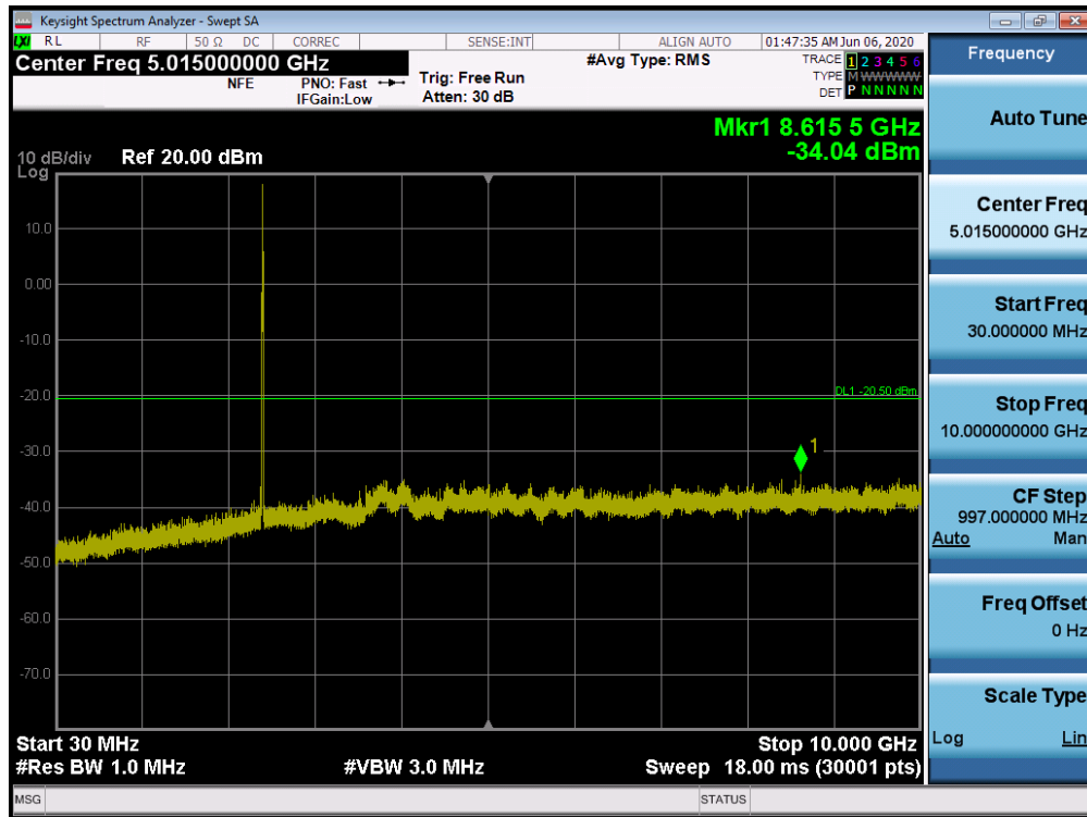
Plot 7-51. Conducted Spurious Plot SISO ANT2 (802.11ax OFDMA – 26 Tones – Ch. 1)
