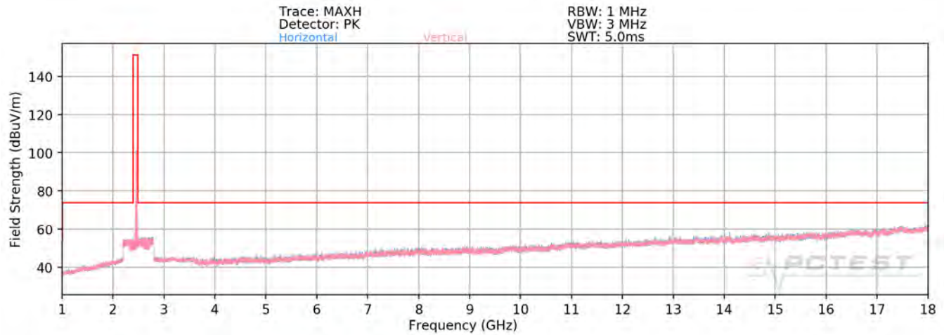
Plot 7-75. Radiated Spurious Plot above 1GHz SISO ANT2 (802.11ax OFDMA – 242 Tones – Ch. 11)
