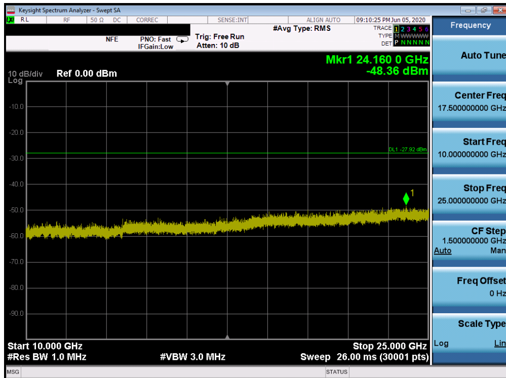
Plot 7-50. Conducted Spurious Plot SISO ANT1 (802.11ax OFDMA – 242 Tones – Ch. 11)
