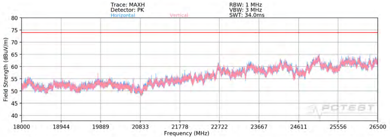
Plot 7-83. Radiated Spurious Plot above 18GHz MIMO (802.11ax OFDMA – 26 Tones)
