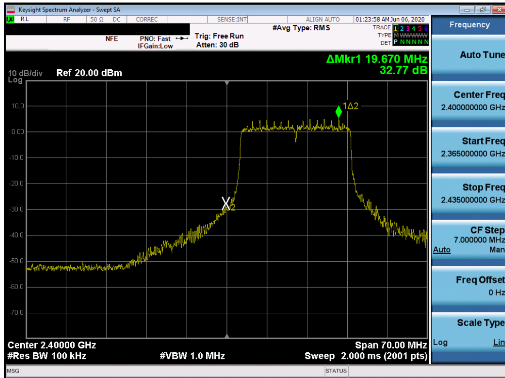
Plot 7-34. Band Edge Plot SISO ANT2 (802.11ax OFDMA – 242 Tones – Ch. 1)
