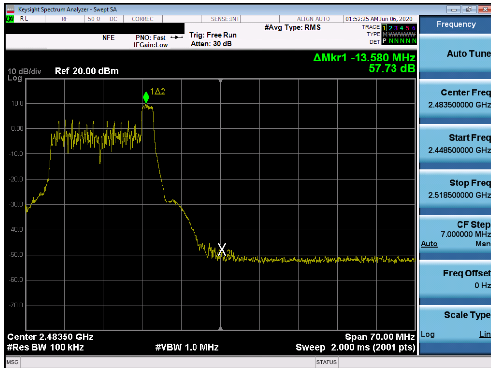
Plot 7-33. Band Edge Plot SISO ANT2 (802.11ax OFDMA – 106 Tones – Ch. 11)
