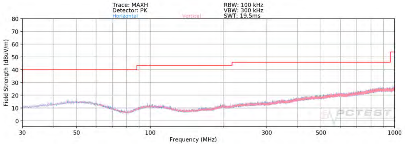
Plot 7-127. Radiated Spurious Plot below 1GHz MIMO (106 Tones)
