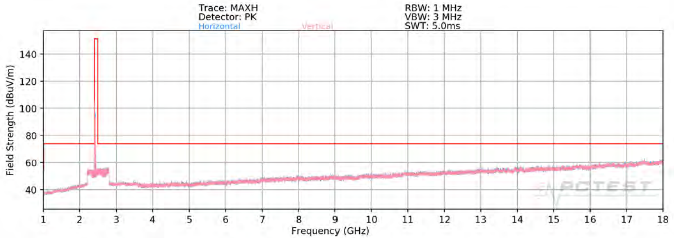
Plot 7-70. Radiated Spurious Plot above 1GHz SISO ANT2 (802.11ax OFDMA – 26 Tones – Ch. 1)
