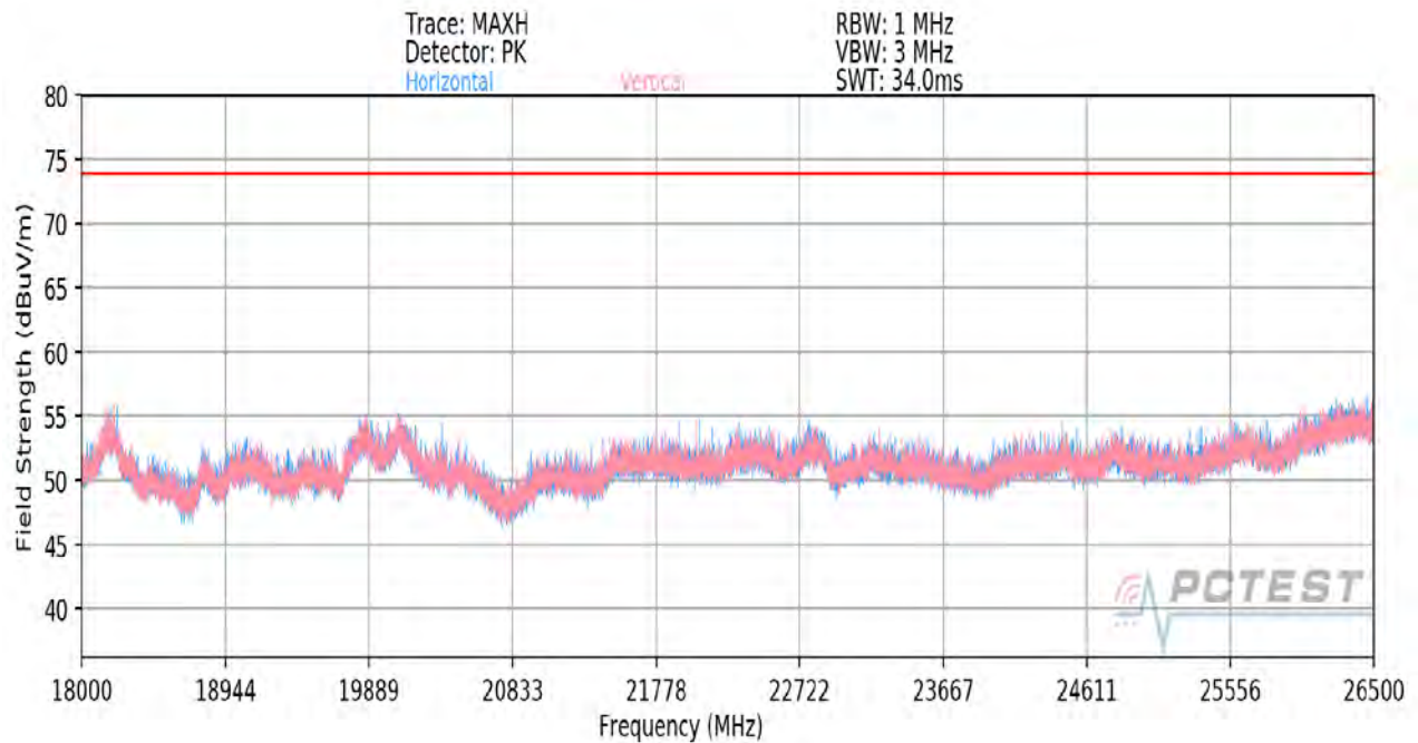
Plot 7-76. Radiated Spurious Plot above 18GHz SISO ANT2 (802.11ax OFDMA – 26 Tones)
