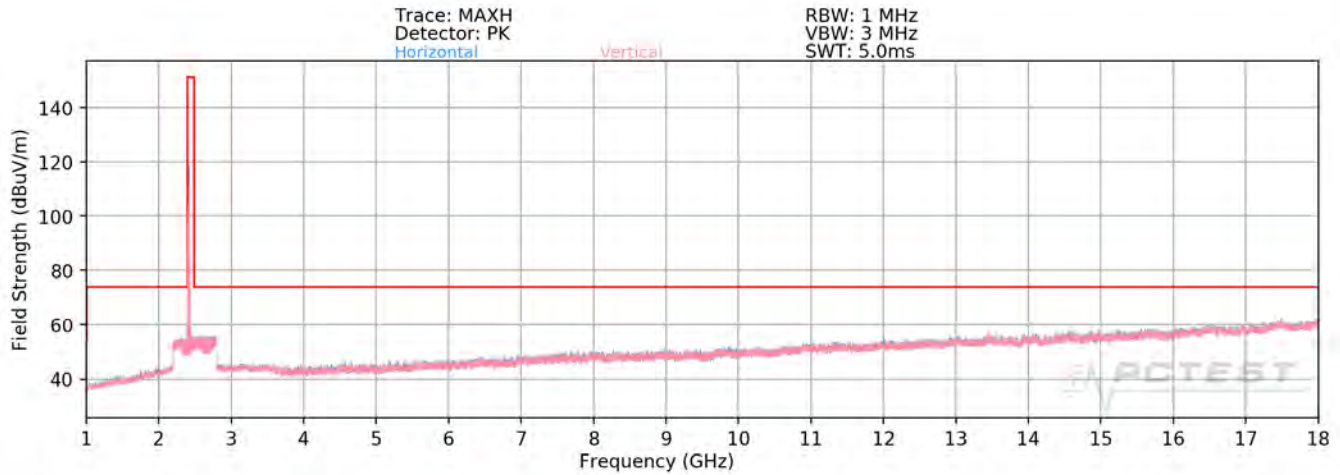
Plot 7-63. Radiated Spurious Plot above 1GHz SISO ANT1 (802.11ax OFDMA – 26 Tones – Ch. 1)
