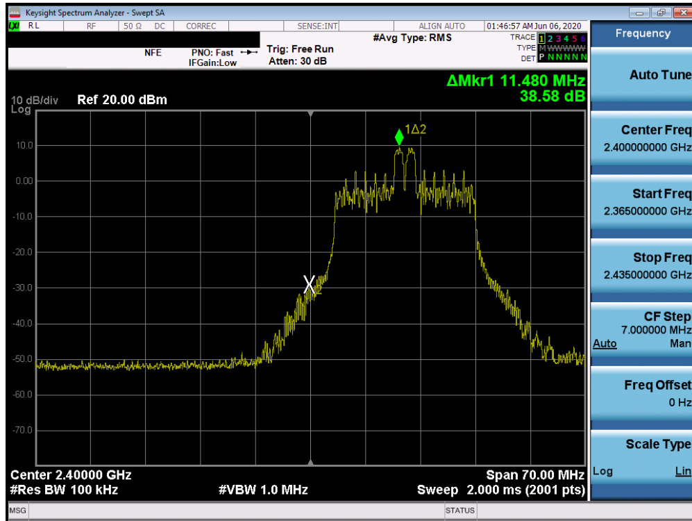
Plot 7-32. Band Edge Plot SISO ANT2 (802.11ax OFDMA – 106 Tones – Ch. 1)
