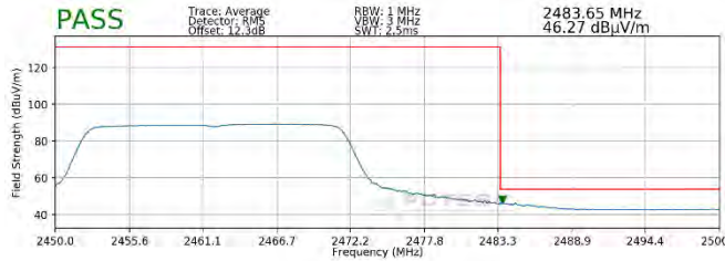
Plot 7-111. Radiated Restricted Upper Band Edge Measurement SISO ANT2 (Average – 242 Tones)
