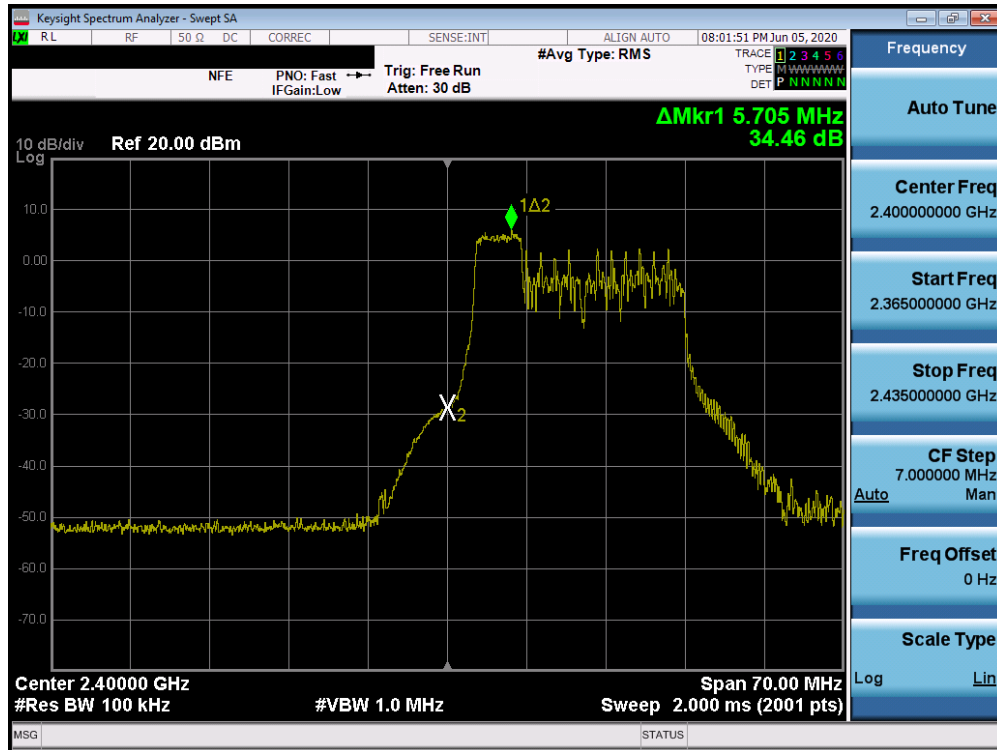
Plot 7-25. Band Edge Plot SISO ANT1 (802.11ax OFDMA - 52 Tones - Ch. 1)
