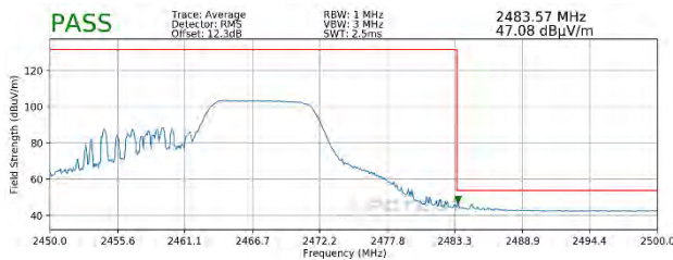
Plot 7-115. Radiated Restricted Upper Band Edge Measurement MIMO (Average – 106 Tones)
