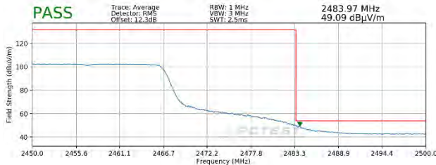
Plot 7-95. Radiated Restricted Upper Band Edge Measurement SISO ANT1 (Average - 242 Tones)
