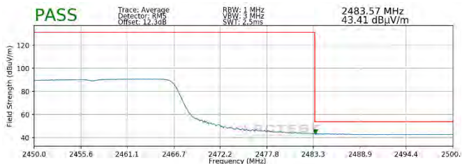
Plot 7-109. Radiated Restricted Upper Band Edge Measurement SISO ANT2 (Average - 242 Tones)
