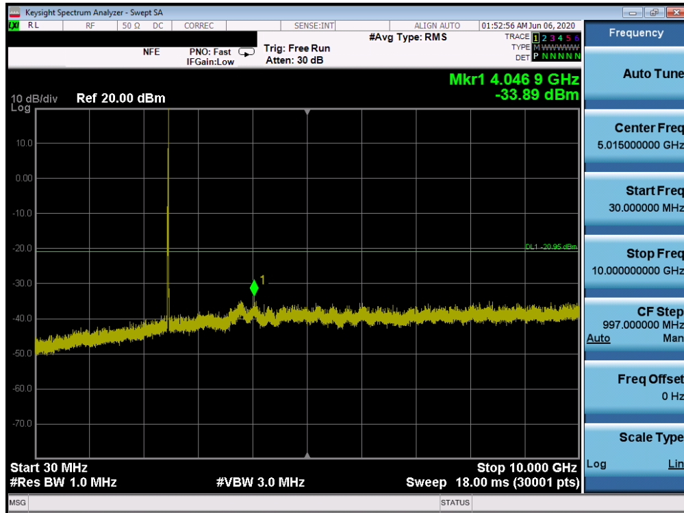
Plot 7-55. Conducted Spurious Plot SISO ANT2 (802.11ax OFDMA – 26 Tones – Ch. 11)
