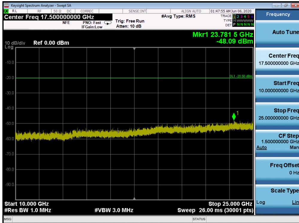
Plot 7-52. Conducted Spurious Plot SISO ANT2 (802.11ax OFDMA – 26 Tones – Ch. 1)
