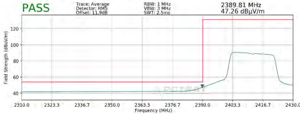
Plot 7-103. Radiated Restricted Lower Band Edge Measurement SISO ANT2 (Average - 242 Tones)
