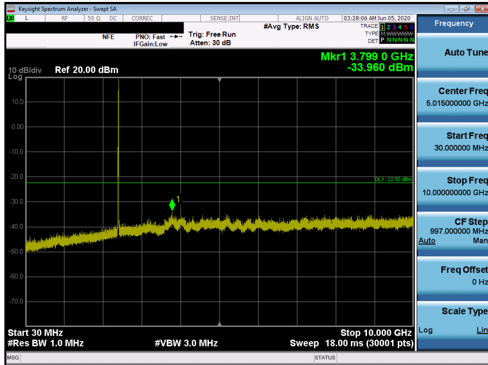
Plot 7-39. Conducted Spurious Plot SISO ANT1 (802.11ax OFDMA – 26 Tones – Ch. 1)
