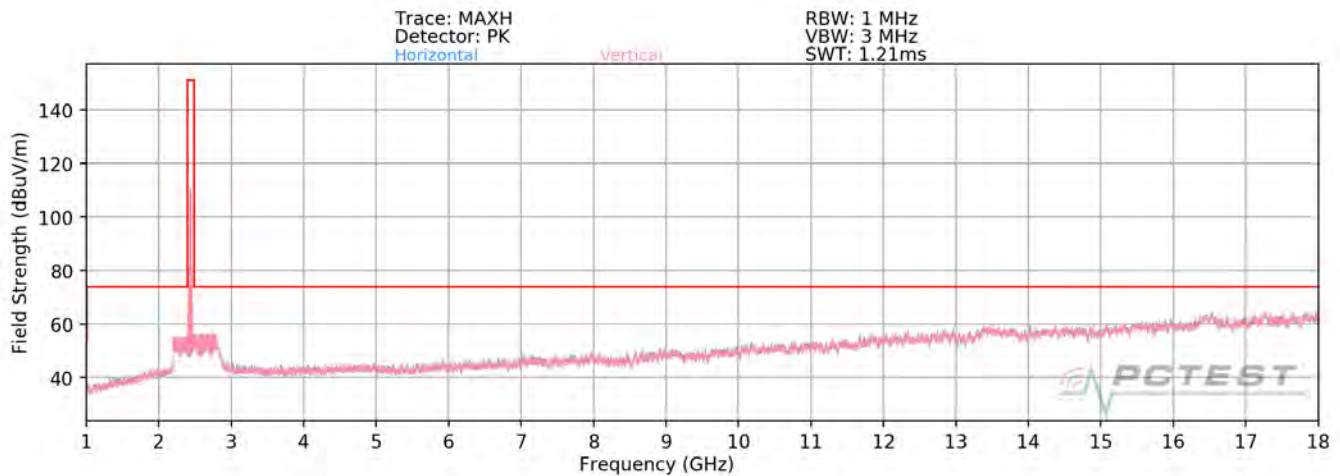
Plot 7-81. Radiated Spurious Plot above 1GHz MIMO (802.11ax OFDMA – 242 Tones – Ch. 6)
