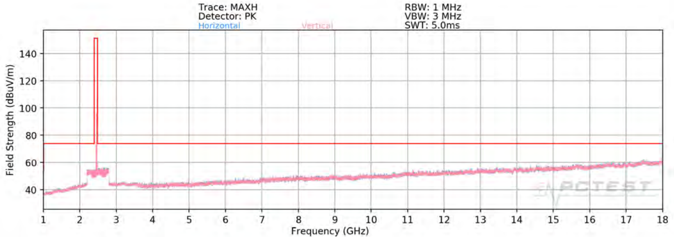
Plot 7-72. Radiated Spurious Plot above 1GHz SISO ANT2 (802.11ax OFDMA – 26 Tones – Ch. 11)
