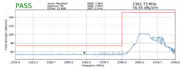
Plot 7-100. Radiated Restricted Lower Band Edge Measurement SISO ANT2 (Peak – 106 Tones)
