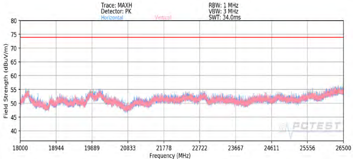
Plot 7-69. Radiated Spurious Plot above 18GHz SISO ANT1 (802.11ax OFDMA – 26 Tones)
