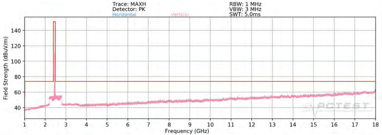
Plot 7-68. Radiated Spurious Plot above 1GHz SISO ANT1 (802.11ax OFDMA – 242 Tones – Ch. 11)
