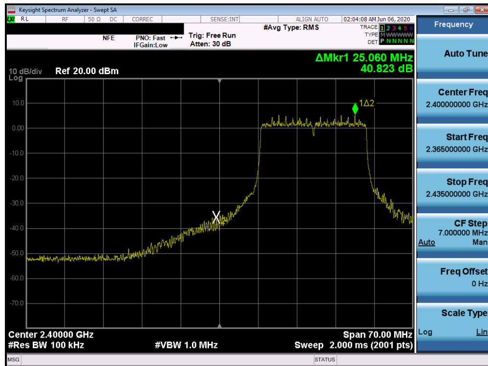
Plot 7-35. Band Edge Plot SISO ANT2 (802.11ax OFDMA – 242 Tones – Ch. 2)
