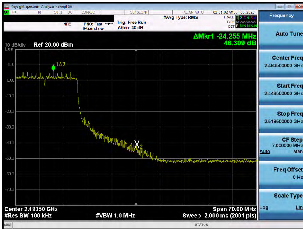
Plot 7-37. Band Edge Plot SISO ANT2 (802.11ax OFDMA – 242 Tones – Ch. 10)
