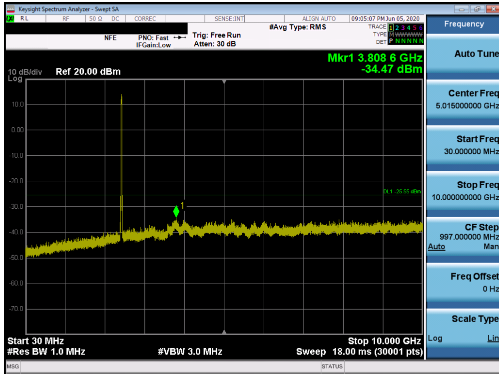
Plot 7-47. Conducted Spurious Plot SISO ANT1 (802.11ax OFDMA – 242 Tones – Ch. 6)
