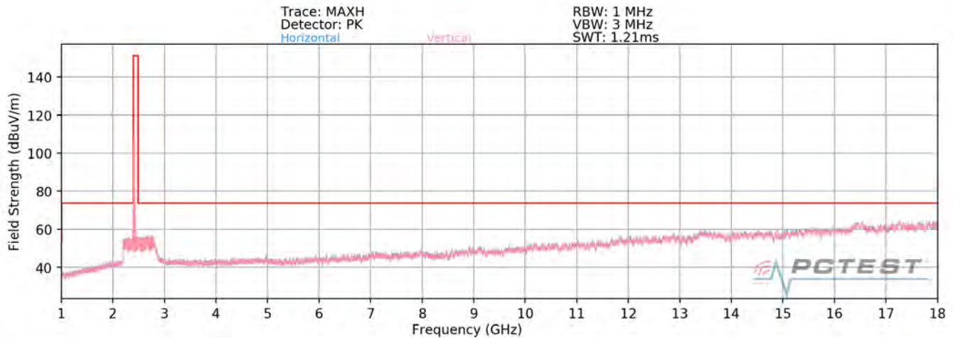
Plot 7-80. Radiated Spurious Plot above 1GHz MIMO (802.11ax OFDMA – 242 Tones – Ch. 1)
