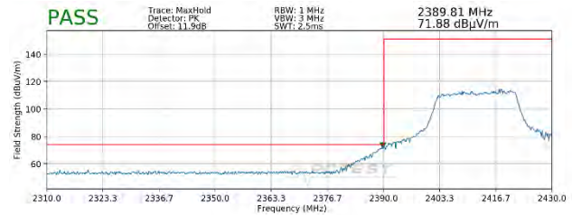
Plot 7-90. Radiated Restricted Lower Band Edge Measurement SISO ANT1 (Peak – 242 Tones)
