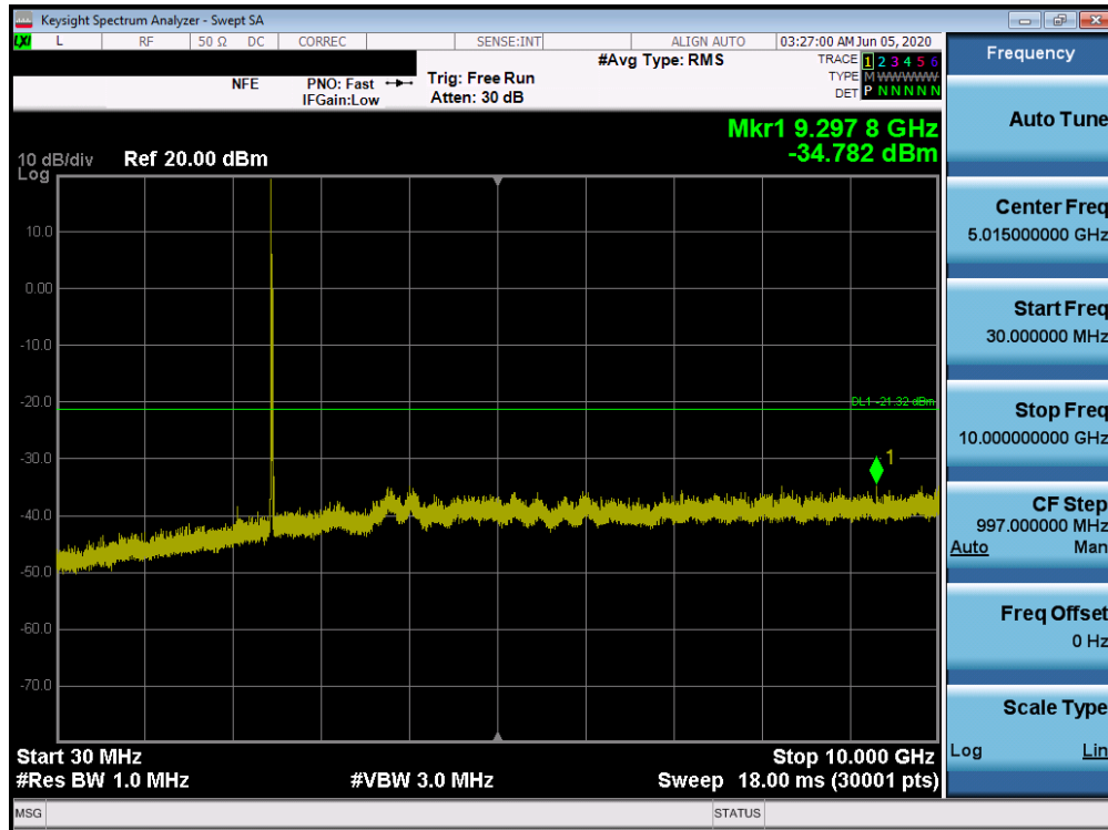
Plot 7-43. Conducted Spurious Plot SISO ANT1 (802.11ax OFDMA – 26 Tones – Ch. 11)
