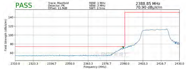
Plot 7-118. Radiated Restricted Lower Band Edge Measurement MIMO (Peak - 242 Tones)
