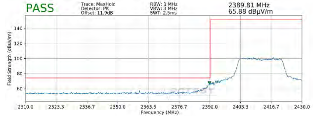
Plot 7-104. Radiated Restricted Lower Band Edge Measurement SISO ANT2 (Peak - 242 Tones)
