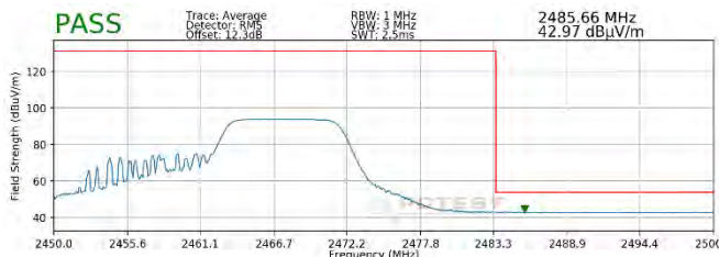
Plot 7-101. Radiated Restricted Upper Band Edge Measurement SISO ANT2 (Average – 106 Tones)
