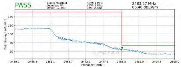
Plot 7-122. Radiated Restricted Upper Band Edge Measurement MIMO (Peak - 242 Tones)
