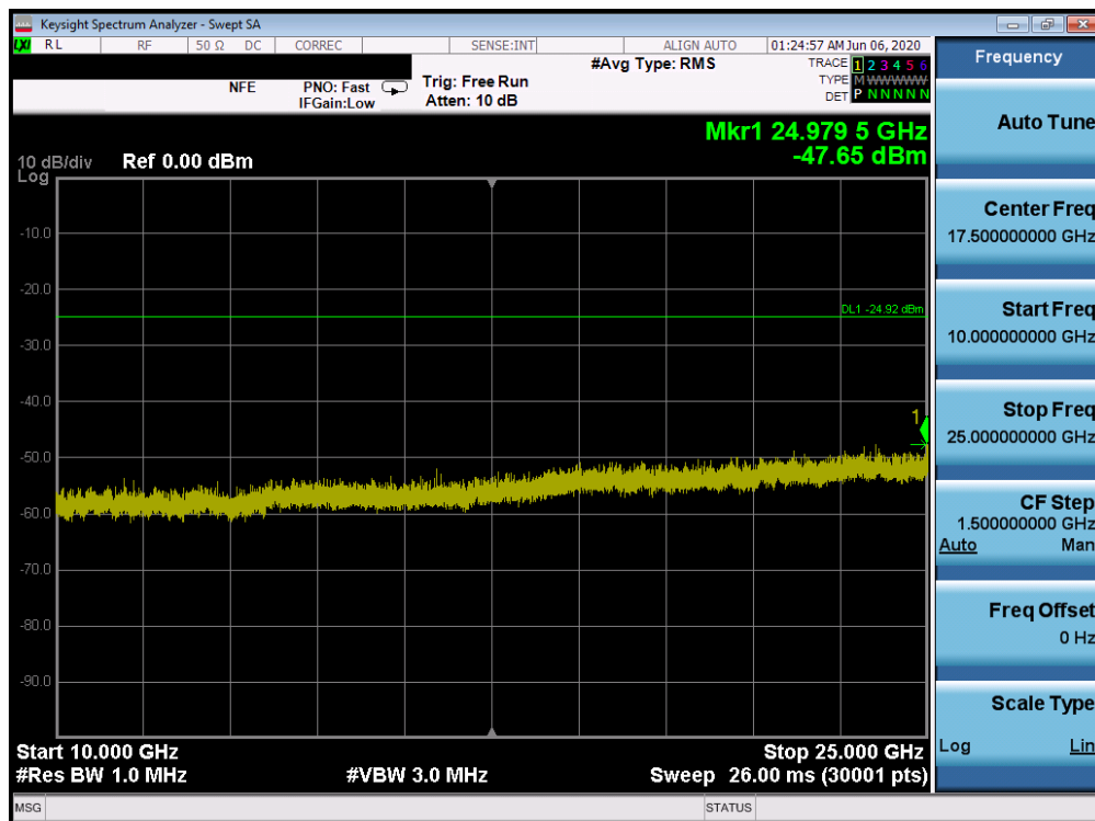
Plot 7-58. Conducted Spurious Plot SISO ANT2 (802.11ax OFDMA – 242 Tones – Ch. 1)
