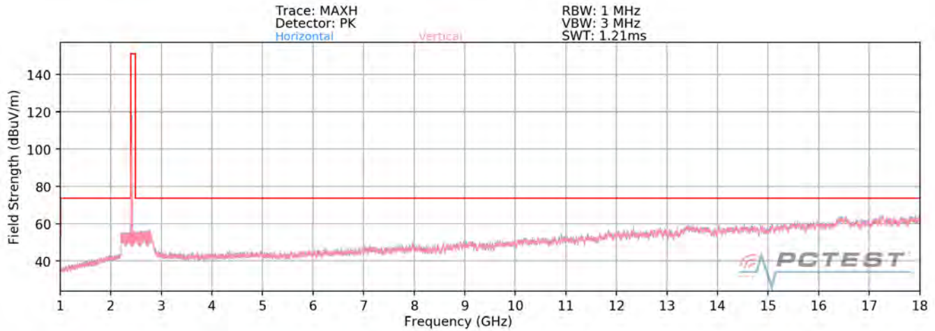
Plot 7-77. Radiated Spurious Plot above 1GHz MIMO (802.11ax OFDMA – 26 Tones – Ch. 1)
