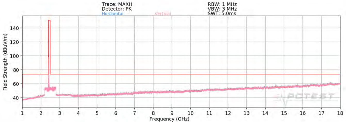
Plot 7-73. Radiated Spurious Plot above 1GHz SISO ANT2 (802.11ax OFDMA – 242 Tones – Ch. 1)
