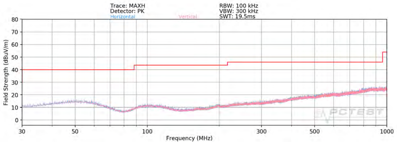
Plot 7-128. Radiated Spurious Plot below 1GHz MIMO (242 Tones)
