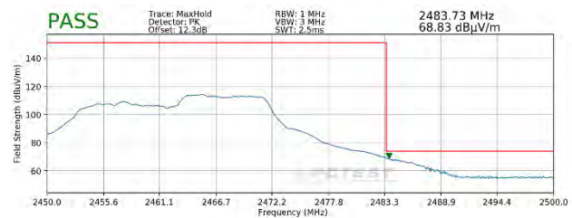
Plot 7-88. Radiated Restricted Upper Band Edge Measurement SISO ANT1 (Peak – 106 Tones)
