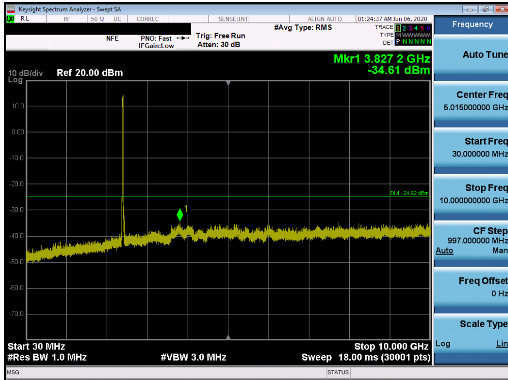
Plot 7-57. Conducted Spurious Plot SISO ANT2 (802.11ax OFDMA – 242 Tones – Ch. 1)
