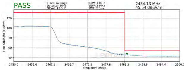
Plot 7-93. Radiated Restricted Upper Band Edge Measurement SISO ANT1 (Average - 242 Tones)
