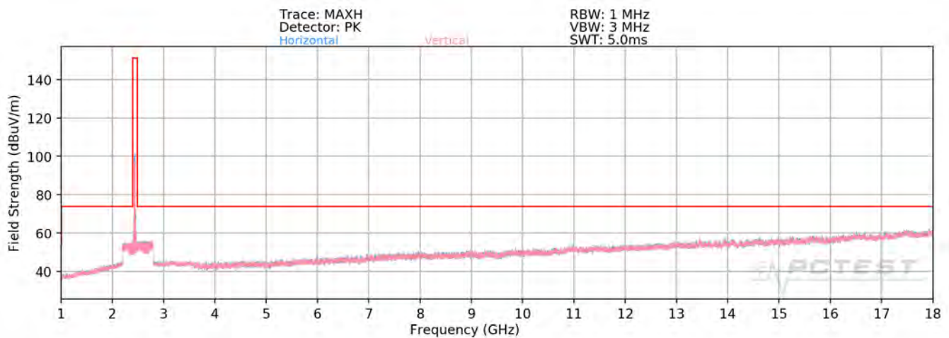
Plot 7-74. Radiated Spurious Plot above 1GHz SISO ANT2 (802.11ax OFDMA – 242 Tones – Ch. 6)
