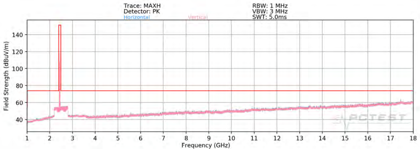
Plot 7-64. Radiated Spurious Plot above 1GHz SISO ANT1 (802.11ax OFDMA – 26 Tones – Ch. 6)
