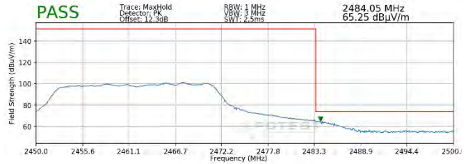
Plot 7-112. Radiated Restricted Upper Band Edge Measurement SISO ANT2 (Peak – 242 Tones)
