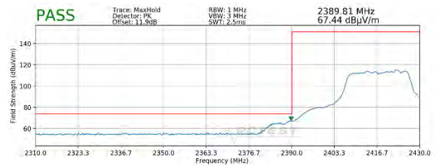
Plot 7-92. Radiated Restricted Lower Band Edge Measurement SISO ANT1 (Peak – 242 Tones)
