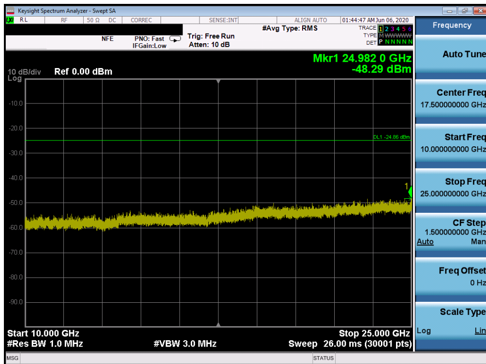
Plot 7-62. Conducted Spurious Plot SISO ANT2 (802.11ax OFDMA – 242 Tones – Ch. 11)
