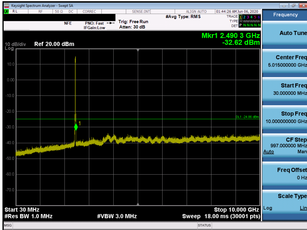
Plot 7-61. Conducted Spurious Plot SISO ANT2 (802.11ax OFDMA – 242 Tones – Ch. 11)
