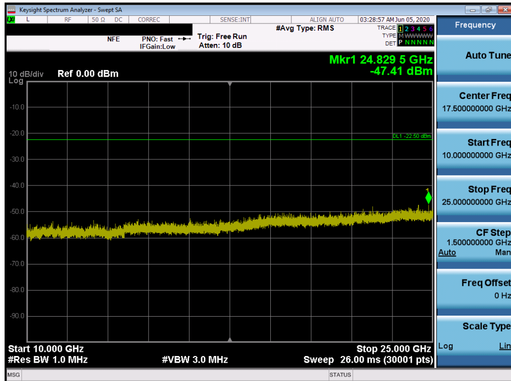
Plot 7-40. Conducted Spurious Plot SISO ANT1 (802.11ax OFDMA – 26 Tones – Ch. 1)
