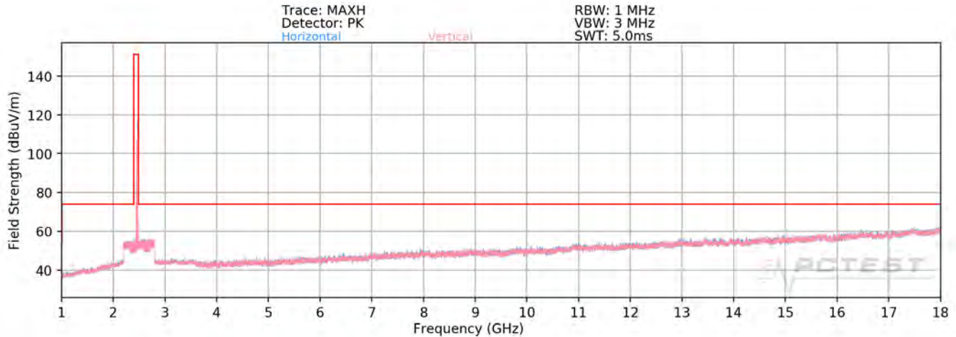
Plot 7-65. Radiated Spurious Plot above 1GHz SISO ANT1 (802.11ax OFDMA – 26 Tones – Ch. 11)
