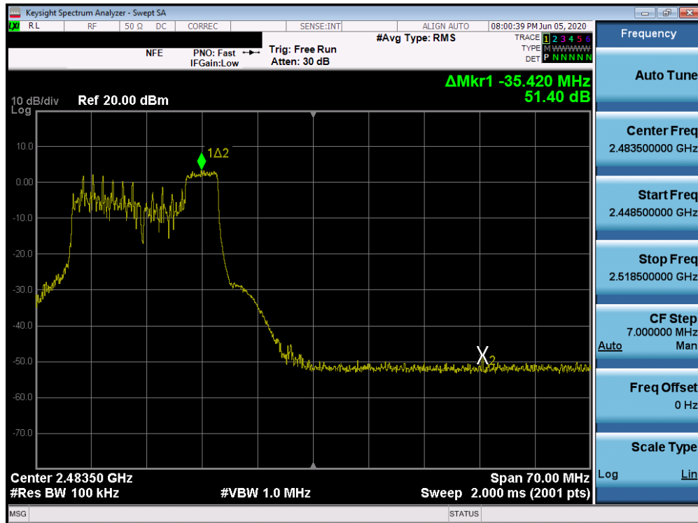
Plot 7-26. Band Edge Plot SISO ANT1 (802.11ax OFDMA - 52 Tones - Ch. 11)
