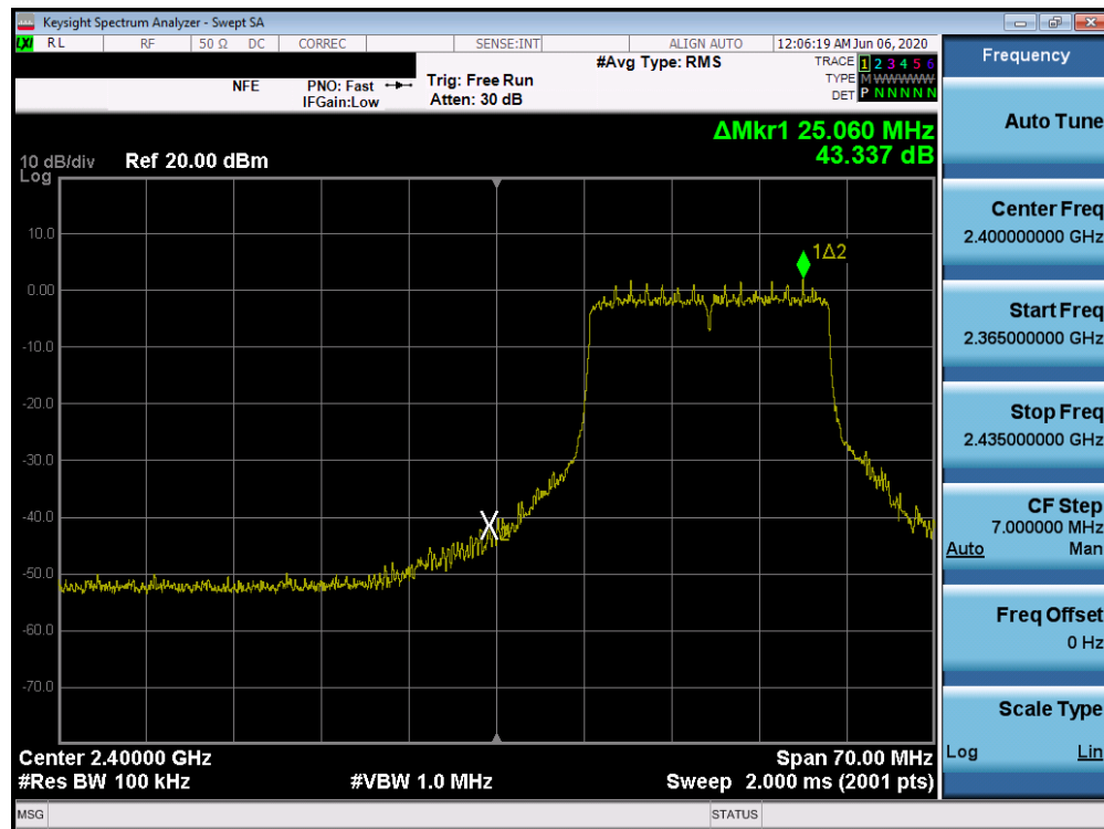
Plot 7-28. Band Edge Plot SISO ANT1 (802.11ax OFDMA – 242 Tones – Ch. 2)
