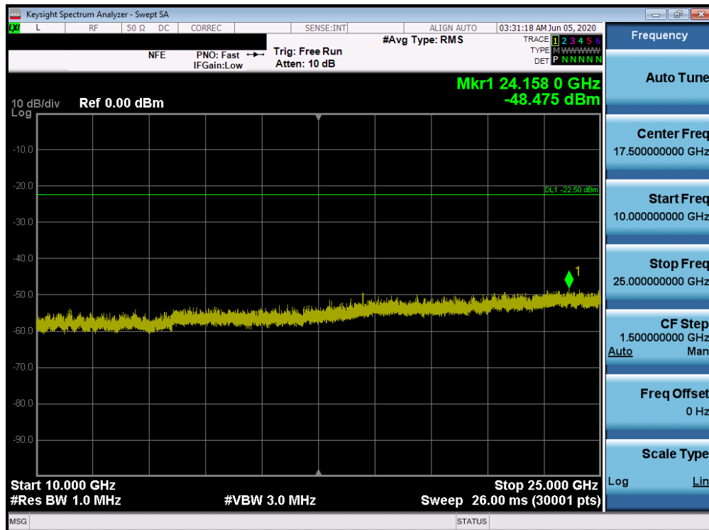
Plot 7-44. Conducted Spurious Plot SISO ANT1 (802.11ax OFDMA – 26 Tones – Ch. 11)
