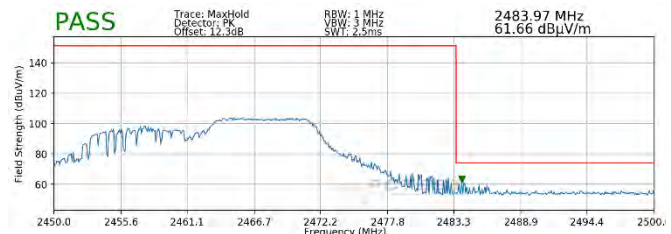
Plot 7-102. Radiated Restricted Upper Band Edge Measurement SISO ANT2 (Peak – 106 Tones)
