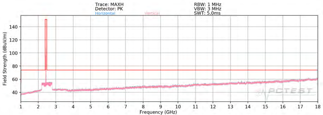
Plot 7-71. Radiated Spurious Plot above 1GHz SISO ANT2 (802.11ax OFDMA – 26 Tones – Ch. 6)
