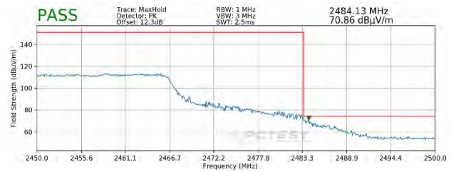
Plot 7-124. Radiated Restricted Upper Band Edge Measurement MIMO (Peak - 242 Tones)
