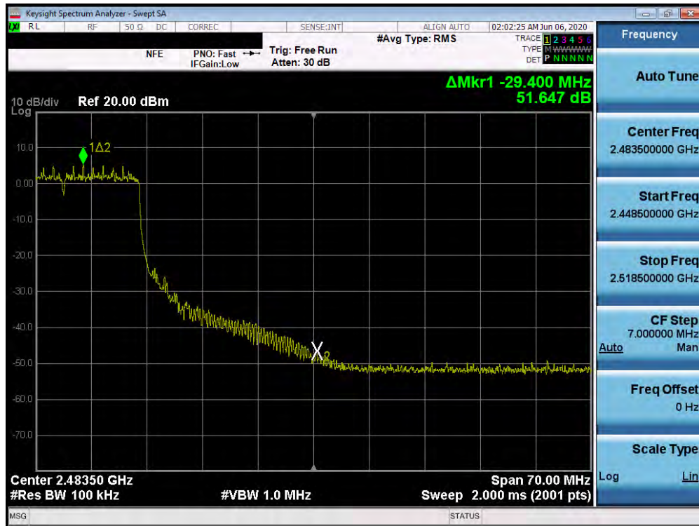
Plot 7-36. Band Edge Plot SISO ANT2 (802.11ax OFDMA – 242 Tones – Ch. 9)
