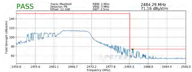
Plot 7-116. Radiated Restricted Upper Band Edge Measurement MIMO (Peak – 106 Tones)
