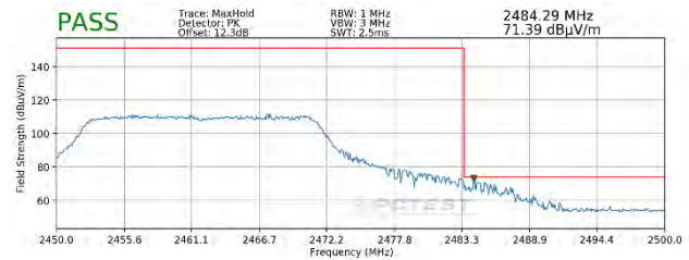
Plot 7-98. Radiated Restricted Upper Band Edge Measurement SISO ANT1 (Peak – 242 Tones)
