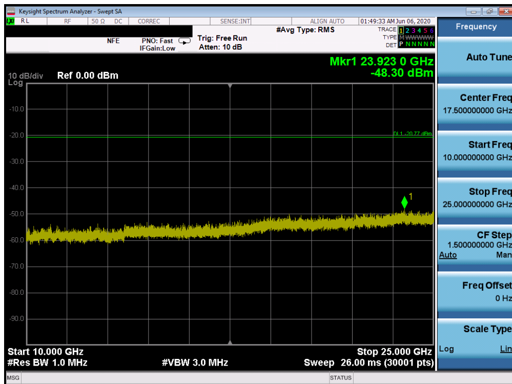
Plot 7-54. Conducted Spurious Plot SISO ANT2 (802.11ax OFDMA – 26 Tones – Ch. 6)
