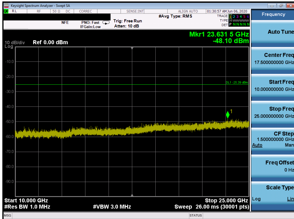
Plot 7-60. Conducted Spurious Plot SISO ANT2 (802.11ax OFDMA - 242 Tones - Ch. 6)
