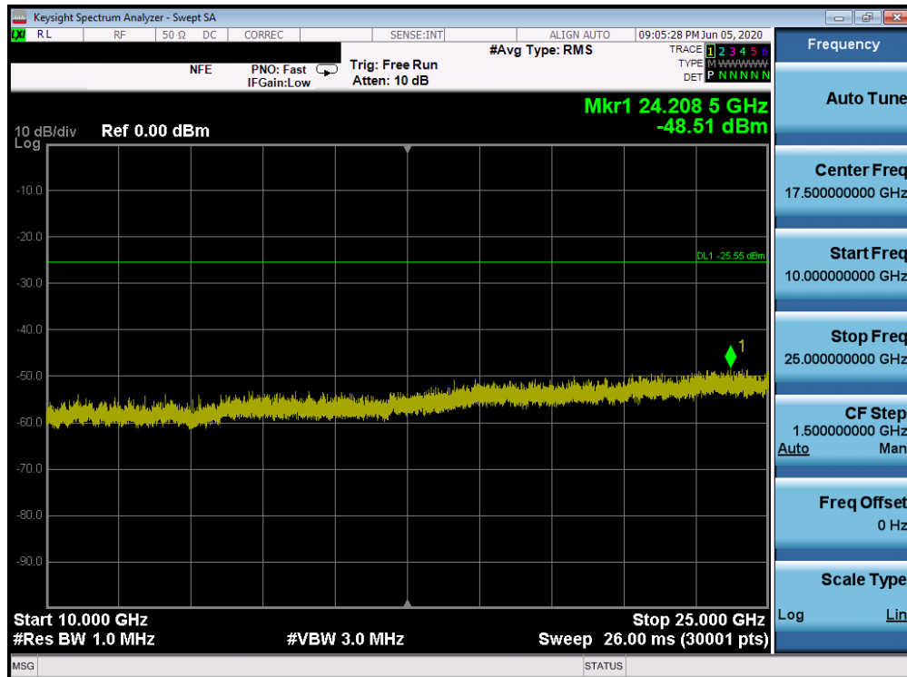
Plot 7-48. Conducted Spurious Plot SISO ANT1 (802.11ax OFDMA – 242 Tones – Ch. 6)
