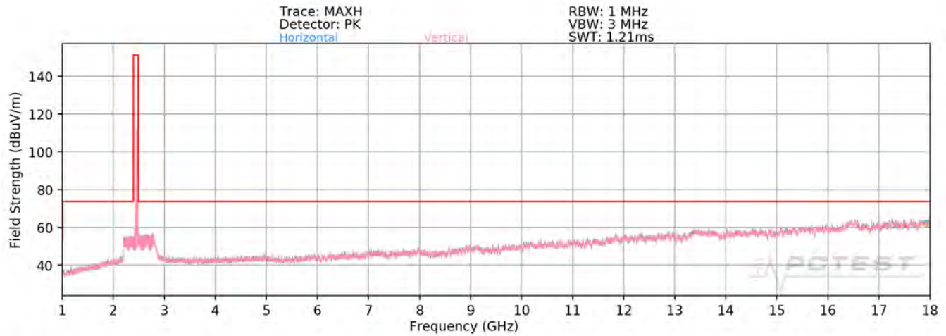
Plot 7-82. Radiated Spurious Plot above 1GHz MIMO (802.11ax OFDMA – 242 Tones – Ch. 11)
