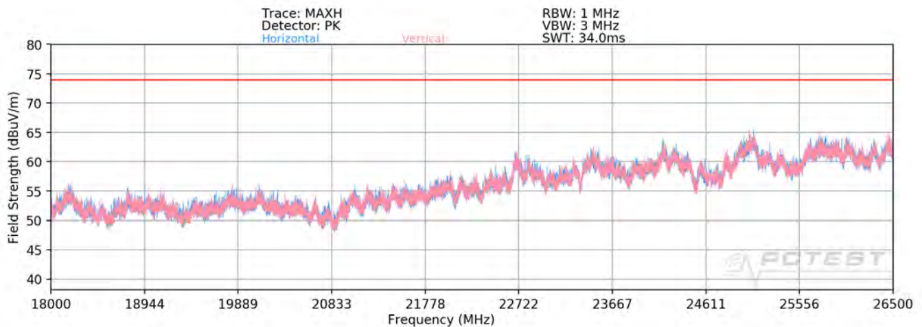
Plot 7-84. Radiated Spurious Plot above 18GHz MIMO (802.11ax OFDMA – 242 Tones)
