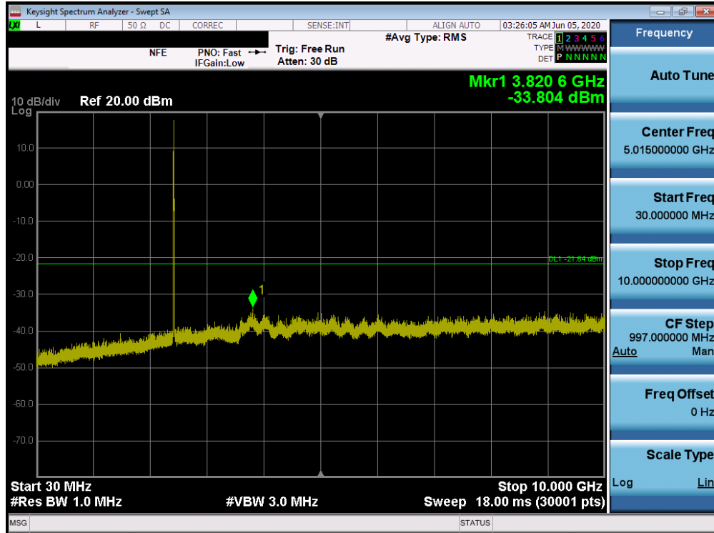
Plot 7-41. Conducted Spurious Plot SISO ANT1 (802.11ax OFDMA – 26 Tones – Ch. 6)
