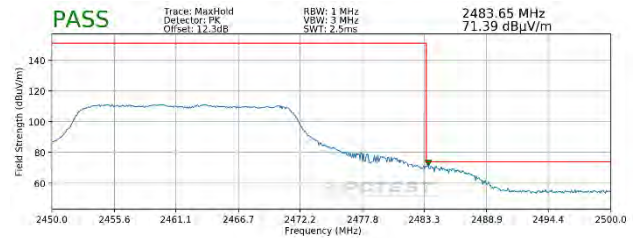
Plot 7-126. Radiated Restricted Upper Band Edge Measurement MIMO (Peak – 242 Tones)
