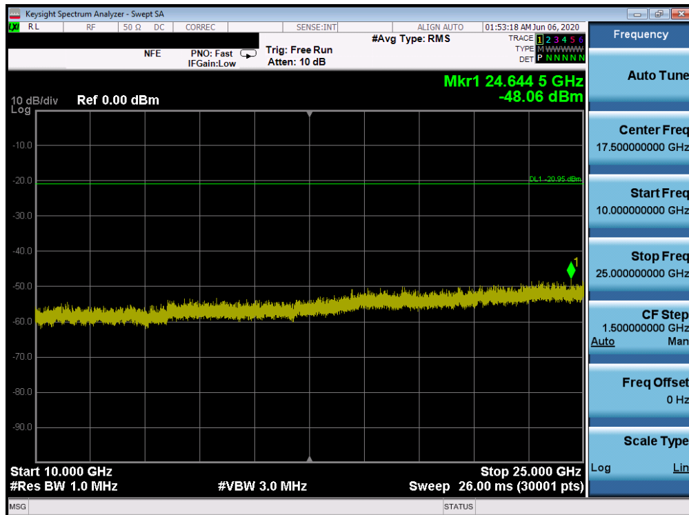
Plot 7-56. Conducted Spurious Plot SISO ANT2 (802.11ax OFDMA – 26 Tones – Ch. 11)
