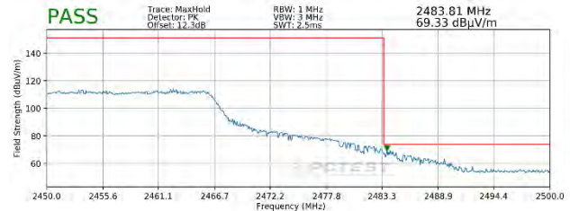
Plot 7-96. Radiated Restricted Upper Band Edge Measurement SISO ANT1 (Peak - 242 Tones)
