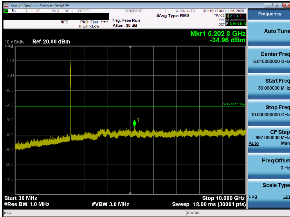
Plot 7-53. Conducted Spurious Plot SISO ANT2 (802.11ax OFDMA – 26 Tones – Ch. 6)
