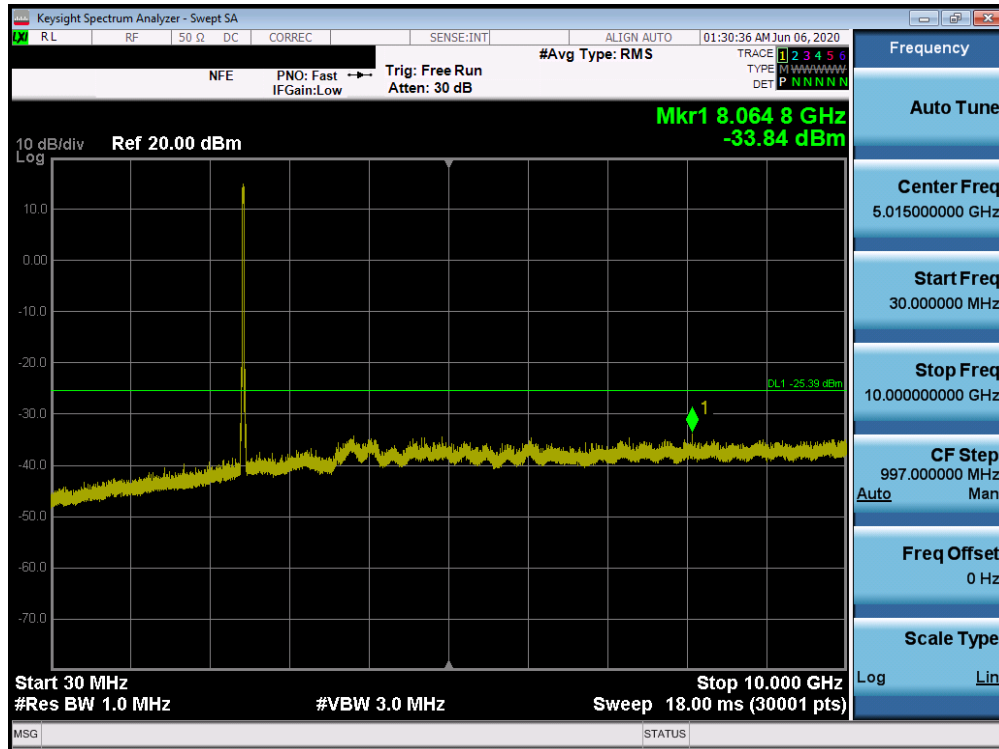
Plot 7-59. Conducted Spurious Plot SISO ANT2 (802.11ax OFDMA - 242 Tones - Ch. 6)
