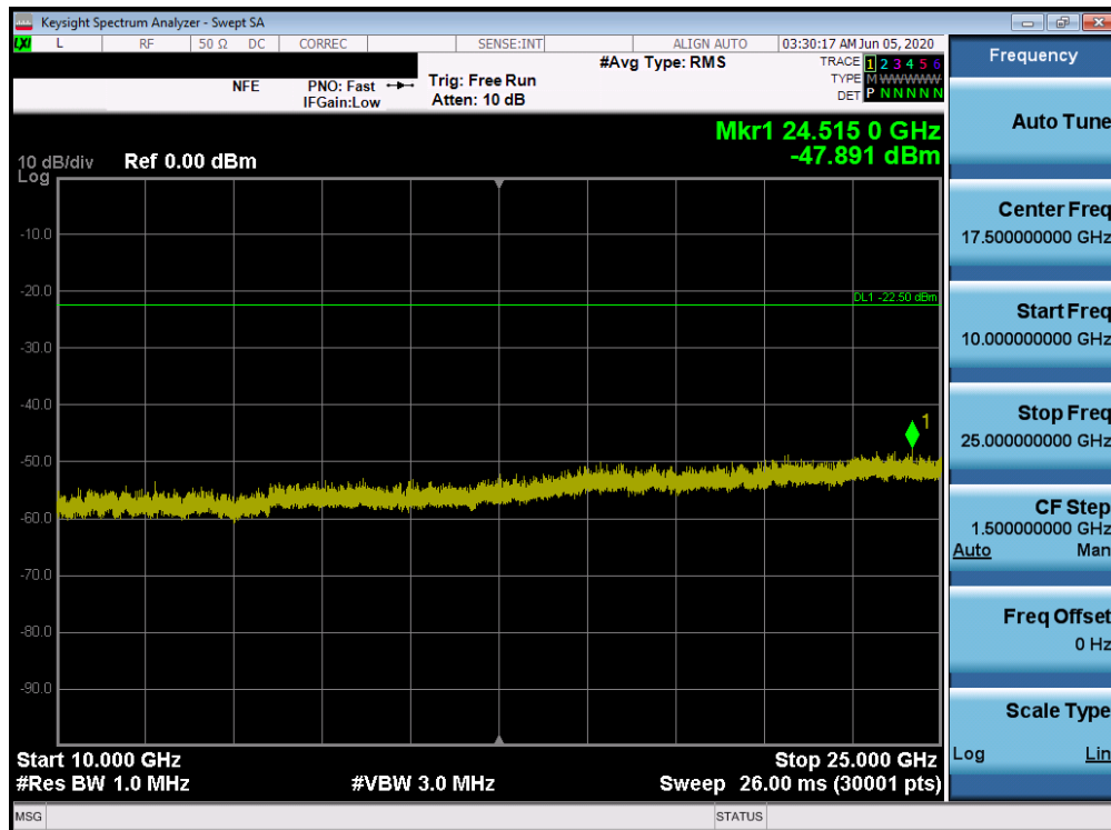
Plot 7-42. Conducted Spurious Plot SISO ANT1 (802.11ax OFDMA – 26 Tones – Ch. 6)
