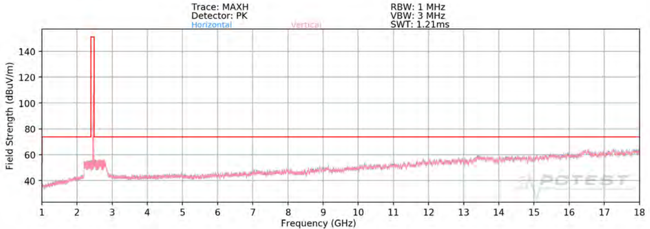
Plot 7-79. Radiated Spurious Plot above 1GHz MIMO (802.11ax OFDMA – 26 Tones – Ch. 11)
