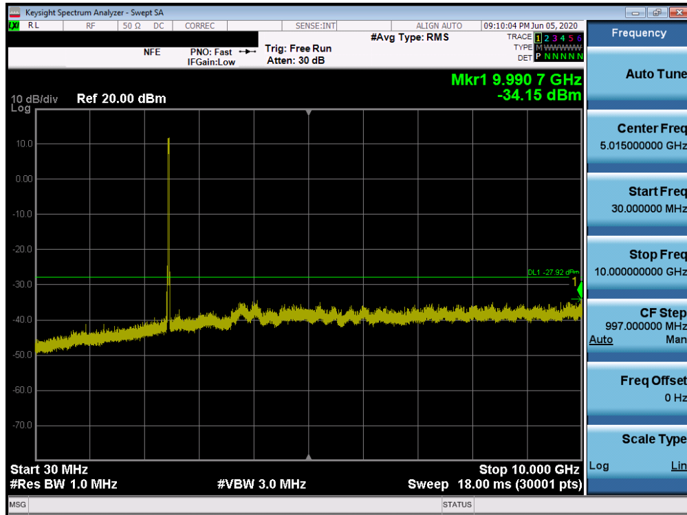
Plot 7-49. Conducted Spurious Plot SISO ANT1 (802.11ax OFDMA – 242 Tones – Ch. 11)
