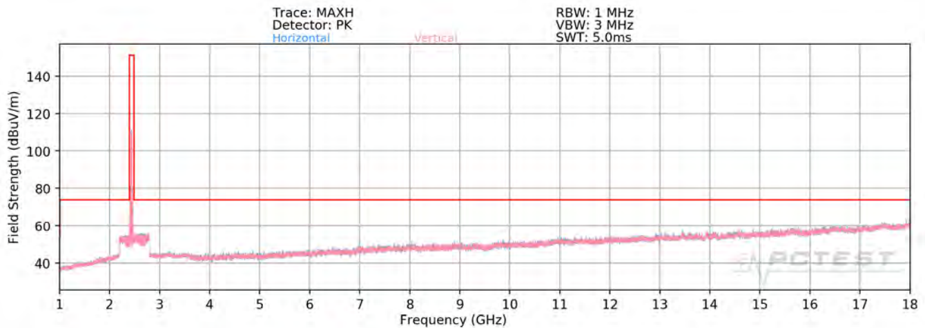
Plot 7-67. Radiated Spurious Plot above 1GHz SISO ANT1 (802.11ax OFDMA – 242 Tones – Ch. 6)
