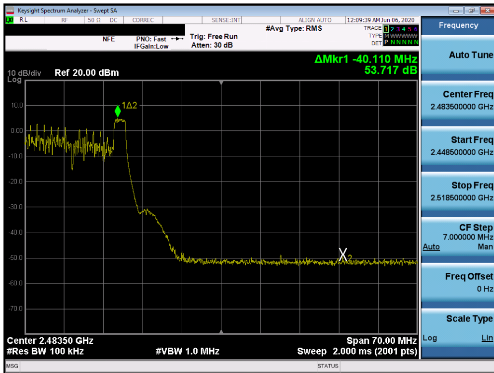
Plot 7-30. Band Edge Plot SISO ANT1 (802.11ax OFDMA - 52 Tones - Ch. 10)
