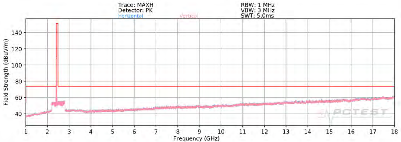
Plot 7-66. Radiated Spurious Plot above 1GHz SISO ANT1 (802.11ax OFDMA – 242 Tones – Ch. 1)
