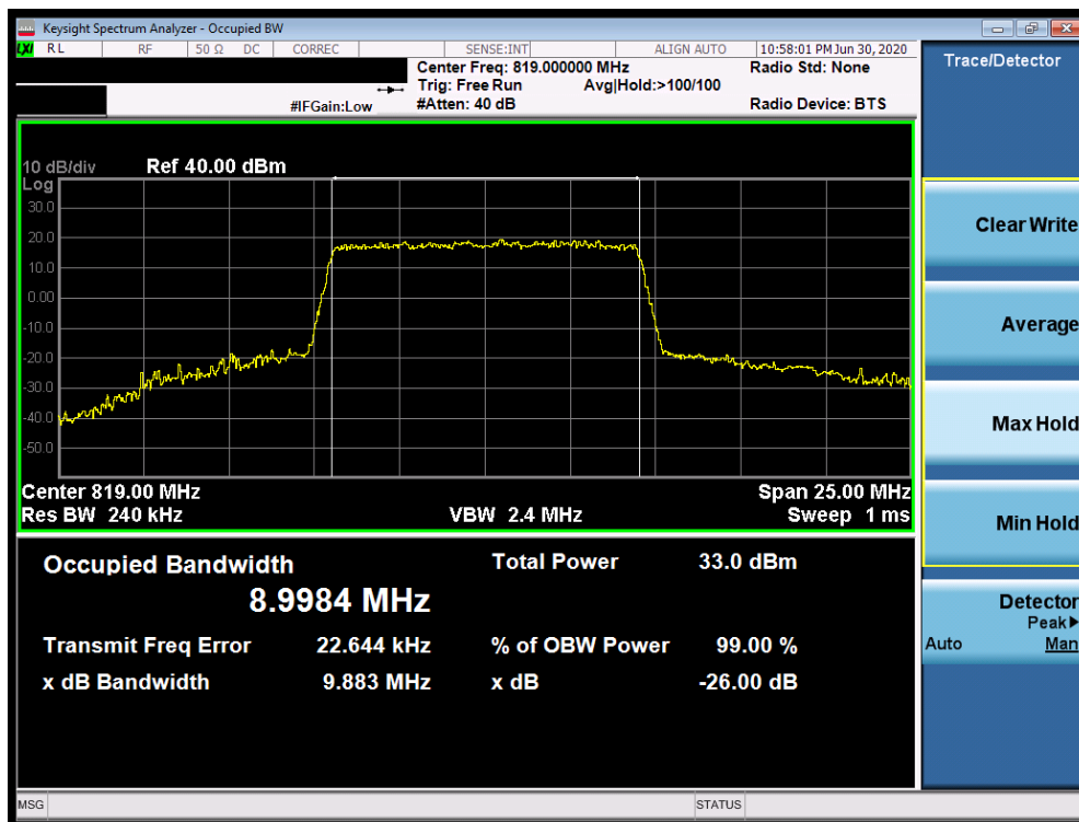
Plot 7-15. Occupied Bandwidth Plot (LTE Band 26 - 10MHz QPSK - Full RB Configuration)
