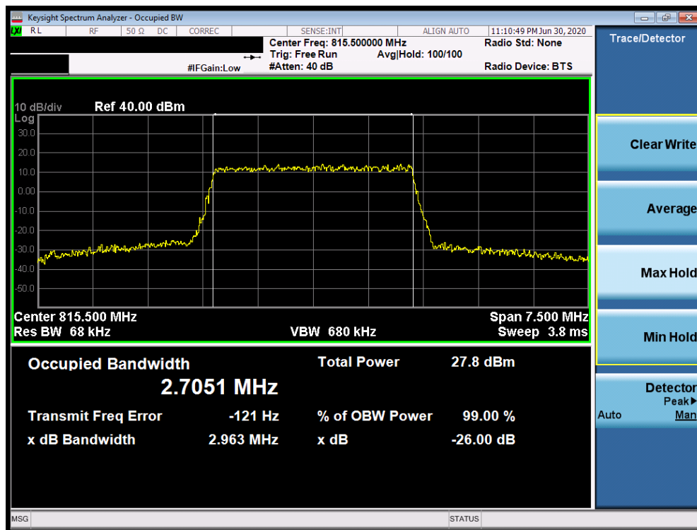
Plot 7-10. Occupied Bandwidth Plot (LTE Band 26 - 3MHz 256-QAM - Full RB Configuration)
