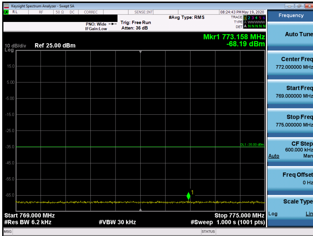
Plot 7-48. Lower Emission Mask Plot (LTE Band 14, 5MHz QPSK - RB Size 25)
