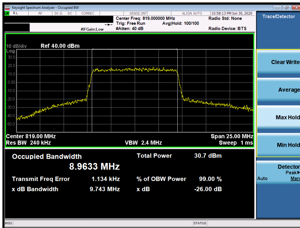
Plot 7-16. Occupied Bandwidth Plot (LTE Band 26 - 10MHz 16-QAM - Full RB Configuration)
