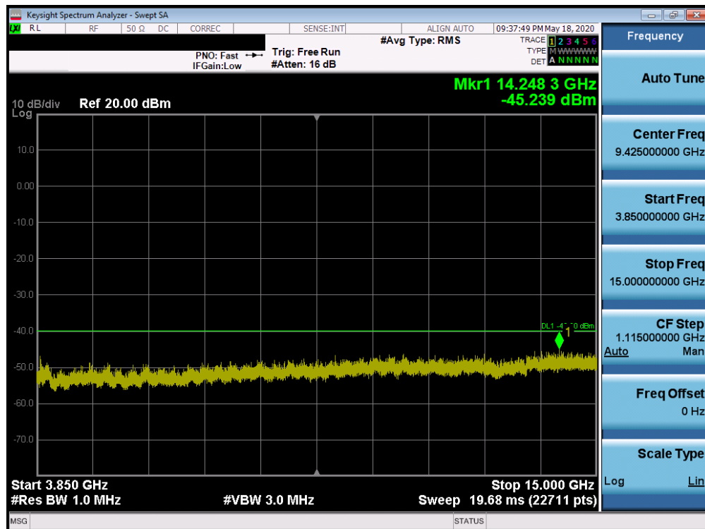
Plot 7-43. Conducted Spurious Plot (LTE Band 48 - 20.0MHz QPSK - RB Size 1, RB Offset 0 - Mid Channel)
