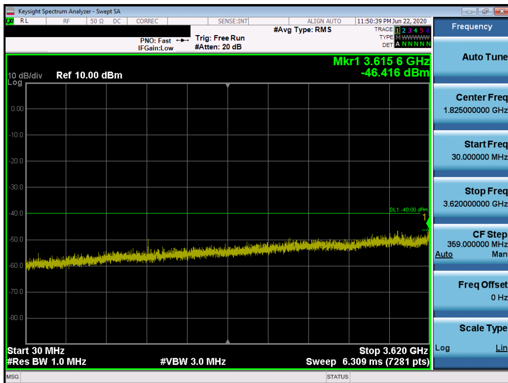
Plot 7-74. Conducted Spurious Plot (Band 48 – 20.0MHz QPSK – PCC 1/0 SCC 1/99 – High Channel)
