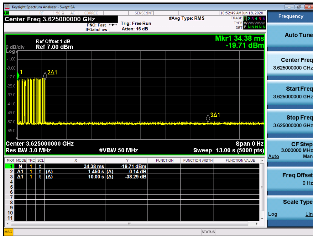
Plot 7-88. Run#1 End User Device Discontinues Operations within 10s
