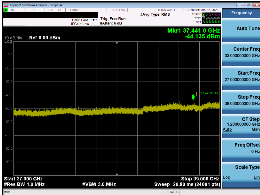
Plot 7-68. Conducted Spurious Plot (Band 48 – 20.0MHz QPSK – PCC 1/99 SCC 1/0 – Low Channel)
