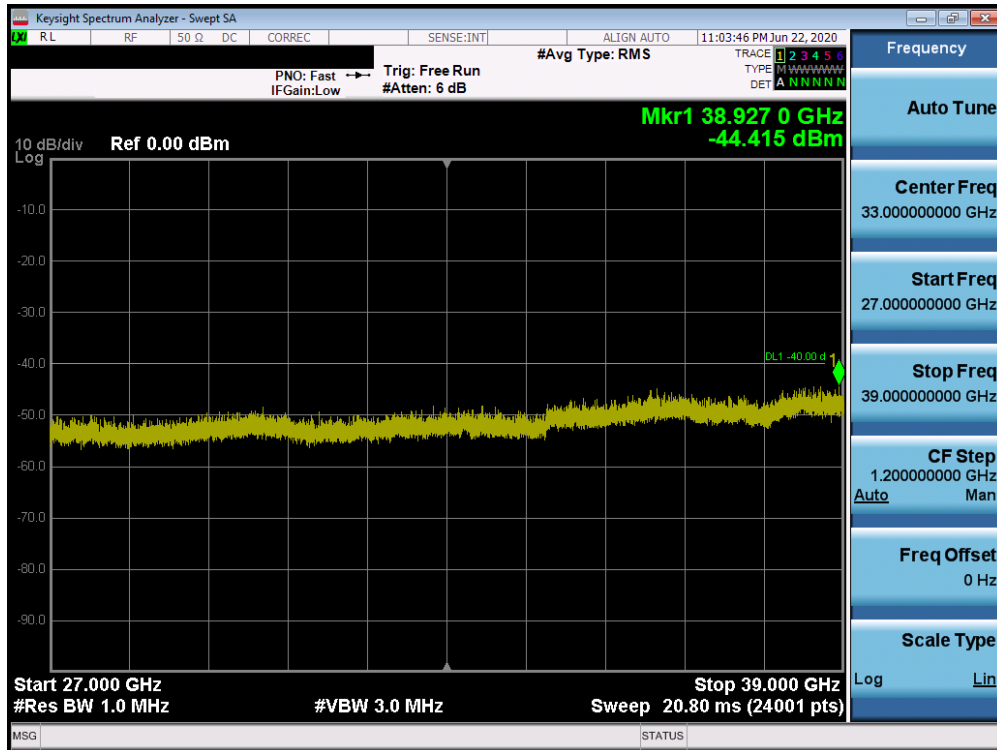
Plot 7-73. Conducted Spurious Plot (Band 48 – 20.0MHz QPSK – PCC 1/99 SCC 1/0 – Mid Channel)
