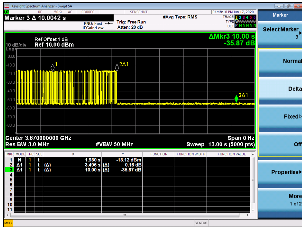
Plot 7-90. Run#2 End User Device Discontinues Operations within 10s
