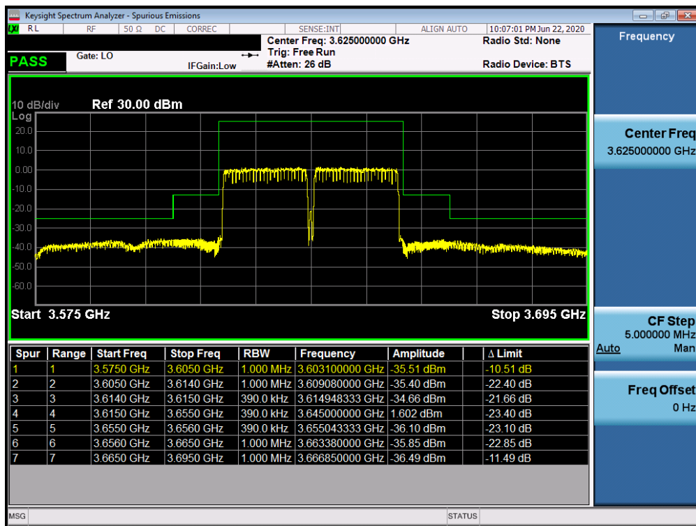
Plot 7-80. Mid Band Edge Plot (Band 48 QPSK – PCC:20 MHz SCC:20 MHz – Full RB)
