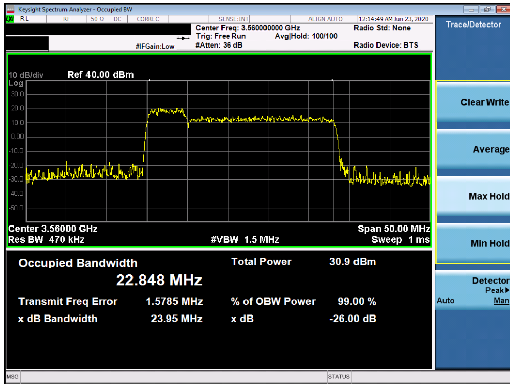
Plot 7-19. Occupied Bandwidth Plot (LTE Band 48 (ULCA)- 5 + 20.0MHz 64-QAM - Full RB Configuration)
