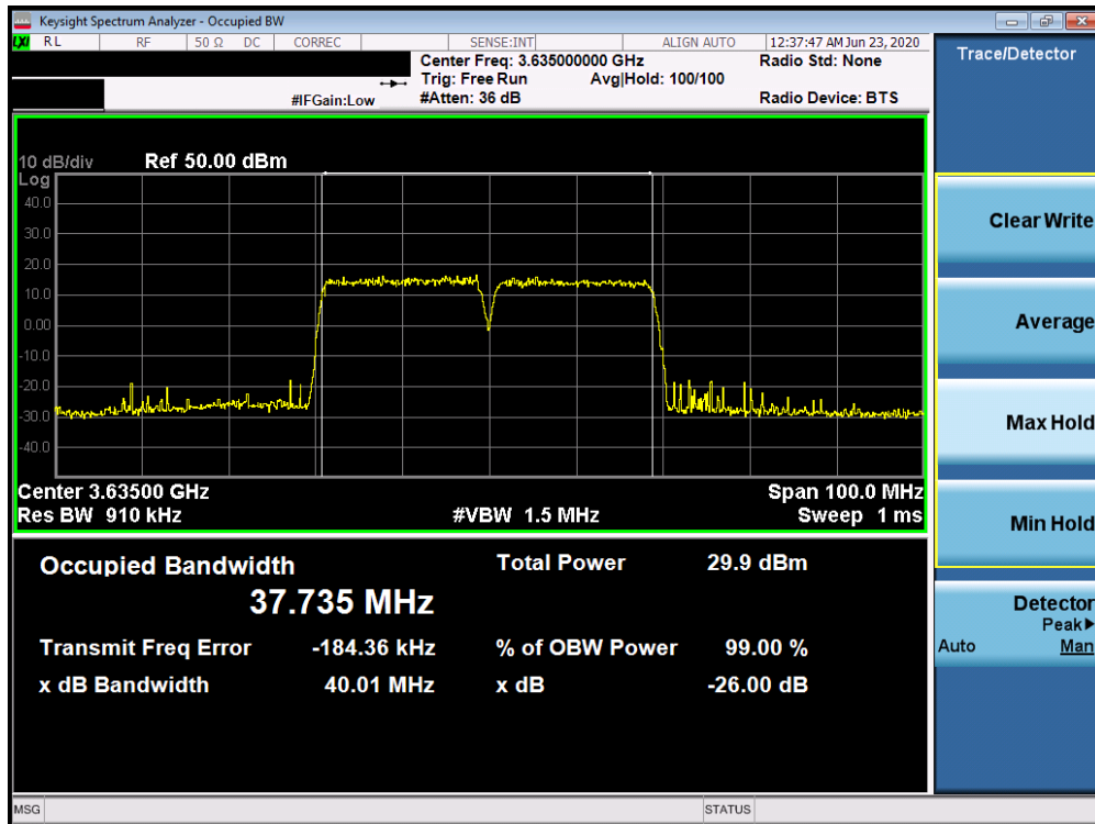
Plot 7-32. Occupied Bandwidth Plot (LTE Band 48 (ULCA) 20 + 20.0MHz 256-QAM - Full RB Configuration)
