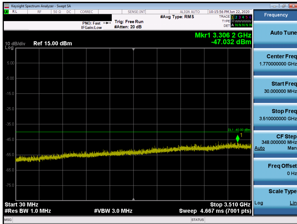
Plot 7-64. Conducted Spurious Plot (Band 48 – 20.0MHz QPSK – PCC 1/99 SCC 1/0 – Low Channel)
