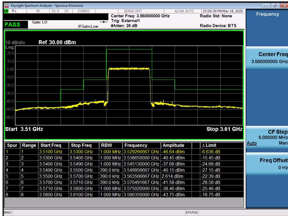
Plot 7-61. Lower ACP Plot (LTE Band 48 - 20.0MHz QPSK - Full RB Configuration)
