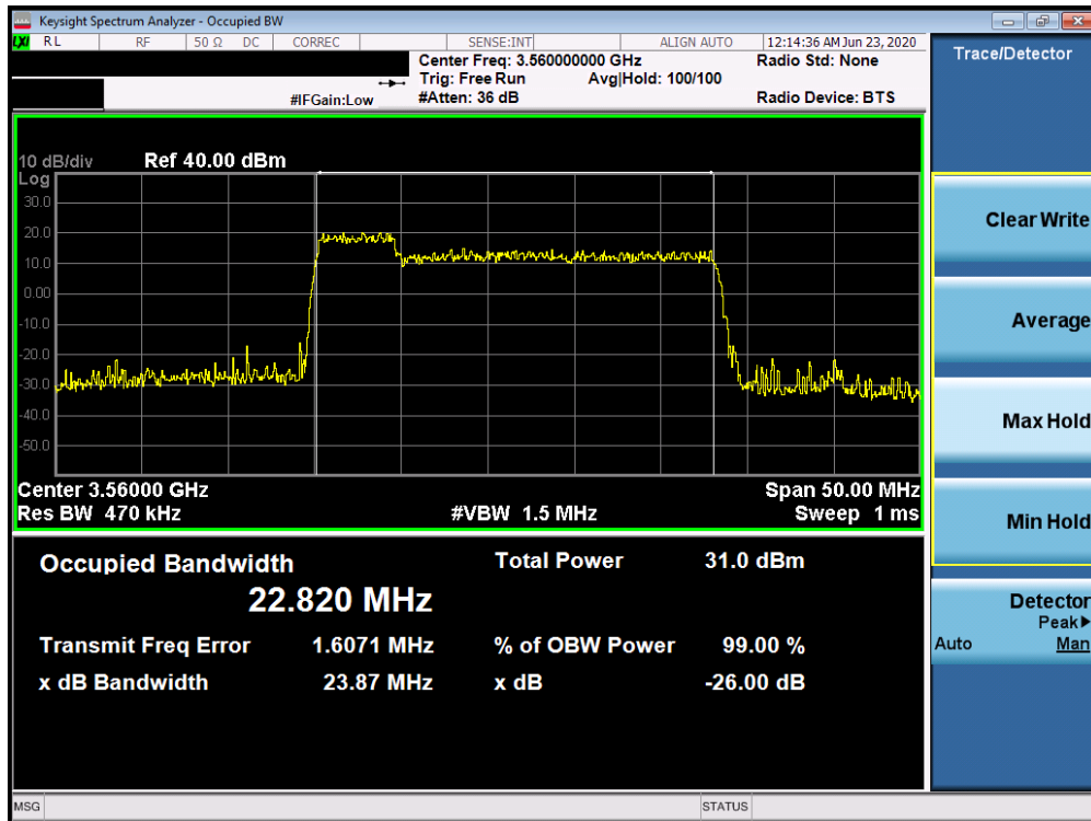
Plot 7-18. Occupied Bandwidth Plot (LTE Band 48(ULCA)- 5 + 20.0MHz 16-QAM - Full RB Configuration)
