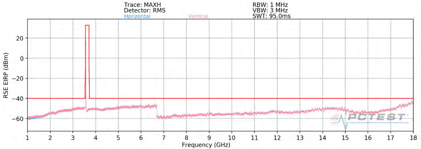
Plot 7-84. Radiated Spurious Plot 1GHz - 18GHz (ULCA Band 48) Low Channel – PCC/SCC: 1RB)
