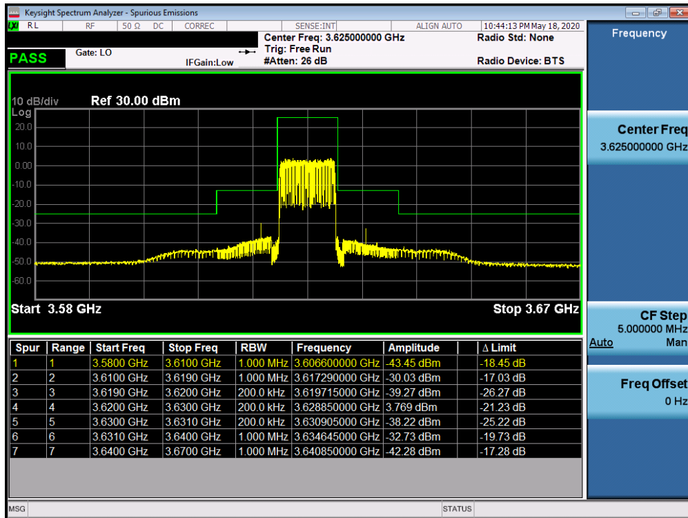
Plot 7-56. Mid ACP Plot (LTE Band 48 - 10.0MHz QPSK - Full RB Configuration)
