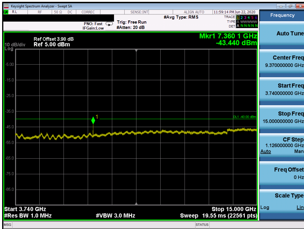
Plot 7-76. Conducted Spurious Plot (Band 48 – 20.0MHz QPSK – PCC 1/0 SCC 1/99 – High Channel)
