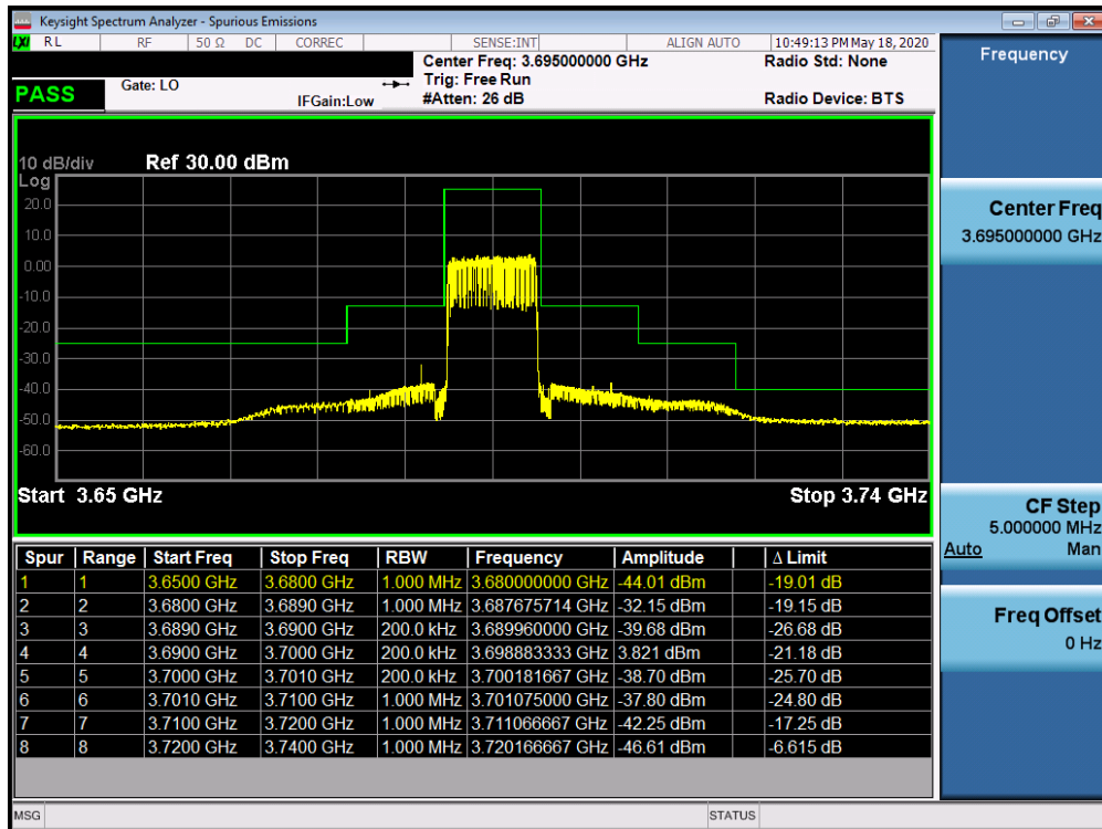
Plot 7-57. Upper ACP Plot (LTE Band 48 - 10.0MHz QPSK - Full RB Configuration)
