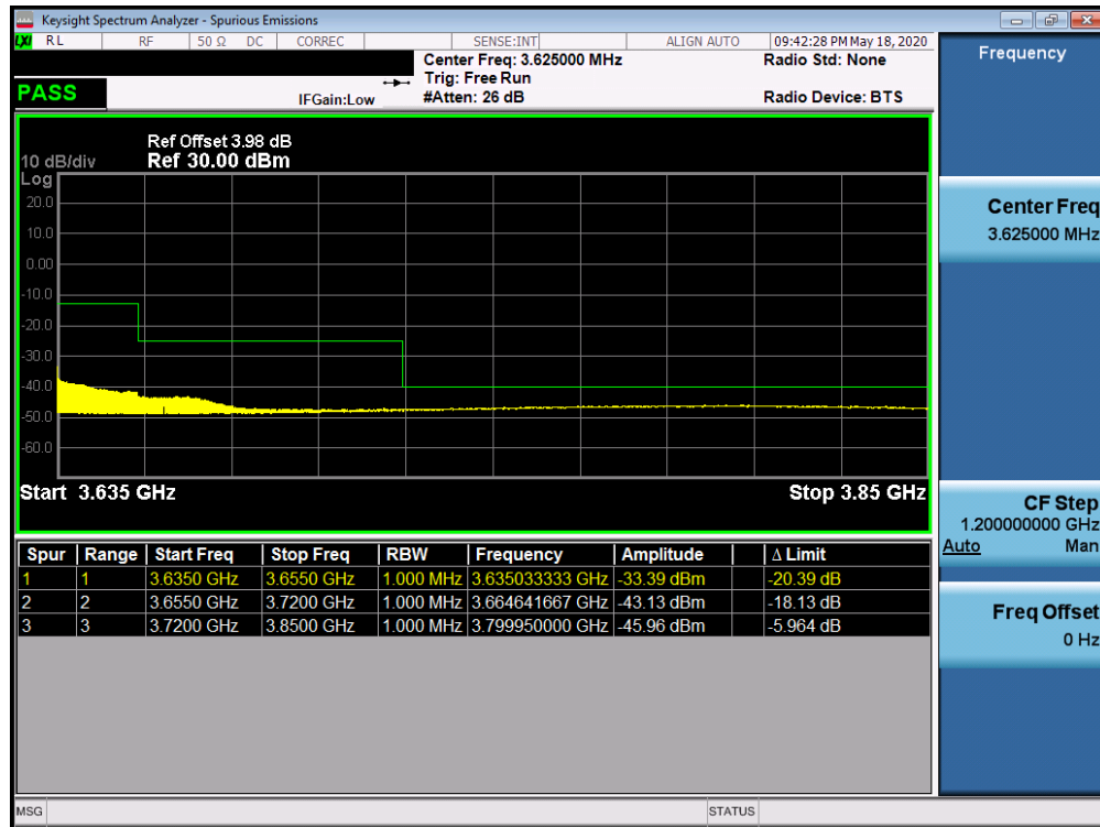
Plot 7-42. Conducted Spurious Plot (LTE Band 48 - 20.0MHz QPSK - RB Size 1, RB Offset 0 - Mid Channel)
