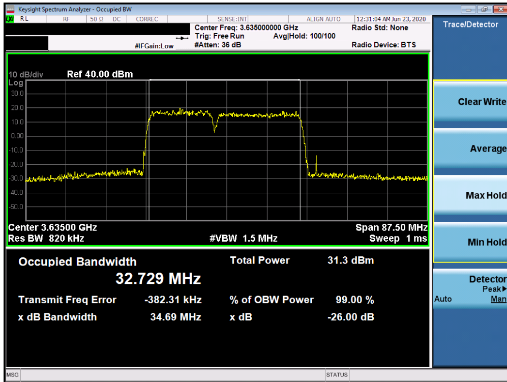
Plot 7-27. Occupied Bandwidth Plot (LTE Band 48 (ULCA) 15 + 20.0MHz 64-QAM - Full RB Configuration)
