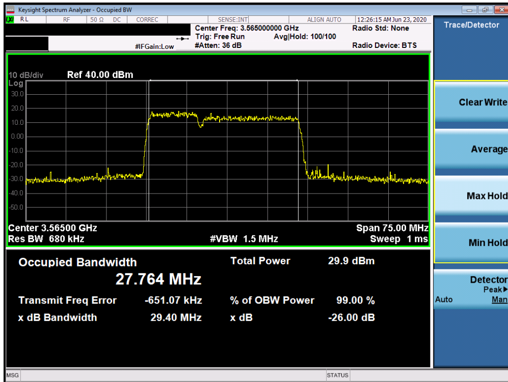
Plot 7-24. Occupied Bandwidth Plot (LTE Band 48 (ULCA) 10 + 20.0MHz 256-QAM - Full RB Configuration)
