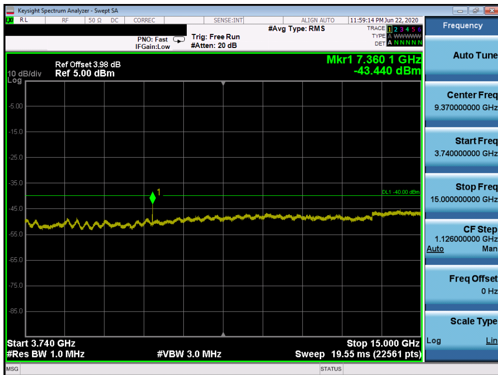
Plot 7-78. Conducted Spurious Plot (Band 48 – 20.0MHz QPSK – PCC 1/0 SCC 1/99 – High Channel)
