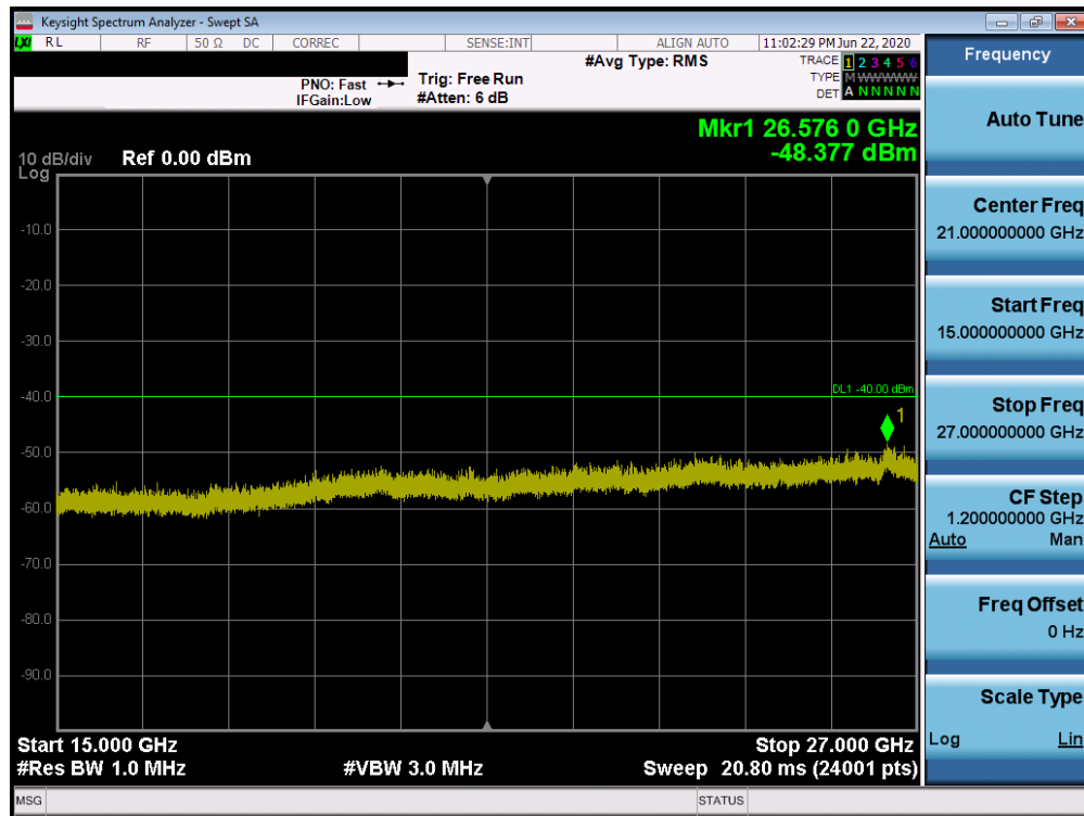
Plot 7-72. Conducted Spurious Plot (Band 48 – 20.0MHZ QPSK – PCC 1/99 SCC 1/0 – Mid Channel)
