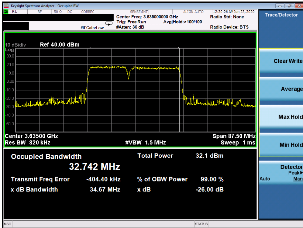
Plot 7-26. Occupied Bandwidth Plot (LTE Band 48(ULCA) 15 + 20.0MHz 16-QAM - Full RB Configuration)
