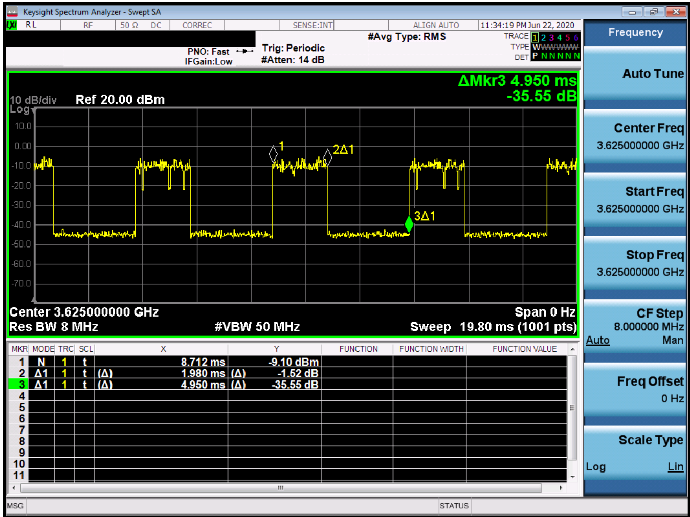
Plot 7-33. Duty Cycle Plot
