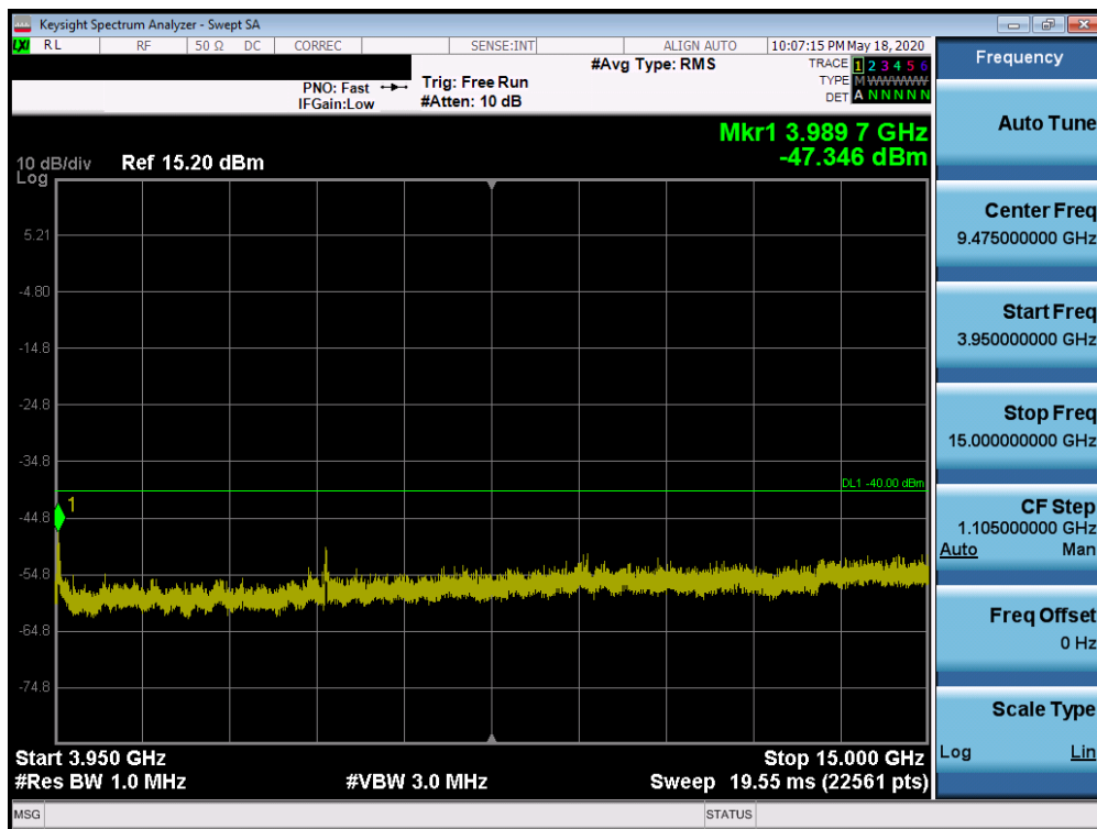
Plot 7-49. Conducted Spurious Plot (LTE Band 48 – 20.0MHz QPSK – RB Size 1, RB Offset 0 – High Channel)
