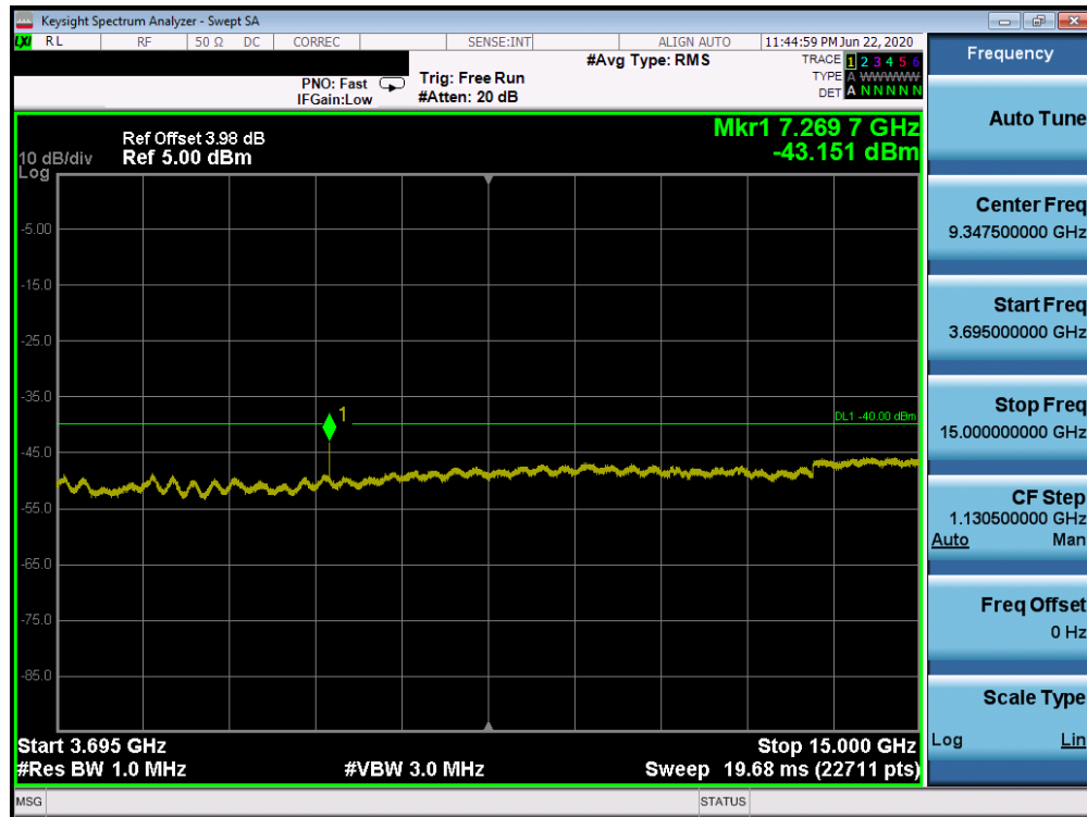
Plot 7-71. Conducted Spurious Plot (Band 48 – 20.0MHZ QPSK – PCC 1/99 SCC 1/0 – Mid Channel)
