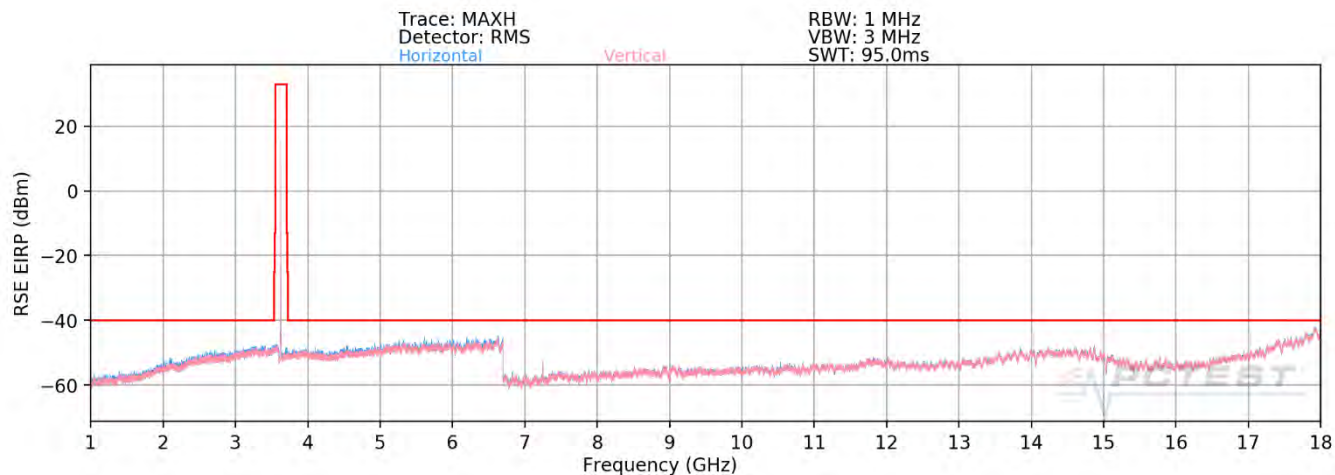
Plot 7-82. Radiated Spurious Plot 1 - 18GHz (Band 48)
