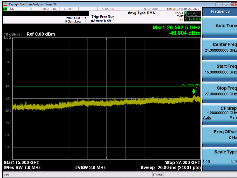
Plot 7-67. Conducted Spurious Plot (Band 48 – 20.0MHz QPSK – PCC 1/99 SCC 1/0 – Low Channel)
