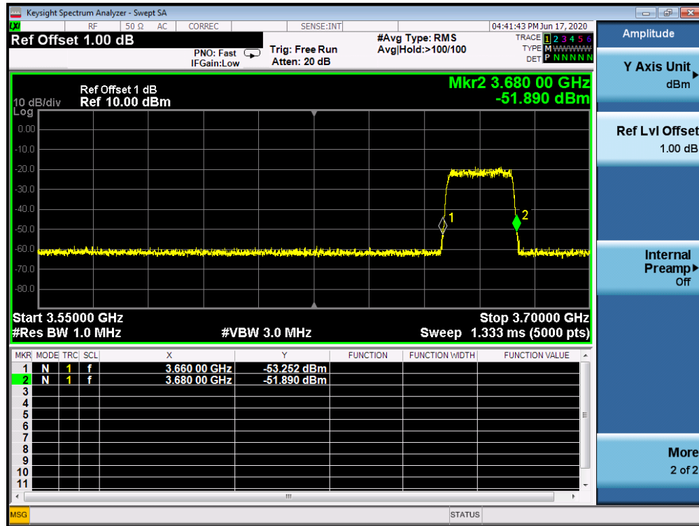
Plot 7-89. Run#2 End User Device Frequency of Operations
