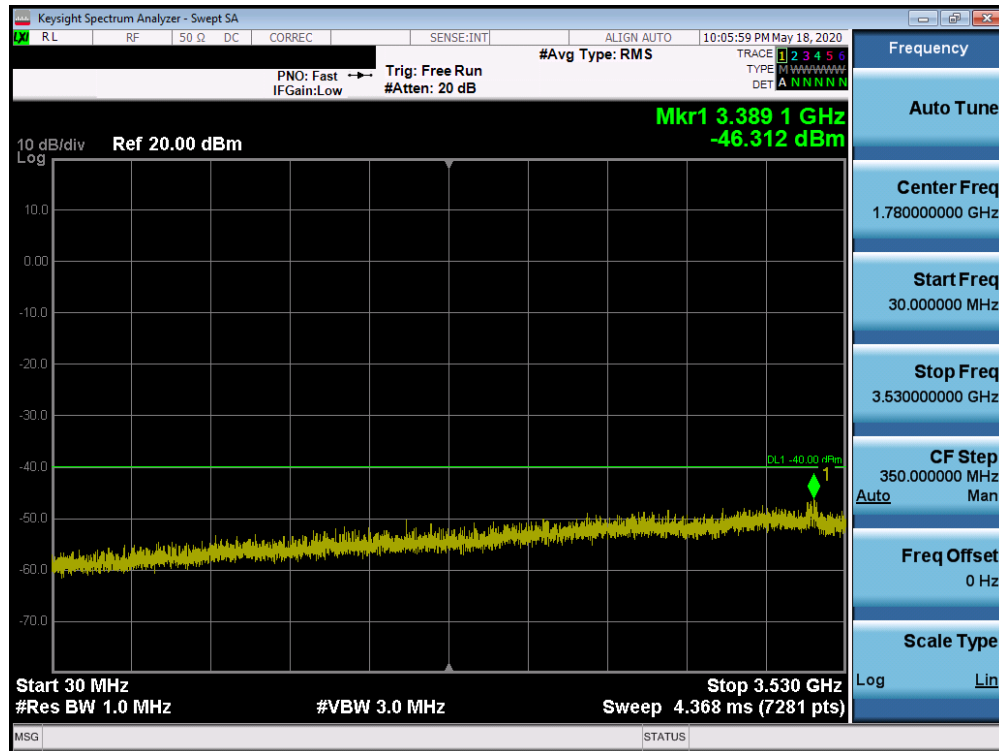
Plot 7-46. Conducted Spurious Plot (LTE Band 48 - 20.0MHz QPSK - RB Size 1, RB Offset 0 - High Channel)
