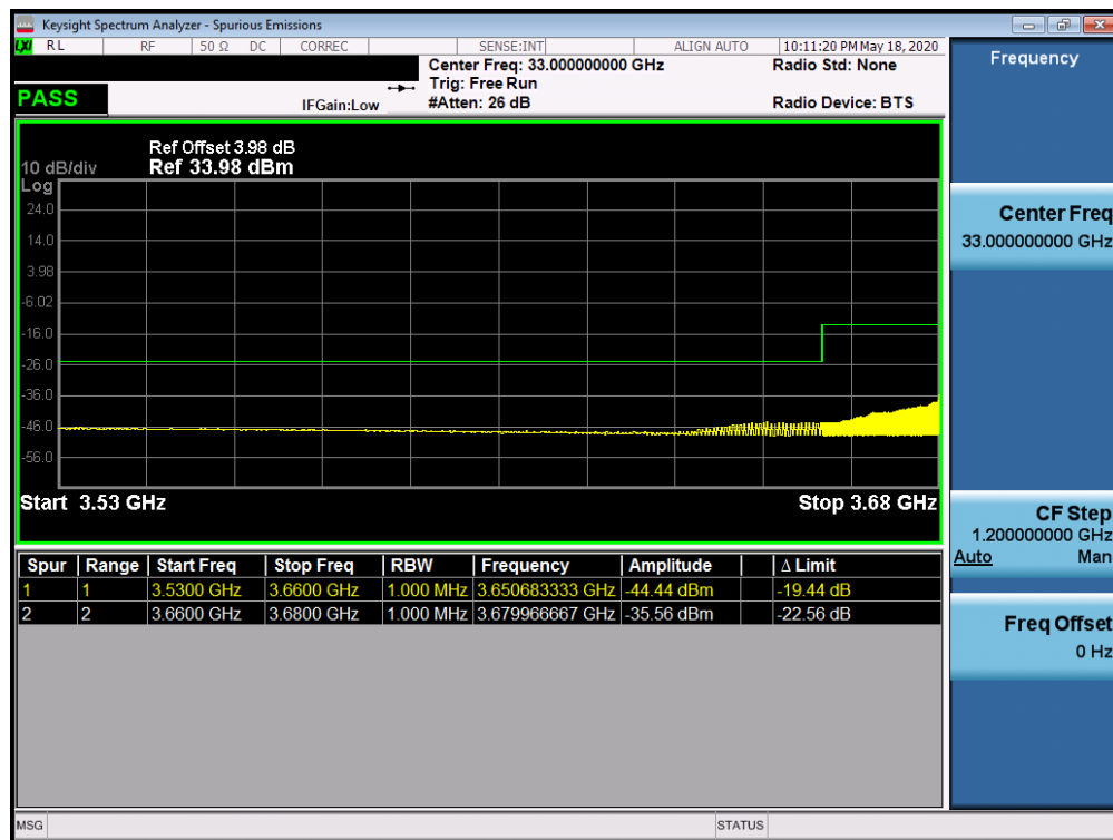
Plot 7-47. Conducted Spurious Plot (LTE Band 48 - 20.0MHz QPSK - RB Size 1, RB Offset 0 - High Channel)
