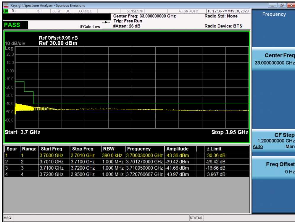
Plot 7-48. Conducted Spurious Plot (LTE Band 48 – 20.0MHz QPSK – RB Size 1, RB Offset 0 – High Channel)
