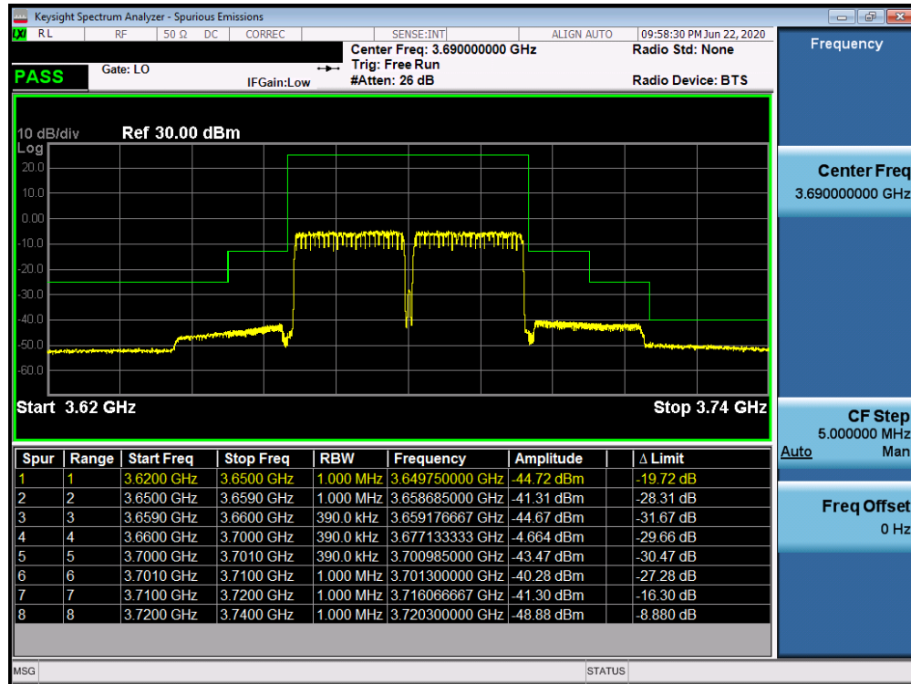
Plot 7-81. Upper Band Edge Plot (Band 48 QPSK – PCC:20 MHz SCC:20 MHz – Full RB)
