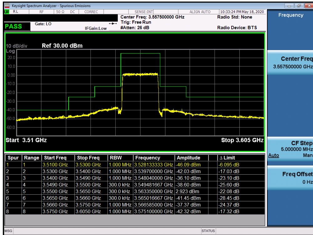
Plot 7-58. Lower ACP Plot (LTE Band 48 - 15.0MHz QPSK - Full RB Configuration)
