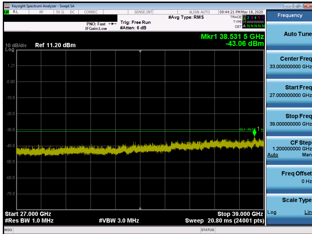
Plot 7-45. Conducted Spurious Plot (LTE Band 48 - 20.0MHz QPSK - RB Size 1, RB Offset 0 - Mid Channel)
