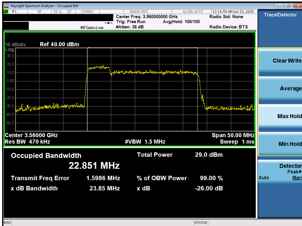
Plot 7-20. Occupied Bandwidth Plot (LTE Band 48 (ULCA)- 5 + 20.0MHz 256-QAM - Full RB Configuration)
