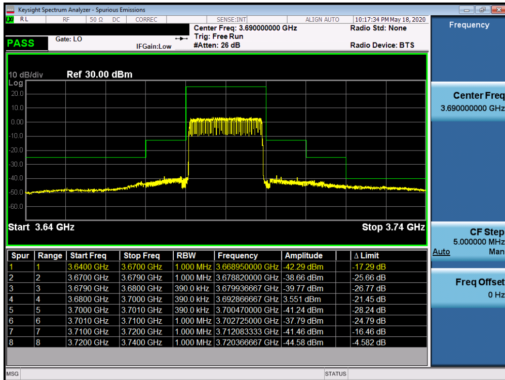
Plot 7-63. Upper ACP Plot (LTE Band 48 - 20.0MHz QPSK - Full RB Configuration)
