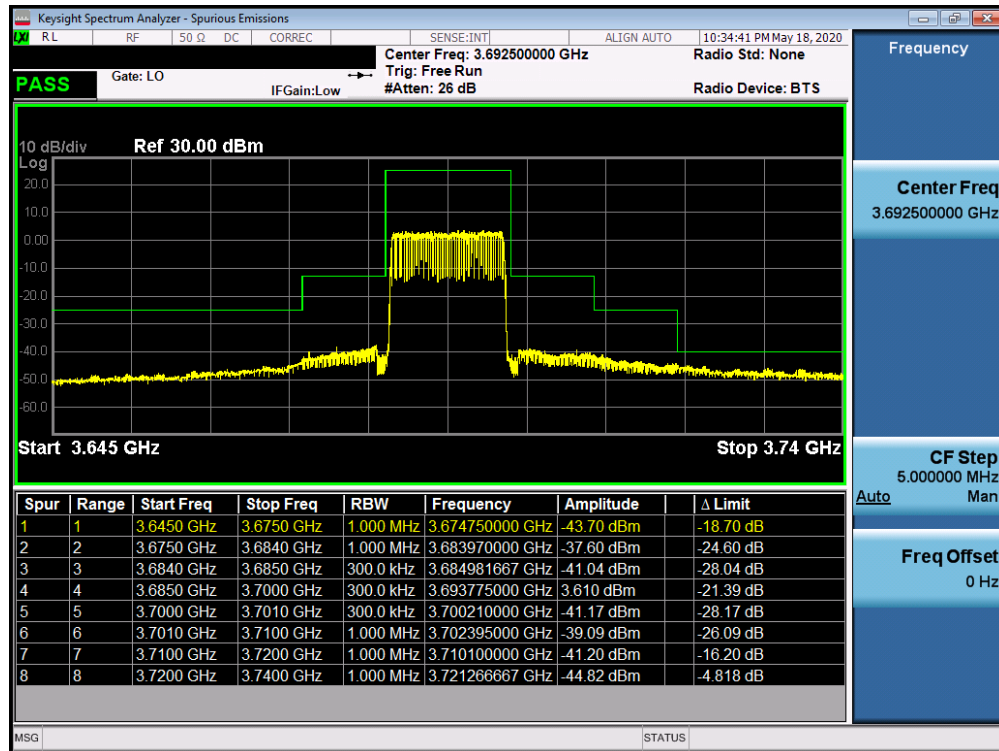
Plot 7-60. Upper ACP Plot (LTE Band 48 - 15.0MHz QPSK - Full RB Configuration)
