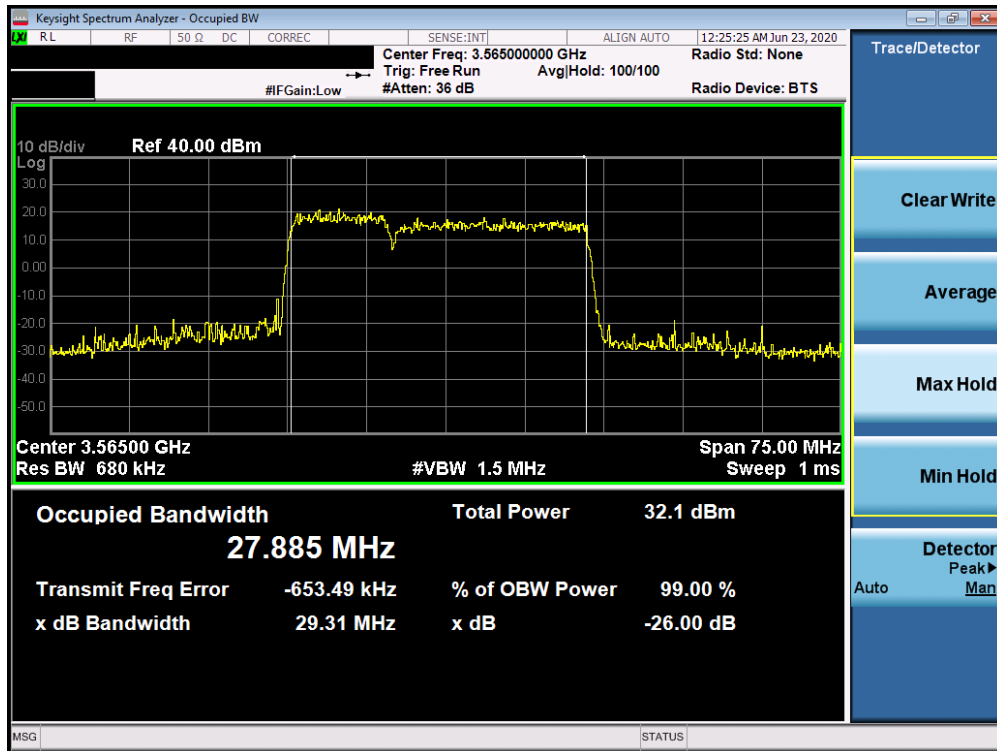
Plot 7-23. Occupied Bandwidth Plot (LTE Band 48 - (ULCA) 10 + 20.0MHz 64-QAM - Full RB Configuration)
