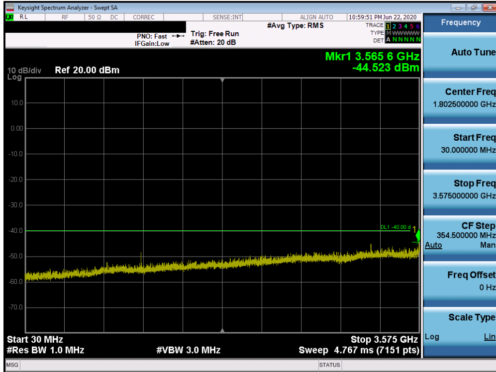
Plot 7-69. Conducted Spurious Plot (Band 48 – 20.0MHZ QPSK – PCC 1/99 SCC 1/0 – Mid Channel)
