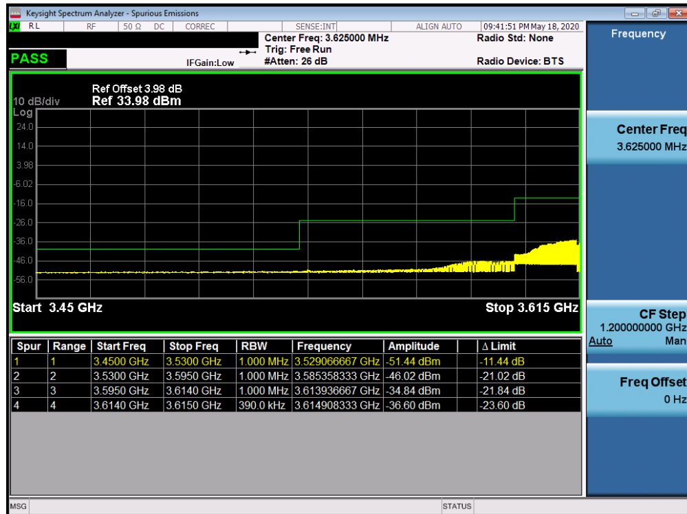
Plot 7-41. Conducted Spurious Plot (LTE Band 48 - 20.0MHz QPSK - RB Size 1, RB Offset 0 - Mid Channel)
