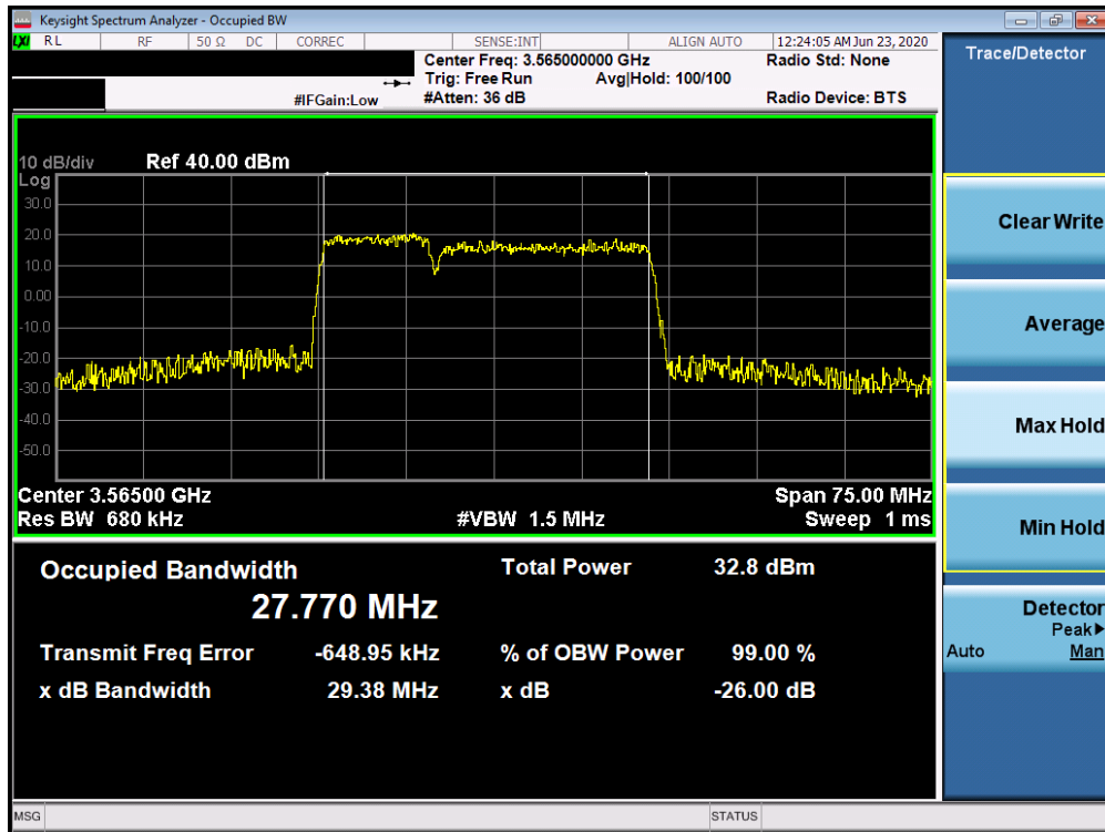
Plot 7-21. Occupied Bandwidth Plot (LTE Band 48 (ULCA) 10 + 20.0MHz QPSK - Full RB Configuration)
