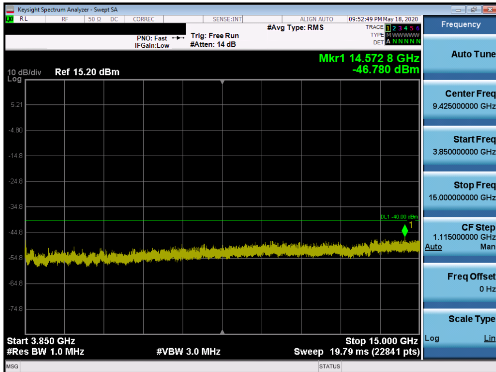
Plot 7-37. Conducted Spurious Plot (LTE Band 48 - 20.0MHz QPSK - RB Size 1, RB Offset 0 - Low Channel)
