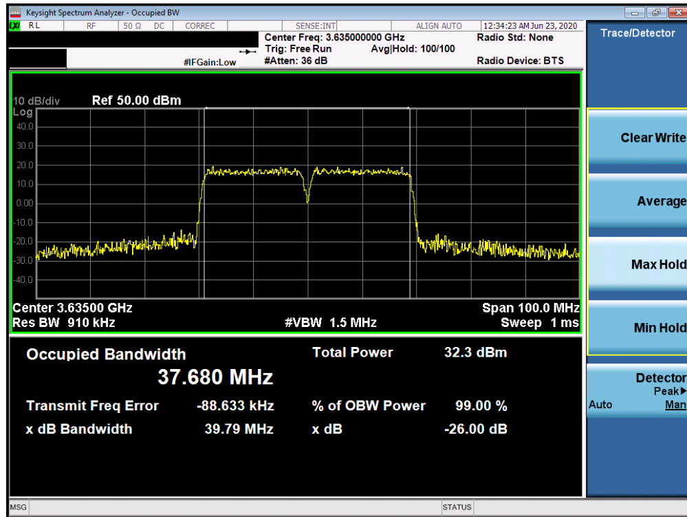
Plot 7-29. Occupied Bandwidth Plot (LTE Band 48 (ULCA) 20 + 20.0MHz QPSK - Full RB Configuration)
