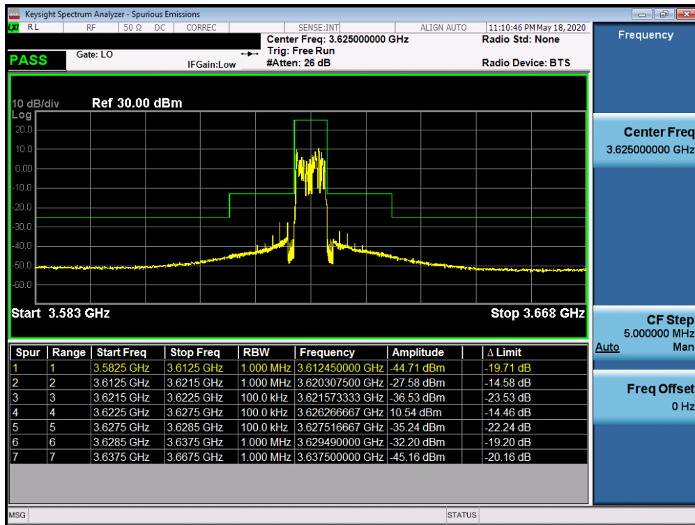
Plot 7-53. Mid ACP Plot (LTE Band 48 - 5.0MHz QPSK - Full RB Configuration)
