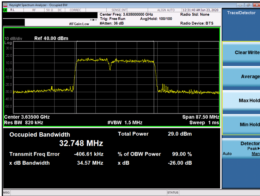
Plot 7-28. Occupied Bandwidth Plot (LTE Band 48 (ULCA) 15 + 20.0MHz 256-QAM - Full RB Configuration)
