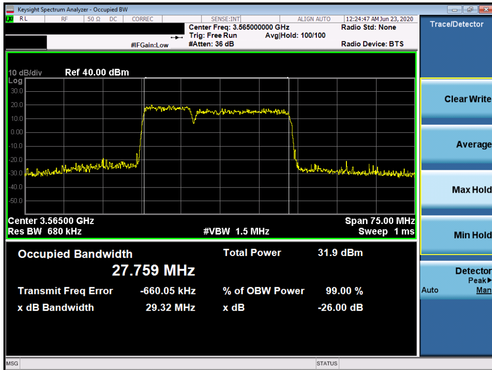
Plot 7-22. Occupied Bandwidth Plot (LTE Band 48 - (ULCA) 10 + 20.0MHz 16-QAM - Full RB Configuration)
