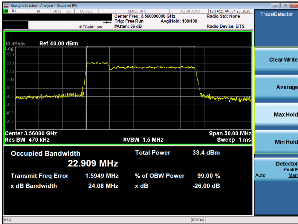
Plot 7-17. Occupied Bandwidth Plot (LTE Band 48 (ULCA)- 5 + 20.0MHz QPSK - Full RB Configuration)
