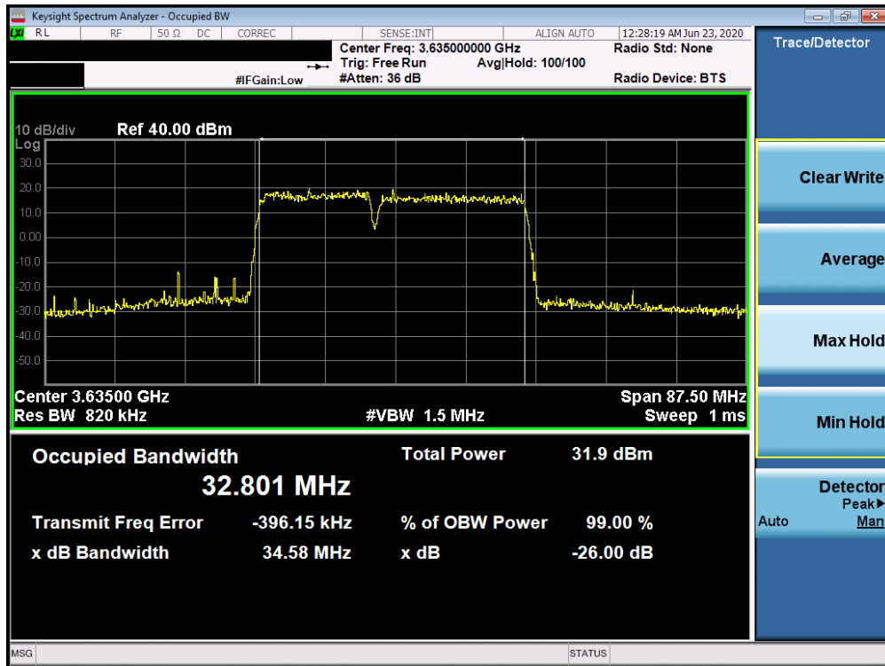
Plot 7-25. Occupied Bandwidth Plot (LTE Band 48 (ULCA) 15 + 20.0MHz QPSK - Full RB Configuration)
