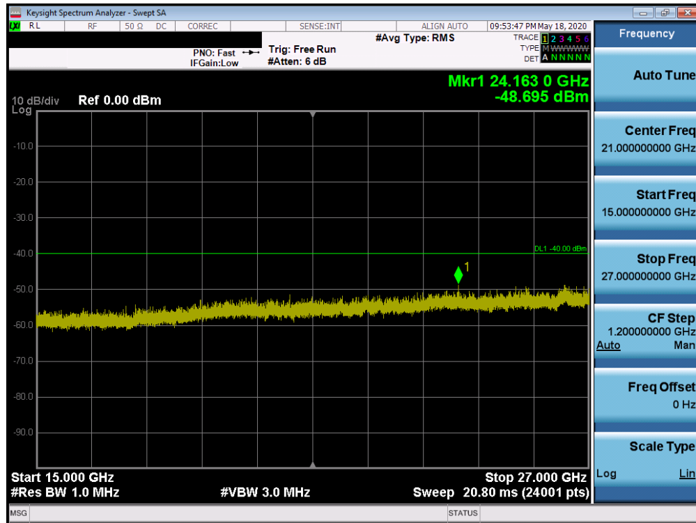
Plot 7-38. Conducted Spurious Plot (LTE Band 48 - 20.0MHz QPSK - RB Size 1, RB Offset 0 - Low Channel)
