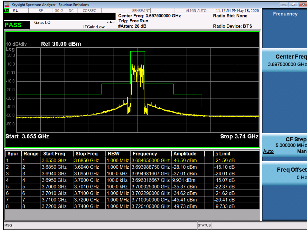
Plot 7-54. Upper ACP Plot (LTE Band 48 - 5.0MHz QPSK - Full RB Configuration)
