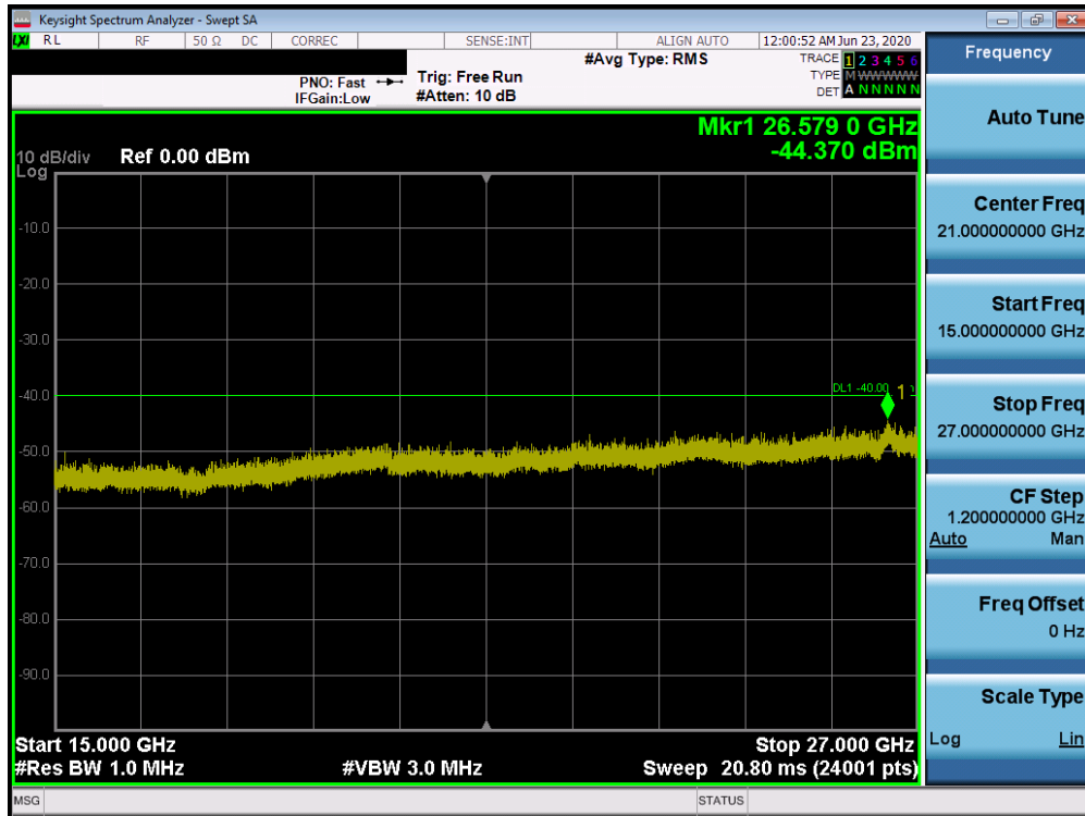
Plot 7-77. Conducted Spurious Plot (Band 48 – 20.0MHz QPSK – PCC 1/0 SCC 1/99 – High Channel)
