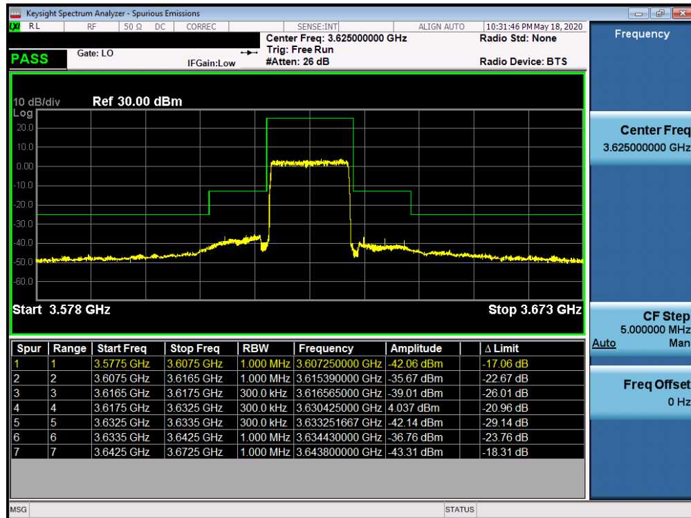
Plot 7-59. Mid ACP Plot (LTE Band 48 - 15.0MHz QPSK - Full RB Configuration)
