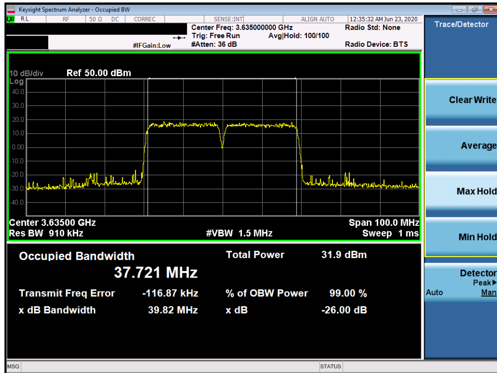
Plot 7-30. Occupied Bandwidth Plot (LTE Band 48 (ULCA) 20 + 20.0MHz 16-QAM - Full RB Configuration)
