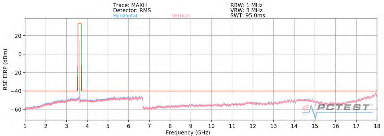
Plot 7-85. Radiated Spurious Plot 1GHz - 18GHz (ULCA Band 48) Mid Channel – PCC/SCC: 1RB)
