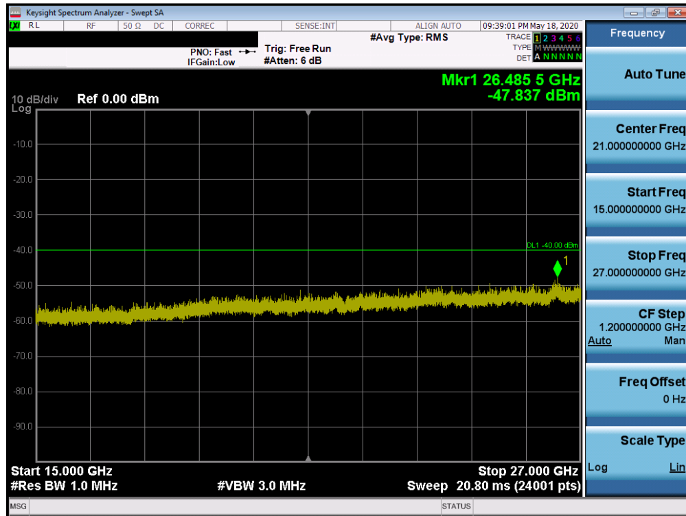
Plot 7-44. Conducted Spurious Plot (LTE Band 48 - 20.0MHz QPSK - RB Size 1, RB Offset 0 - Mid Channel)
