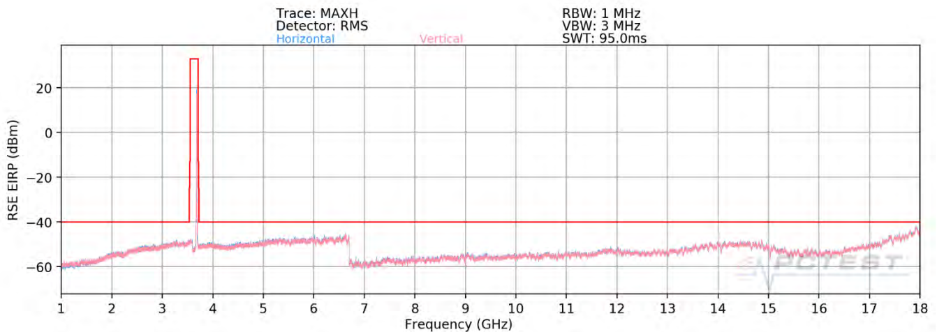
Plot 7-86. Radiated Spurious Plot 1GHz - 18GHz (ULCA Band 48) High Channel – PCC/SCC: 1RB)
