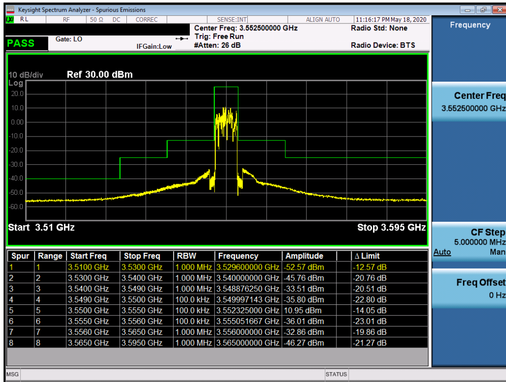
Plot 7-52. Lower ACP Plot (LTE Band 48 - 5.0MHz QPSK - Full RB Configuration)
