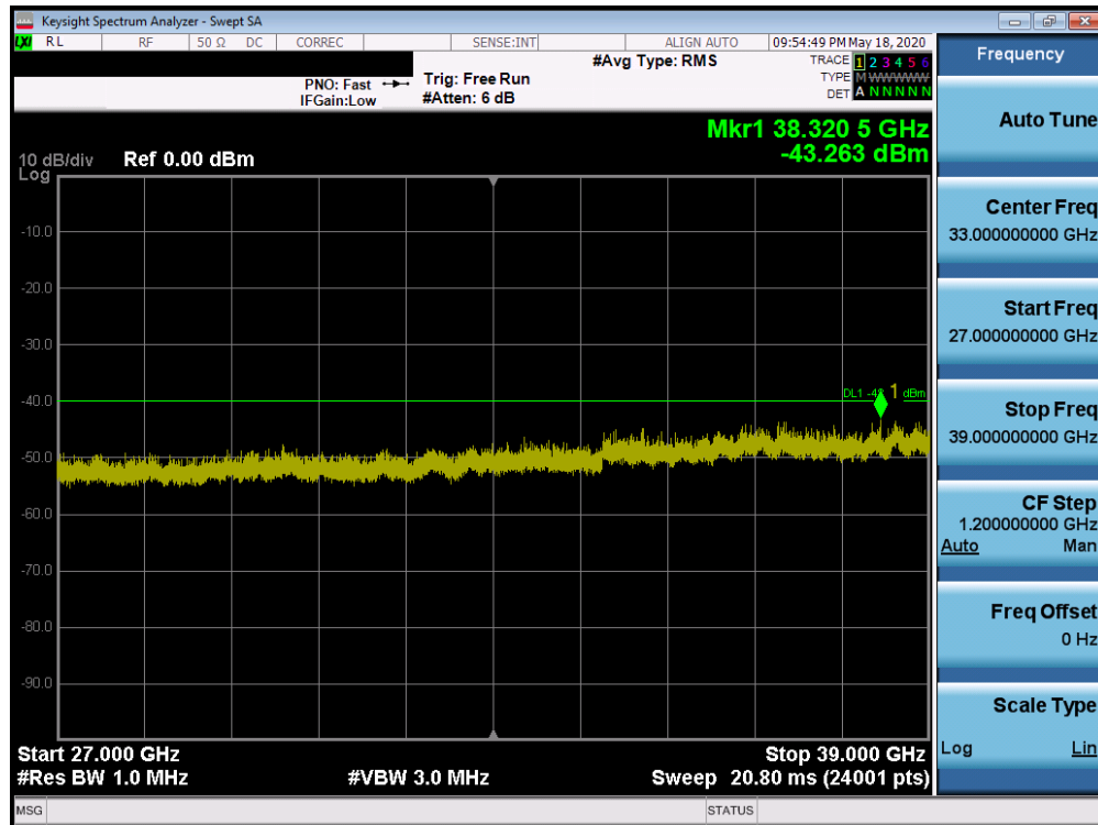
Plot 7-39. Conducted Spurious Plot (LTE Band 48 - 20.0MHz QPSK - RB Size 1, RB Offset 0 - Low Channel)
