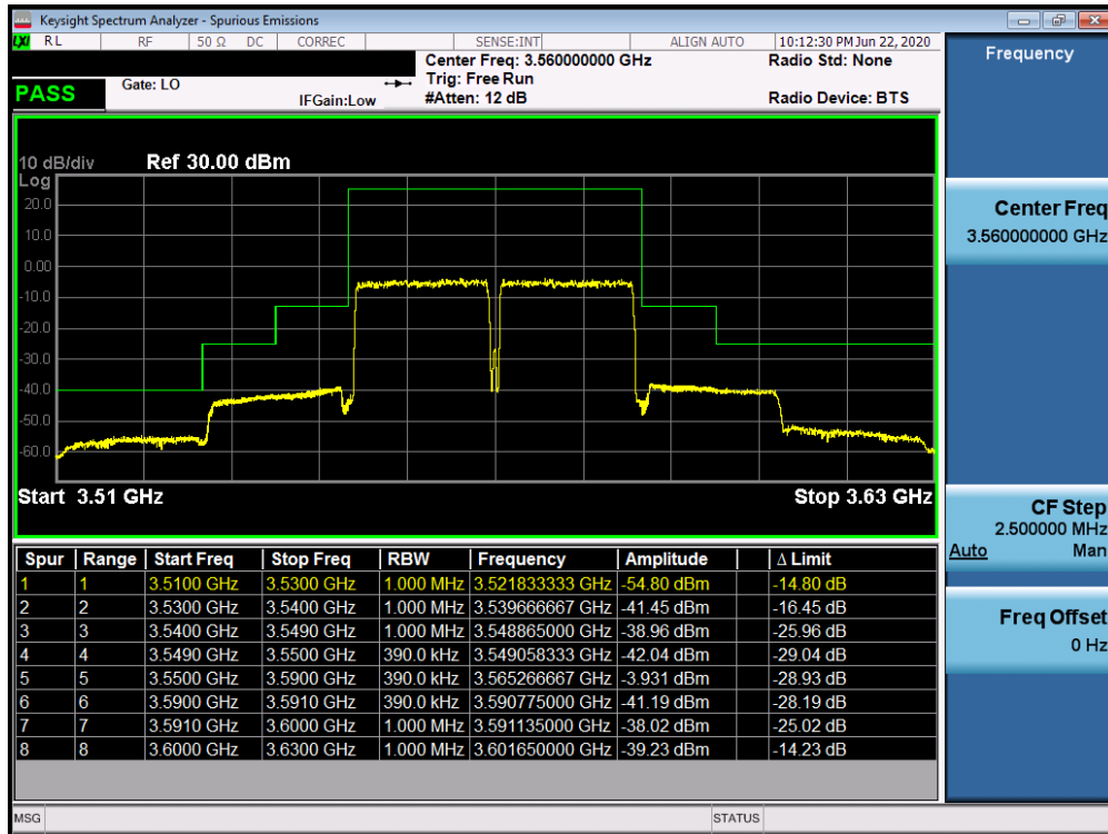
Plot 7-79. Lower Band Edge Plot (Band 48 QPSK – PCC:20 MHz SCC:20 MHz – Full RB)
