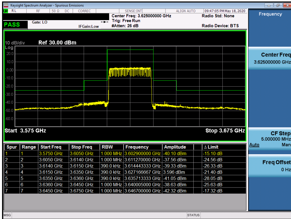
Plot 7-62. Mid ACP Plot (LTE Band 48 - 20.0MHz QPSK - Full RB Configuration)
