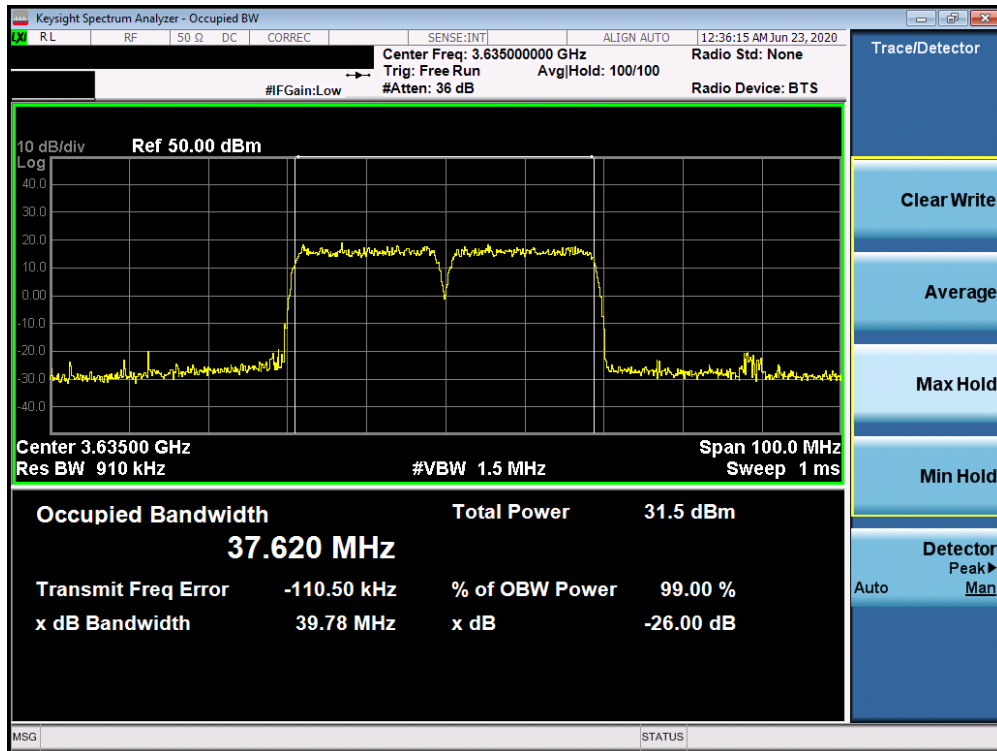
Plot 7-31. Occupied Bandwidth Plot (LTE Band 48 (ULCA) 20 + 20.0MHz 64-QAM - Full RB Configuration)
