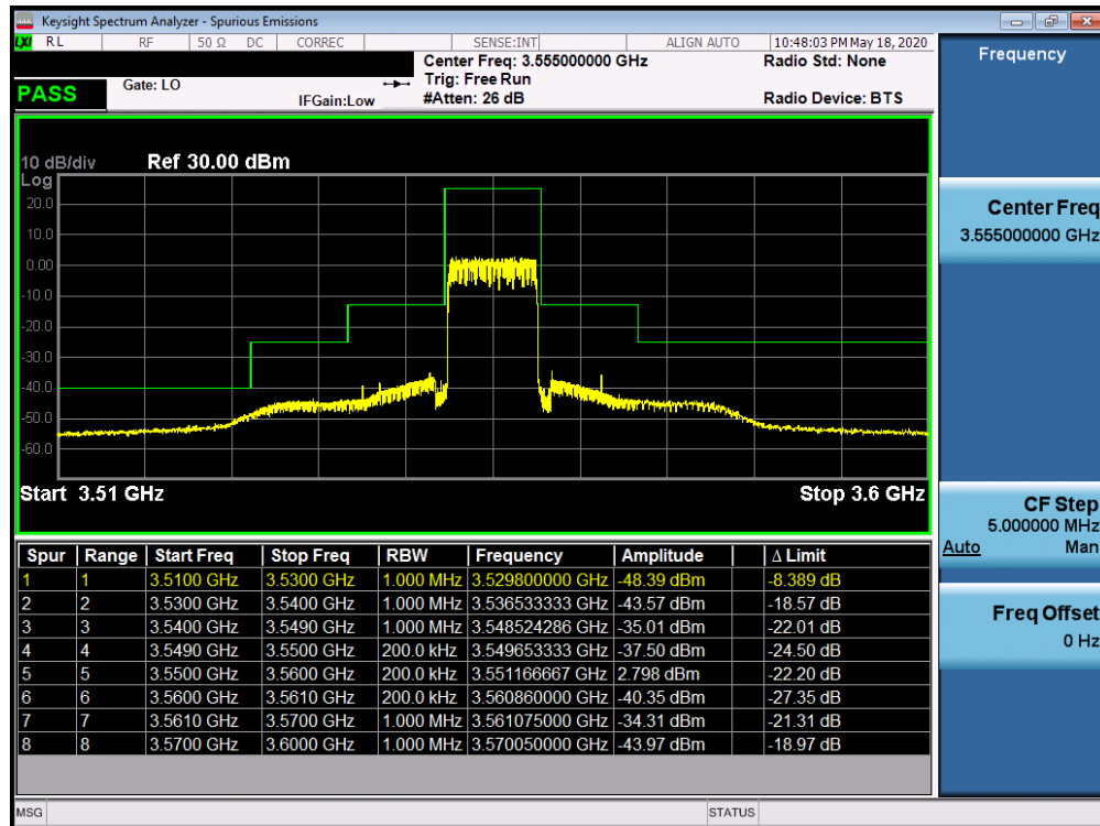
Plot 7-55. Lower ACP Plot (LTE Band 48 - 10.0MHz QPSK - Full RB Configuration)
