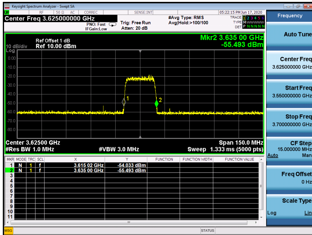
Plot 7-87. Run#1 End User Device Frequency of Operations
