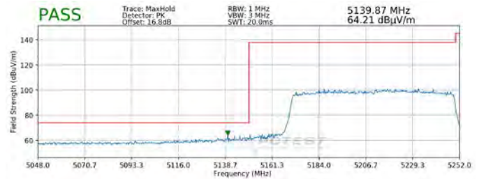
Plot 7-303. Radiated Lower Band Edge Plot SISO ANT1 (Peak – UNII Band 1)
