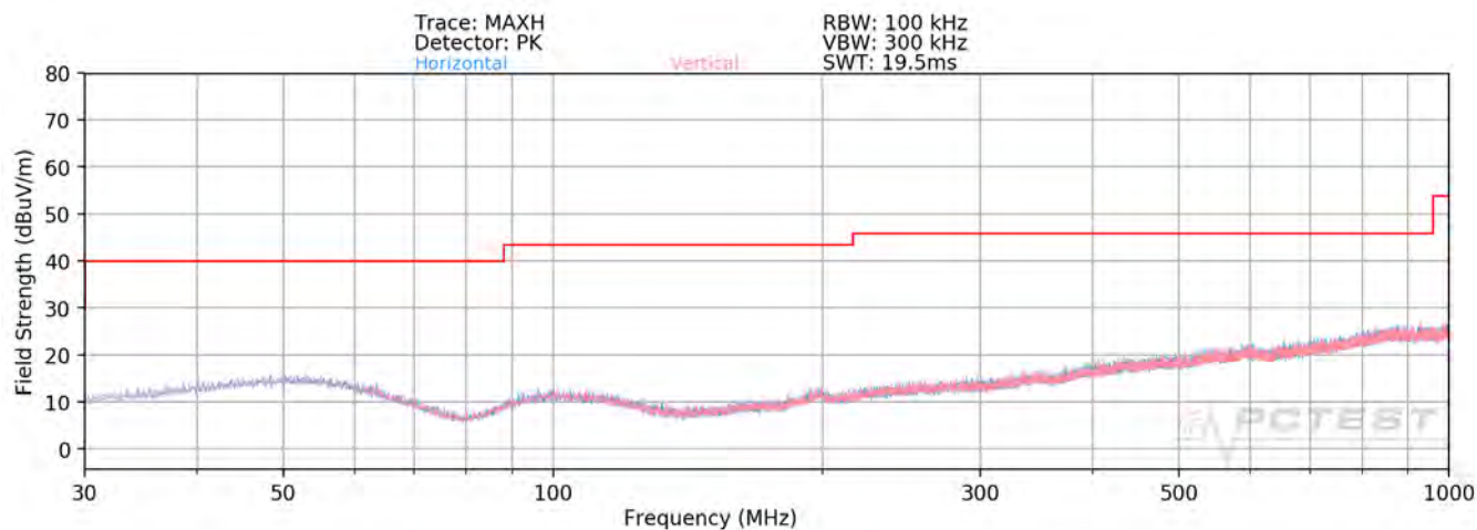
Plot 7-351. Radiated Spurious Plot below 1GHz MIMO ANT1 (802.11a – U3 Ch. 157)
