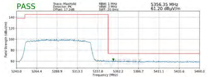
Plot 7-305. Radiated Upper Band Edge Plot SISO ANT1 (Peak – UNII Band 2A)
