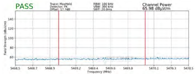
Plot 7-335. Radiated Lower Band Edge Plot MIMO (Peak – UNII Band 2C)
