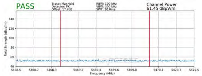
Plot 7-349. Radiated Lower Band Edge Plot MIMO (Peak - UNII Band 2C)
