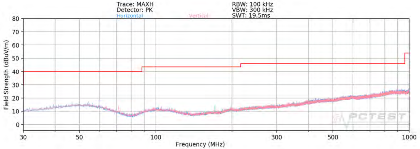
Plot 7-352. Radiated Spurious Plot be 1GHz (2.4GHz – 5GHz)
