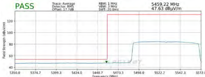
Plot 7-327. Radiated Lower Band Edge Plot SISO ANT2 (Average – UNII Band 2C)
