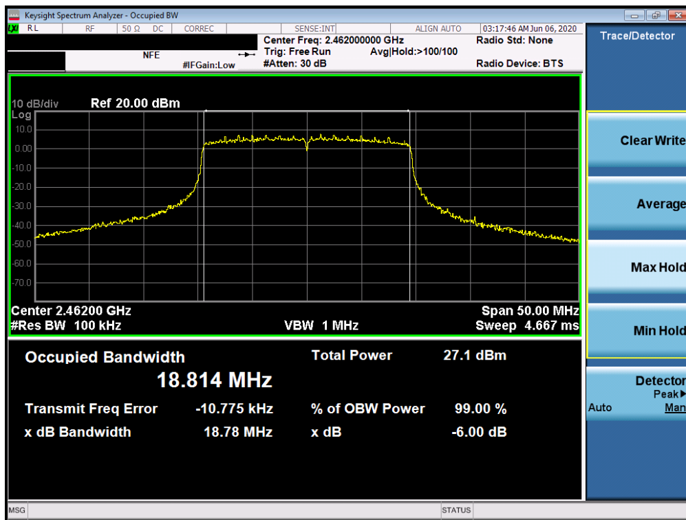
Plot 7-24. 6dB Bandwidth Plot SISO ANT1 (802.11ax SU – Ch. 11)
