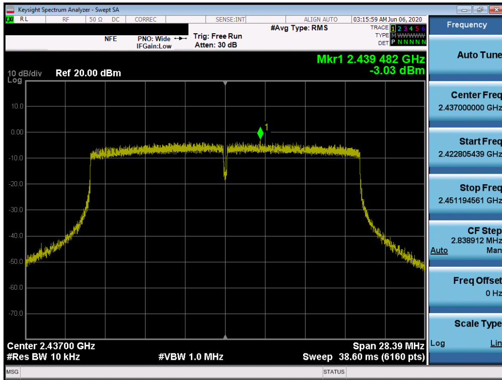
Plot 7-47. Power Spectral Density Plot SISO ANT2 (802.11ax SU – Ch. 6)
