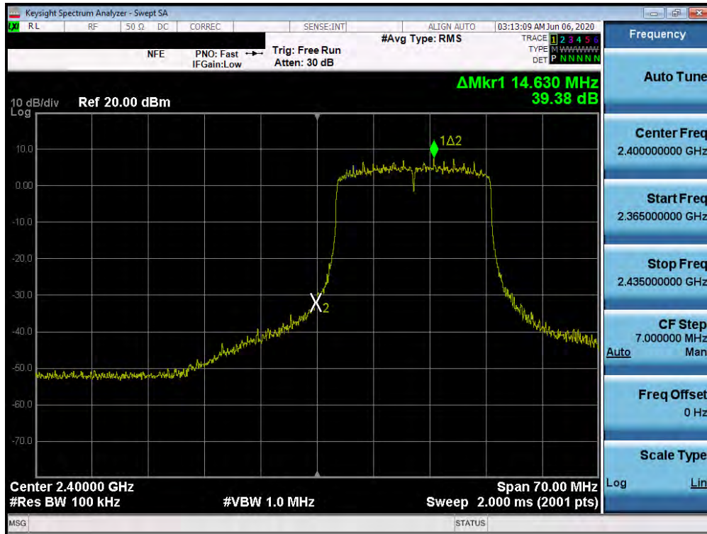
Plot 7-77. Band Edge Plot SISO ANT2 (802.11ax SU – Ch. 1)
