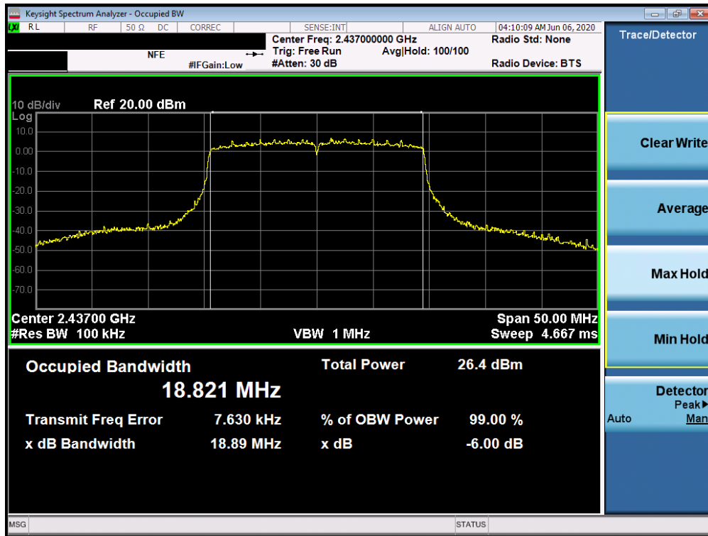
Plot 7-11. 6dB Bandwidth Plot SISO ANT1 (802.11ax SU - Ch. 6)
