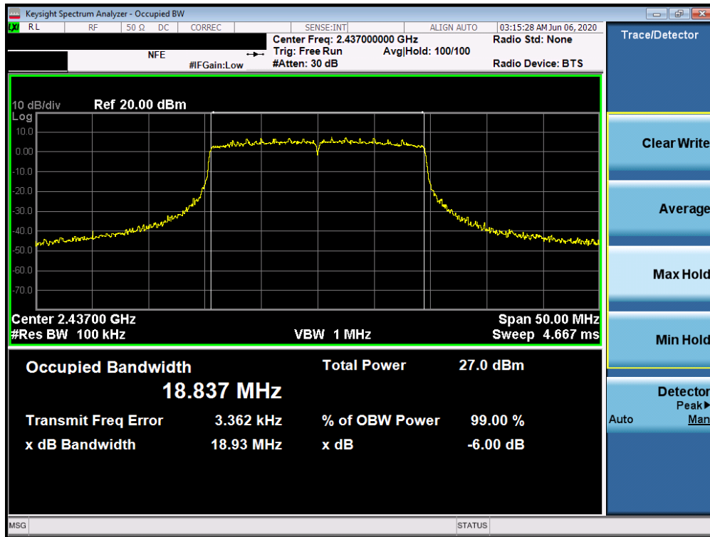
Plot 7-23. 6dB Bandwidth Plot SISO ANT1 (802.11ax SU – Ch. 6)
