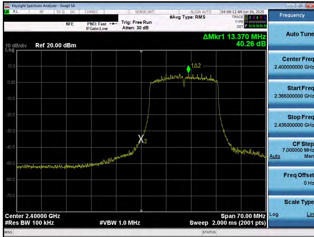
Plot 7-61. Band Edge Plot SISO ANT1 (802.11ax SU – Ch. 1)
