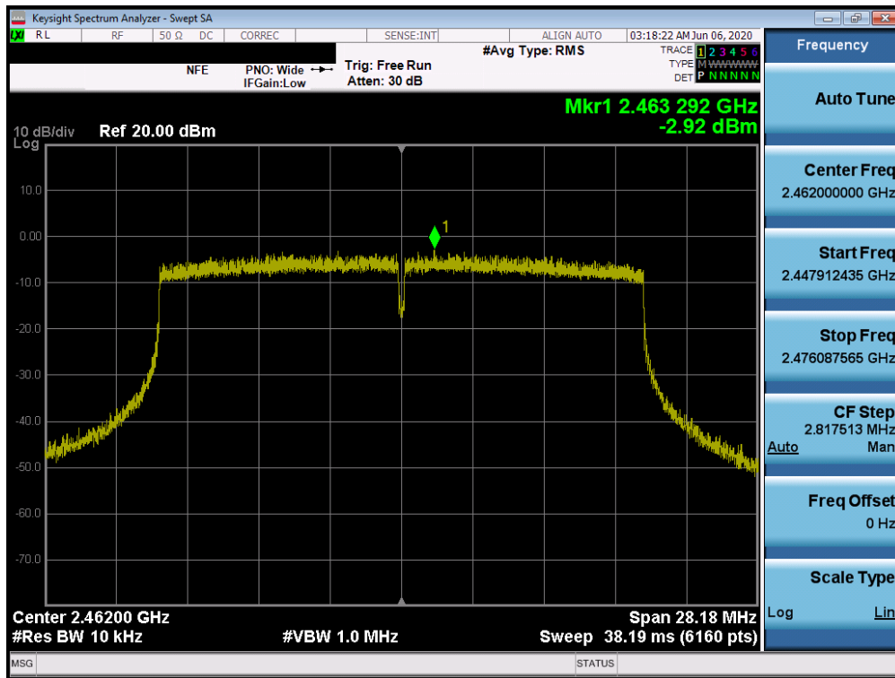
Plot 7-48. Power Spectral Density Plot SISO ANT2 (802.11ax SU – Ch. 11)
