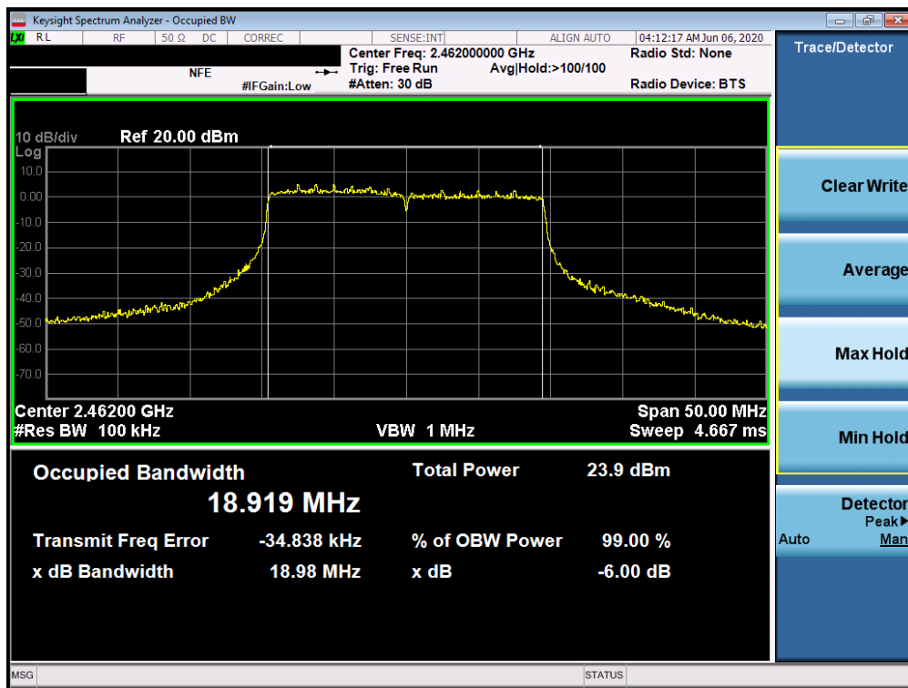
Plot 7-12. 6dB Bandwidth Plot SISO ANT1 (802.11ax SU - Ch. 11)
