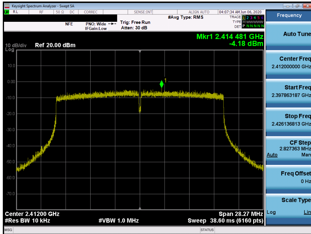
Plot 7-34. Power Spectral Density Plot SISO ANT1 (802.11ax SU – Ch. 1)
