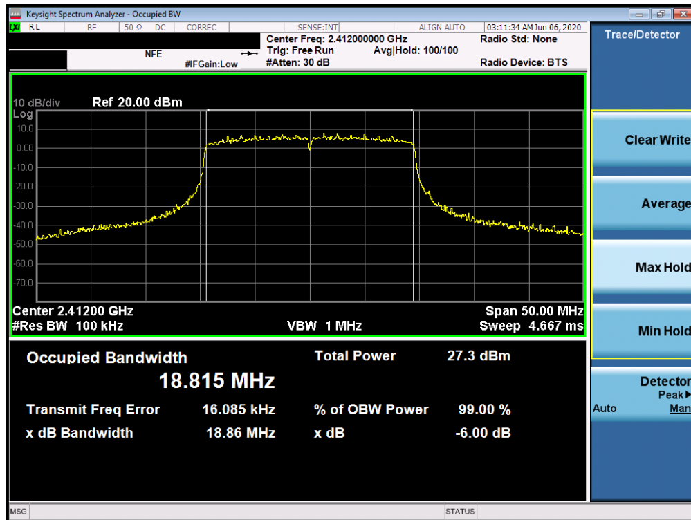
Plot 7-22. 6dB Bandwidth Plot SISO ANT1 (802.11ax SU – Ch. 1)
