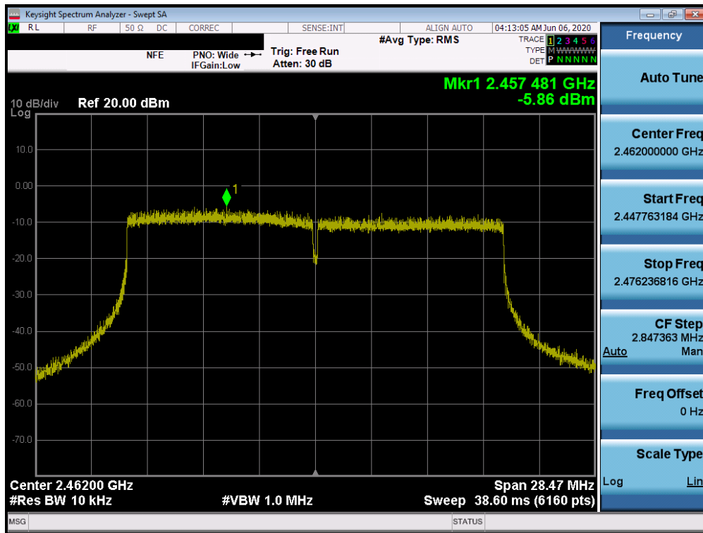
Plot 7-36. Power Spectral Density Plot SISO ANT1 (802.11ax SU – Ch. 11)
