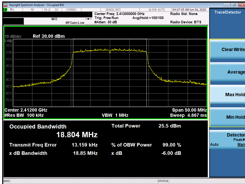
Plot 7-10. 6dB Bandwidth Plot SISO ANT1 (802.11ax SU – Ch. 1)
