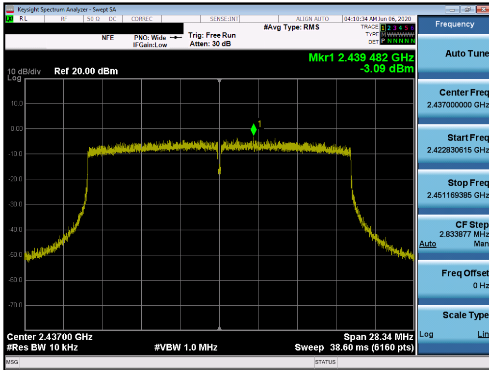
Plot 7-35. Power Spectral Density Plot SISO ANT1 (802.11ax SU – Ch. 6)
