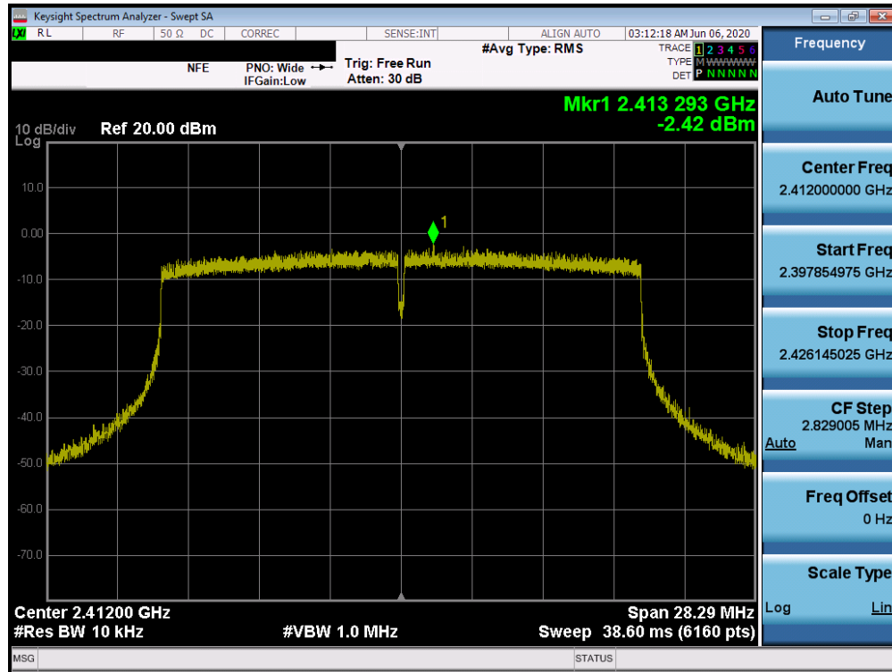
Plot 7-46. Power Spectral Density Plot SISO ANT2 (802.11ax SU – Ch. 1)
