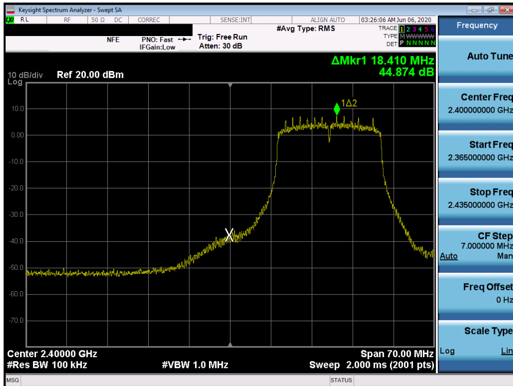
Plot 7-78. Band Edge Plot SISO ANT2 (802.11ax SU – Ch. 2)
