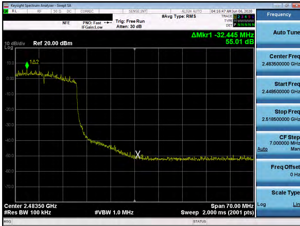
Plot 7-63. Band Edge Plot SISO ANT1 (802.11ax SU – Ch. 10)
