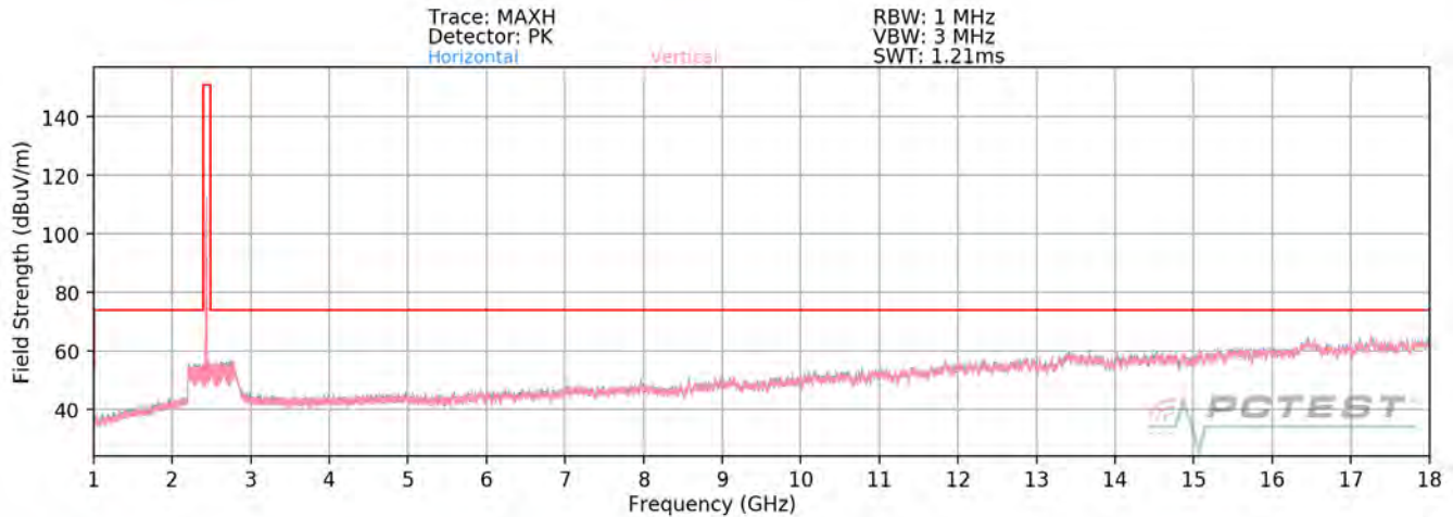
Plot 7-94. Radiated Spurious Plot above 1GHz SISO ANT1 (802.11b – Ch. 6)
