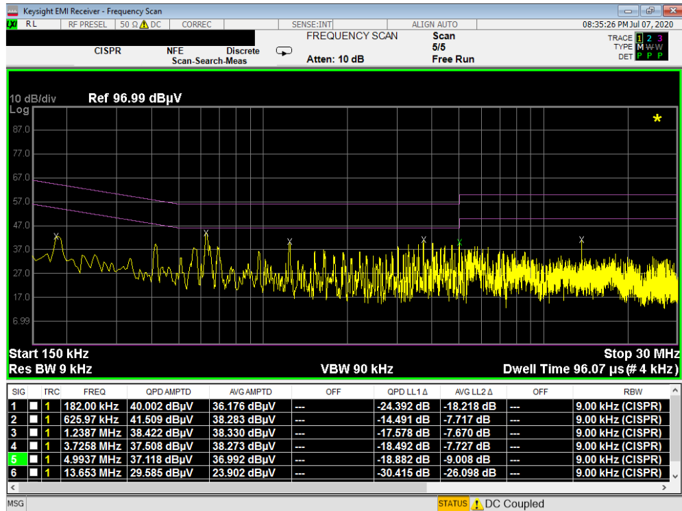
Plot 7-133. Line Conducted Plot with 802.11b (N) with WCP
