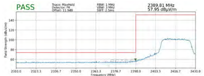
Plot 7-116. Radiated Restricted Lower Band Edge Measurement SISO ANT2 (Peak)
