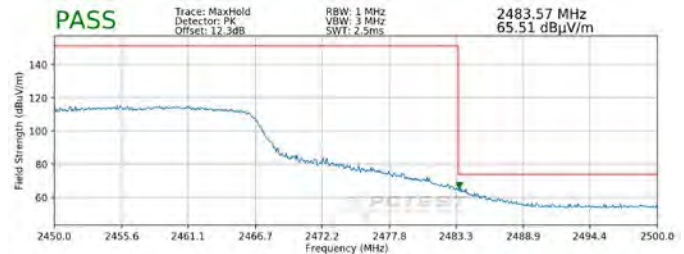
Plot 7-126. Radiated Restricted Upper Band Edge Measurement MIMO (Peak)
