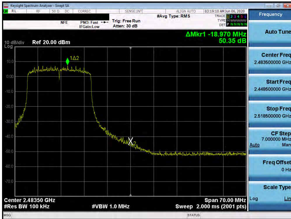
Plot 7-80. Band Edge Plot SISO ANT2 (802.11ax SU - Ch. 11)
