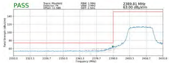
Plot 7-114. Radiated Restricted Lower Band Edge Measurement SISO ANT2 (Peak)
