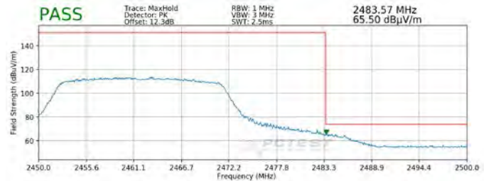
Plot 7-128. Radiated Restricted Upper Band Edge Measurement MIMO (Peak)
