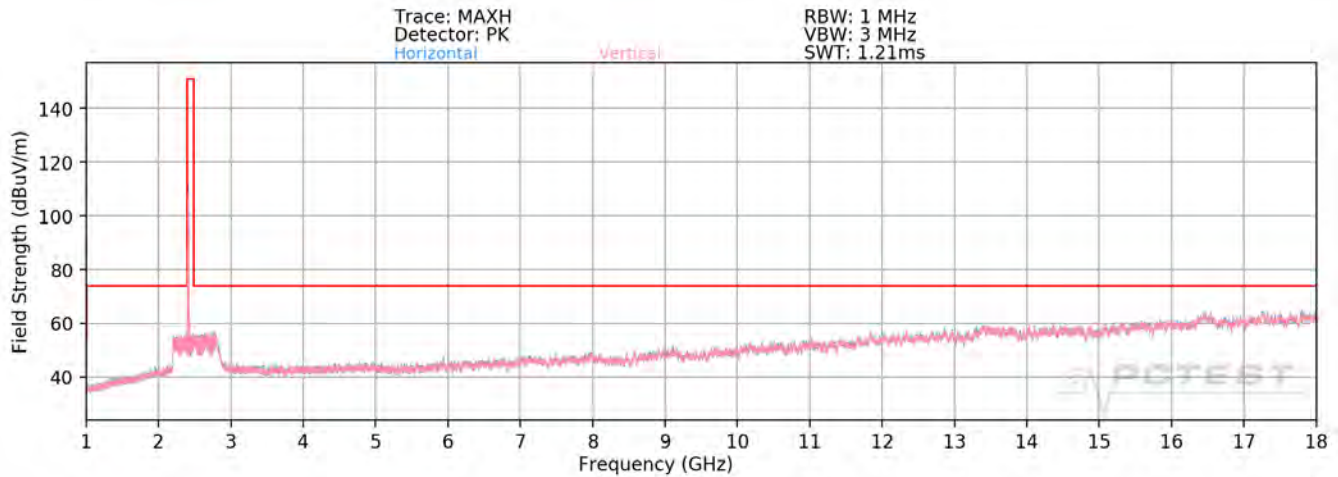
Plot 7-93. Radiated Spurious Plot above 1GHz SISO ANT1 (802.11b – Ch. 1)
