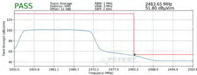
Plot 7-127. Radiated Restricted Upper Band Edge Measurement MIMO (Average)
