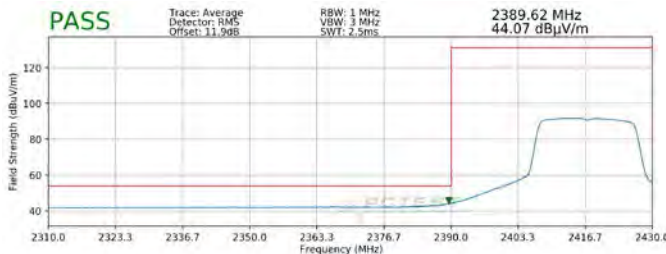
Plot 7-115. Radiated Restricted Lower Band Edge Measurement SISO ANT2 (Average)
