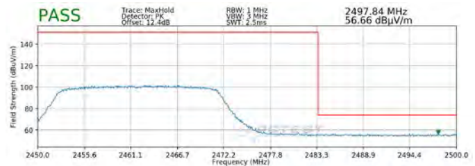
Plot 7-120. Radiated Restricted Upper Band Edge Measurement SISO ANT2 (Peak)
