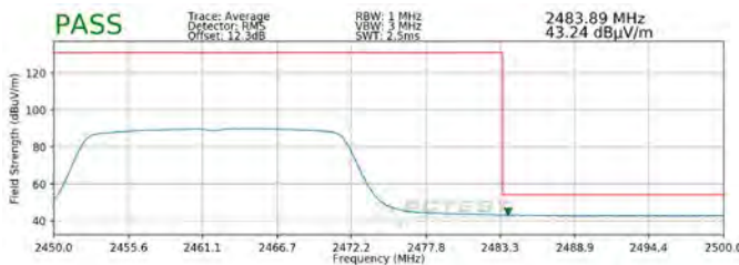
Plot 7-119. Radiated Restricted Upper Band Edge Measurement SISO ANT2 (Average)
