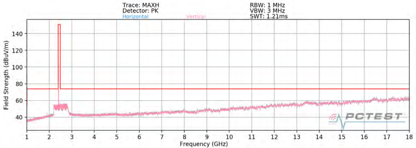
Plot 7-97. Radiated Spurious Plot above 1GHz SISO ANT2 (802.11b – Ch. 1)
