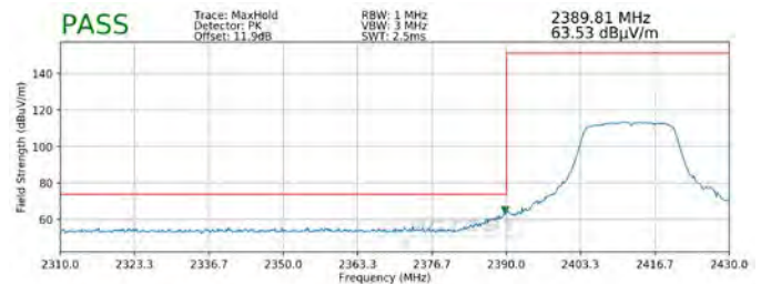
Plot 7-106. Radiated Restricted Lower Band Edge Measurement SISO ANT1 (Peak)
