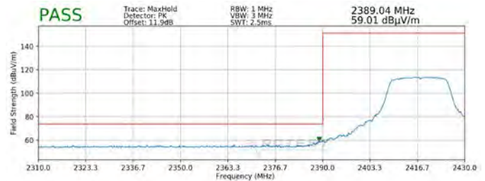
Plot 7-108. Radiated Restricted Lower Band Edge Measurement SISO ANT1 (Peak)
