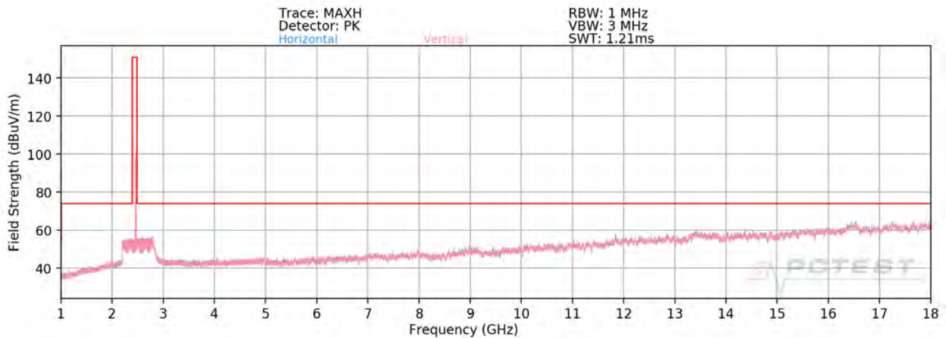
Plot 7-99. Radiated Spurious Plot above 1GHz SISO ANT2 (802.11b – Ch. 11)
