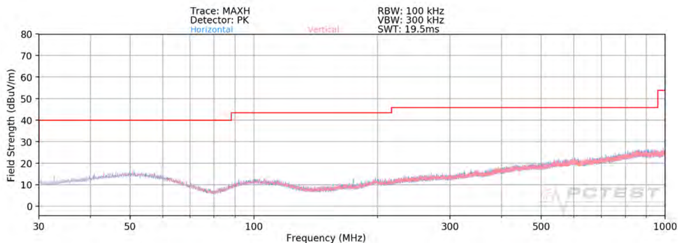
Plot 7-129. Radiated Spurious Plot below 1GHz MIMO
