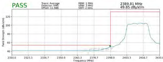
Plot 7-121. Radiated Restricted Lower Band Edge Measurement MIMO (Average)
