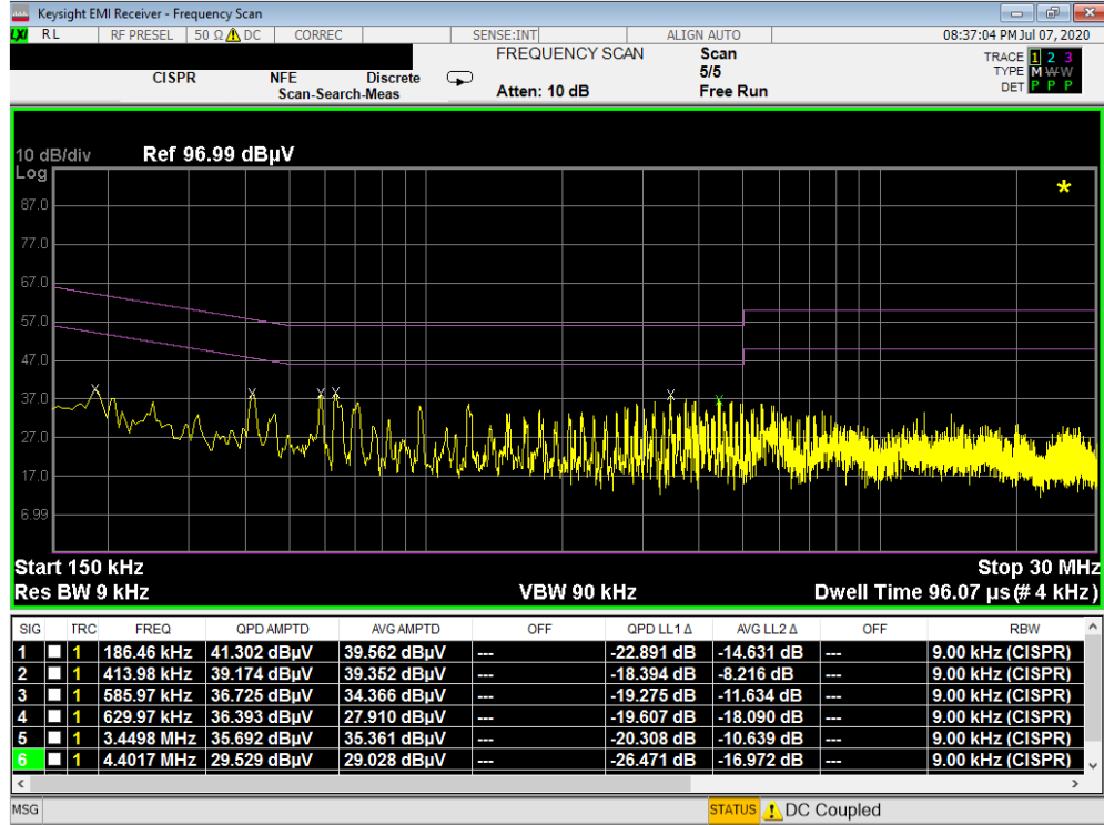
Plot 7-132. Line Conducted Plot with 802.11b (L1) with WCP
