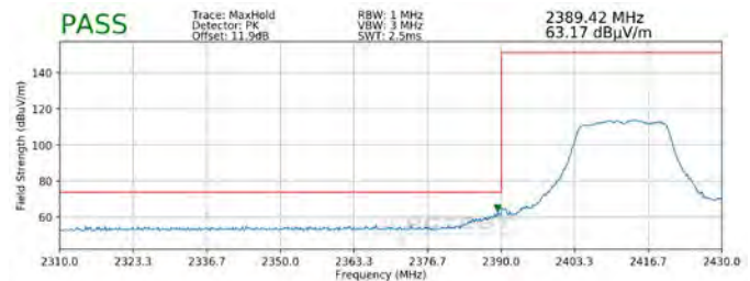
Plot 7-122. Radiated Restricted Lower Band Edge Measurement MIMO (Peak)
