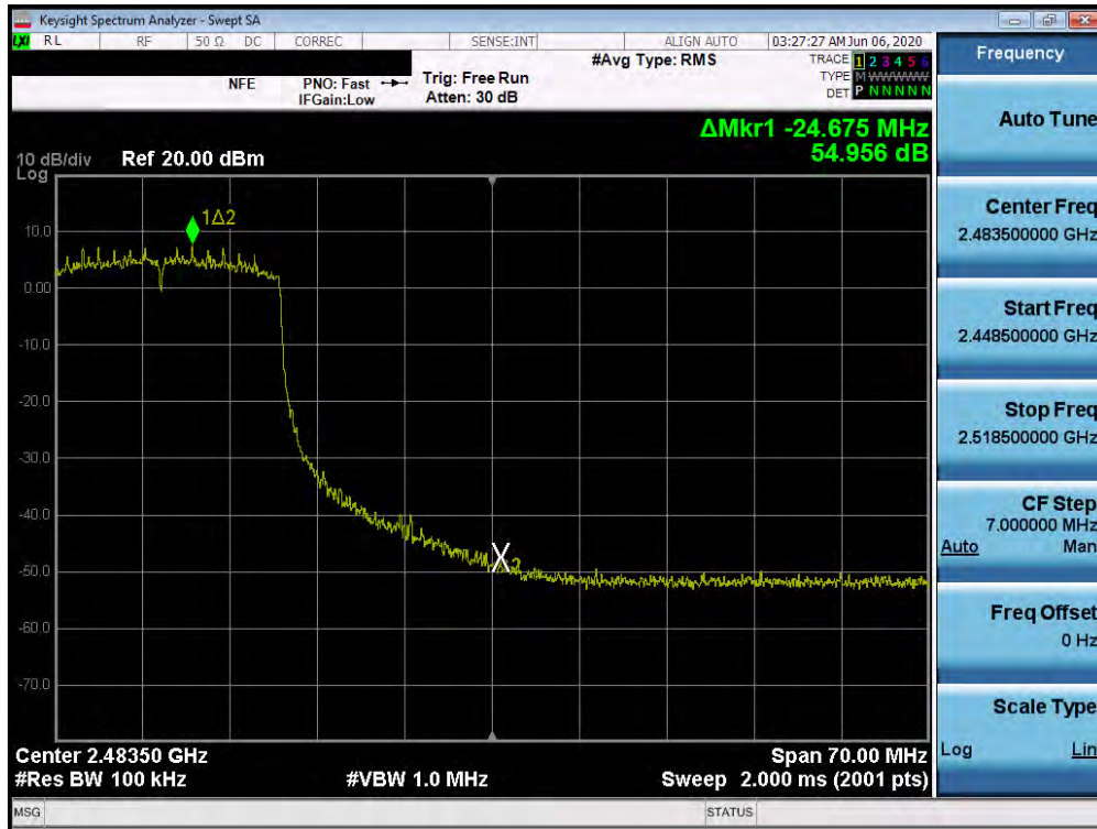
Plot 7-79. Band Edge Plot SISO ANT2 (802.11ax SU - Ch. 10)
