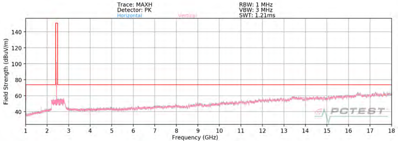
Plot 7-98. Radiated Spurious Plot above 1GHz SISO ANT2 (802.11b – Ch. 6)
