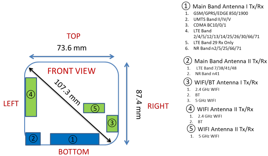
Figure E-3 DUT Antenna Locations Closed Configuration
