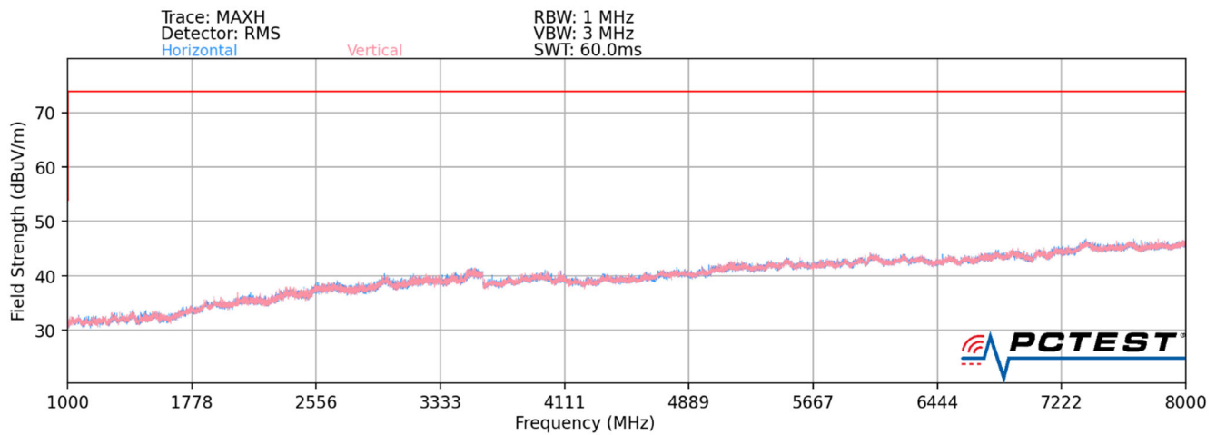
Plot 7-3. Radiated Spurious Plot above 1GHz – Open
