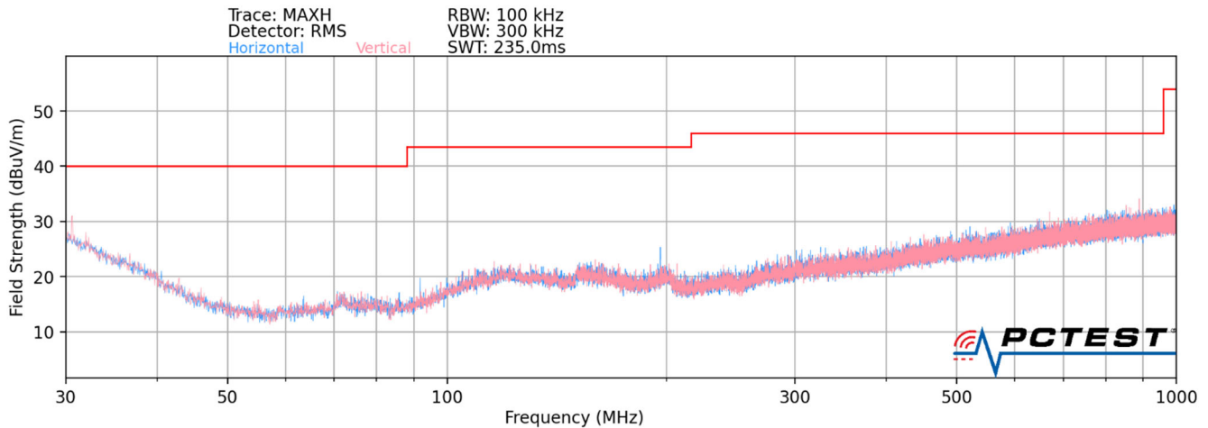
Plot 7-2. Radiated Spurious Plot below 1GHz – Closed
