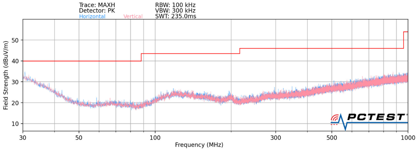
Plot 7-1. Radiated Spurious Plot below 1GHz – Open
