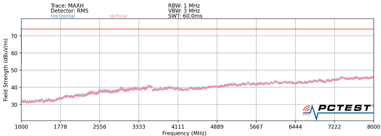
Plot 7-4. Radiated Spurious Plot above 1GHz – Closed
