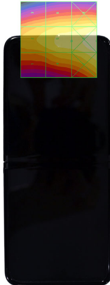
Figure 18-4 E-Field WD Scan overlay
