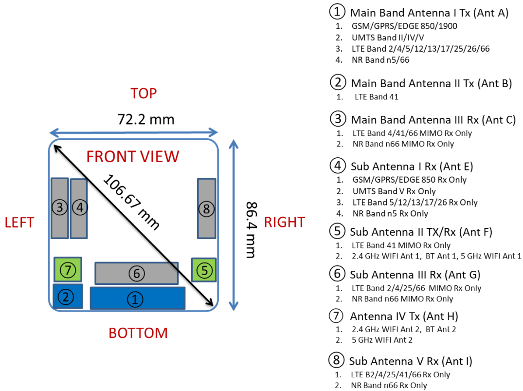
Figure E-3 DUT Antenna Locations Closed Configuration
