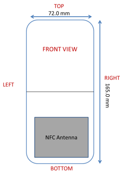
Figure E-2 NFC Antenna Open Configuration Locations
