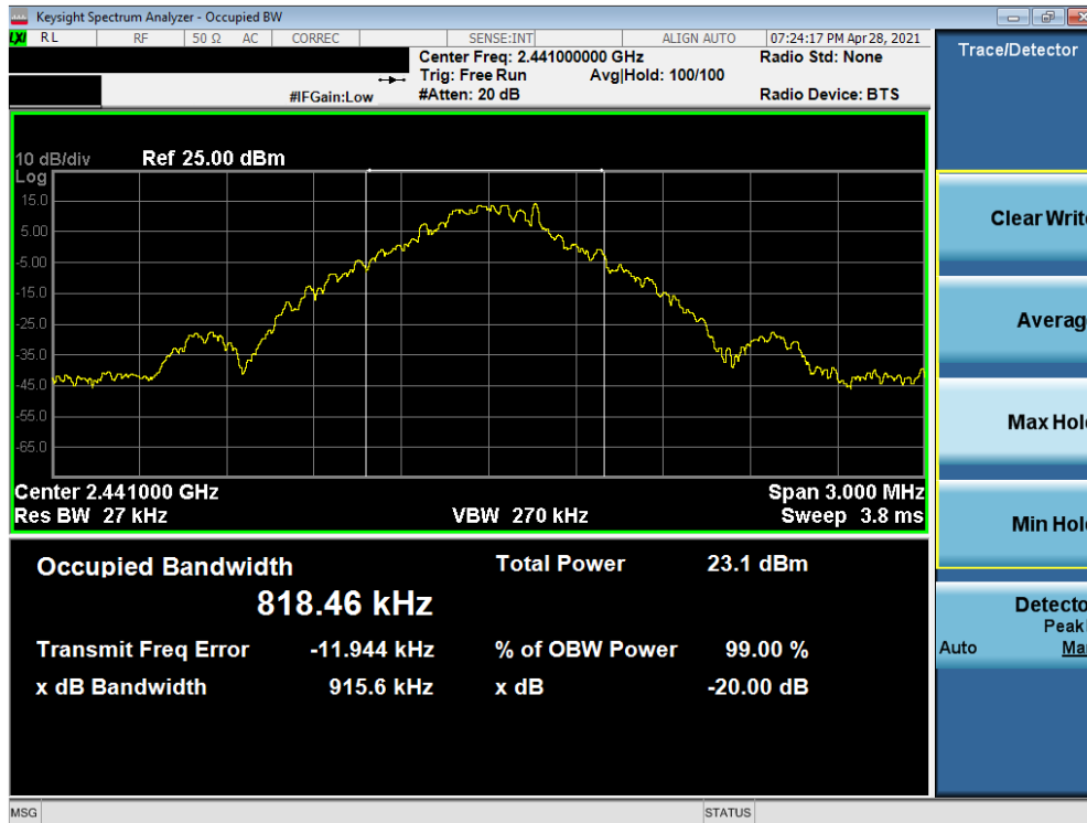
Plot 7-20. 20dB Bandwidth Plot (Bluetooth, 1Mbps, ePA – Ch. 39) – ANT1
