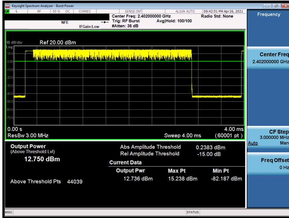
Plot 7-67. Average Conducted Power (3Mbps, ePA – Ch. 0) – ANT0
