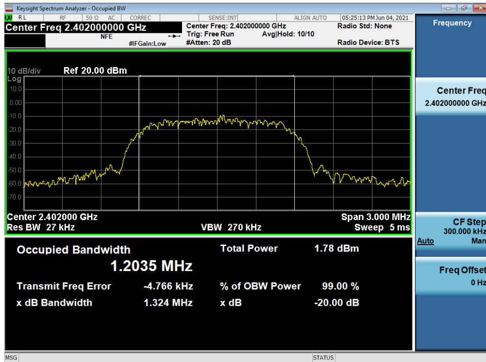
Plot 7-16. 20dB Bandwidth Plot (Bluetooth, 3Mbps, iPA - Ch. 0) - ANT0
