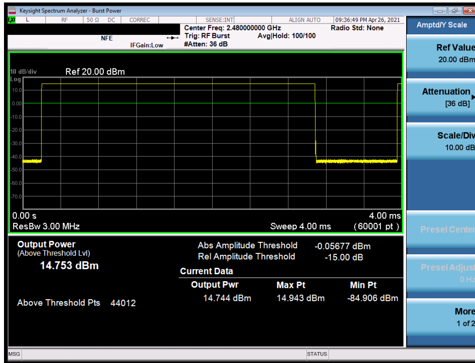
Plot 7-57. Average Conducted Power (1Mbps, ePA - Ch. 78) - ANT0
