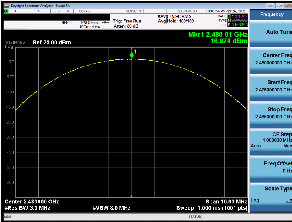
Plot 7-81. Peak Conducted Power (2Mbps, ePA – Ch. 78) – ANT1
