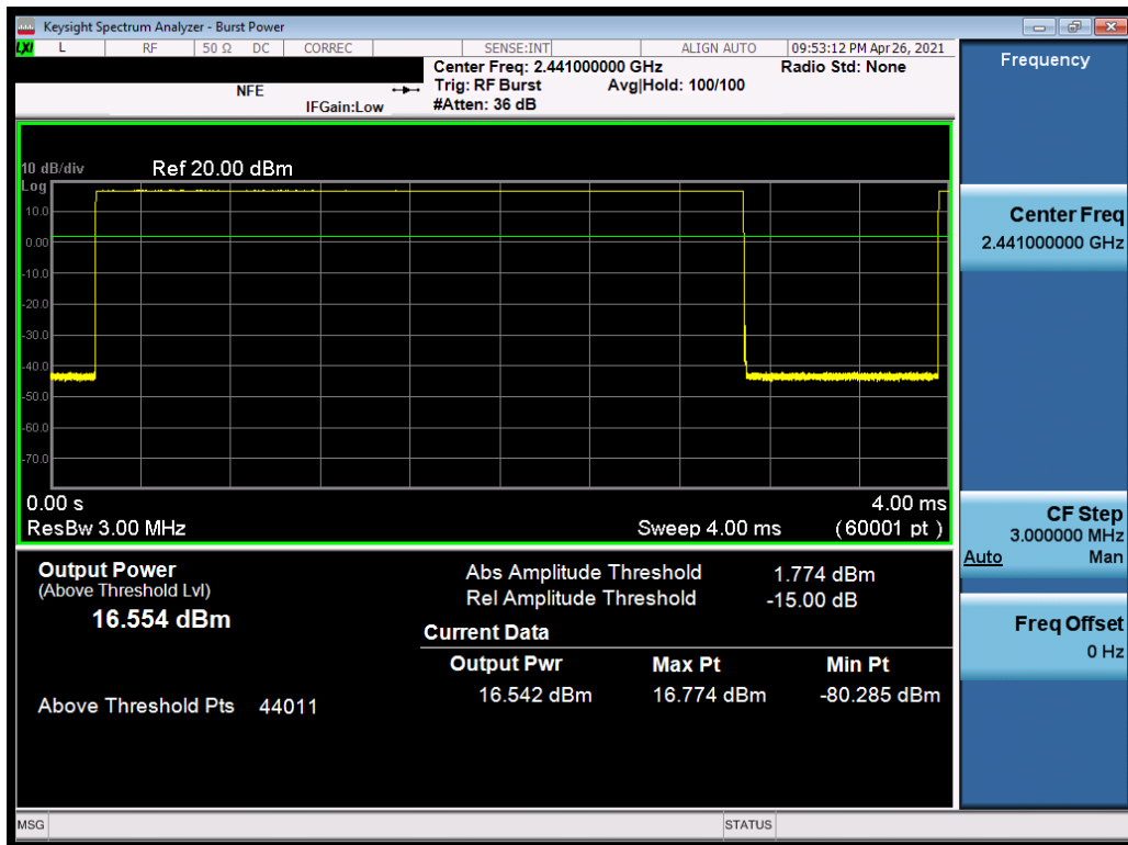
Plot 7-92. Average Conducted Power (1Mbps, ePA – Ch. 39) – ANT1
