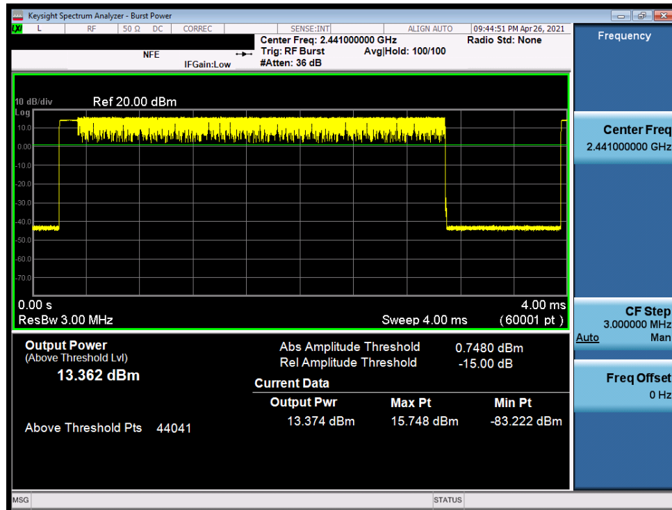
Plot 7-68. Average Conducted Power (3Mbps, ePA – Ch. 39) – ANT0
