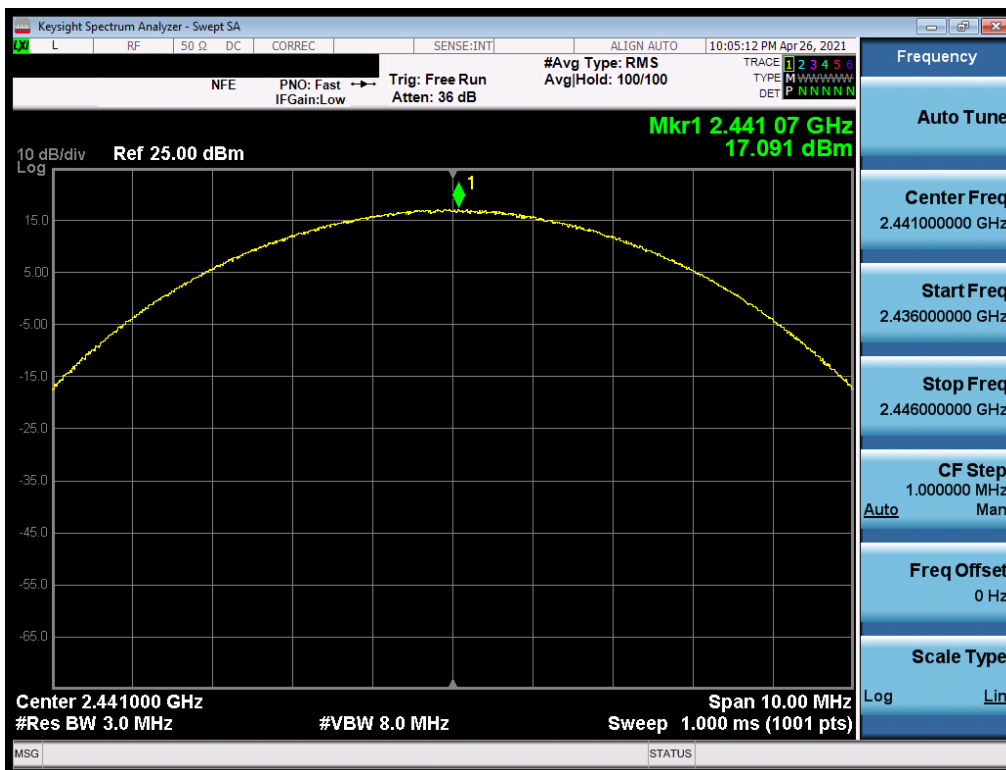
Plot 7-86. Peak Conducted Power (3Mbps, ePA - Ch. 39) - ANT1
