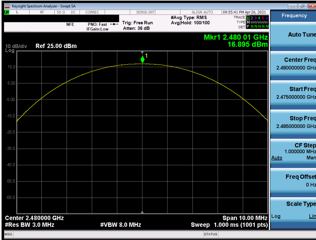
Plot 7-75. Peak Conducted Power (1Mbps, ePA - Ch. 78) - ANT1
