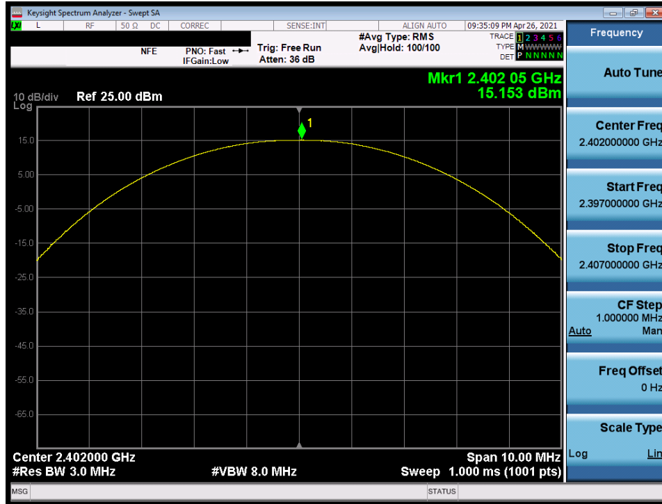
Plot 7-37. Peak Conducted Power (1Mbps, ePA - Ch. 0) – ANT0
