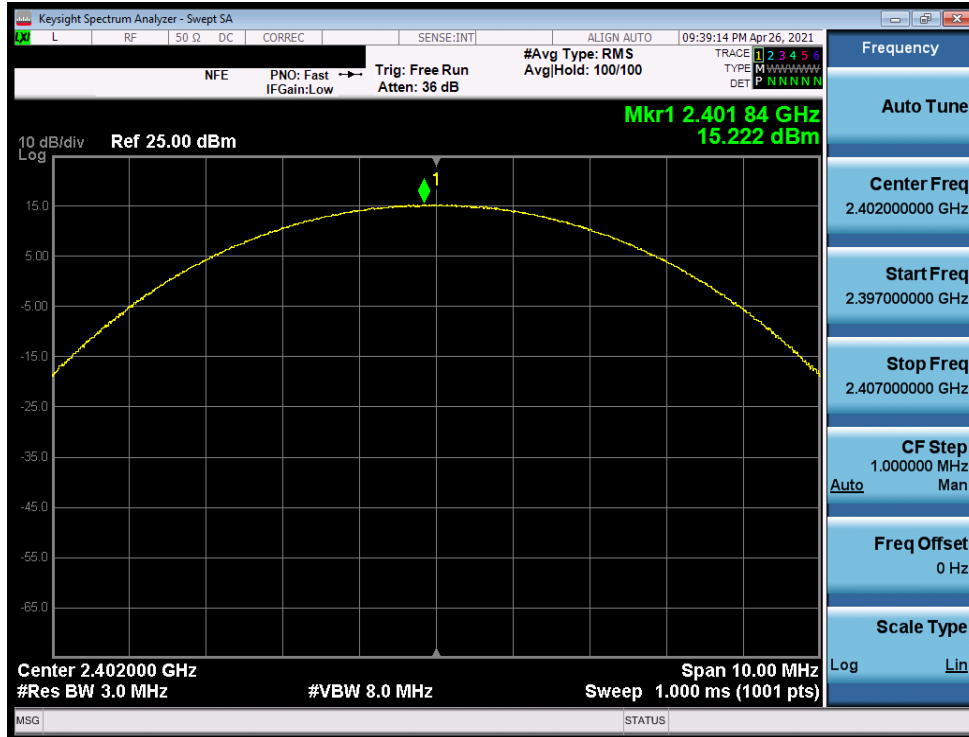
Plot 7-43. Peak Conducted Power (2Mbps, ePA - Ch. 0) - ANT0
