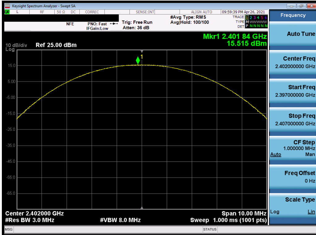
Plot 7-79. Peak Conducted Power (2Mbps, ePA - Ch. 0) - ANT1
