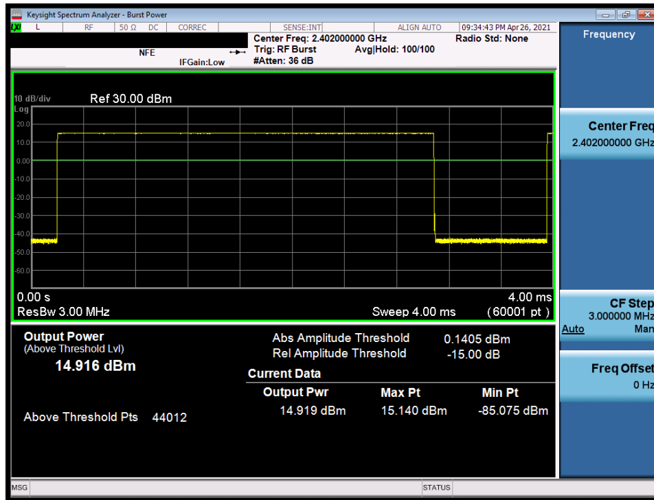
Plot 7-55. Average Conducted Power (1Mbps, ePA – Ch. 0) – ANT0
