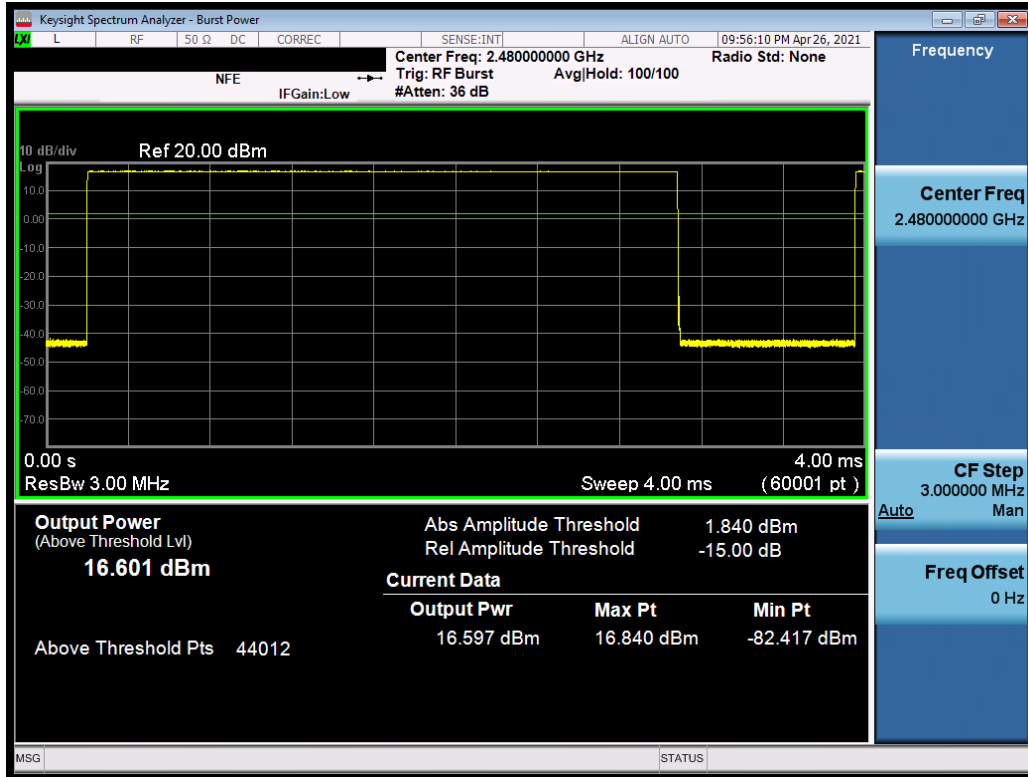
Plot 7-93. Average Conducted Power (1Mbps, ePA - Ch. 78) - ANT1
