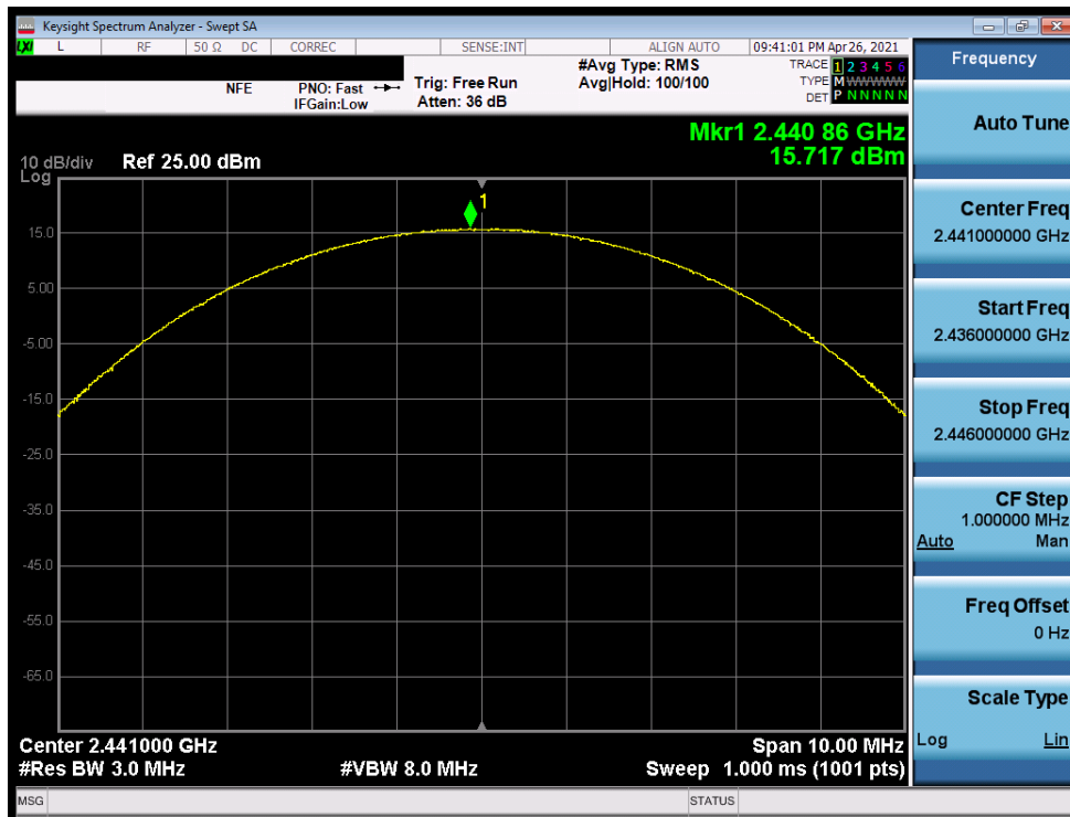
Plot 7-44. Peak Conducted Power (2Mbps, ePA - Ch. 39) - ANT0
