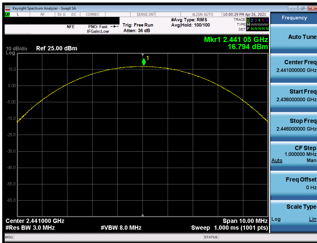
Plot 7-80. Peak Conducted Power (2Mbps, ePA - Ch. 39) - ANT1
