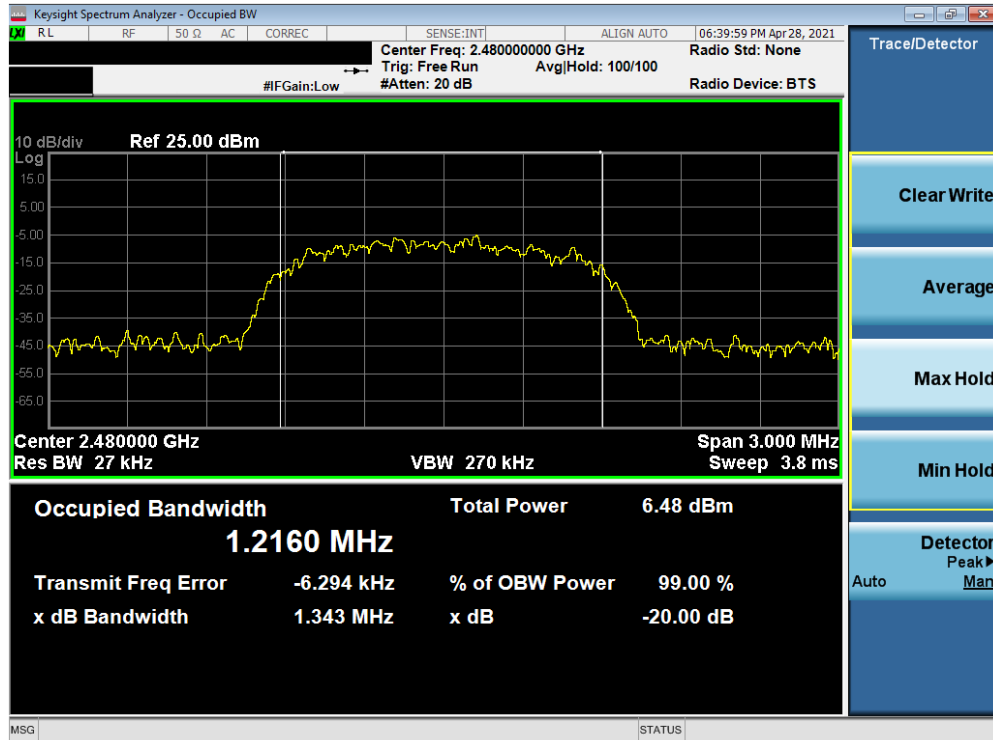
Plot 7-15. 20dB Bandwidth Plot (Bluetooth, 3Mbps, ePA - Ch. 78) - ANT0
