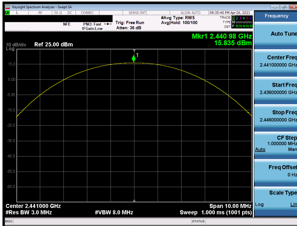
Plot 7-38. Peak Conducted Power (1Mbps, ePA - Ch. 39) – ANT0
