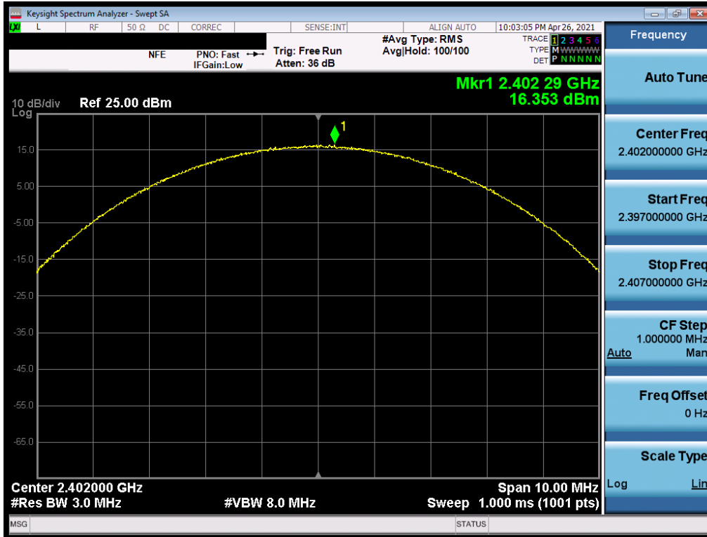
Plot 7-85. Peak Conducted Power (3Mbps, ePA - Ch. 0) - ANT1
