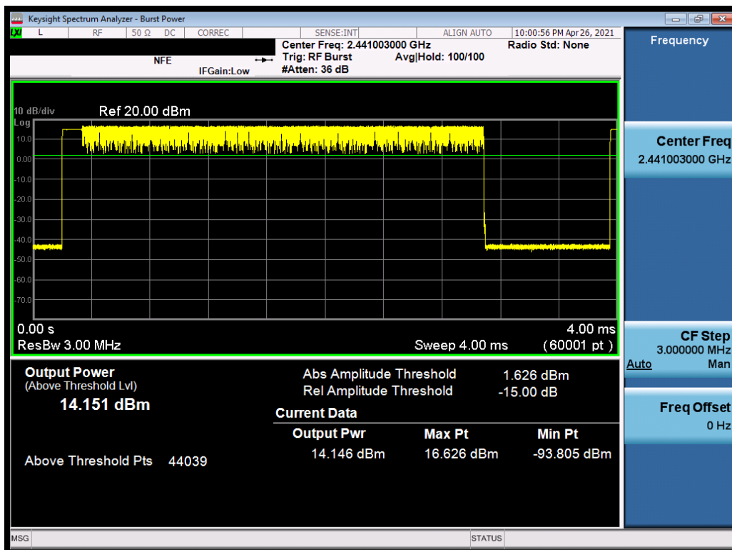
Plot 7-98. Average Conducted Power (2Mbps, ePA – Ch. 39) – ANT1
