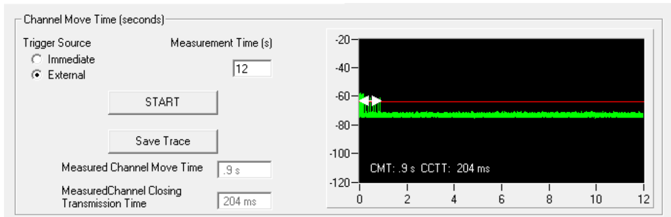
Figure 9-2. 5510MHz CMT and CCTT
