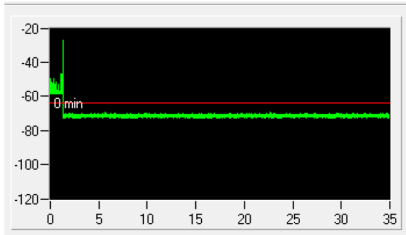
Figure 9-3. 5590MHz Client Beacon Test – Monitoring live spectrum – Elapse time 30 minutes
