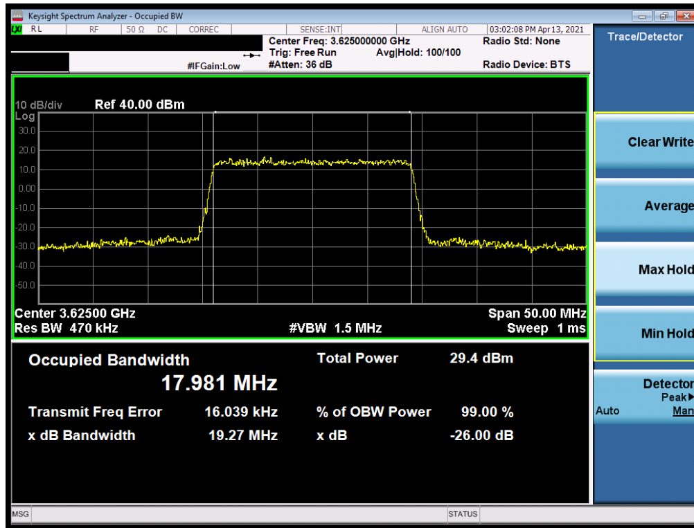
Plot 7-1. Occupied Bandwidth Plot (LTE Band 48 - 20MHz QPSK - Full RB Configuration)
