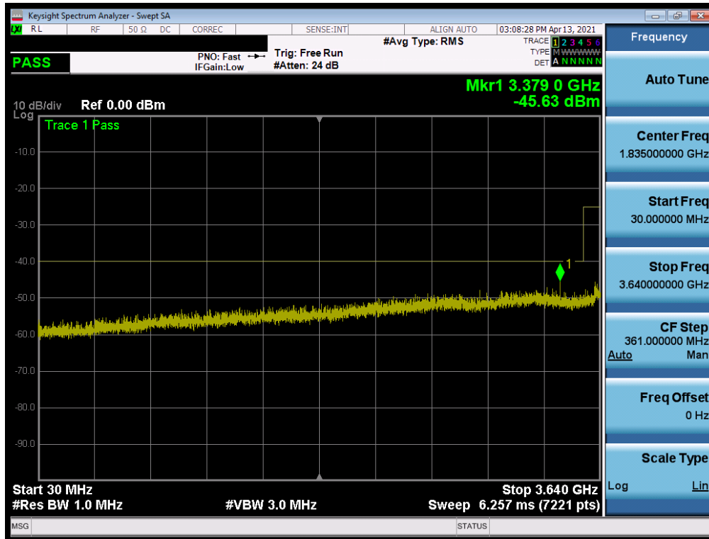
Plot 7-25. Conducted Spurious Plot (LTE Band 48 - 20MHz QPSK - RB Size 1, RB Offset 0 - High Channel)
