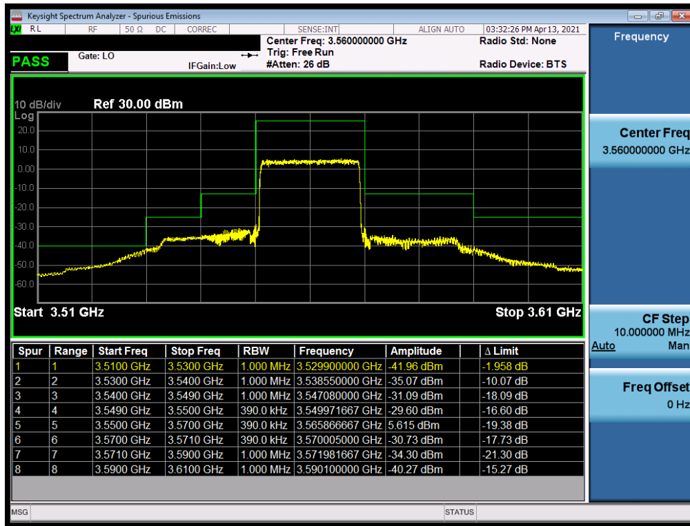
Plot 7-41. Channel Edge Plot (LTE Band 48 - 20MHz QPSK - Low Channel)
