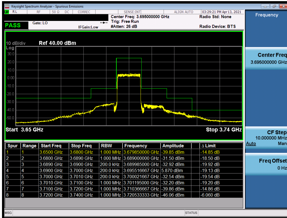
Plot 7-49. Channel Edge Plot (LTE Band 48 - 10MHz QPSK - High Channel)
