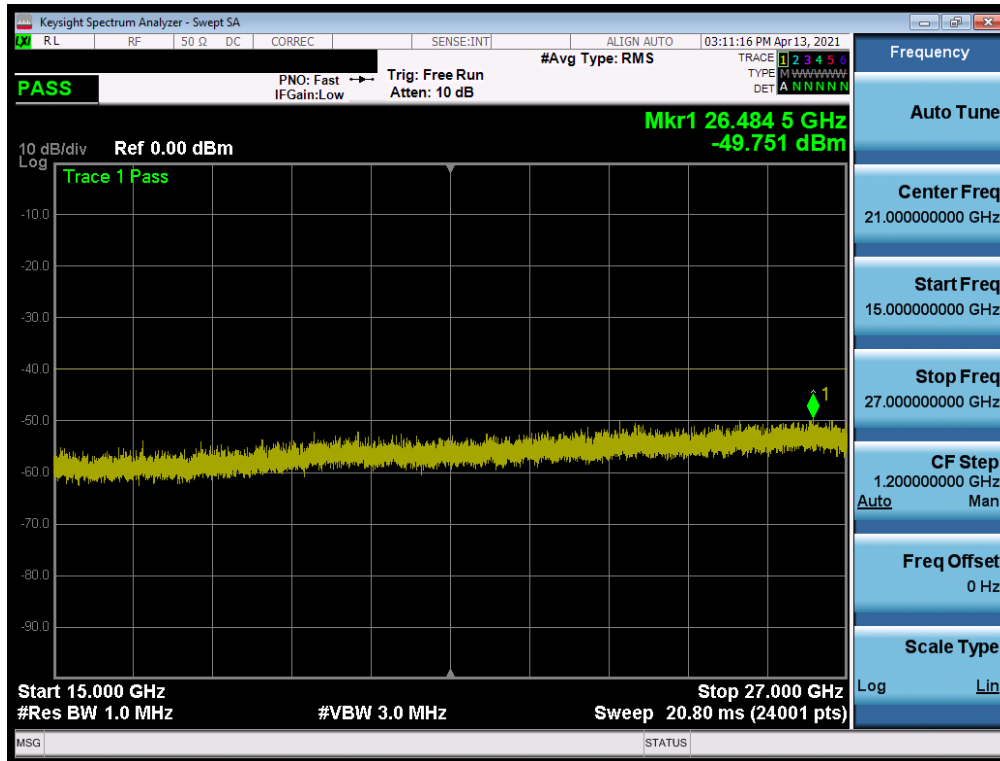
Plot 7-27. Conducted Spurious Plot (LTE Band 48 - 20MHz QPSK - RB Size 1, RB Offset 0 - High Channel)
