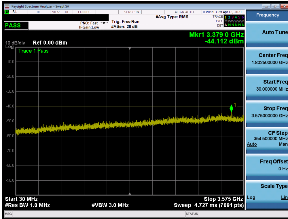
Plot 7-21. Conducted Spurious Plot (LTE Band 48 - 20MHz QPSK - RB Size 1, RB Offset 0 - Mid Channel)
