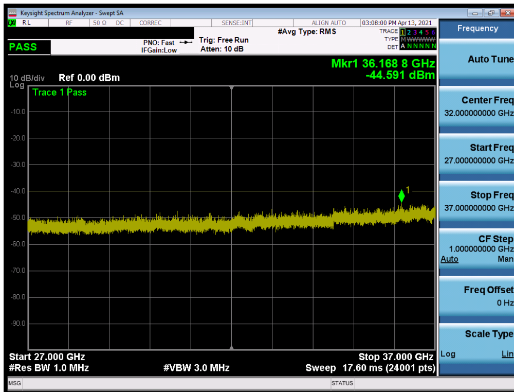
Plot 7-20. Conducted Spurious Plot (LTE Band 48 - 20MHz QPSK - RB Size 1, RB Offset 0 - Low Channel)
