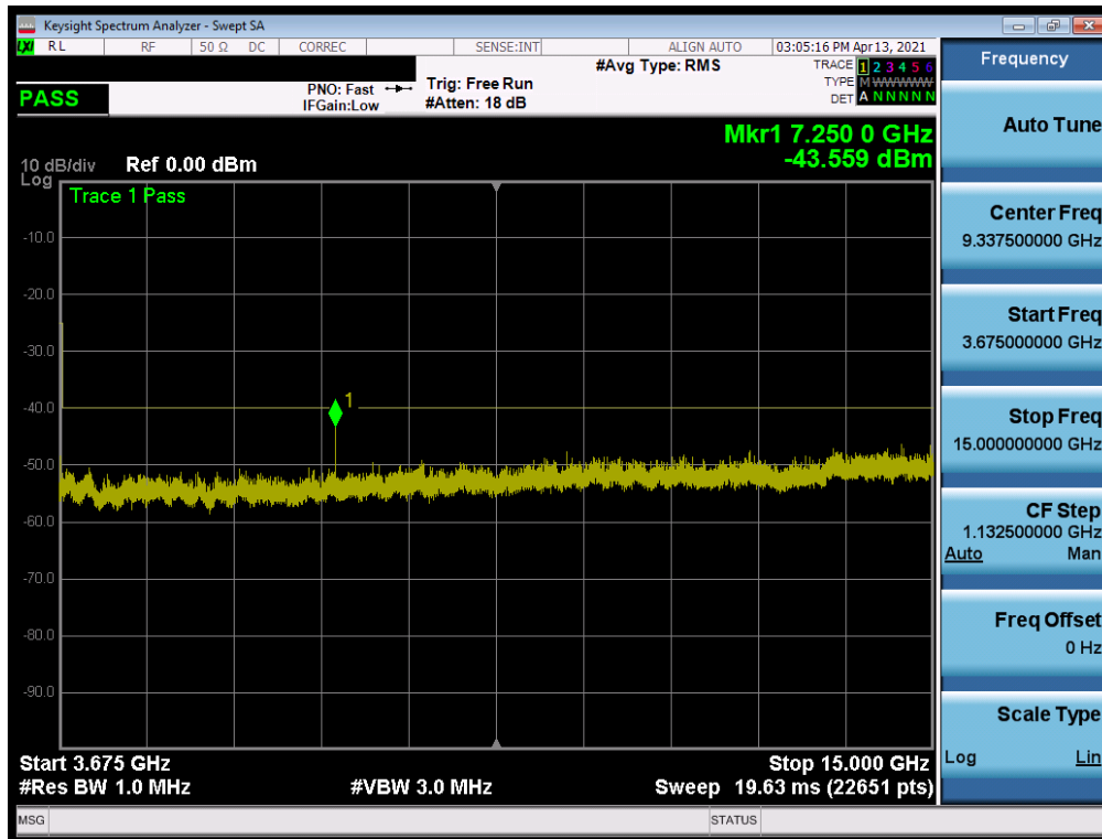
Plot 7-22. Conducted Spurious Plot (LTE Band 48 - 20MHz QPSK - RB Size 1, RB Offset 0 - Mid Channel)
