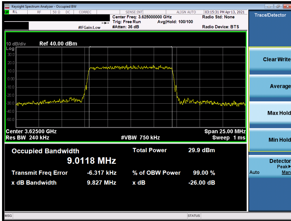
Plot 7-5. Occupied Bandwidth Plot (LTE Band 48 - 10MHz QPSK - Full RB Configuration)
