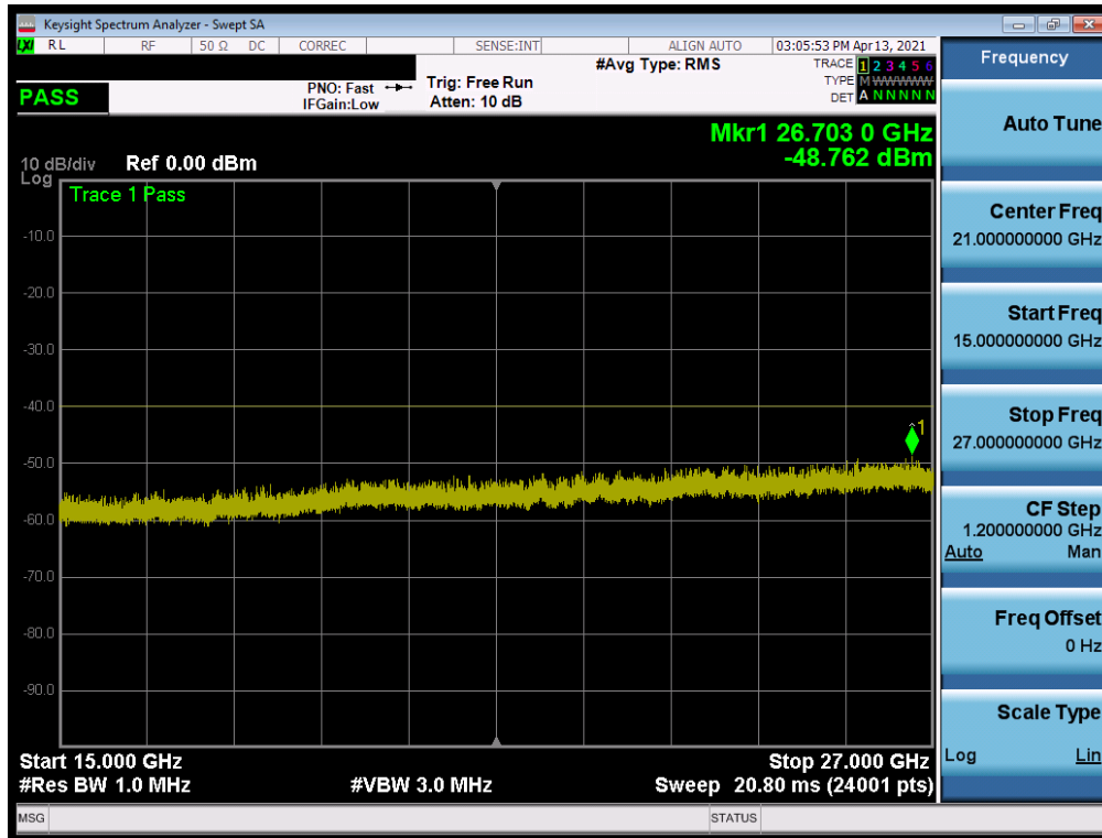
Plot 7-23. Conducted Spurious Plot (LTE Band 48 - 20MHz QPSK - RB Size 1, RB Offset 0 - Mid Channel)
