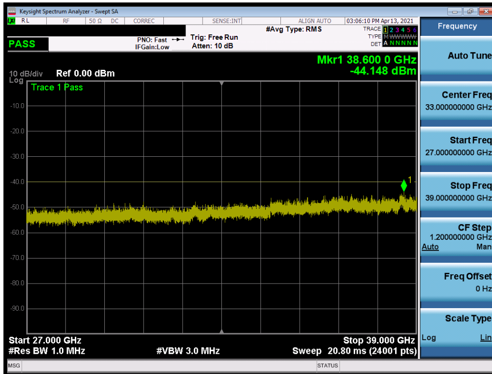
Plot 7-24. Conducted Spurious Plot (LTE Band 48 - 20MHz QPSK - RB Size 1, RB Offset 0 - Mid Channel)
