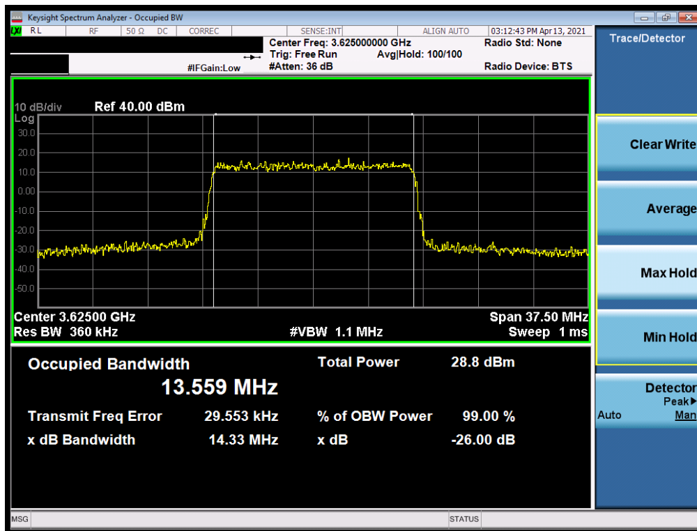
Plot 7-4. Occupied Bandwidth Plot (LTE Band 48 - 15MHz 16-QAM - Full RB Configuration)
