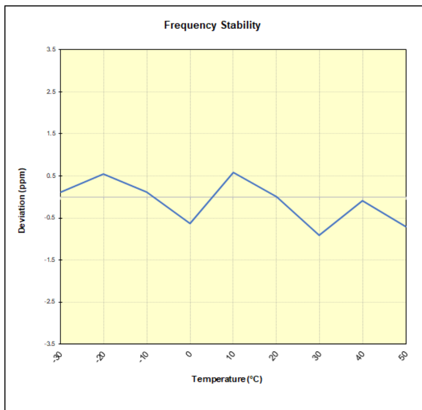
Plot 7-65. LTE Band 48 Frequency Stability Chart
