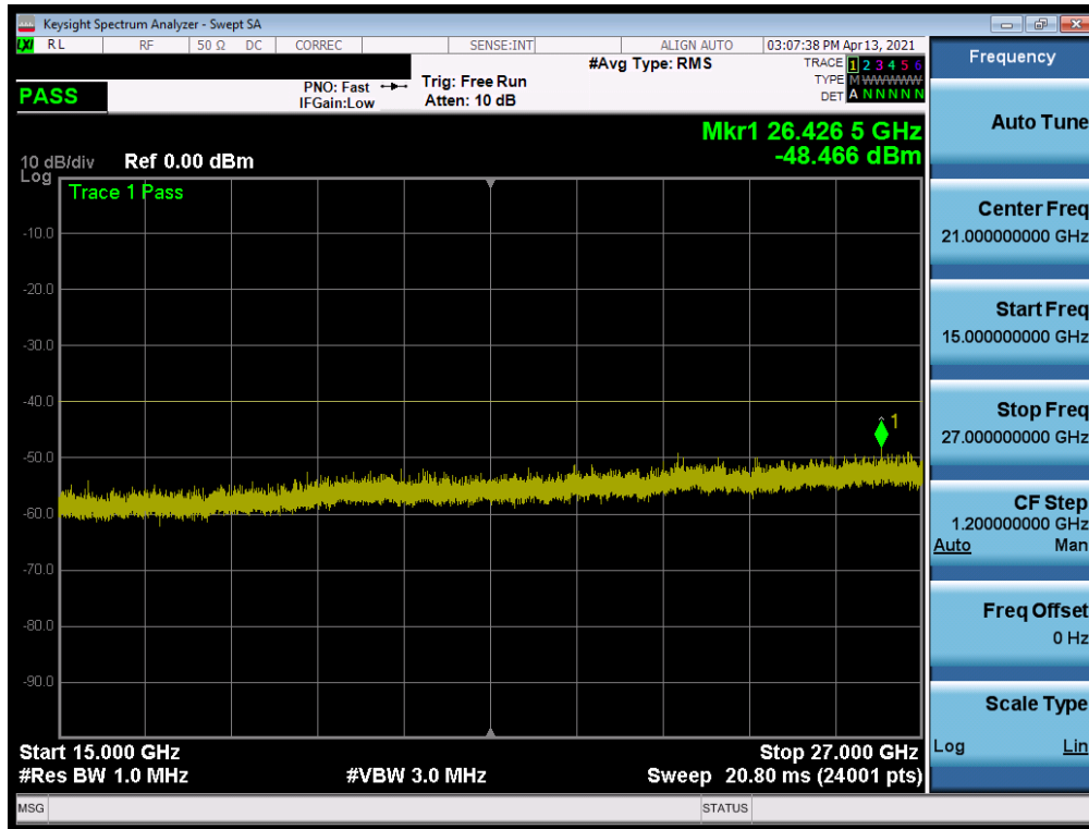
Plot 7-19. Conducted Spurious Plot (LTE Band 48 - 20MHz QPSK - RB Size 1, RB Offset 0 - Low Channel)
