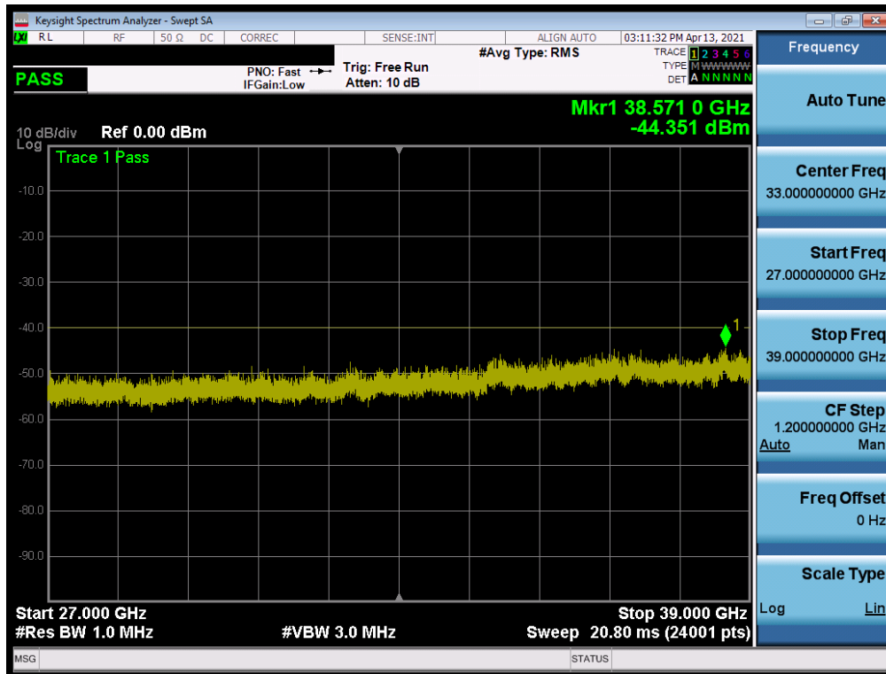
Plot 7-28. Conducted Spurious Plot (LTE Band 48 - 20MHz QPSK - RB Size 1, RB Offset 0 - High Channel)
