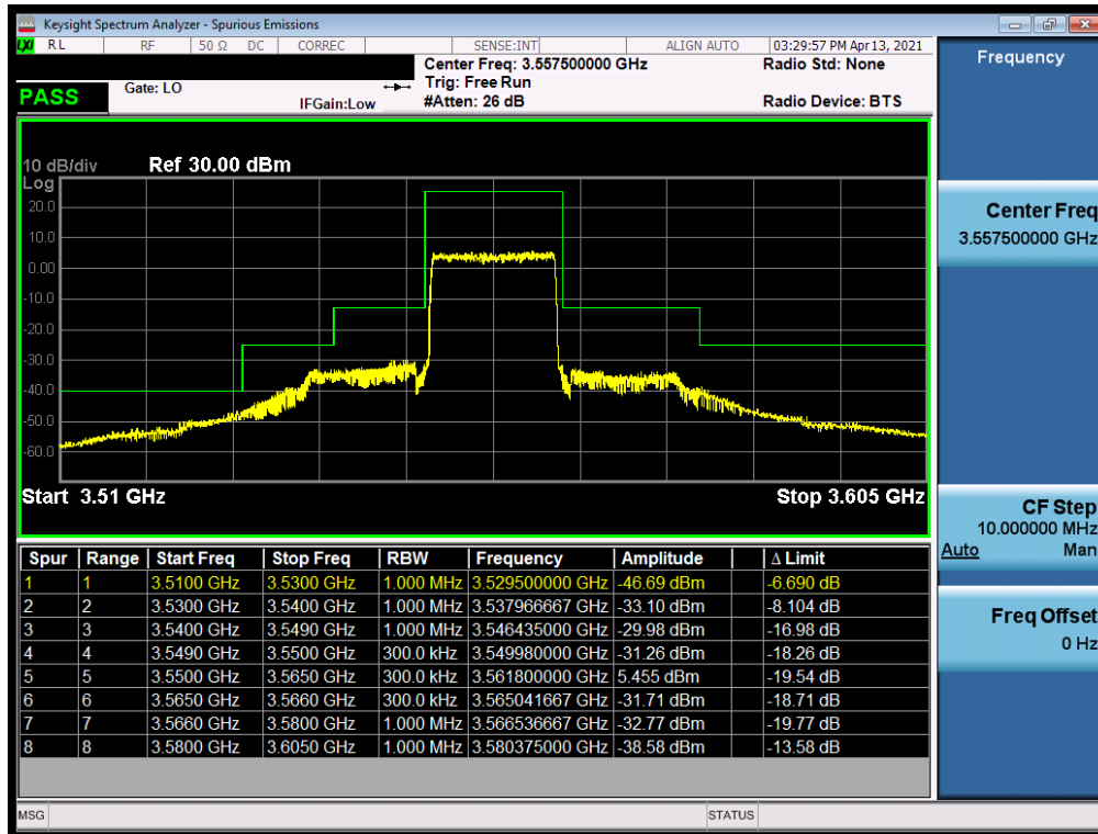
Plot 7-44. Channel Edge Plot (LTE Band 48 - 15MHz QPSK - Low Channel)
