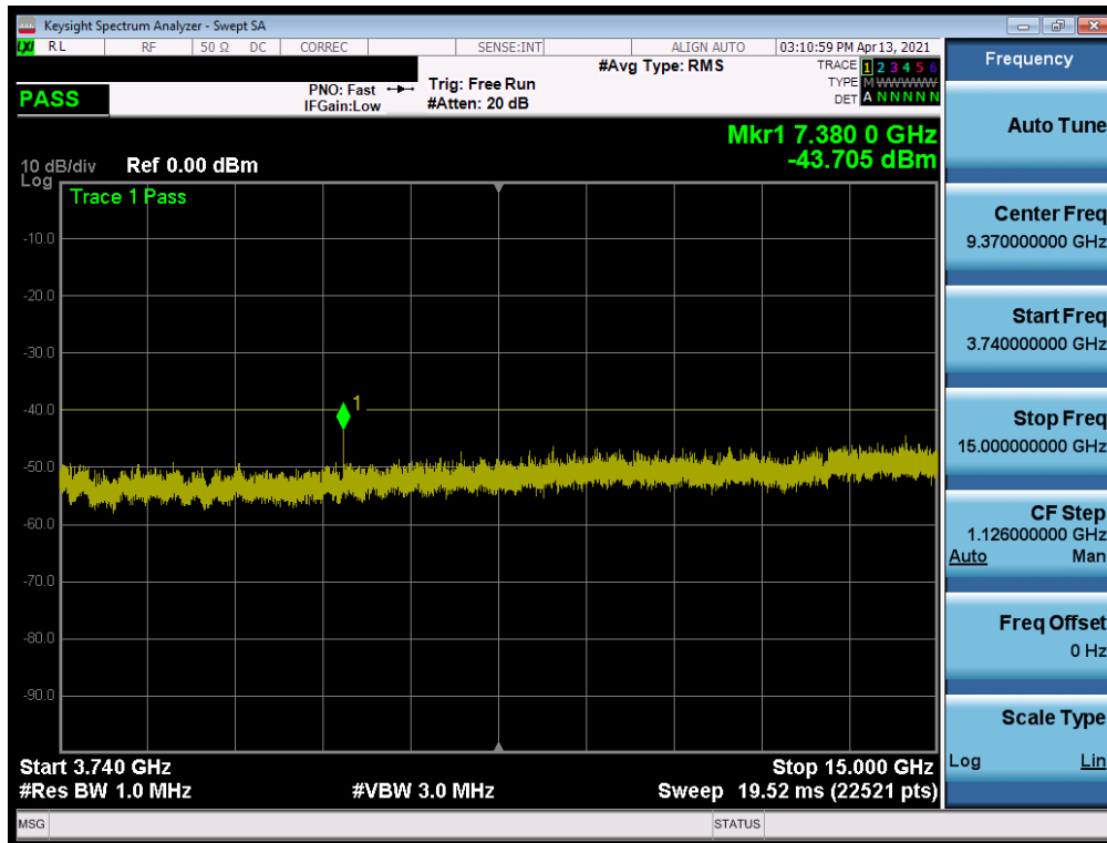
Plot 7-26. Conducted Spurious Plot (LTE Band 48 - 20MHz QPSK - RB Size 1, RB Offset 0 - High Channel)
