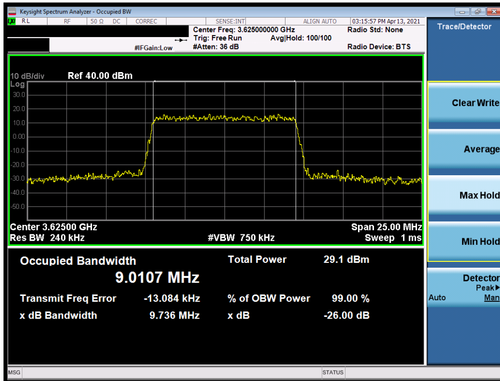
Plot 7-6. Occupied Bandwidth Plot (LTE Band 48 - 10MHz 16-QAM - Full RB Configuration)
