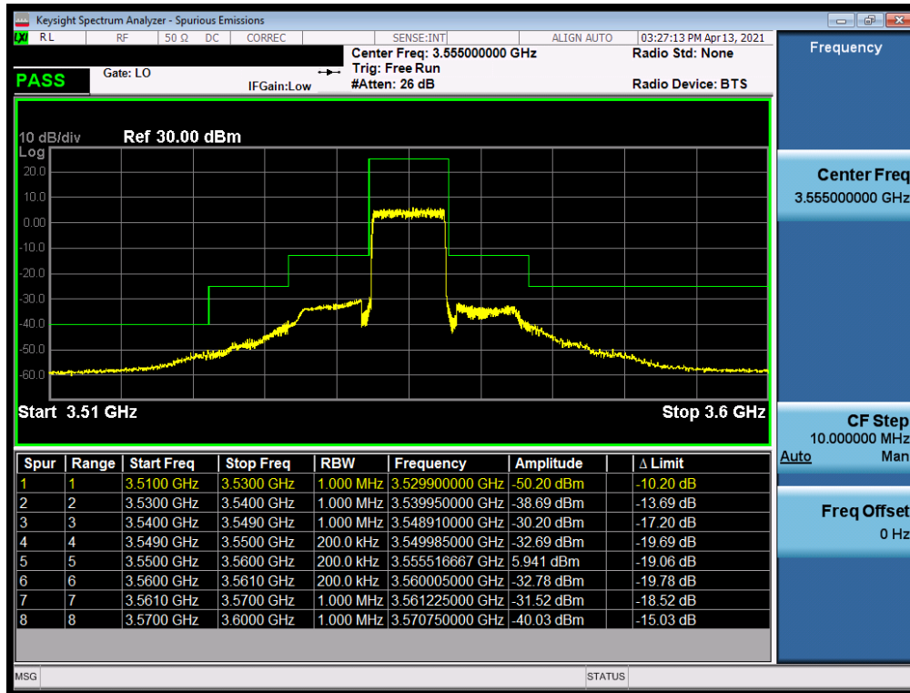
Plot 7-47. Channel Edge Plot (LTE Band 48 - 10MHz QPSK - Low Channel)
