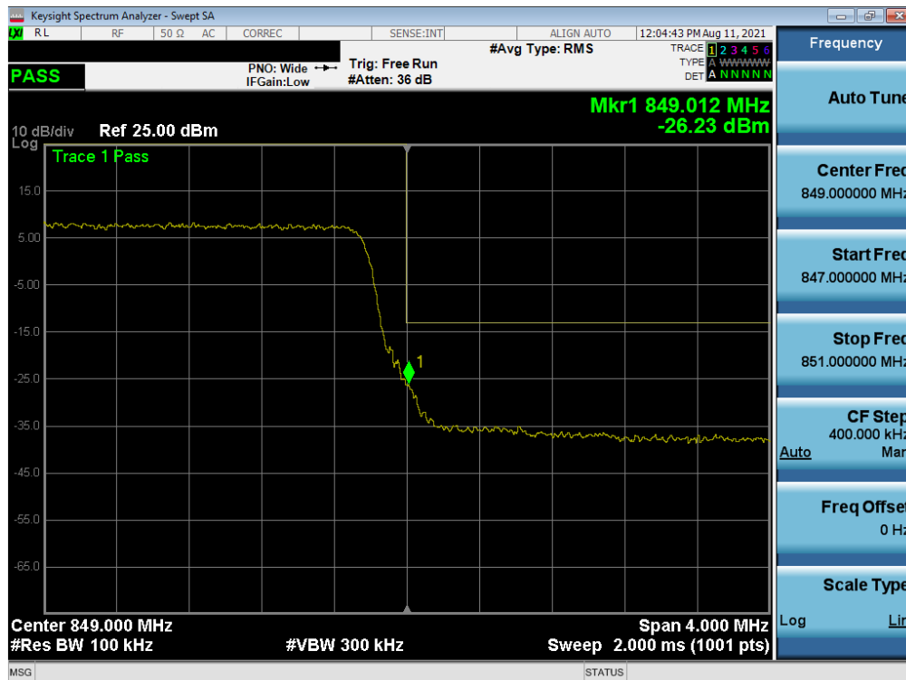
Plot 7-77. Upper Band Edge Plot (LTE Band 26/5 - 5MHz QPSK – Full RB)
