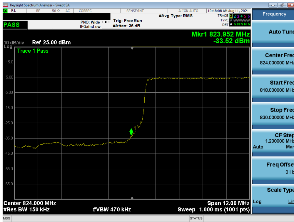
Plot 7-72. Lower Band Edge Plot (LTE Band 26 - 15MHz QPSK – Full RB)
