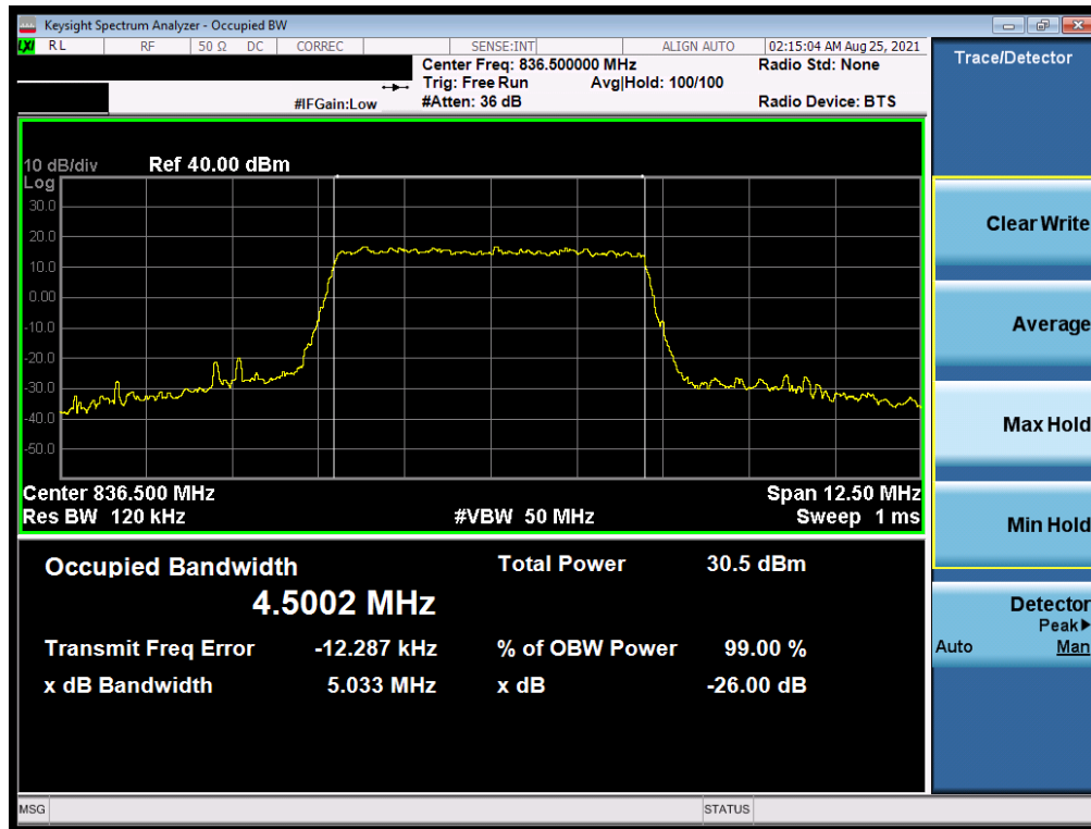
Plot 7-22. Occupied Bandwidth Plot (NR Band n5 - 5MHz 16-QAM - Full RB)
