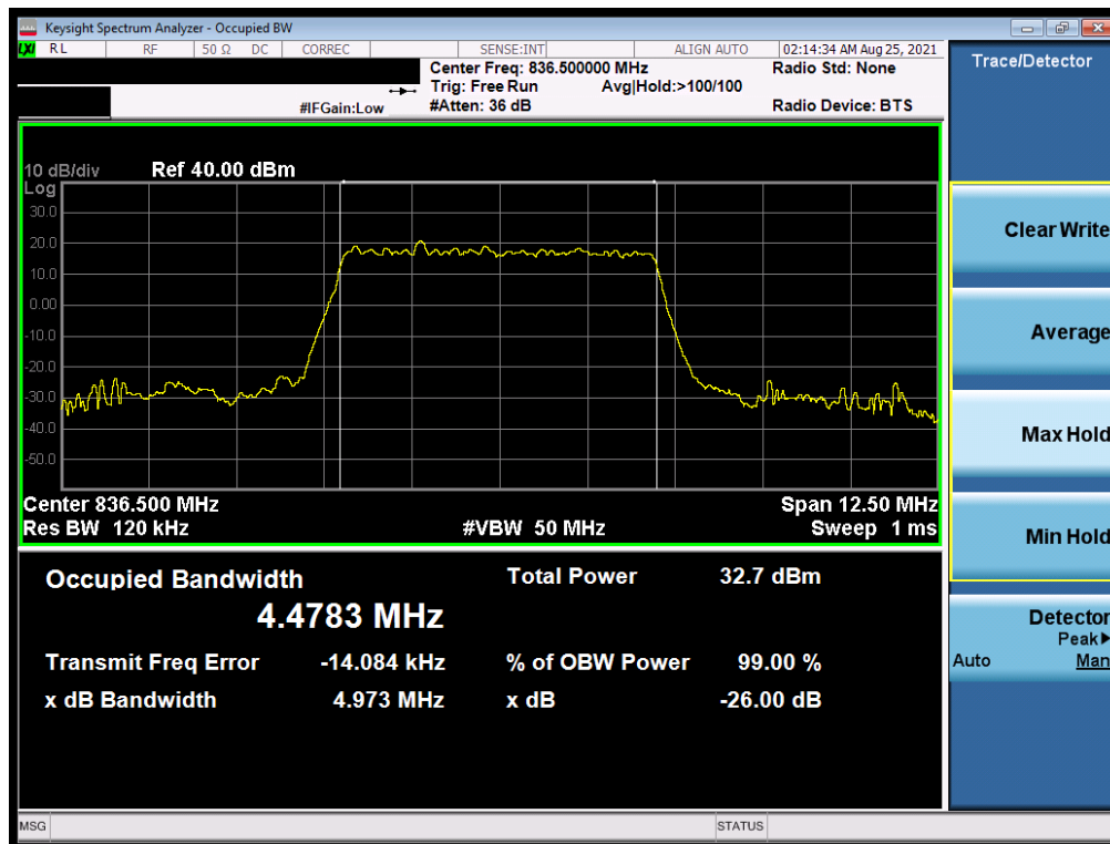
Plot 7-20. Occupied Bandwidth Plot (NR Band n5 - 5MHz \pi/2 BPSK - Full RB)
