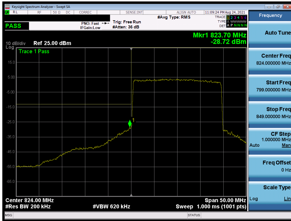
Plot 7-82. Lower Band Edge Plot (NR Band n5 – 20.0MHz - Full RB)
