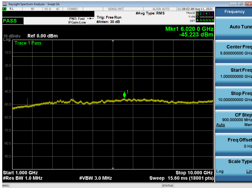
Plot 7-32. Conducted Spurious Plot (LTE Band 26/5 - 10MHz QPSK - 1 RB - Mid Channel)
