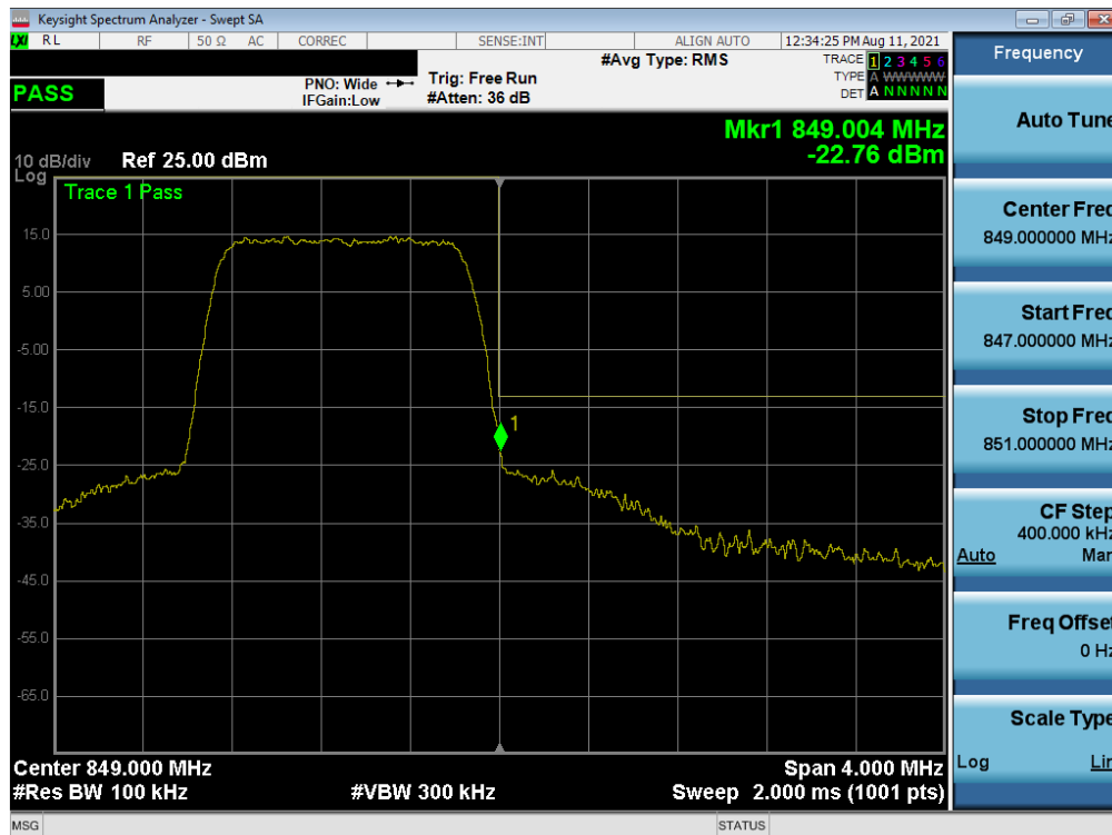
Plot 7-81. Upper Band Edge Plot (LTE Band 26/5 - 1.4MHz QPSK - Full RB)
