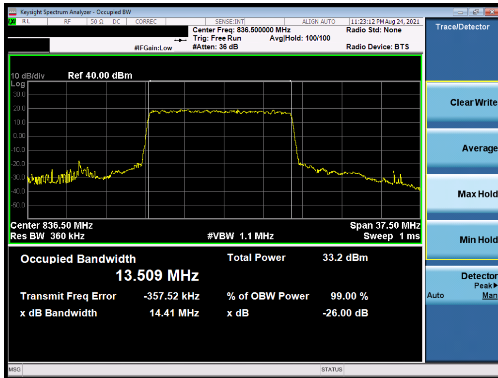
Plot 7-14. Occupied Bandwidth Plot (NR Band n5 - 15MHz \pi/2 BPSK - Full RB)
