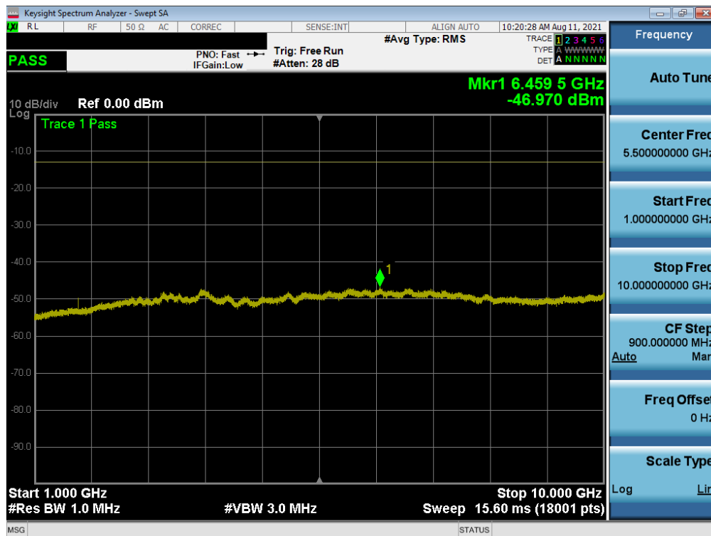
Plot 7-62. Conducted Spurious Plot (WCDMA Ch. 4233)
