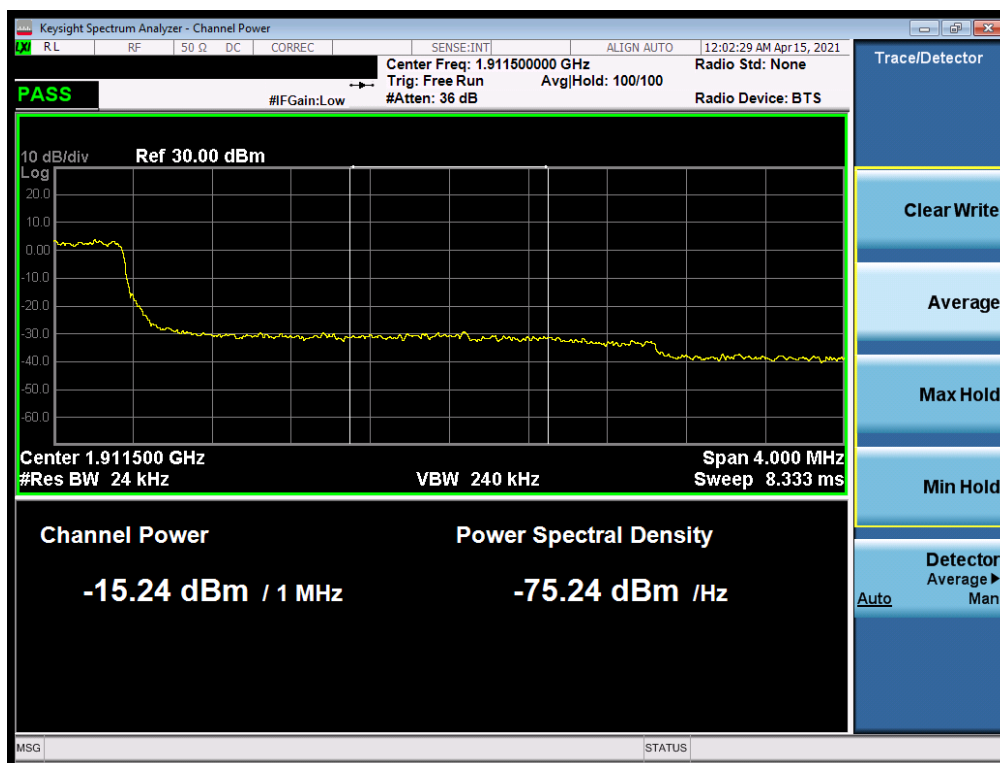
Plot 7-140. Extended Upper Band Edge Plot (LTE Band 2 - 3MHz QPSK – Full RB)
