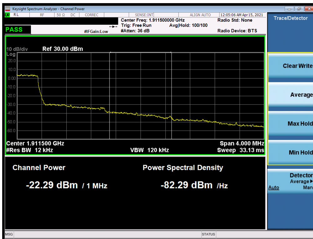
Plot 7-146. Extended Upper Band Edge Plot (LTE Band 2 – 1.4MHz QPSK – Full RB)
