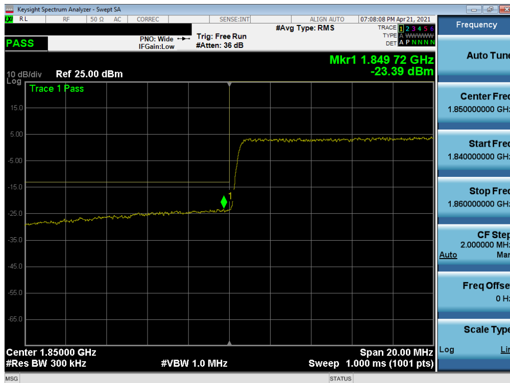
Plot 7-157. Lower Band Edge Plot (NR Band n25 - 25MHz QPSK – Full RB)
