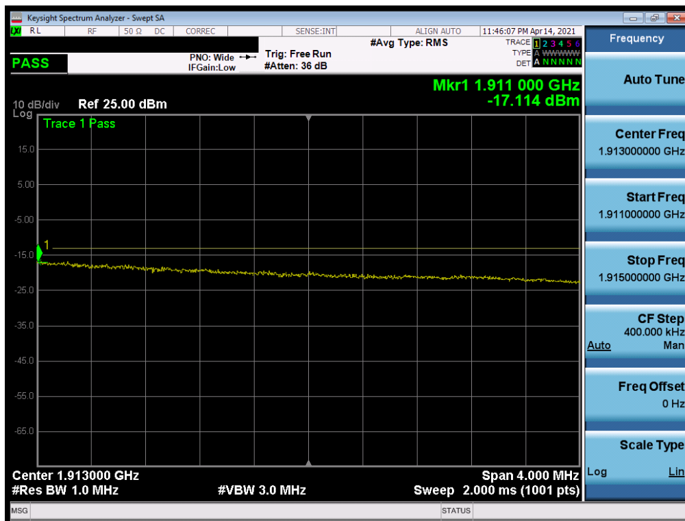
Plot 7-128. Extended Upper Band Edge Plot (LTE Band 2 - 10MHz QPSK – Full RB)
