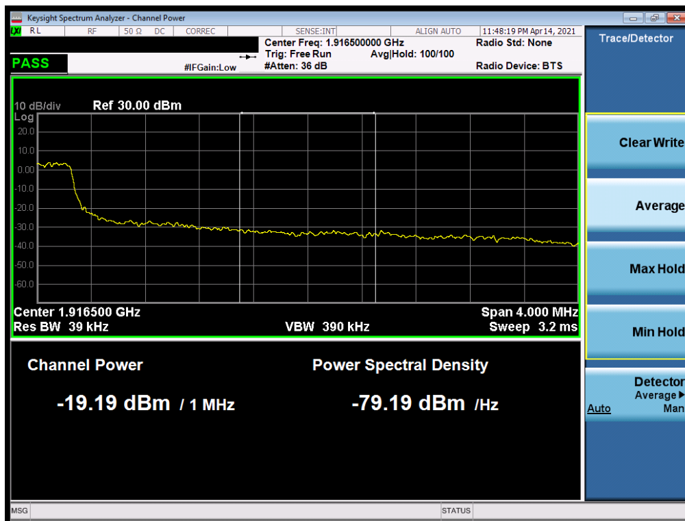
Plot 7-136. Extended Upper Band Edge Plot (LTE Band 25 - 5MHz QPSK – Full RB)
