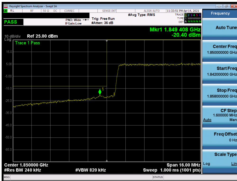
Plot 7-113. Lower Band Edge Plot (LTE Band 25/2 - 20MHz QPSK – Full RB)
