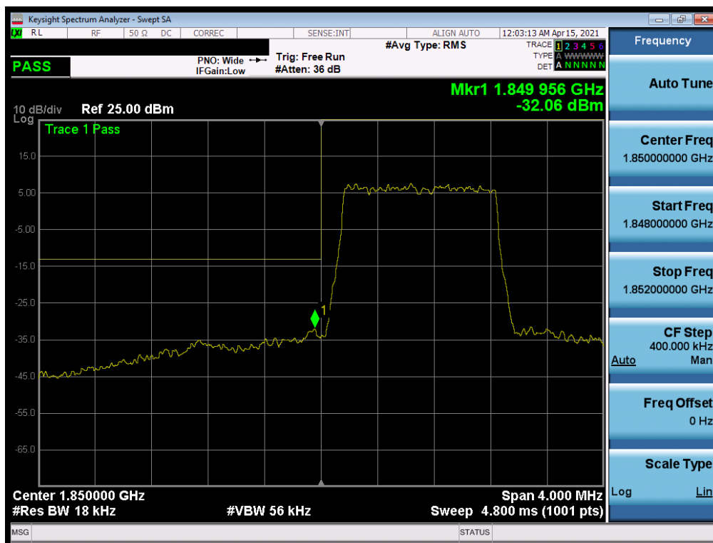
Plot 7-143. Lower Band Edge Plot (LTE Band 25/2 – 1.4MHz QPSK – Full RB)
