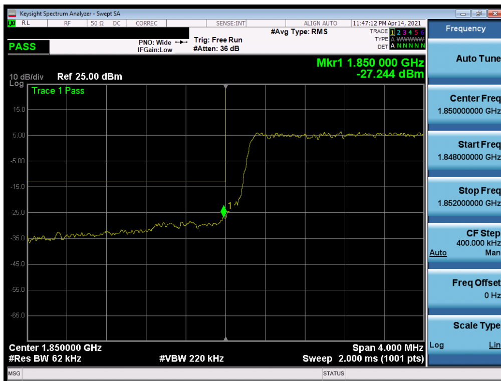
Plot 7-131. Lower Band Edge Plot (LTE Band 25/2 - 5MHz QPSK – Full RB)
