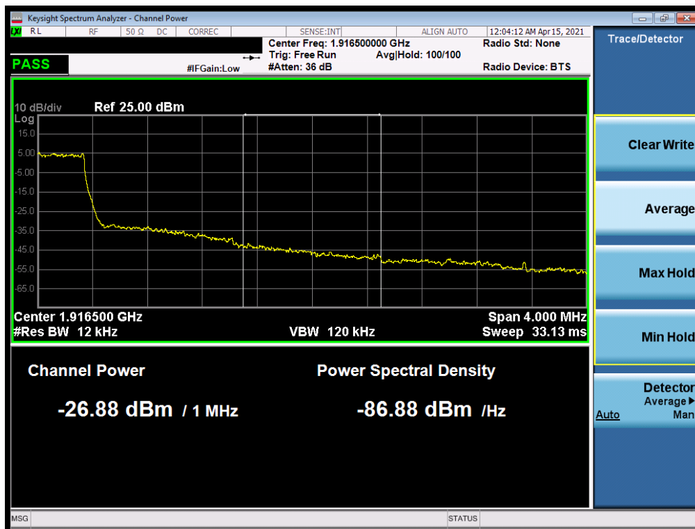
Plot 7-148. Extended Upper Band Edge Plot (LTE Band 25 – 1.4MHz QPSK – Full RB)
