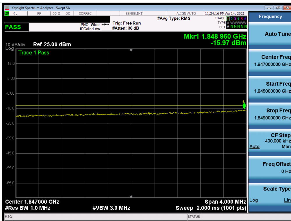
Plot 7-114. Extended Lower Band Edge Plot (LTE Band 25/2 - 20MHz QPSK – Full RB)
