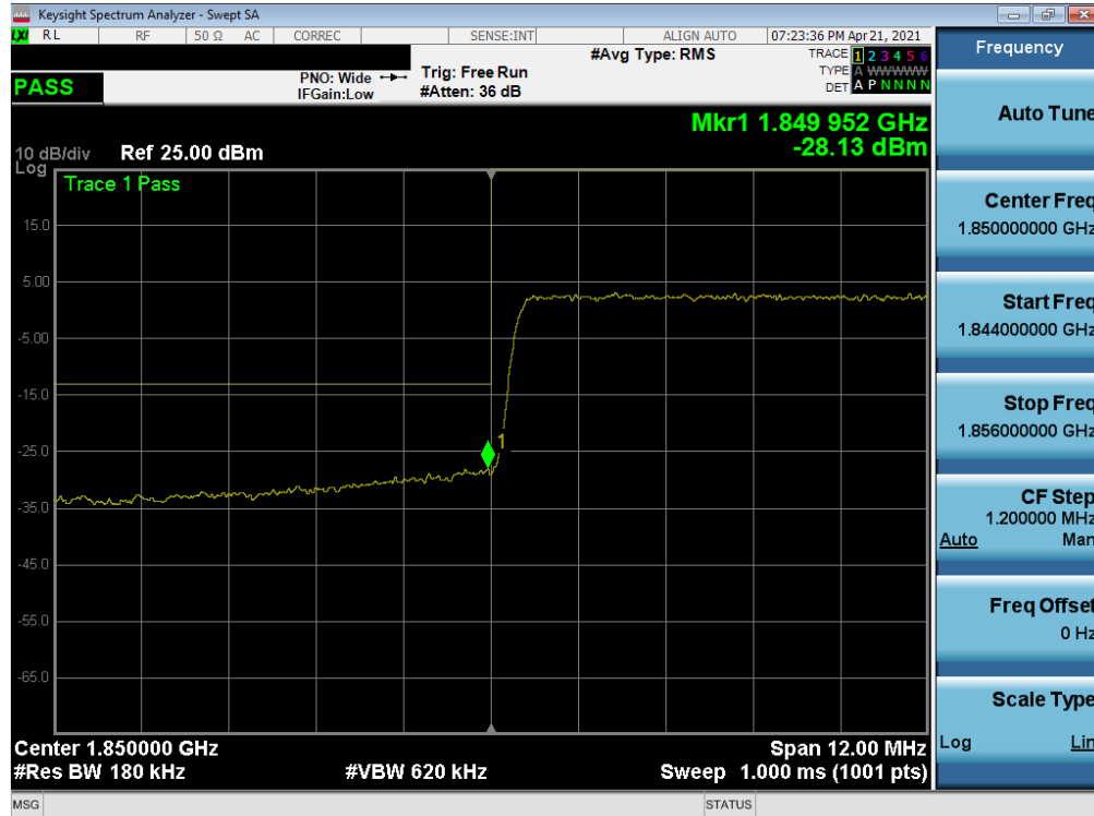
Plot 7-167. Lower Band Edge Plot (NR Band n25/2 - 15MHz QPSK – Full RB)
