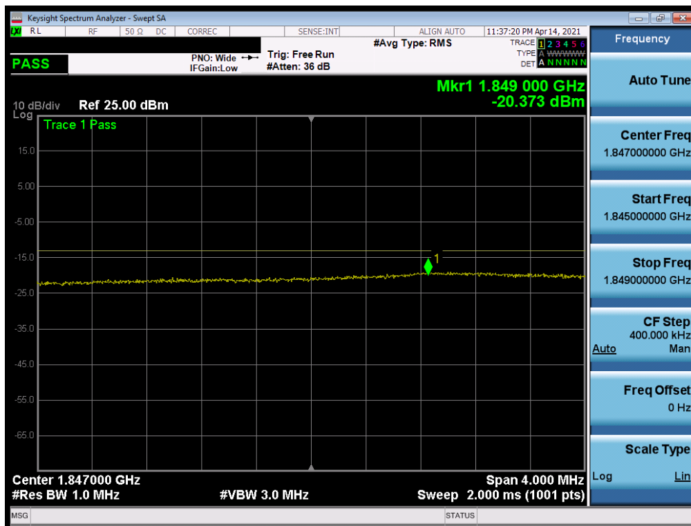
Plot 7-120. Extended Lower Band Edge Plot (LTE Band 25/2 - 15MHz QPSK - Full RB)
