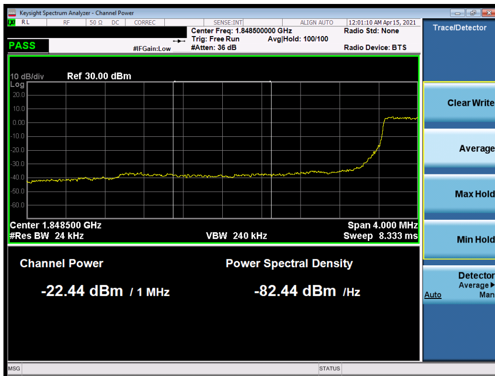
Plot 7-138. Extended Lower Band Edge Plot (LTE Band 25/2 - 3MHz QPSK – Full RB)
