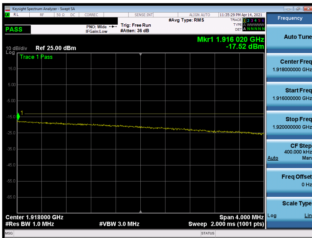
Plot 7-118. Extended Upper Band Edge Plot (LTE Band 25 - 20MHz QPSK – Full RB)
