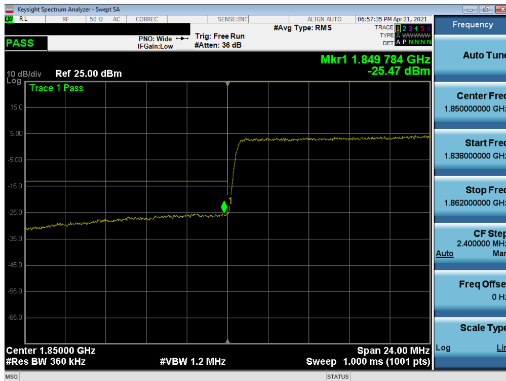
Plot 7-153. Lower Band Edge Plot (NR Band n25 - 30MHz QPSK – Full RB)
