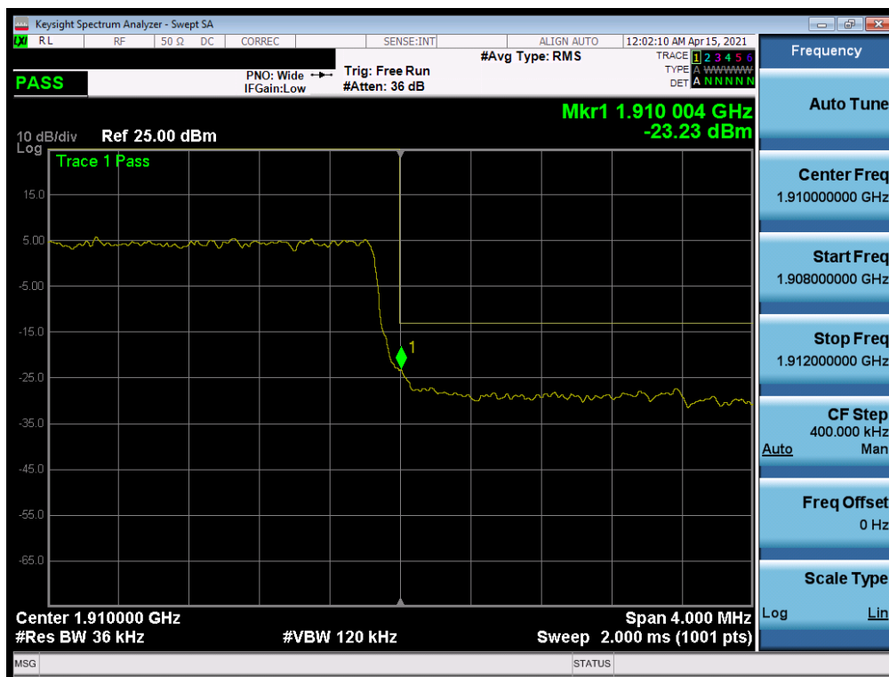
Plot 7-139. Upper Band Edge Plot (LTE Band 2 - 3MHz QPSK – Full RB)
