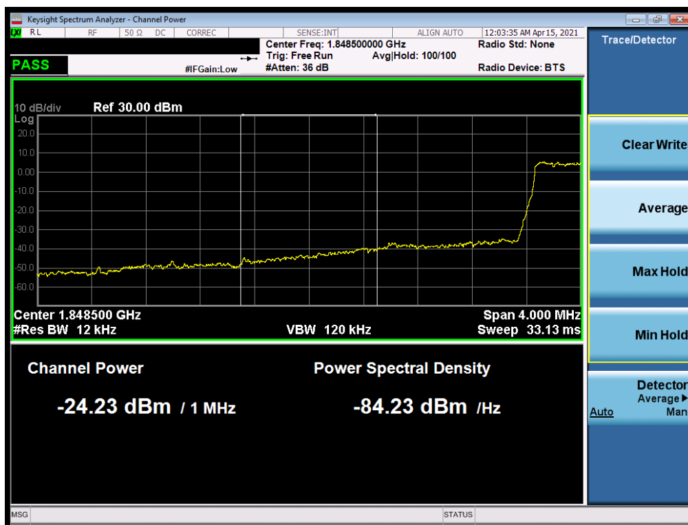
Plot 7-144. Extended Lower Band Edge Plot (LTE Band 25/2 – 1.4MHz QPSK – Full RB)
