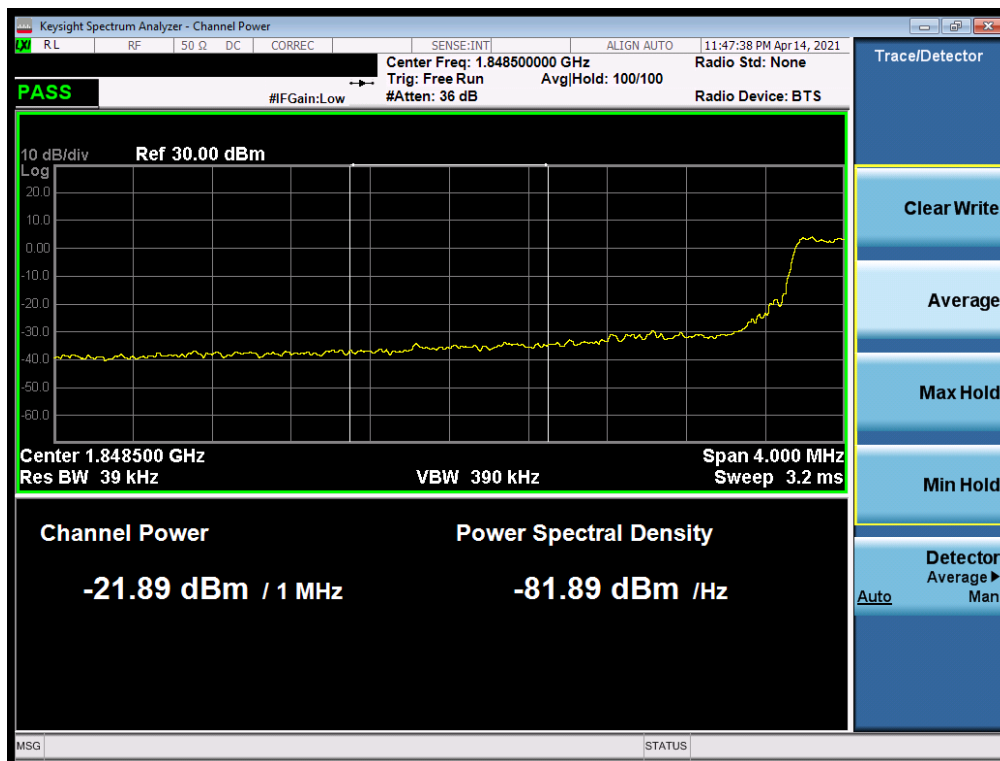
Plot 7-132. Extended Lower Band Edge Plot (LTE Band 25/2 - 5MHz QPSK – Full RB)
