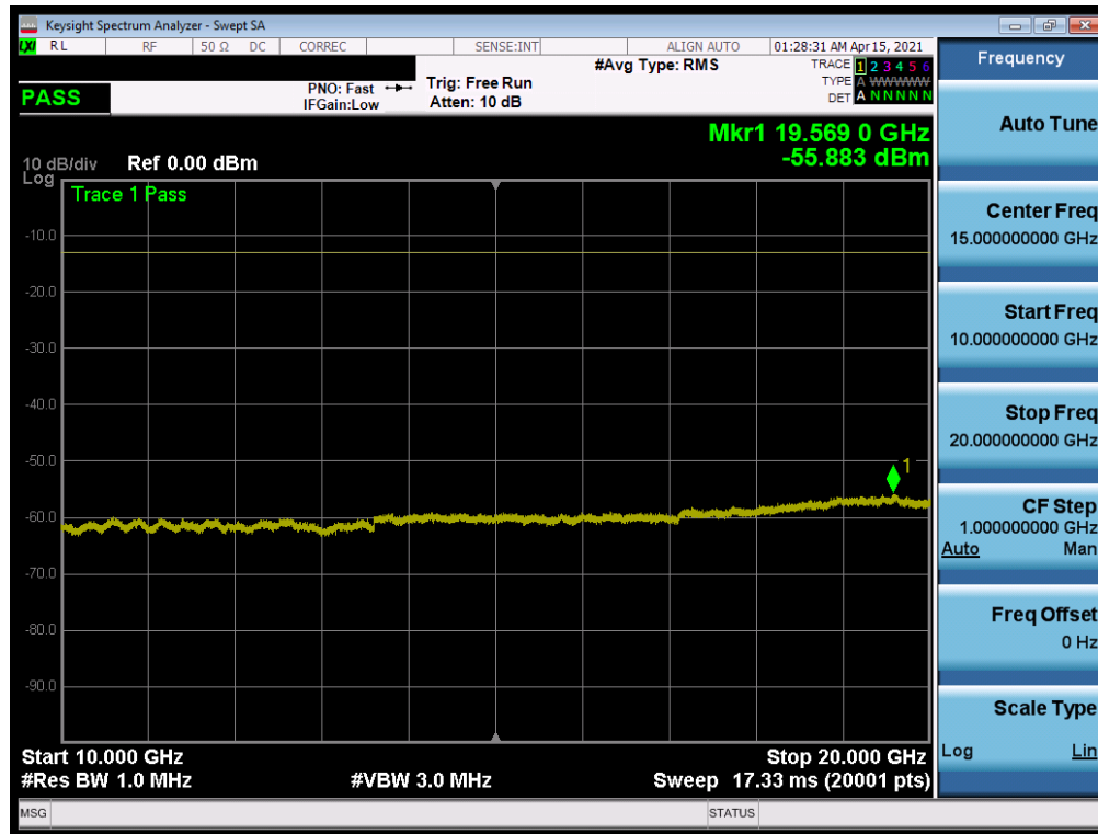
Plot 7-112. Conducted Spurious Plot (CDMA Ch. 1175)
