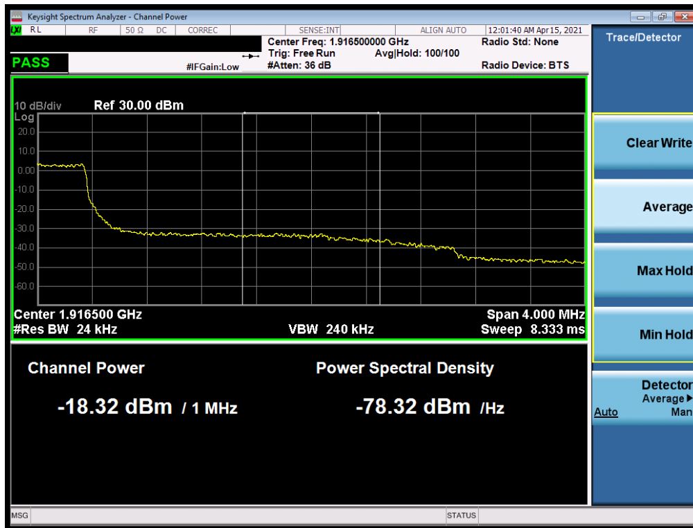
Plot 7-142. Extended Upper Band Edge Plot (LTE Band 25 - 3MHz QPSK – Full RB)
