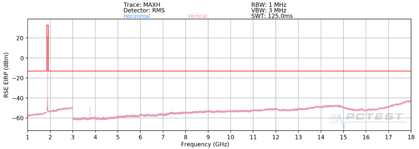
Plot 7-294. Radiated Spurious Plot (NR Band n25/2 - Closed)
