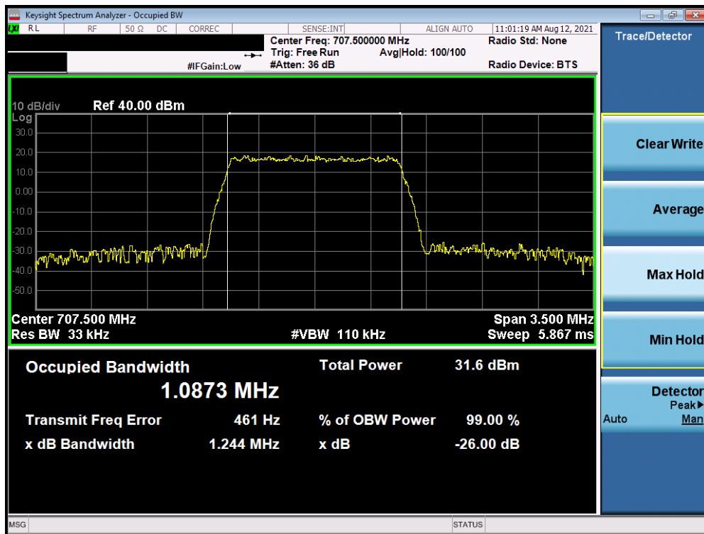
Plot 7-15. Occupied Bandwidth Plot (LTE Band 12 – 1.4MHz QPSK - Full RB – Ant I)
