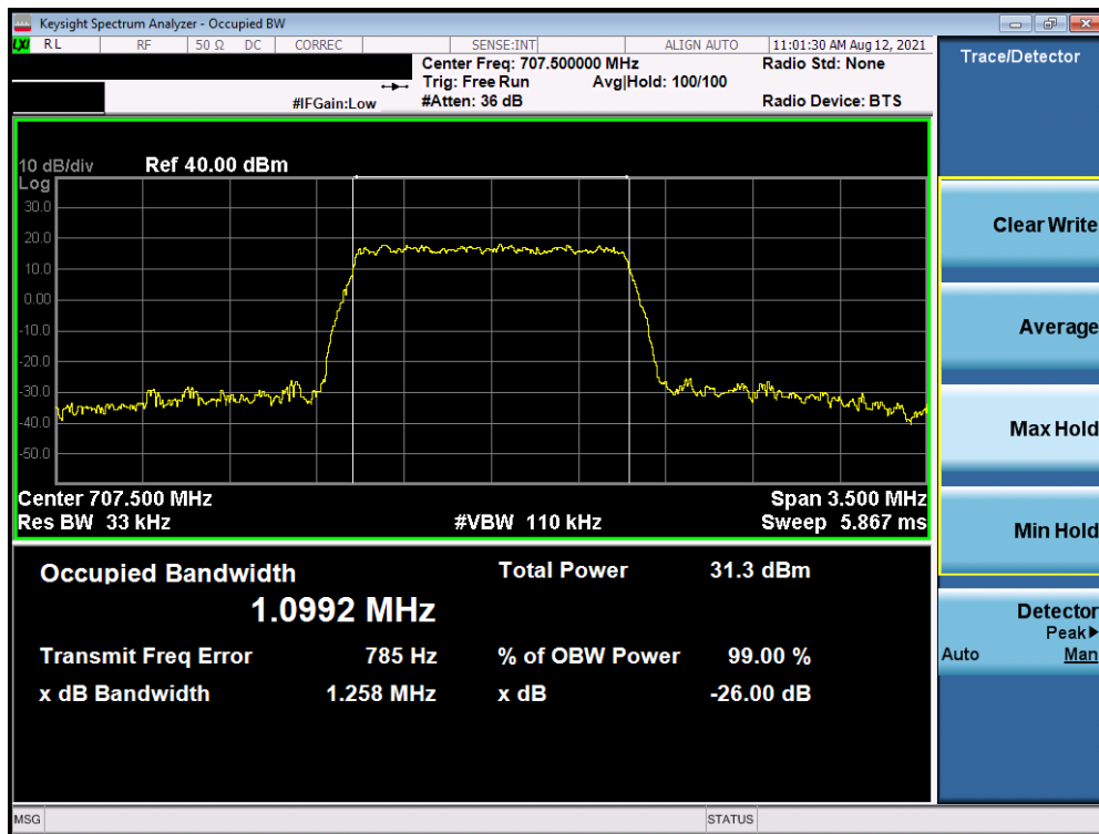
Plot 7-16. Occupied Bandwidth Plot (LTE Band 12 – 1.4MHz 16-QAM - Full RB – Ant I)
