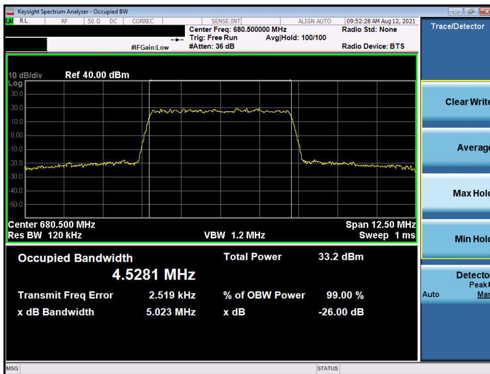
Plot 7-7. Occupied Bandwidth Plot (LTE Band 71 - 5MHz QPSK - Full RB - Ant I)
