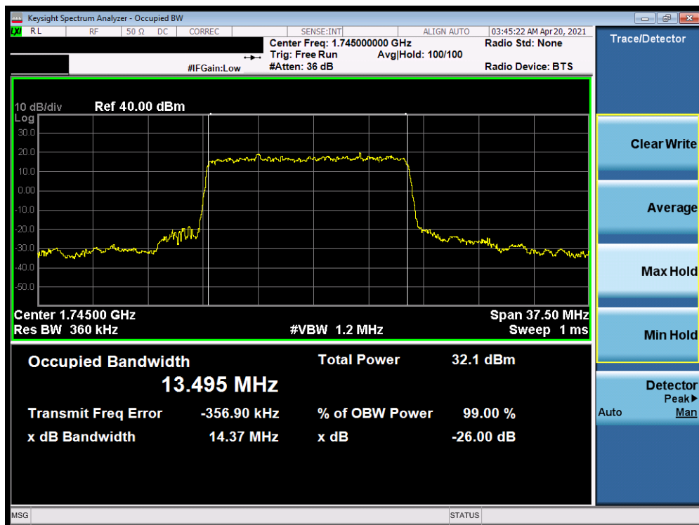
Plot 7-64. Occupied Bandwidth Plot (NR Band n66 - 15.0MHz DFT-s-OFDM BPSK - Full RB)
