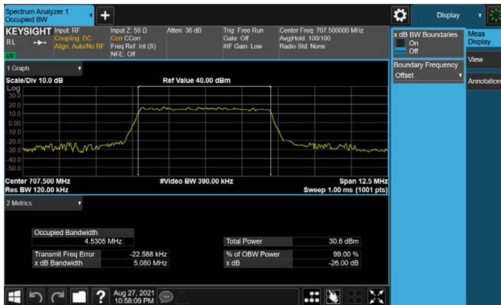
Plot 7-40. Occupied Bandwidth Plot (NR Band n12 - 5MHz CP-OFDM QPSK - Full RB – Ant I)
