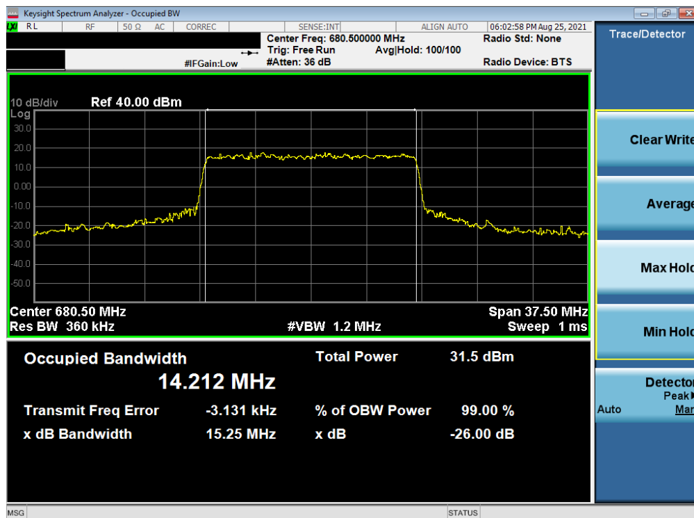
Plot 7-26. Occupied Bandwidth Plot (NR Band n71 - 15MHz CP-OFDM 16-QAM - Full RB – Ant I)
