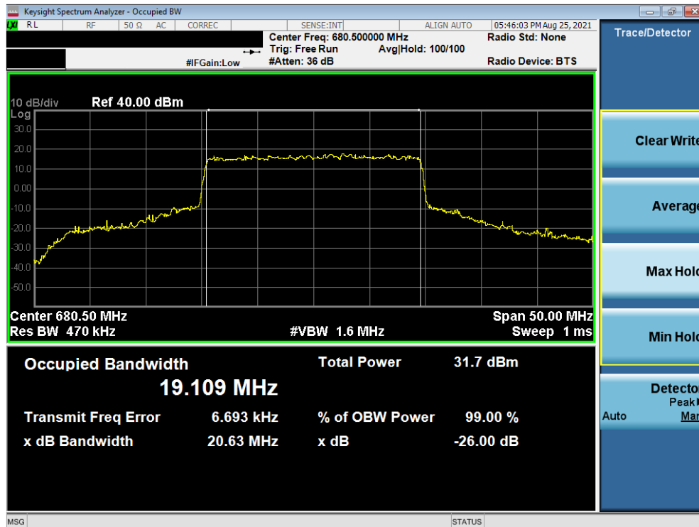
Plot 7-23. Occupied Bandwidth Plot (NR Band n71 - 20MHz CP-OFDM 16-QAM - Full RB – Ant I)
