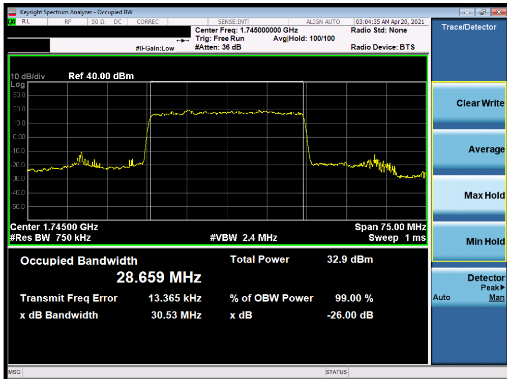
Plot 7-58. Occupied Bandwidth Plot (NR Band n66 - 30.0MHz DFT-s-OFDM BPSK - Full RB)
