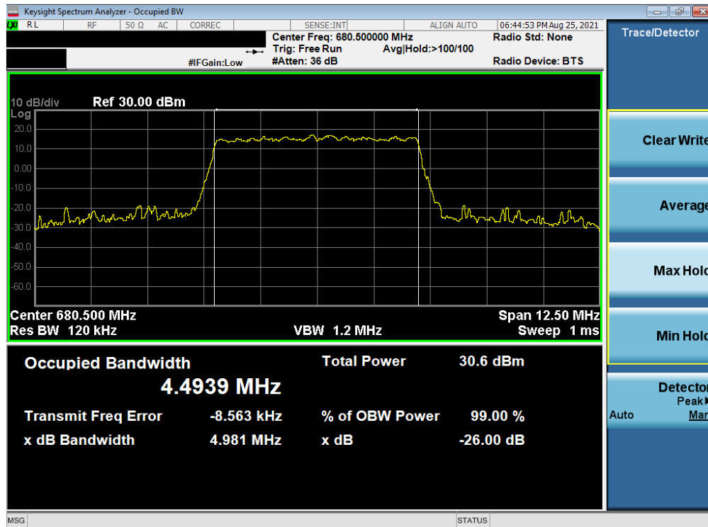
Plot 7-31. Occupied Bandwidth Plot (NR Band n71 - 5MHz CP-OFDM QPSK - Full RB - Ant I)
