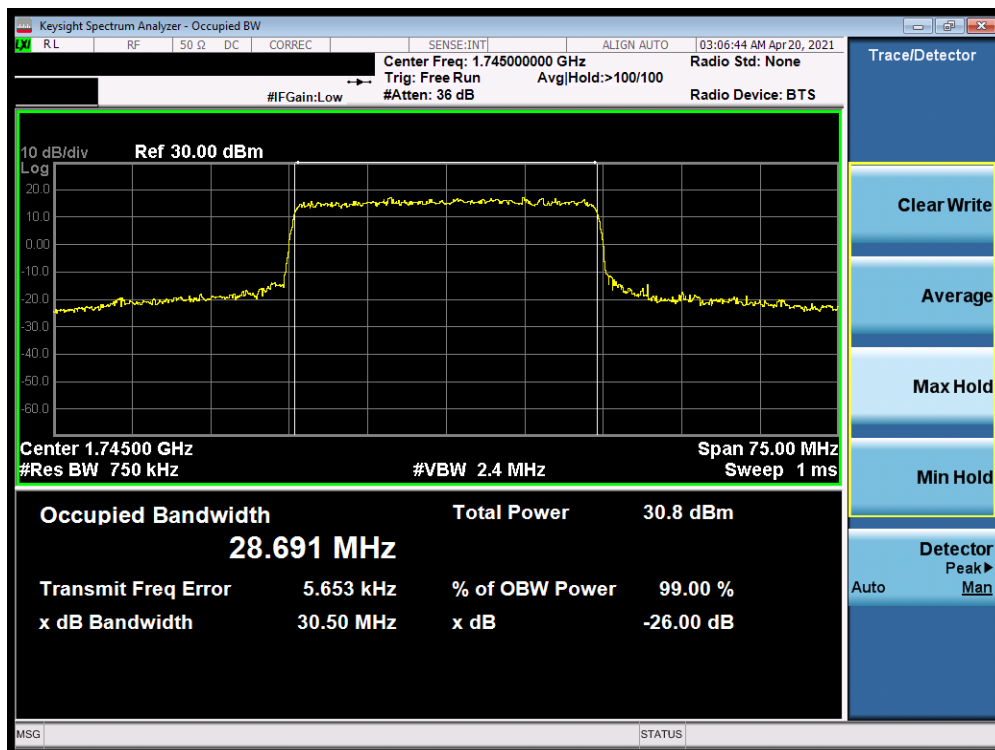
Plot 7-60. Occupied Bandwidth Plot (NR Band n66 - 30.0MHz CP-OFDM 16QAM - Full RB)
