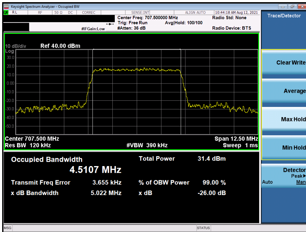
Plot 7-12. Occupied Bandwidth Plot (LTE Band 12 - 5MHz 16-QAM - Full RB – Ant I)
