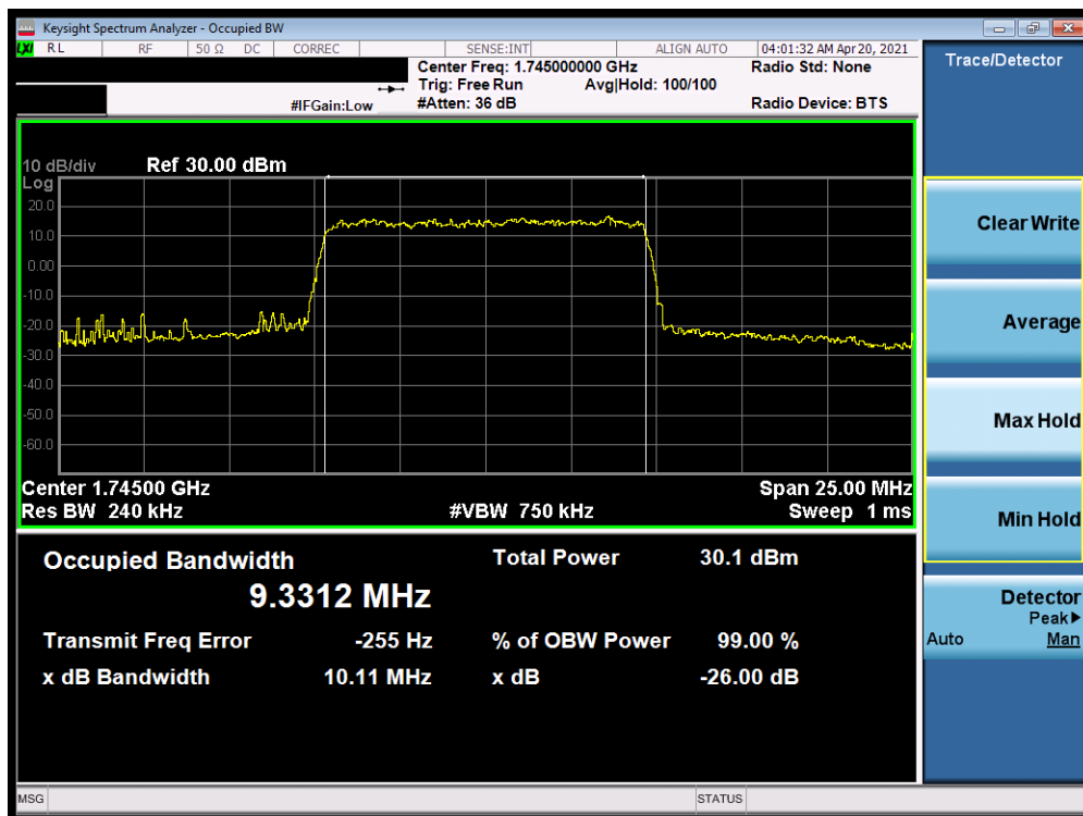
Plot 7-68. Occupied Bandwidth Plot (NR Band n66 - 10.0MHz CP-OFDM QPSK - Full RB)
