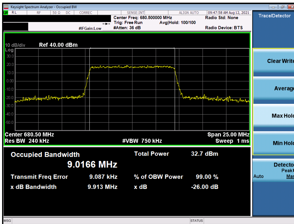
Plot 7-5. Occupied Bandwidth Plot (LTE Band 71 - 10MHz QPSK - Full RB - Ant I)
