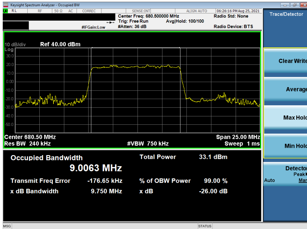
Plot 7-27. Occupied Bandwidth Plot (NR Band n71 - 10MHz DFT-s-OFDM BPSK - Full RB - Ant I)
