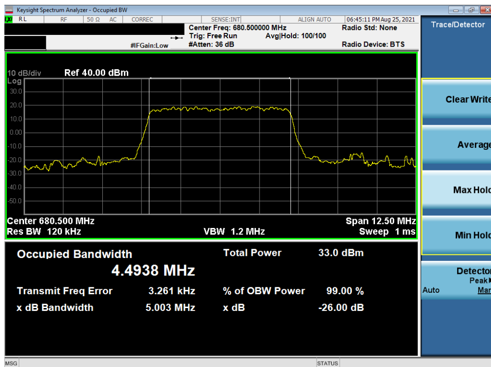
Plot 7-30. Occupied Bandwidth Plot (NR Band n71 - 5MHz DFT-s-OFDM BPSK - Full RB - Ant I)
