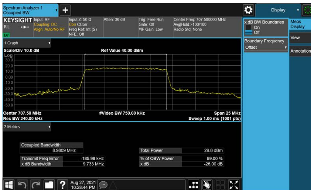
Plot 7-38. Occupied Bandwidth Plot (NR Band n12 - 10MHz CP-OFDM 16-QAM - Full RB – Ant I)
