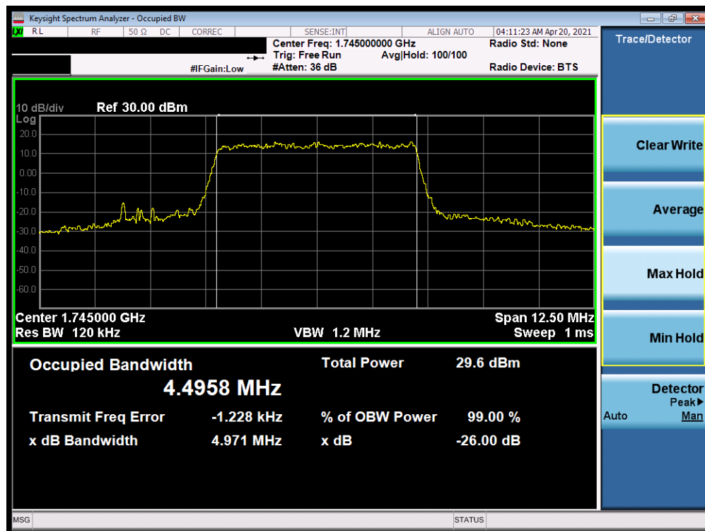
Plot 7-72. Occupied Bandwidth Plot (NR Band n66 - 5.0MHz CP-OFDM 16QAM - Full RB)
