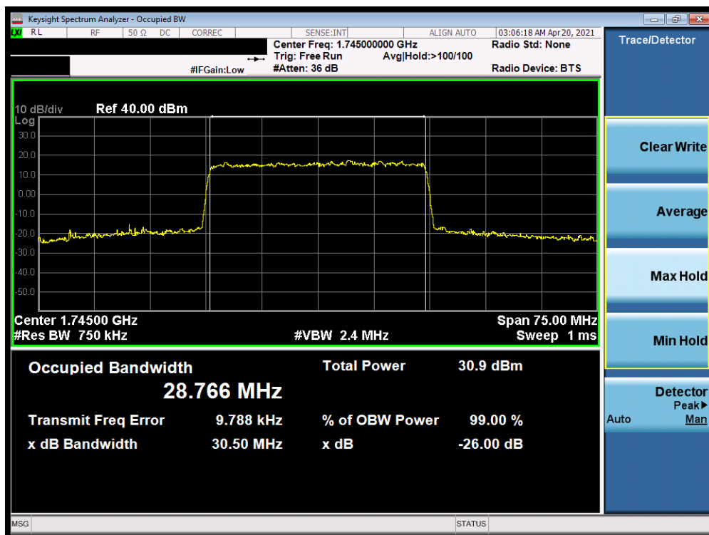
Plot 7-59. Occupied Bandwidth Plot (NR Band n66 - 30.0MHz CP-OFDM QPSK - Full RB)
