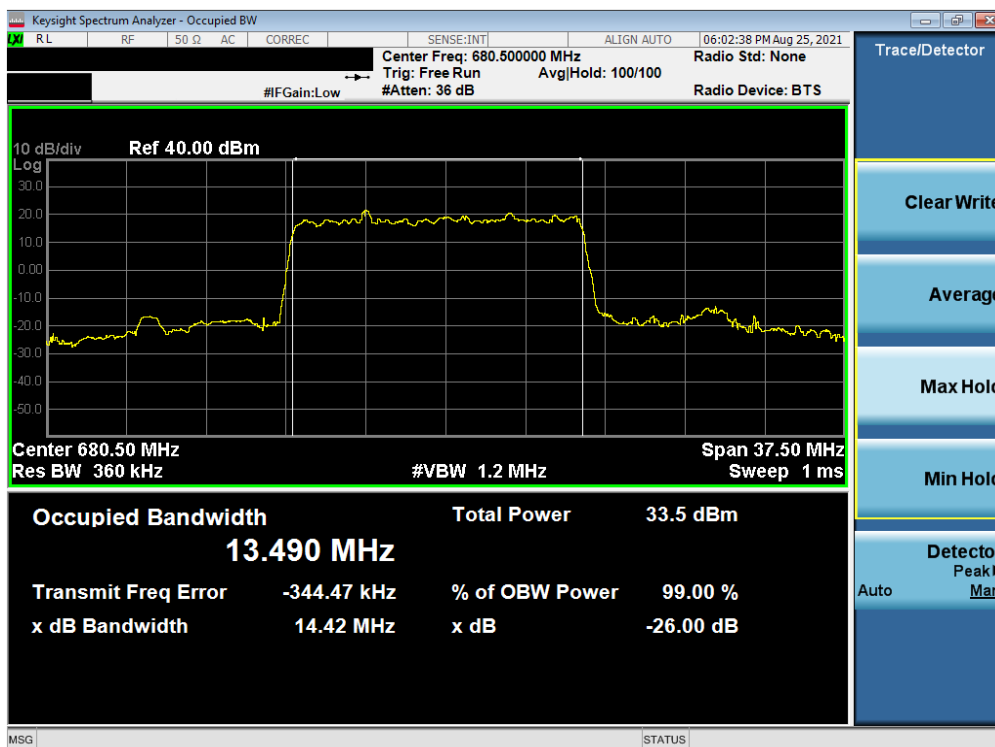
Plot 7-24. Occupied Bandwidth Plot (NR Band n71 - 15MHz DFT-s-OFDM BPSK - Full RB – Ant I)
