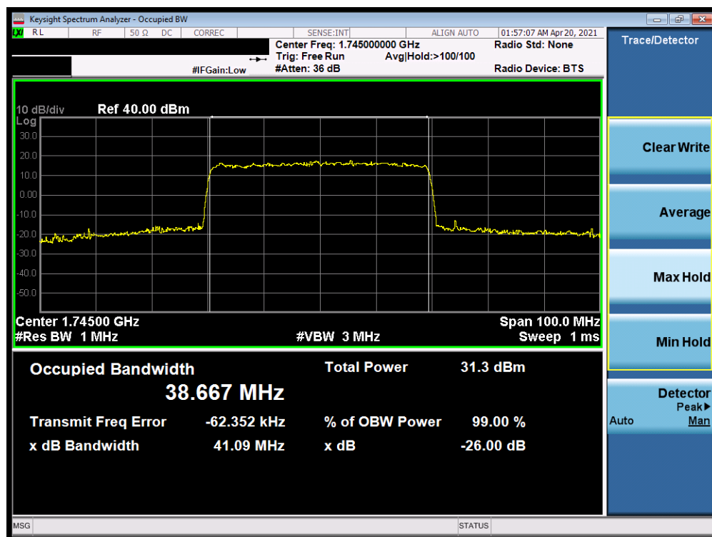
Plot 7-56. Occupied Bandwidth Plot (NR Band n66 - 40.0MHz CP-OFDM QPSK - Full RB)
