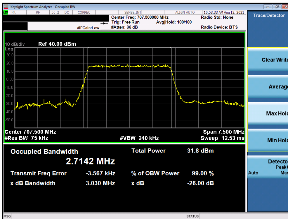
Plot 7-14. Occupied Bandwidth Plot (LTE Band 12 - 3MHz 16-QAM - Full RB - Ant I)
