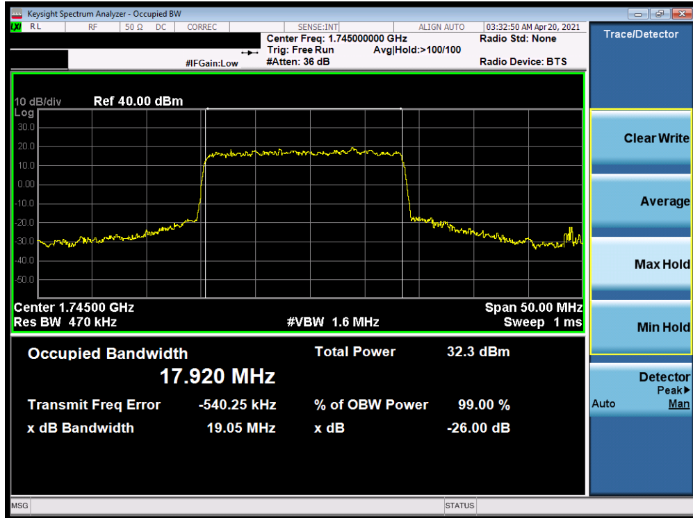
Plot 7-61. Occupied Bandwidth Plot (NR Band n66 - 20.0MHz DFT-s-OFDM BPSK - Full RB)
