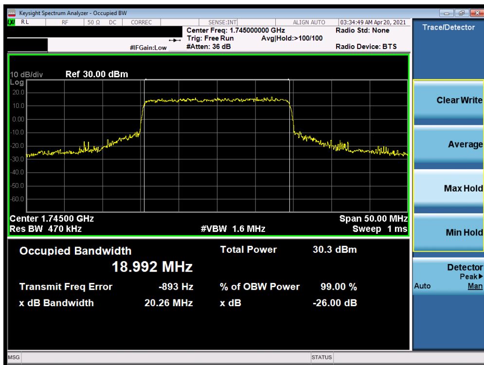
Plot 7-63. Occupied Bandwidth Plot (NR Band n66 - 20.0MHz CP-OFDM 16QAM - Full RB)
