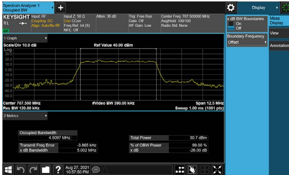
Plot 7-39. Occupied Bandwidth Plot (NR Band n12 - 5MHz DFT-s-OFDM BPSK - Full RB – Ant I)
