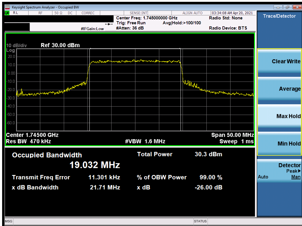
Plot 7-62. Occupied Bandwidth Plot (NR Band n66 - 20.0MHz CP-OFDM QPSK - Full RB)
