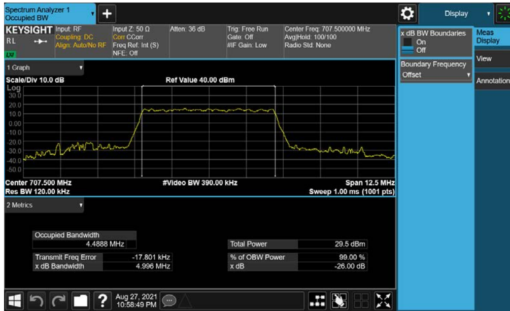
Plot 7-41. Occupied Bandwidth Plot (NR Band n12 - 5MHz CP-OFDM 16-QAM - Full RB – Ant I)
