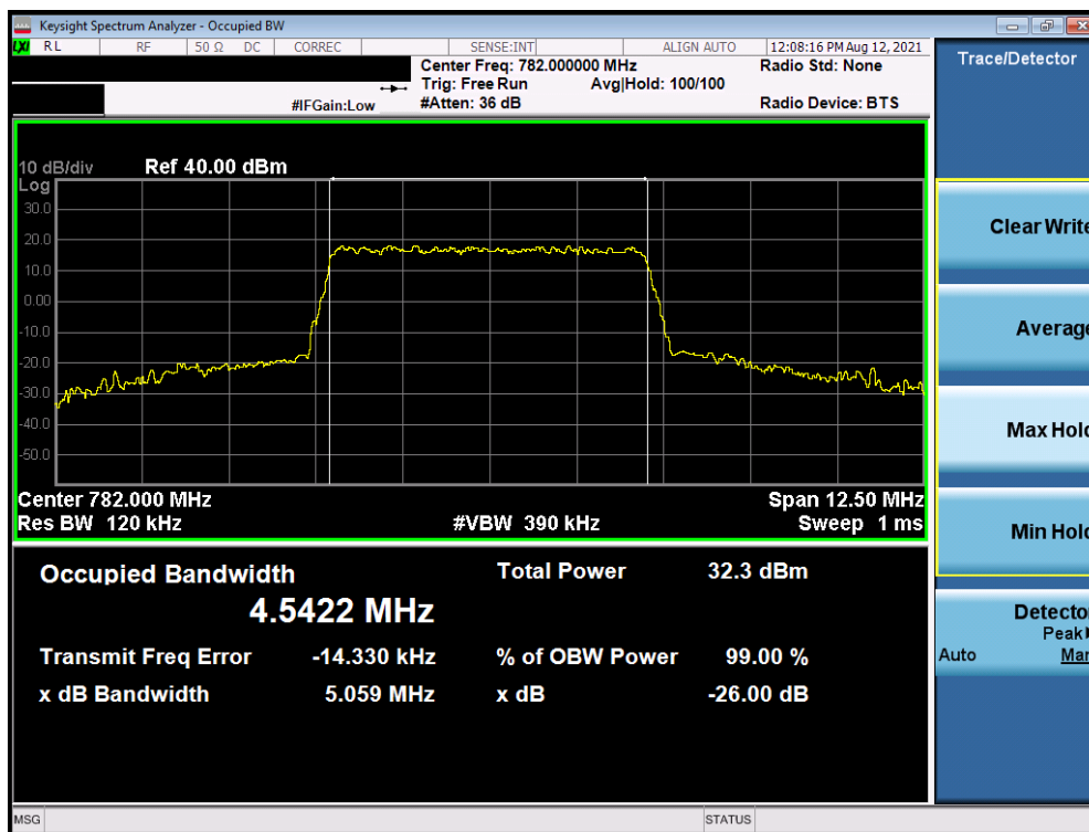
Plot 7-19. Occupied Bandwidth Plot (LTE Band 13 - 5MHz QPSK - Full RB – Ant I)
