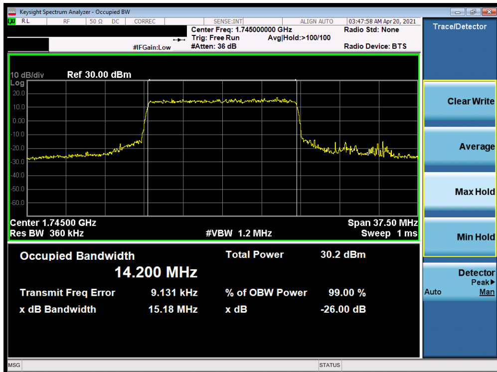
Plot 7-66. Occupied Bandwidth Plot (NR Band n66 - 15.0MHz CP-OFDM 16QAM - Full RB)
