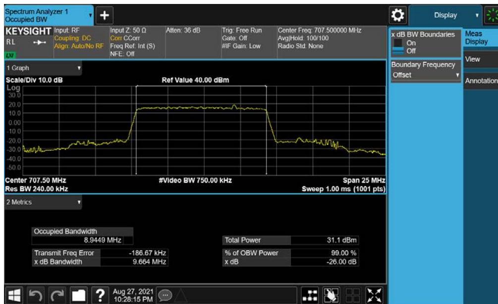
Plot 7-36. Occupied Bandwidth Plot (NR Band n12 - 10MHz DFT-s-OFDM BPSK - Full RB – Ant I)
