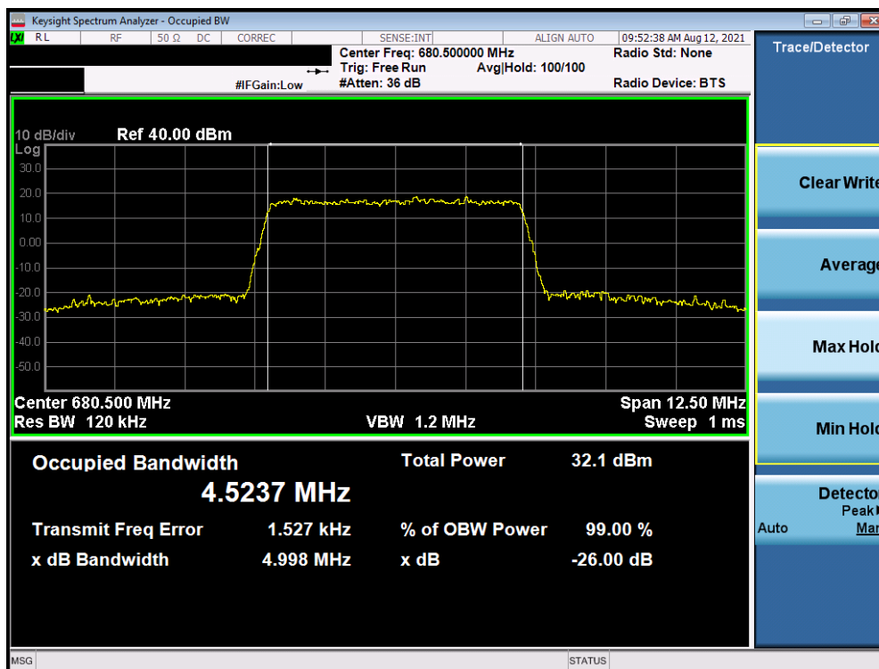
Plot 7-8. Occupied Bandwidth Plot (LTE Band 71 - 5MHz 16-QAM - Full RB - Ant I)
