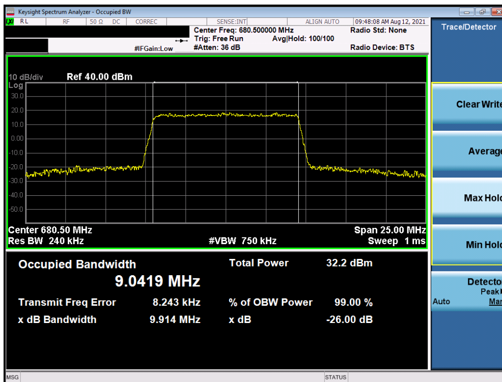
Plot 7-6. Occupied Bandwidth Plot (LTE Band 71 - 10MHz 16-QAM - Full RB - Ant I)
