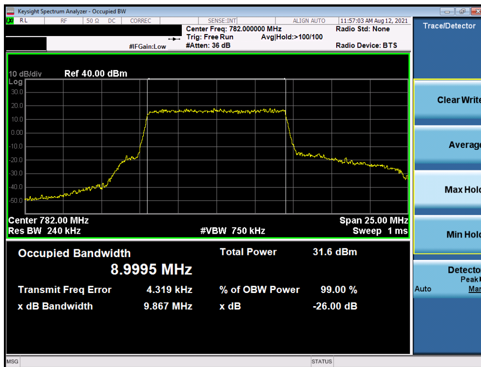
Plot 7-18. Occupied Bandwidth Plot (LTE Band 13 - 10MHz 16-QAM - Full RB – Ant I)
