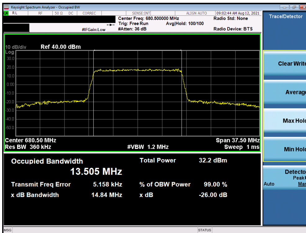
Plot 7-4. Occupied Bandwidth Plot (LTE Band 71 - 15MHz 16-QAM - Full RB - Ant I)
