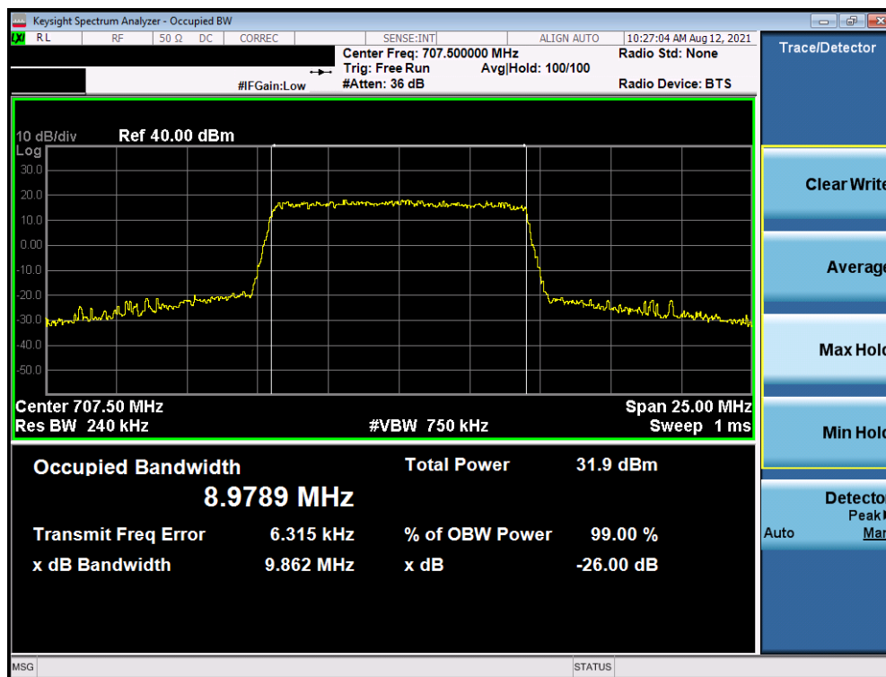
Plot 7-10. Occupied Bandwidth Plot (LTE Band 12 - 10MHz 16-QAM - Full RB – Ant I)
