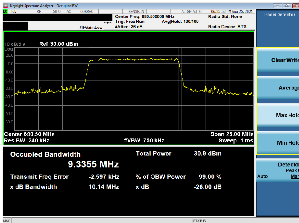
Plot 7-28. Occupied Bandwidth Plot (NR Band n71 - 10MHz CP-OFDM QPSK - Full RB - Ant I)
