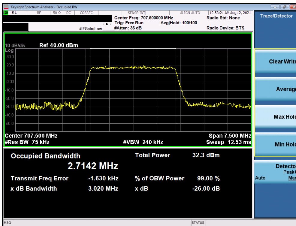
Plot 7-13. Occupied Bandwidth Plot (LTE Band 12 - 3MHz QPSK - Full RB - Ant I)
