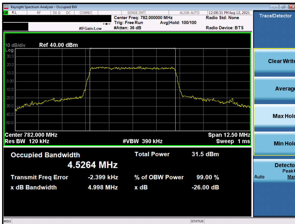
Plot 7-20. Occupied Bandwidth Plot (LTE Band 13 - 5MHz 16-QAM - Full RB – Ant I)
