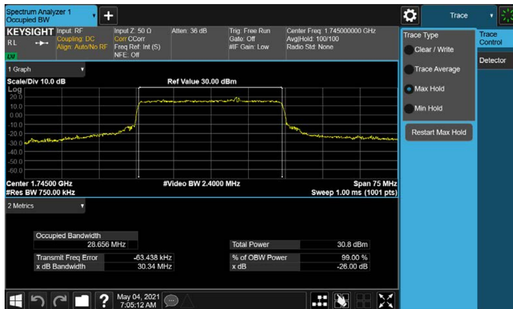
Plot 7-78. Occupied Bandwidth Plot (NR Band n66 - 30.0MHz CP-OFDM 16QAM - Full RB)
