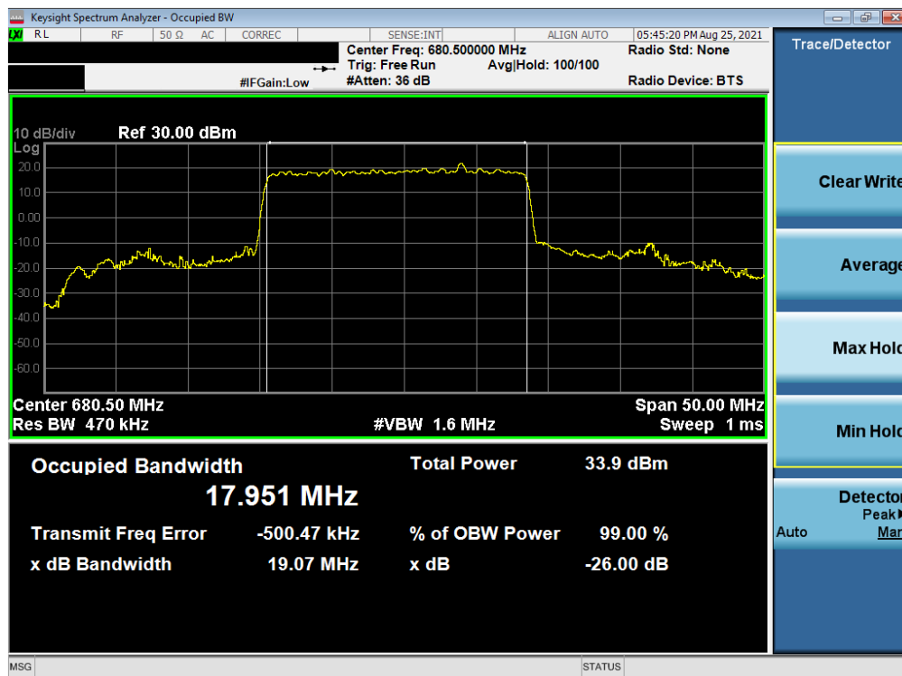
Plot 7-21. Occupied Bandwidth Plot (NR Band n71 - 20MHz DFT-s-OFDM BPSK - Full RB – Ant I)
