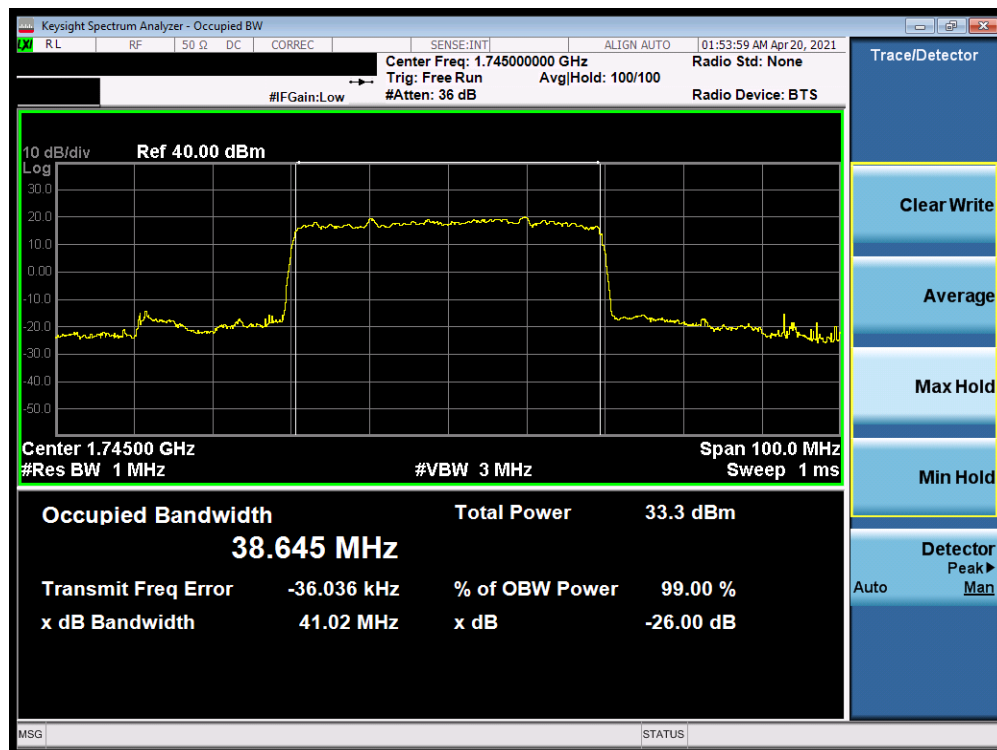
Plot 7-55. Occupied Bandwidth Plot (NR Band n66 - 40.0MHz DFT-s-OFDM BPSK - Full RB)
