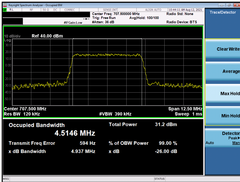
Plot 7-11. Occupied Bandwidth Plot (LTE Band 12 - 5MHz QPSK - Full RB – Ant I)
