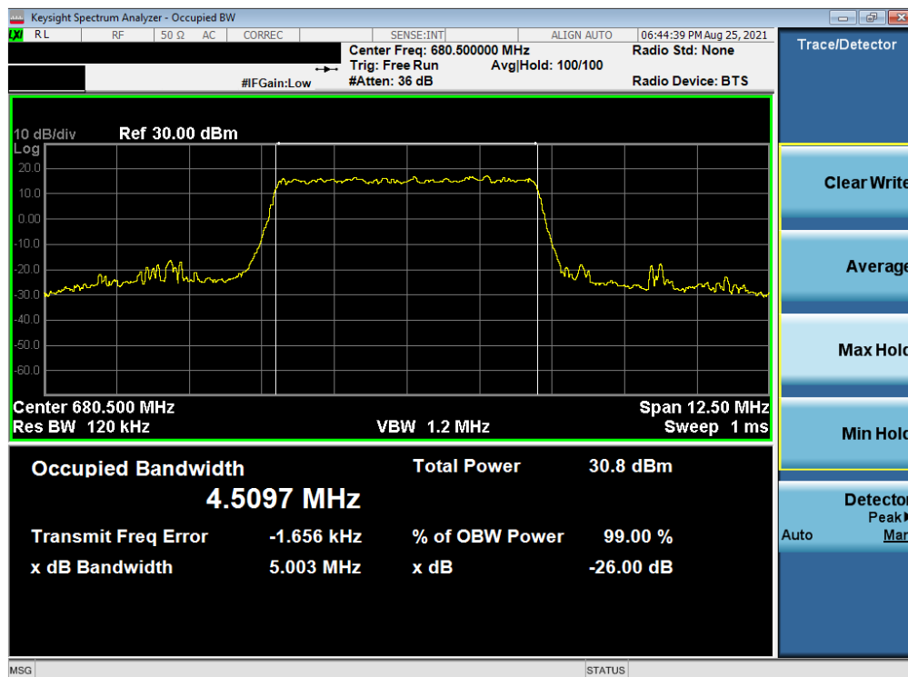
Plot 7-32. Occupied Bandwidth Plot (NR Band n71 - 5MHz CP-OFDM 16-QAM - Full RB - Ant I)
