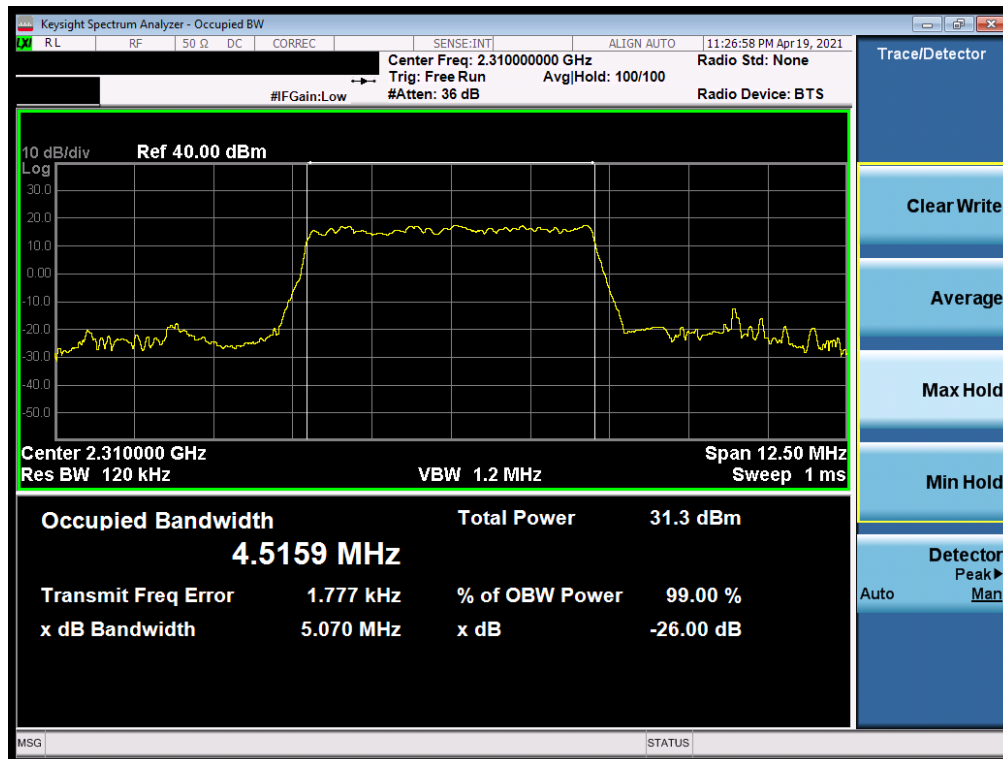
Plot 7-32. Occupied Bandwidth Plot (NR Band n30 - 5MHz \pi/2 BPSK - Full RB)
