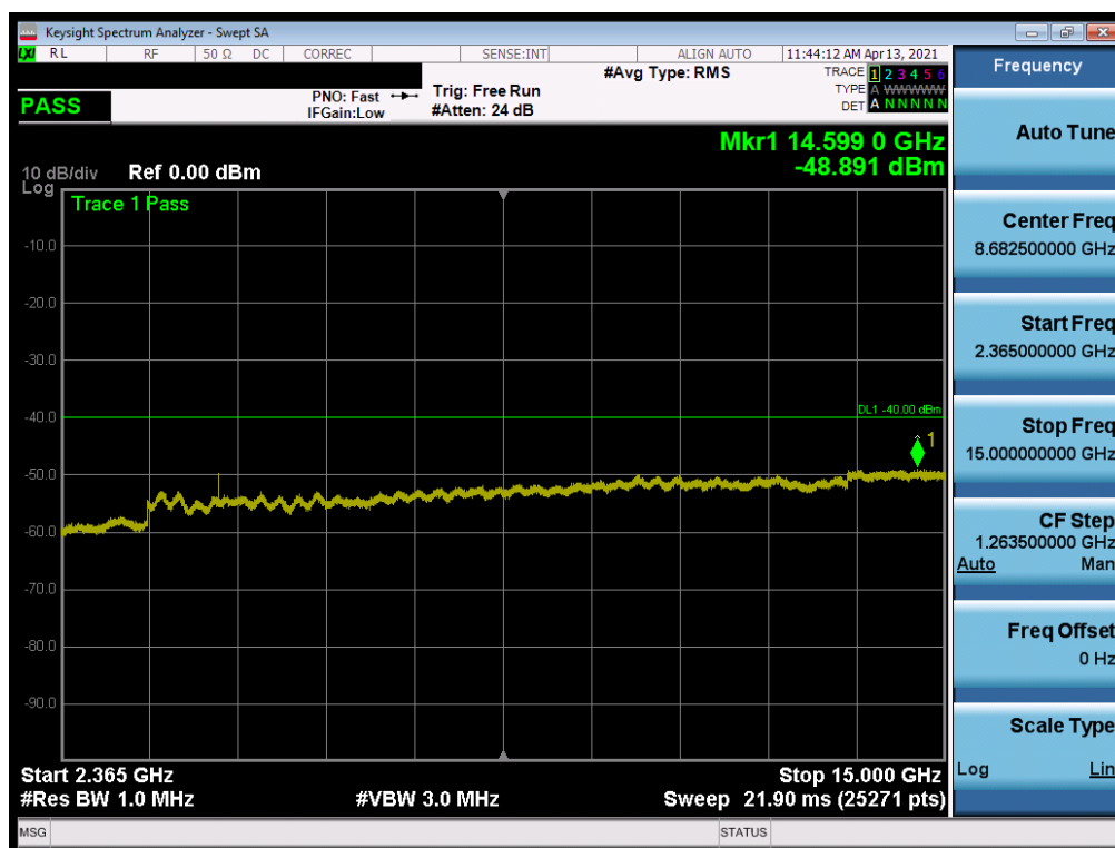
Plot 7-84. Conducted Spurious Plot (LTE Band 30 - 10MHz QPSK - RB Size 1, RB Offset 0)
