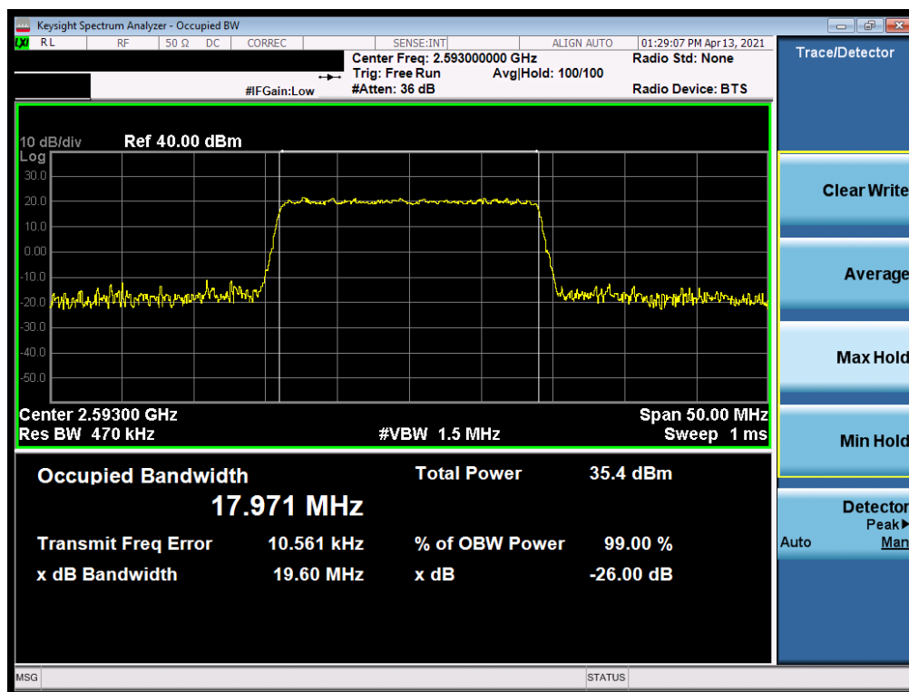
Plot 7-13. Occupied Bandwidth Plot (LTE Band 41(PC2) - 20MHz QPSK - Full RB)
