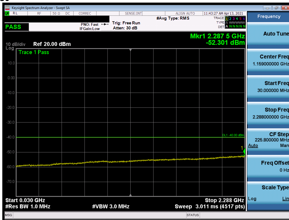
Plot 7-83. Conducted Spurious Plot (LTE Band 30 - 10MHz QPSK - RB Size 1, RB Offset 0)
