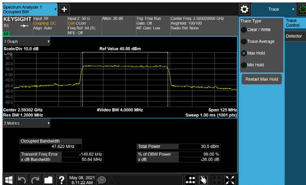
Plot 7-72. Occupied Bandwidth Plot (NR Band n41 - 50MHz QPSK - Full RB)
