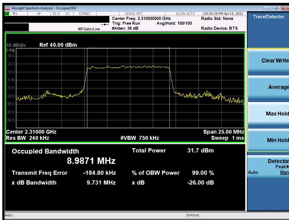
Plot 7-29. Occupied Bandwidth Plot (NR Band n30 - 10MHz \pi/2 BPSK - Full RB)
